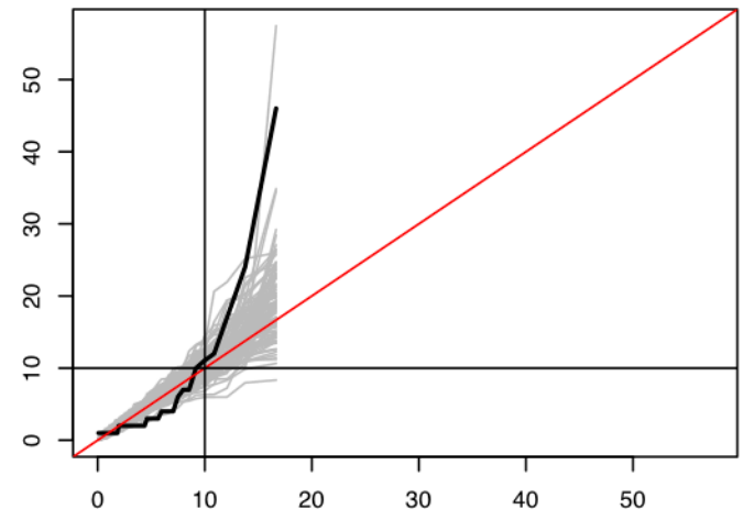
(e) Gamma QQ Plot: C57, M2, REM→NREM
