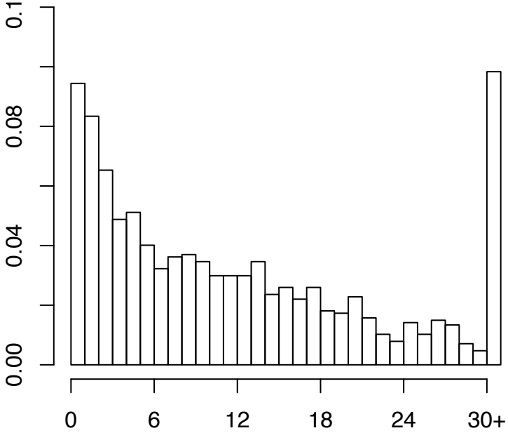
(e) REM→WAKE Bout Duration
