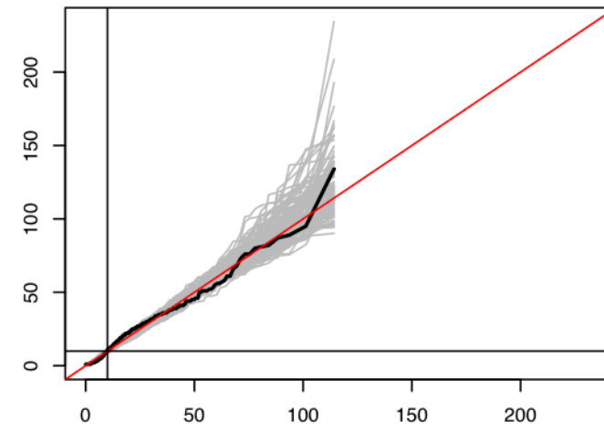
(g) Gamma QQ Plot: C57, M2, WAKE→NREM
