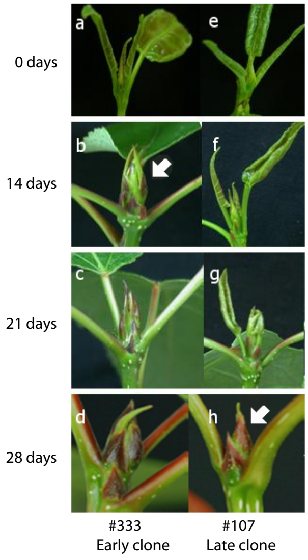
Supplementary Figure 1. (a-d) Characterization of bud set in the early (#333) and the late (#107) hybrid poplar clones (e-h) after short day treatment. Bud formation is indicated by the arrow.
