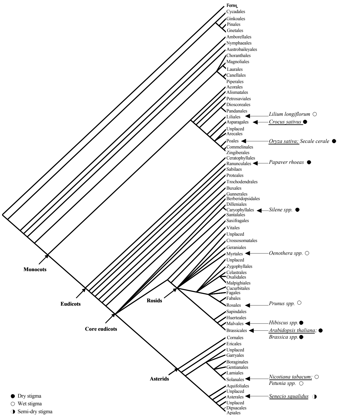
Figure S1. The phylogenetic distribution of species most widely used in studies of pollen-pistil interactions. The species for which pistil transcriptome data have been produced are underlined. The stigma state is indicated next to the species. The tree is based on APG II (2003).
