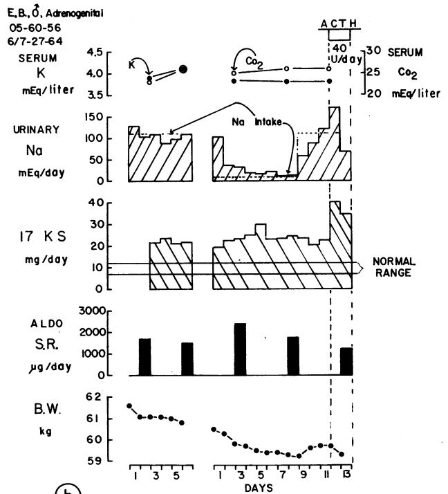
FIGURE 1 Design of experiment in patients studied without suppressive medication: (a) in D.H., who had previously been treated with prednisone; (b) in E.B., who had never been treated. Aldo SR , aldosterone secretion rate; KS , ketosteroid.
