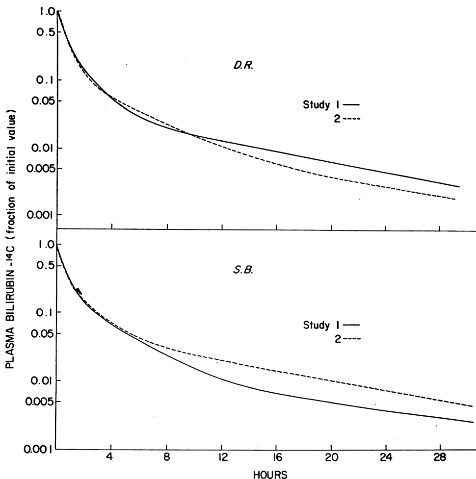
FIGURE 5 Paired bilirubin- 14 C clearance studies in two subjects. Lines represent computer fits to the data. Individual data points are not presented, but scatter in these studies was similar to that in Fig. 2. To facilitate comparison between studies, curves have been normalized to an initial value of unity.
