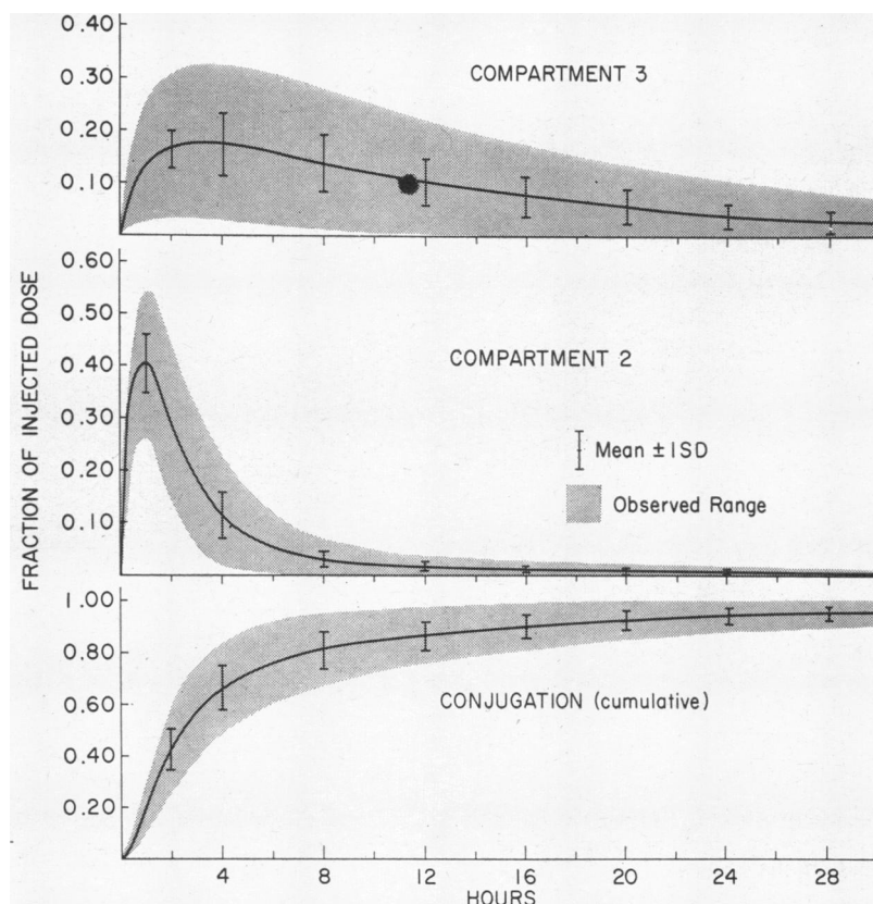
FIGURE 7 Isotope content of the extrahepatic extravascular (upper panel) and hepatic (middle panel) unconjugated bilirubin pools; and cumulative fraction of bilirubin- 14 C conjugated (lower panel) at various times after injection. This information is calculated by computer from the experimental bilirubin- 14 C plasma clearance data and the equations of the model.
