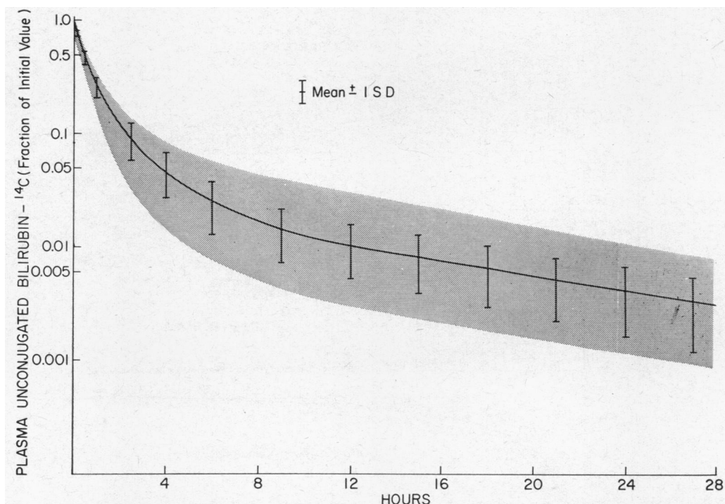
FIGURE 6 Composite of 19 plasma bilirubin- 14 C clearance studies in 13 normal subjects. Stippled area is the observed range. Solid line is the "average" curve corresponding to the mean values for the lambdas.
