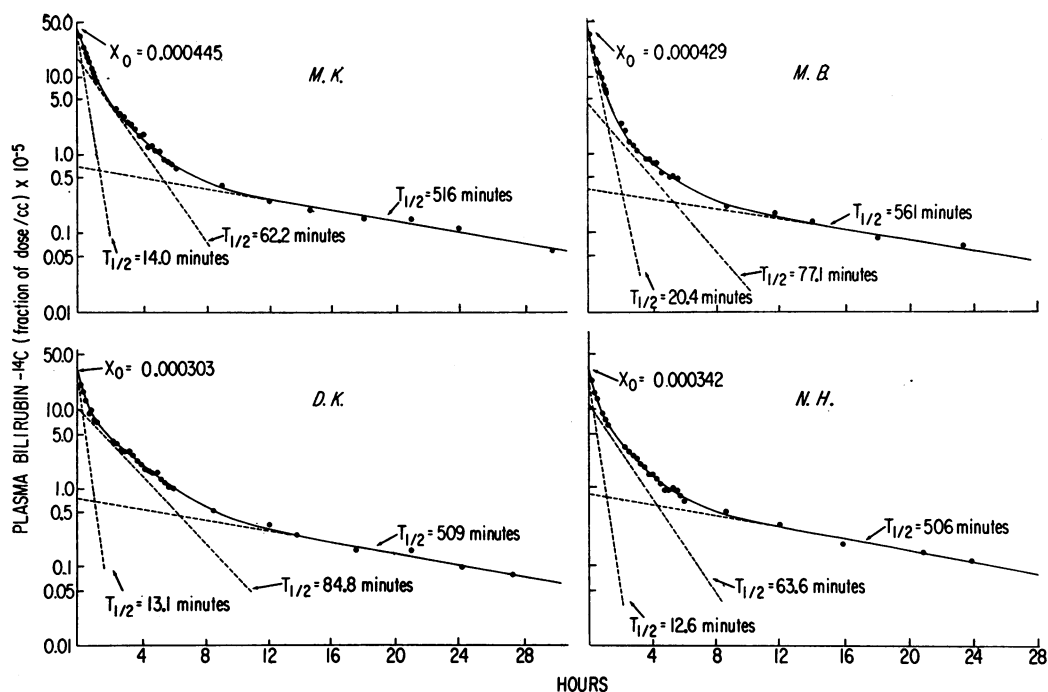
FIGURE 2 Bilirubin- 14 C disappearance curves in four subjects. Solid curve represents the computer fit to a three exponential function. Dotted lines are the individual exponential components. X_0 , the value at zero time, is the reciprocal of the initial distribution volume of the injected bilirubin- 14 C.
