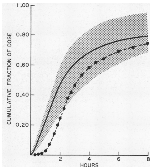
FIGURE 8 Cumulative recovery in the bile of intravenously injected bilirubin- 14 C in a patient with an external biliary fistula but with normal liver function (●--●--●). This data parallels the computer-calculated curve of cumulative bilirubin- 14 C conjugation in the same patient (solid line), with a time lag of approximately 1 hr. Volume of the biliary tree, calculated from this time lag and the average bile flow of 0.3 ml/min agrees closely with the value of 20 ml determined at operation by the injection of radiographic contrast media. Stippled area corresponds to the normal range for conjugation shown in Fig. 7.
