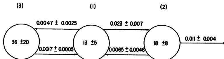
FIGURE 3 Weighted mean values for the parameters of the model. Compartments and pathways correspond to Fig. 1. Values within the circles are pool sizes (mean ±SD) in milligrams. Values above each arrow represent fractional transfer rates per minute in the direction of the arrow.
