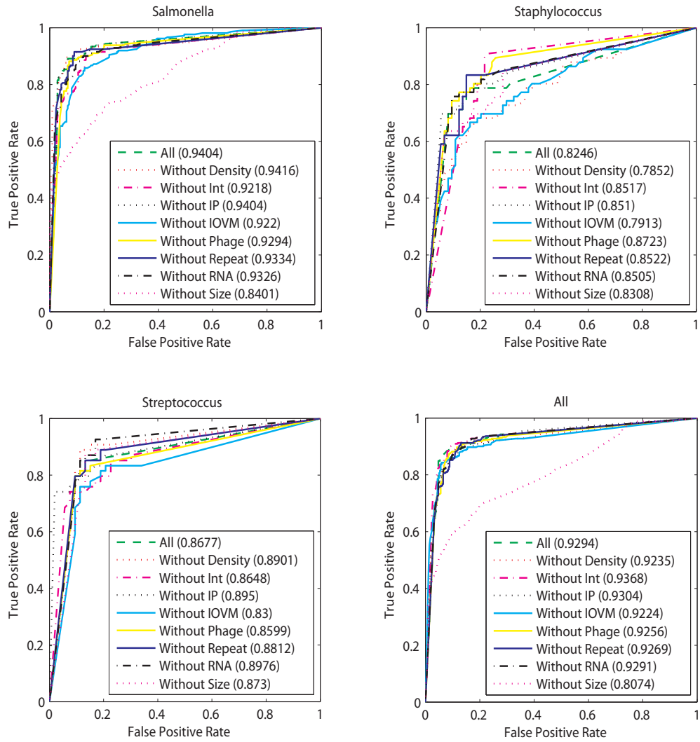
Fig. 1: ROC curves for the “leave-one-feature-out” models using adaboost.
