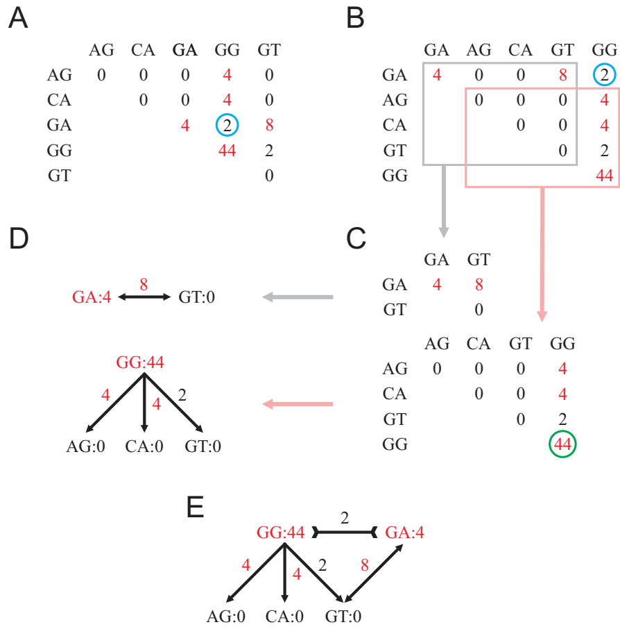
Figure S7: Protocol to distinguish among the different types of degenerate recognitions in the set of binding sites associated to a same recognition sequence ( K_{15}S_{16} in this example). See Text S1 for details.
