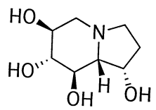
(+)-Castanospermine (2)
