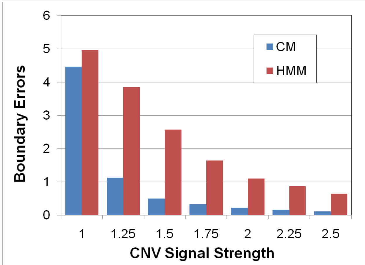
Supplementary Figure 1: Comparison of CopyMap and classical HMM algorithms. The horizontal axes shows the difference in signal strength \delta between the CNV- probes and probes with baseline copy number. We simulated a total of 100 CNVs. Each bar illustrates the average distance in probes between the start-and endpoints of correctly inferred CNV and the true CNV boundaries.
