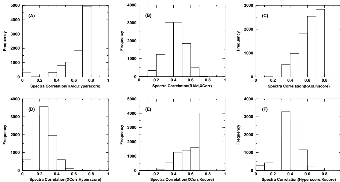
Figure S2. Histograms of correlations between filtering strategies. This Figure is the same as Figure 3 except that the 10,000 raw spectra used are profile data from the NHLBI data set. [1]
