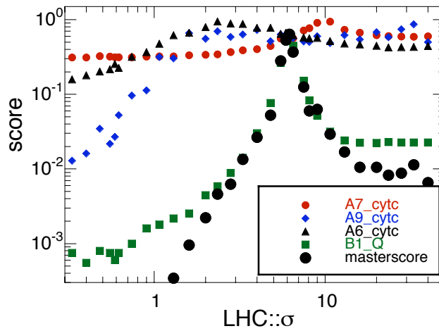
Figure S4: Scores from Some Experiments During the Scan of One Parameter
