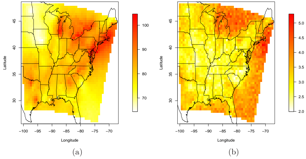
Figure 7 (Color version): (a) Posterior predictive mean and (b) posterior predictive standard deviation of the 4th highest ozone concentration during the period May 1–October 15 2001.
