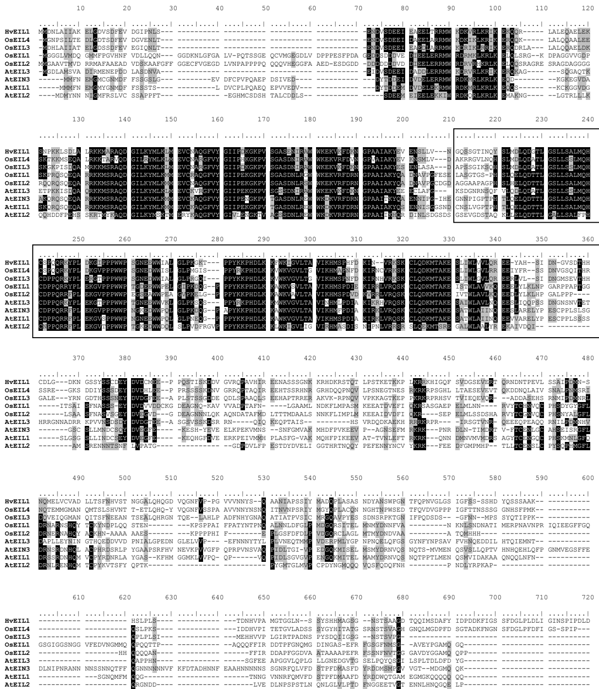
Supplemental Figure 3B. Sequence alignment of Ethylene Insensitive Like proteins. The sequences reported are, besides BEI1, from Oryza sativa and Arabidopsis thaliana . The box includes the \alpha -helical structures that constitute the DNA binding domain (Yamasaki et al.,2005).
