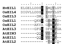
Supplemental Figure 3B. Sequence alignment of Ethylene Insensitive Like proteins. The sequences reported are, besides BEI1, from Oryza sativa and Arabidopsis thaliana . The box includes the \alpha -helical structures that constitute the DNA binding domain (Yamasaki et al.,2005).
