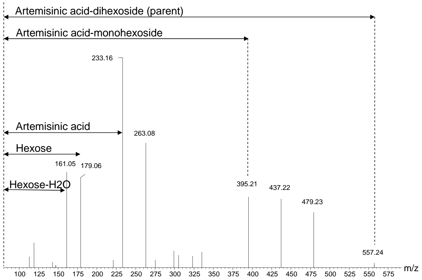
Figure S2: MSMS mass spectrum, showing collision mass fragments of artemisinin acid-12-β-diglucoside (m/z 557.24; [M-H]).
