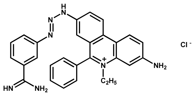
Isometamedium chloride
