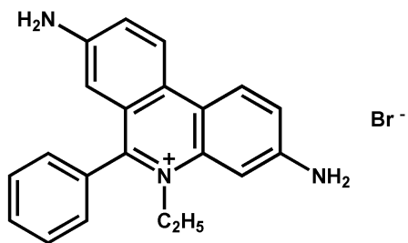
Ethidium bromide
