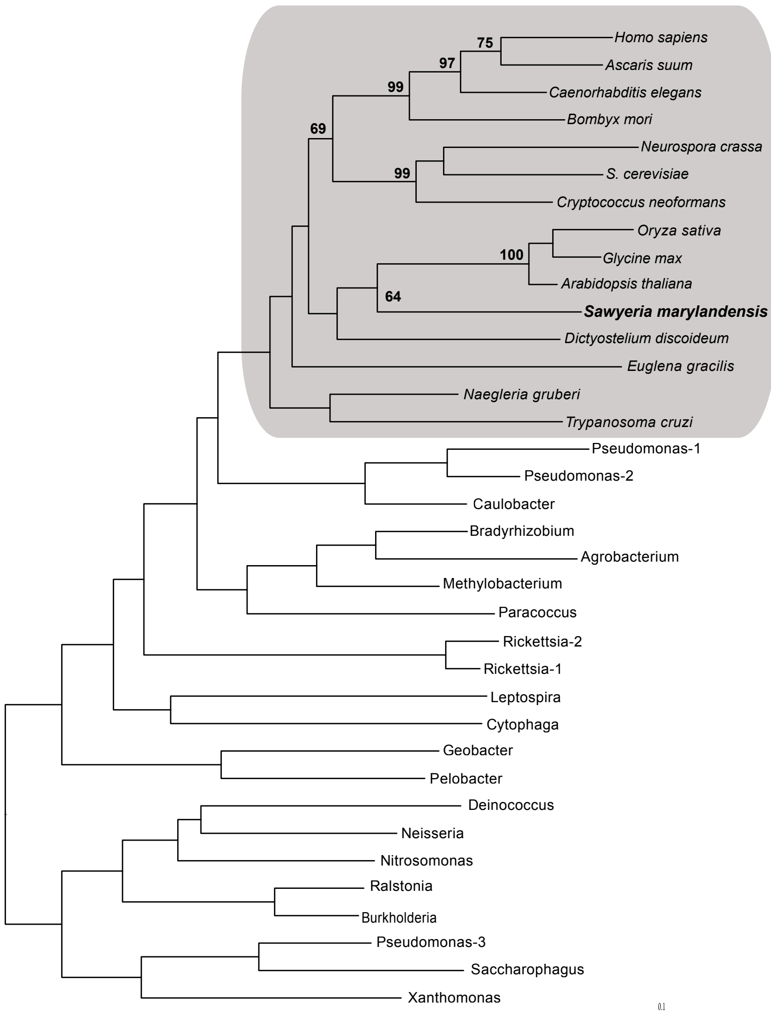
Fig. S8-Dihydrolipoamide dehydrogenase ML tree
