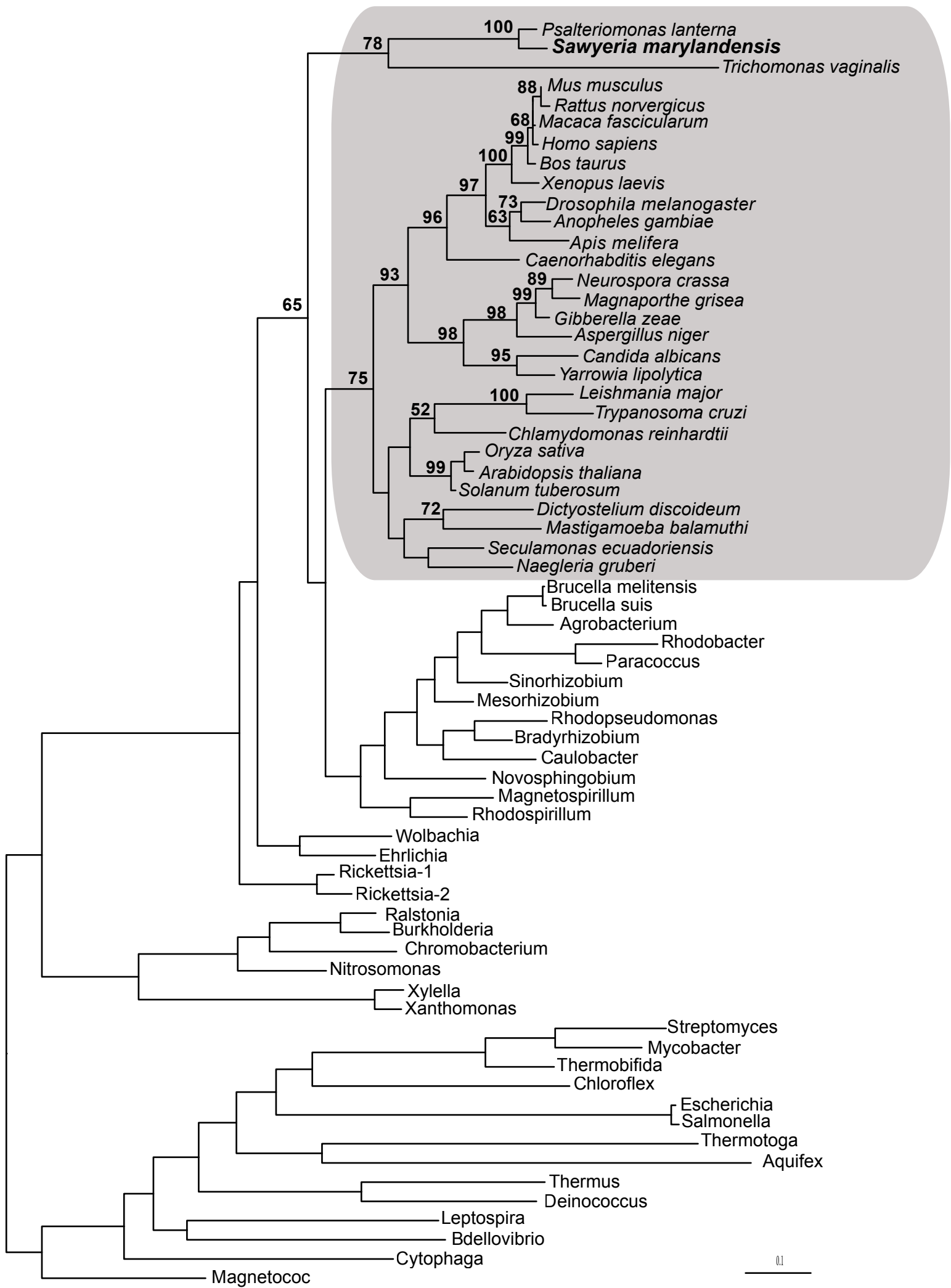
Fig. S3-Nuof ML tree
