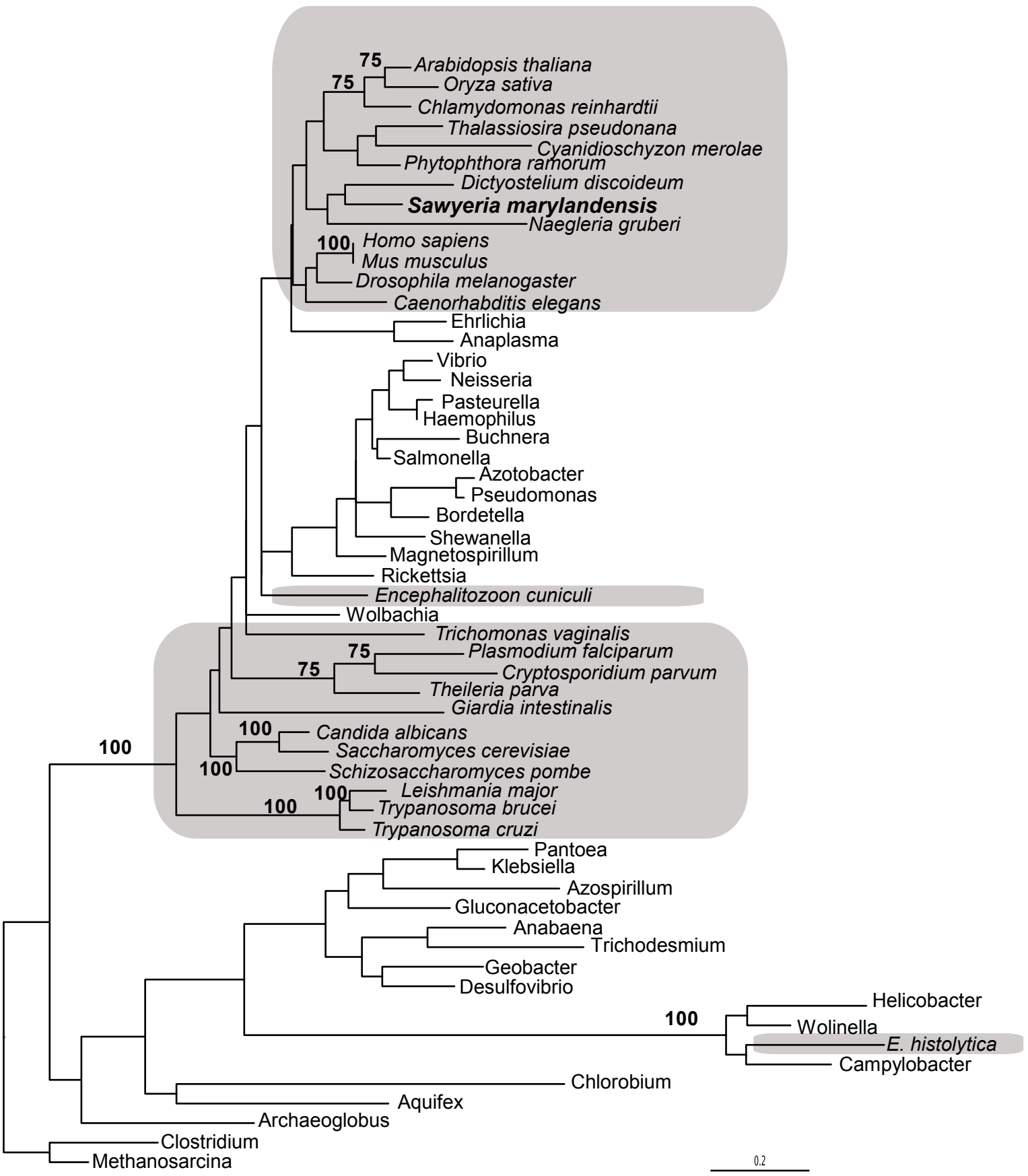
Fig. S7-18S ML tree
