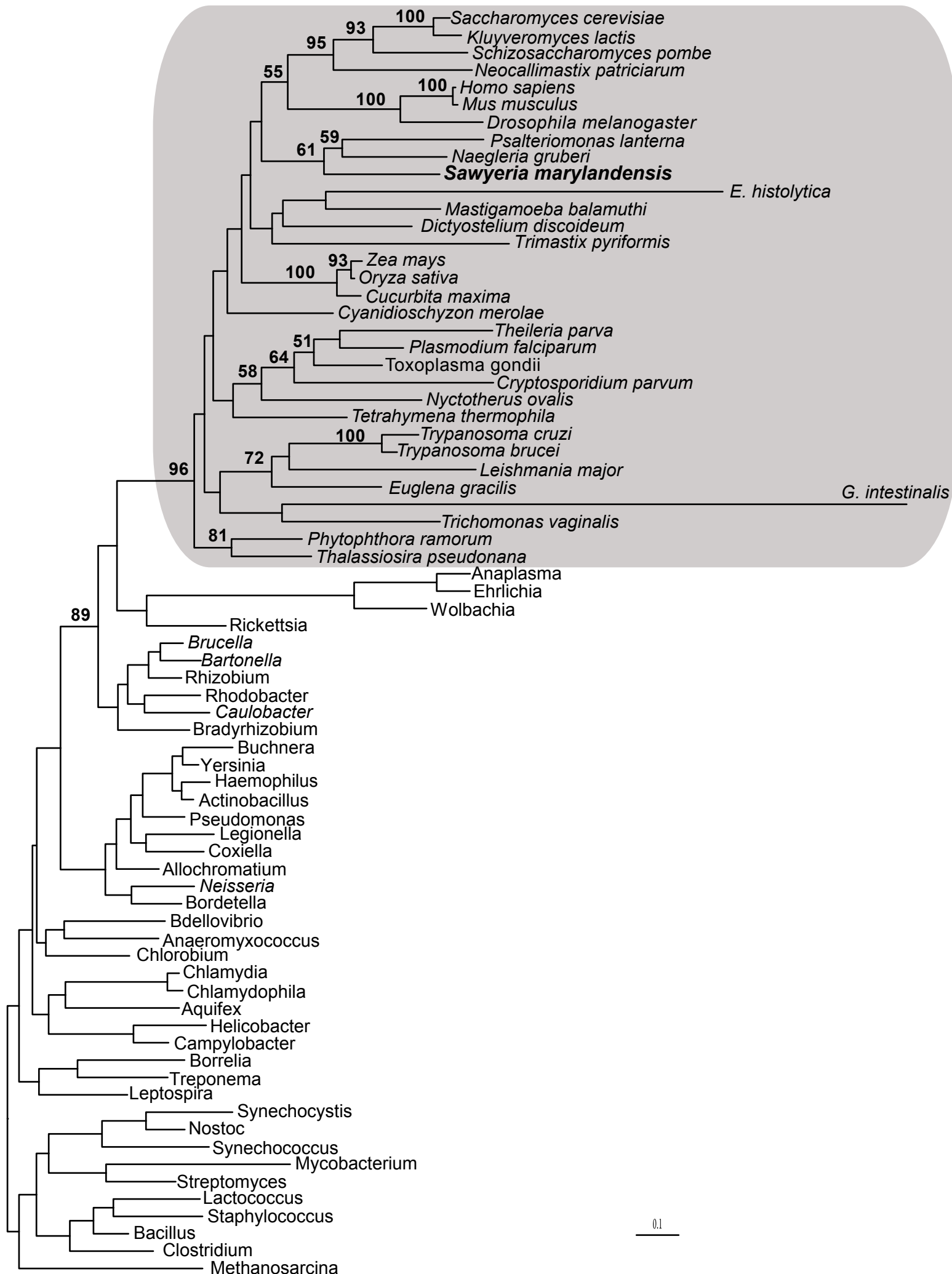
Fig. S5-cpn60 ML tree
