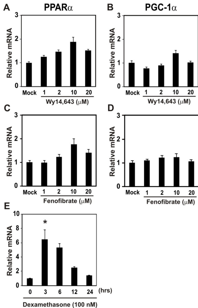
Supplemental figure 1. Effects of PPAR \alpha ligands on the mRNA levels of PPAR \alpha and PGC-1 \alpha . Hepatocytes isolated from mice were treated with 1, 2, 10 \mu M or 20 \mu M Wy14,643 (A and B) or fenofibrate (C and D), respectively for 24 h. PPAR \alpha (A and C) and PGC-1 \alpha (B and D) mRNA levels were measured by qPCR. E, Effect of dexamethasone on the PPAR \alpha mRNA levels was measured by qPCR as indicated. All the mRNA levels were normalized to Rplp0 mRNA levels.
