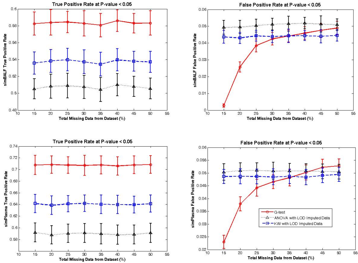
Figure S3. The true (A) and false (B) positive rates, respectively, for simBALF and true (C) and false (D) positive rates, respectively, for simPlasma. Data represent the mean and one SD from analyzing 100 simulated datasets.
