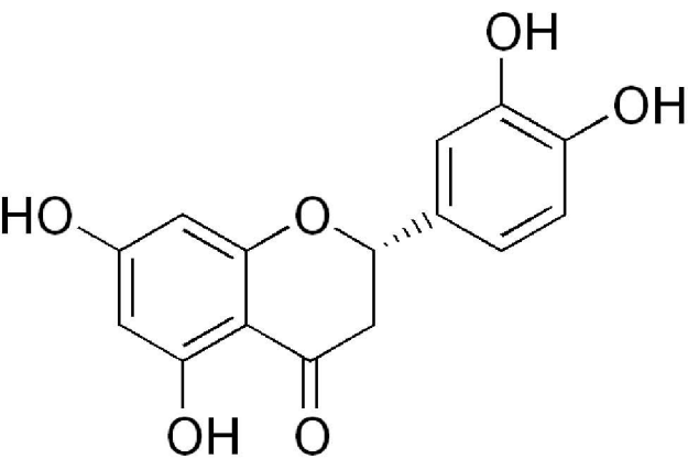
eriodictyol
