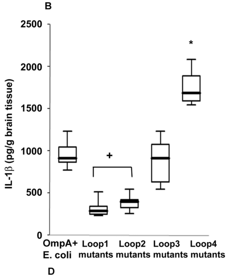
Supplementary Figure 4
