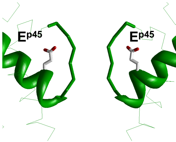
Figure S2. The outer pore in KcsA in which E^{p45} sidechains are projected towards the ascending limbs.
