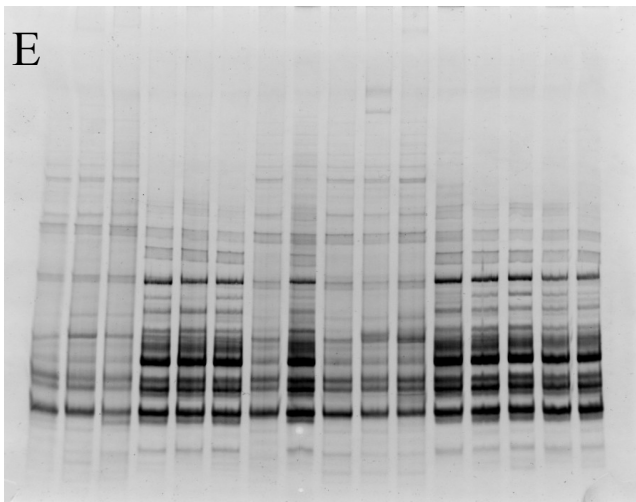
S2 DGGE profiles of the 16S rRNA gene. For all images numbers relate to plot numbers in the field. Symbols indicate treatments; ● = orgFM conCP, □ = conFM conCP, ○ = conFM orgCP, ■ = orgFM conCP. A = March after beans. B = June after beans. C = September after beans. D = March after barley. E = June after barley. F = September after barley.
