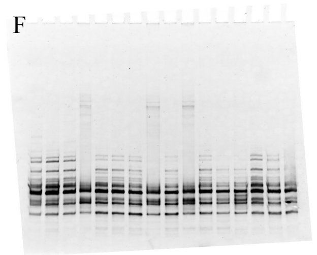
S2 DGGE profiles of the 16S rRNA gene. For all images numbers relate to plot numbers in the field. Symbols indicate treatments; ● = orgFM conCP, □ = conFM conCP, ○ = conFM orgCP, ■ = orgFM conCP. A = March after beans. B = June after beans. C = September after beans. D = March after barley. E = June after barley. F = September after barley.
