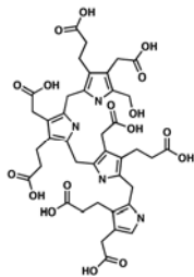
Hydroxymethylbilane
