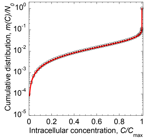
Figure S3. Validation of the solution methodology. Comparison of the numerical solution (symbols) obtained by integrating Eqs. (4) when D(C_i)=D_0 at steady state with the corresponding analytical solution (line) provided by Eq. (S6.4). Parameter values employed are listed in Table 1.
