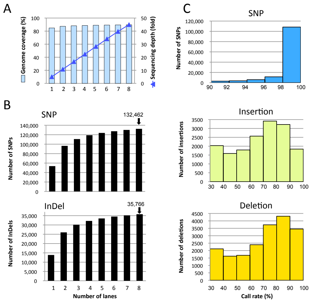
Supplementary Figure S2. Relationships among genome coverage, sequencing depth, call rate and the number of detected SNPs and InDels. (A) Blue bars correspond to the left vertical scale (% coverage of the genome by the mapped GA reads) and the blue line corresponds to the right vertical scale (sequencing depths merged stepwise). (B) The number of identified SNPs and InDels in each lane was merged stepwise. (C) Call rate (%) of SNPs, Insertions, and deletions.
