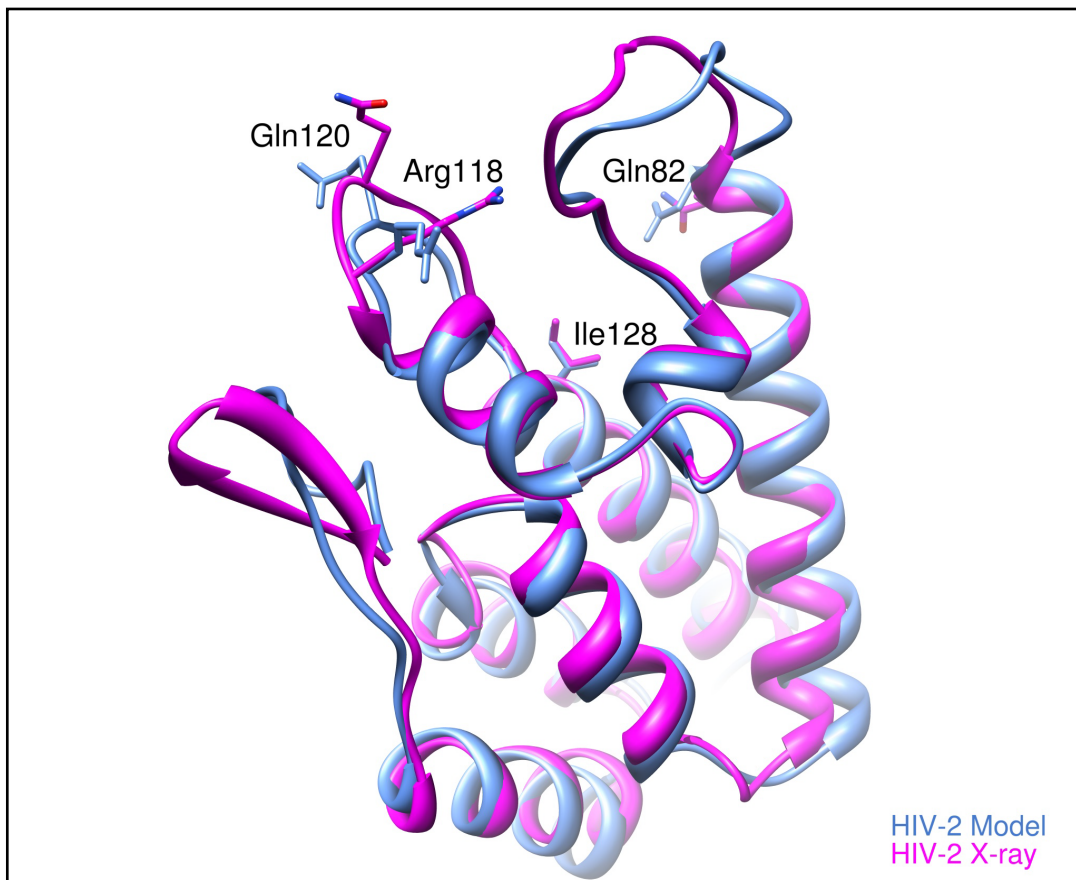
Figure S1. Superimposition between the predicted and the identified structure of the N-terminal domain of the capsid of HIV2.
