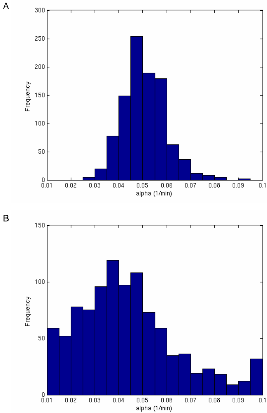
Supplementary Figure 1. Histograms of the basis function exponent (alpha) for simulated normoxic (A) and hypoxic (B) data. The spectra are for the 1000 simulations conducted for each tissue type at noise level 11.
