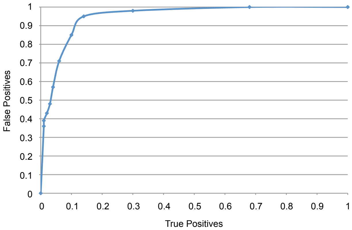
ROC curve of new HMMerThread data
