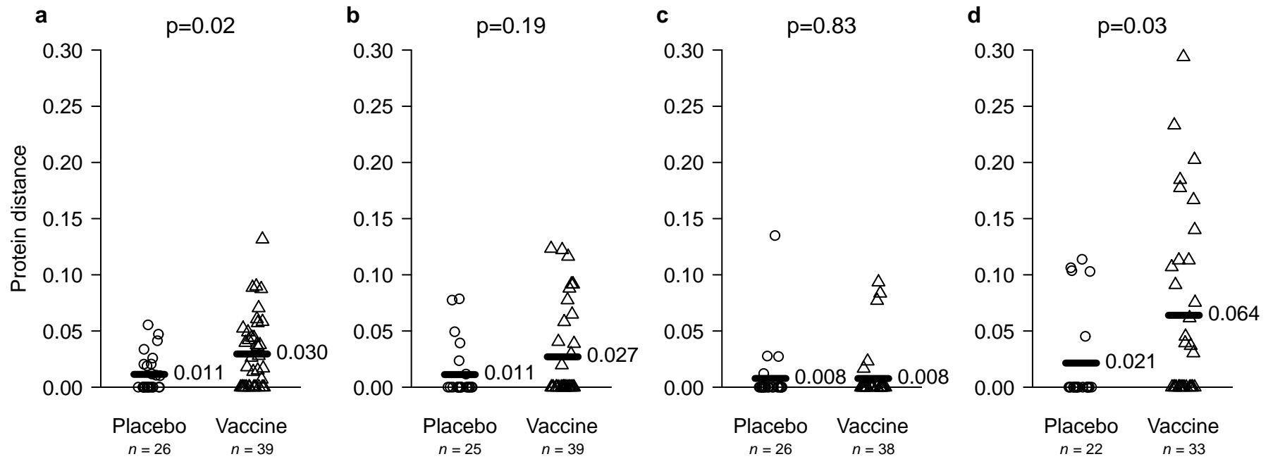
Supplementary Fig. 2. Epitope-specific protein distances between epitopes from founder sequences and the MRKAd5 insert sequence (Epipred). Comparison of epitopic distances across treatment assignment based on NetMHC predictions using Gag, Pol and Nef epitopes combined (a), or separately (b-d).
