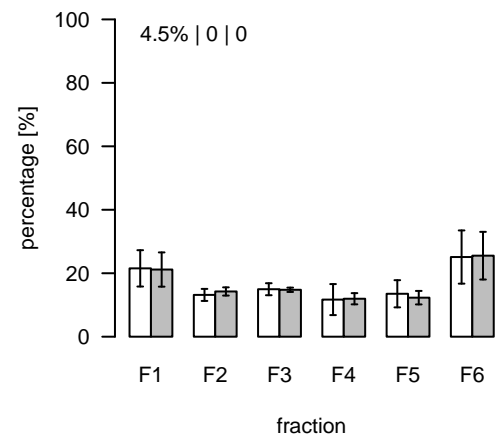
L1551 (m/z=782.513908; rt=8.05675) T/S Cluster: L-8.1-2
