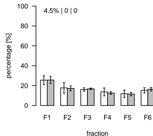
L1816 (m/z=747.576029; rt=9.03767) T/S Cluster: L-9-3
