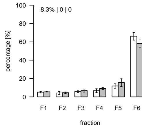
L774 (m/z=807.549961; rt=5.36093) T/S Cluster: L-5.4-2
