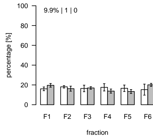
L1173 (m/z=391.288442; rt=6.65877) T/S Cluster: L-6.7-5
