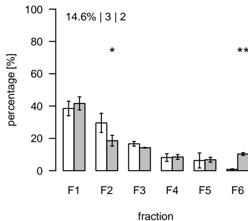
L1786 (m/z=716.526954; rt=8.91709) T/S Cluster: L-8.9-1
