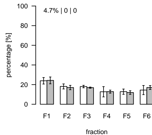
L1498 (m/z=378.279673; rt=7.9393) T/S Cluster: L-7.9-14
