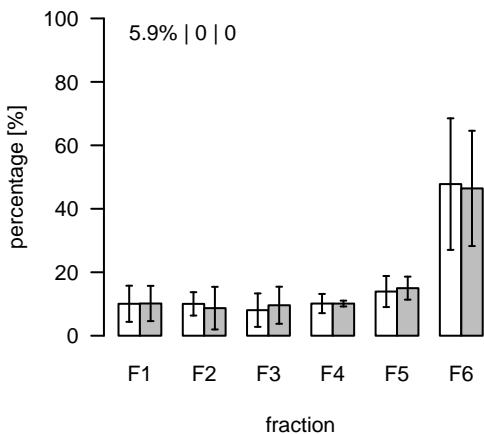
S450 (m/z=704.387894; rt=12.67521) T/S Cluster: S-12.7-4
