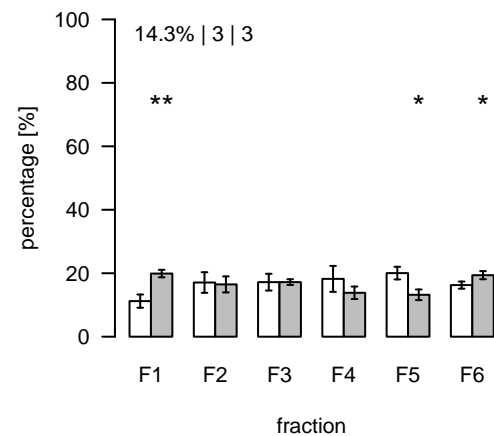
L2232 (m/z=551.634468; rt=11.30635) T/S Cluster: L-11.3-3
