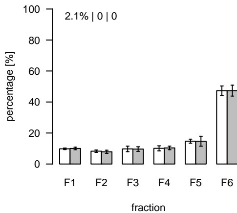
L519 (m/z=826.566902; rt=4.80063) T/S Cluster: L-4.8-10
