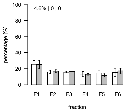
L380 (m/z=839.504151; rt=4.38093) T/S Cluster: L-4.4-7
