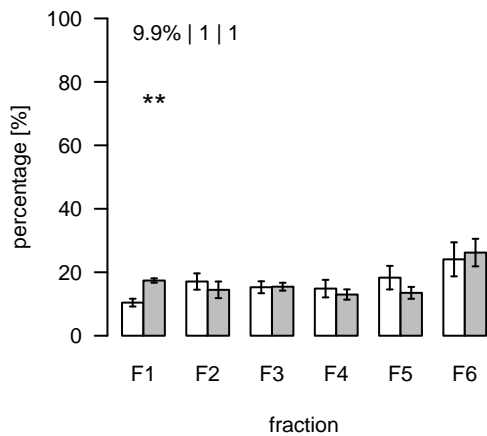
L2539 (m/z=417.122289; rt=14.79651) T/S Cluster: L-14.8-1
