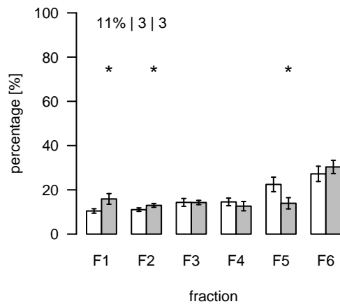
L921 (m/z=955.600851; rt=6.10552) T/S Cluster: L-6.1-2
