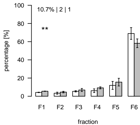
L27 (m/z=674.386117; rt=2.87155) T/S Cluster: L-2.9-1
