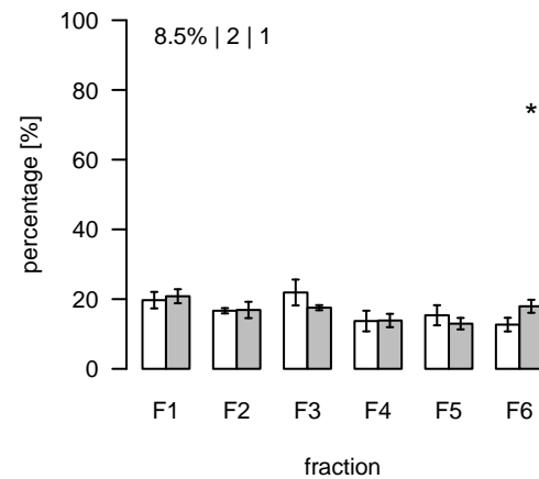
L2605 (m/z=823.761539; rt=15.5744) T/S Cluster: L-15.6-2
