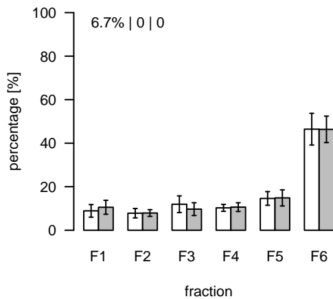
L2482 (m/z=435.787263; rt=12.38338) T/S Cluster: L-12.4-1
