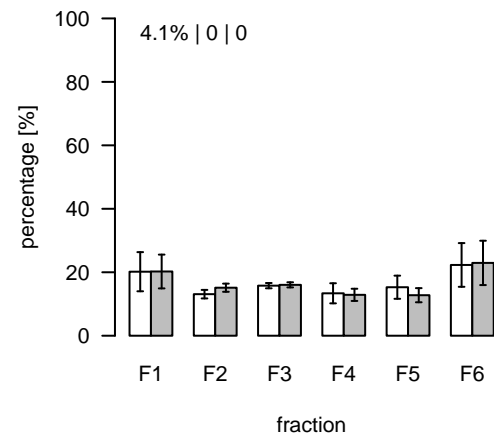
L1194 (m/z=390.274682; rt=6.66682) T/S Cluster: L-6.7-8
