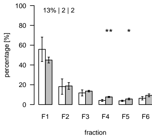
S584 (m/z=496.341211; rt=14.38789) T/S Cluster: S-14.4-2
