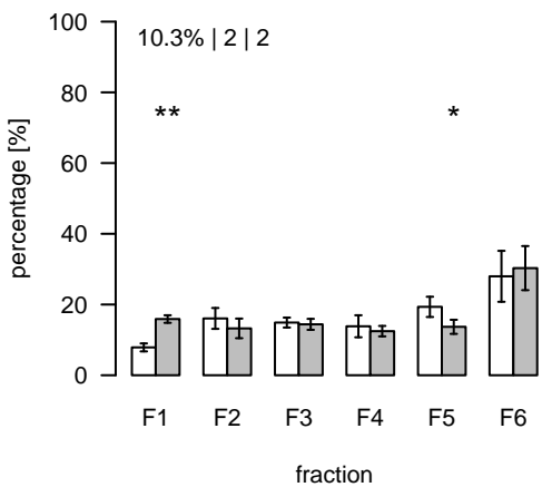
L2799 (m/z=1350.386176; rt=18.07326) T/S Cluster: L-18.1-1
