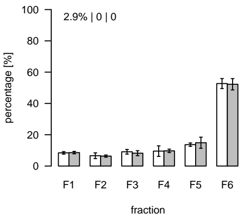
L927 (m/z=667.418257; rt=6.12452) T/S Cluster: L-6.1-1
