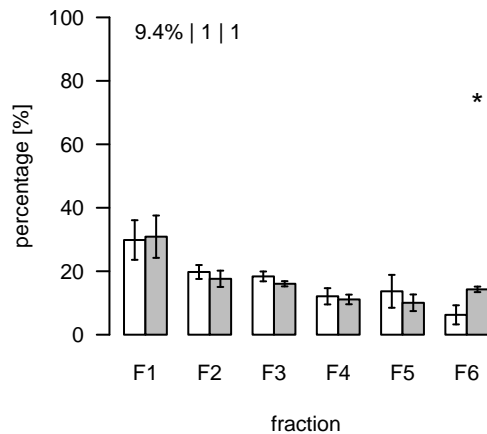
L1750 (m/z=784.589414; rt=8.87984) T/S Cluster: L-8.9-1
