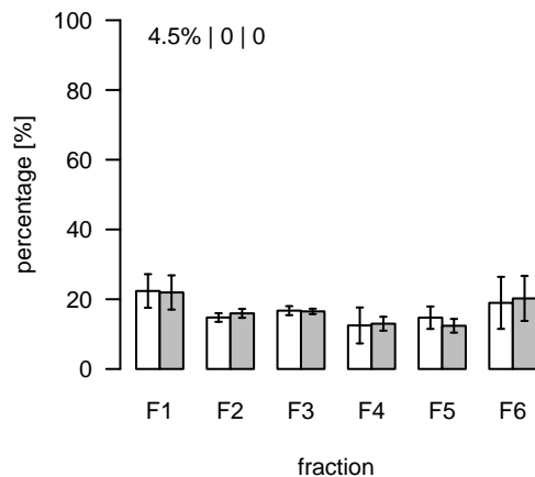
L1314 (m/z=782.53386; rt=7.32823) T/S Cluster: L-7.3-5
