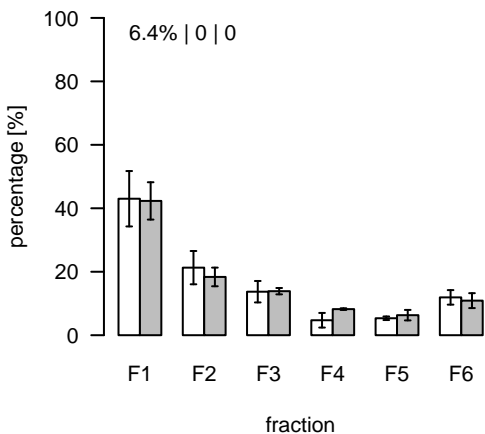
S659 (m/z=678.408826; rt=14.90934) T/S Cluster: S-14.9-2
