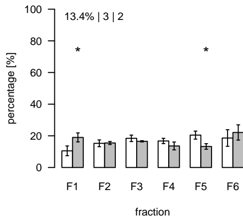
L2283 (m/z=341.24374; rt=11.32785) T/S Cluster: L-11.3-4
