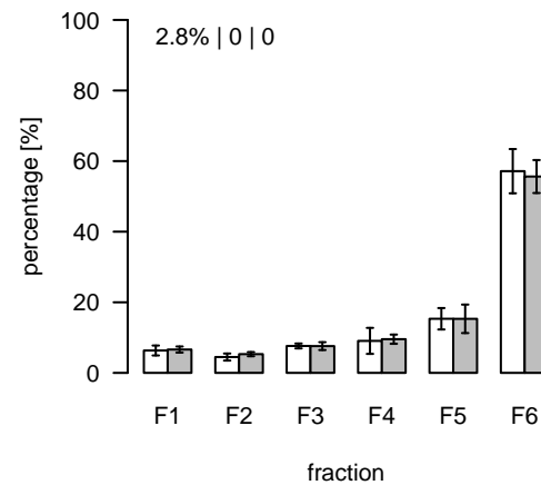
L573 (m/z=611.47042; rt=4.89589) T/S Cluster: L-4.9-9
