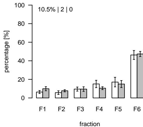
L1730 (m/z=895.529644; rt=8.74288) T/S Cluster: L-8.7-8
