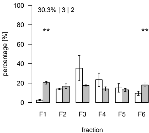
S878 (m/z=760.586698; rt=16.99649) T/S Cluster: S-17-13
