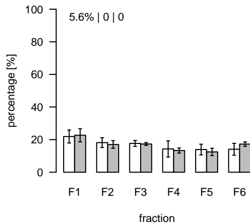
L1209 (m/z=776.584556; rt=6.69969) T/S Cluster: L-6.7-11
