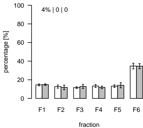
L2456 (m/z=873.584403; rt=11.84768) T/S Cluster: L-11.8-5
