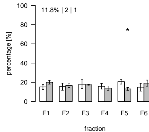
L850 (m/z=388.34341; rt=5.71303) T/S Cluster: L-5.7-11
