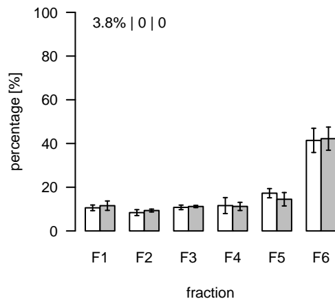
L1445 (m/z=466.320014; rt=7.90391) T/S Cluster: L-7.9-9
