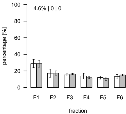
L307 (m/z=867.539361; rt=4.15645) T/S Cluster: L-4.2-5
