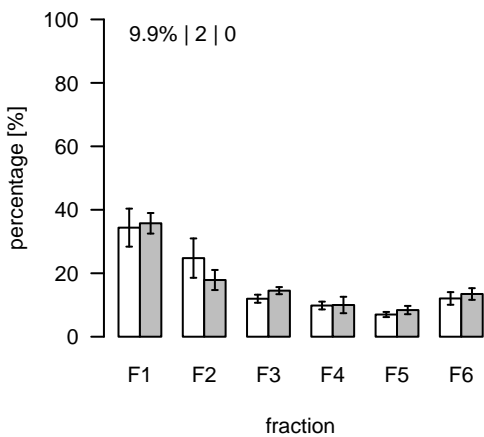
S847 (m/z=716.5699; rt=16.65967) T/S Cluster: S-16.7-2
