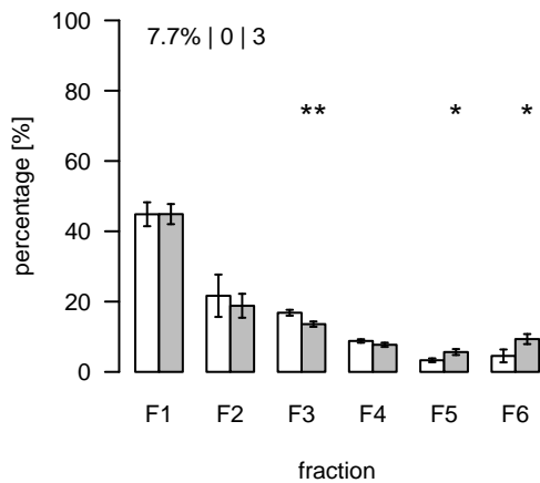
S209 (m/z=1159.348552; rt=7.19387) T/S Cluster: S-7.2-2
