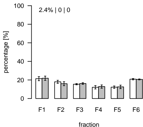
S527 (m/z=288.253794; rt=13.31835) T/S Cluster: S-13.3-3
