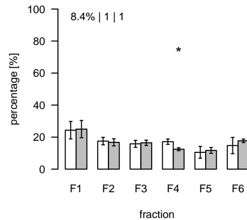
S306 (m/z=824.374478; rt=9.64238) T/S Cluster: S-9.6-3
