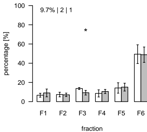
L1863 (m/z=454.262123; rt=9.43492) T/S Cluster: L-9.4-1
