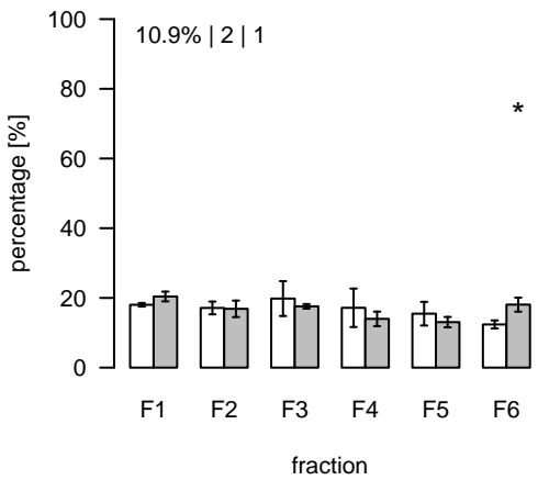
L2659 (m/z=877.820599; rt=15.83185) T/S Cluster: L-15.8-3
