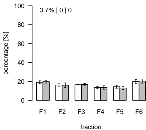
S489 (m/z=384.278791; rt=12.91247) T/S Cluster: S-12.9-20
