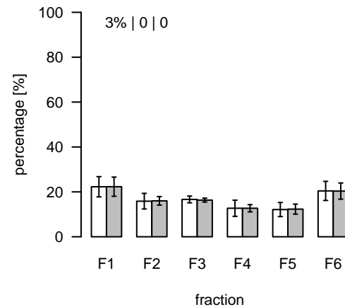
L878 (m/z=771.519222; rt=5.7223) T/S Cluster: L-5.7-7
