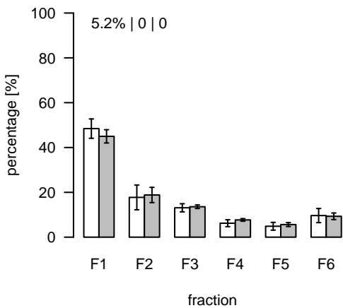
S57 (m/z=513.141113; rt=4.64567) T/S Cluster: S-4.6-1
