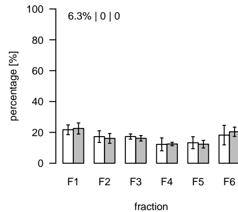
L633 (m/z=810.530376; rt=4.94704) T/S Cluster: L-4.9-22
