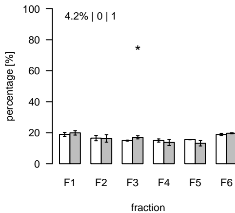
S421 (m/z=363.253758; rt=12.54992) T/S Cluster: S-12.5-13
