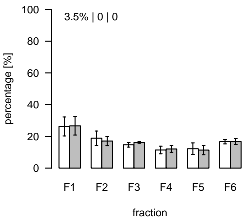
L230 (m/z=803.532361; rt=3.87479) T/S Cluster: L-3.9-4
