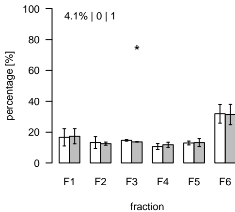
L2395 (m/z=869.551428; rt=11.37292) T/S Cluster: L-11.4-1
