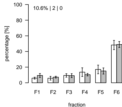
L1737 (m/z=898.500387; rt=8.74419) T/S Cluster: L-8.7-8
