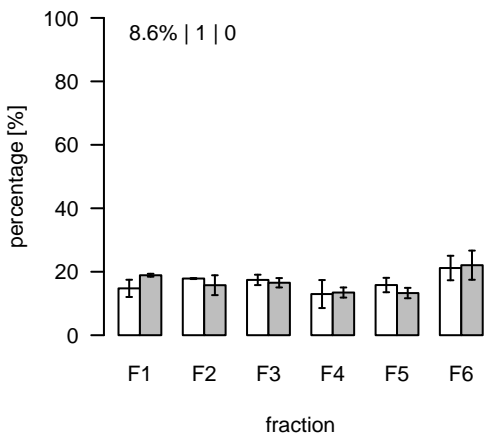
L2132 (m/z=388.343887; rt=10.5259) T/S Cluster: L-10.5-18
