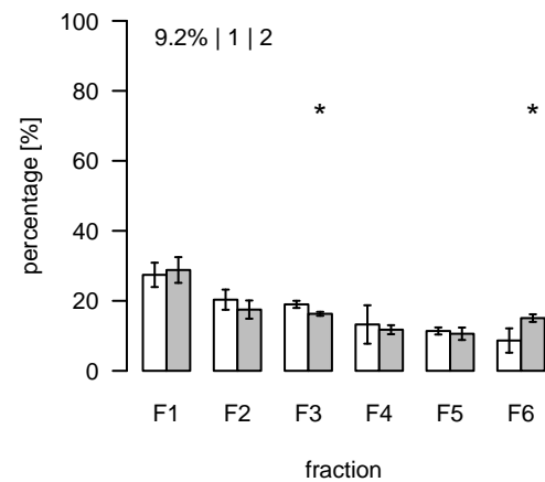
L1691 (m/z=759.536817; rt=8.70704) T/S Cluster: L-8.7-5
