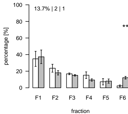
L1572 (m/z=714.510935; rt=8.1307) T/S Cluster: L-8.1-3
