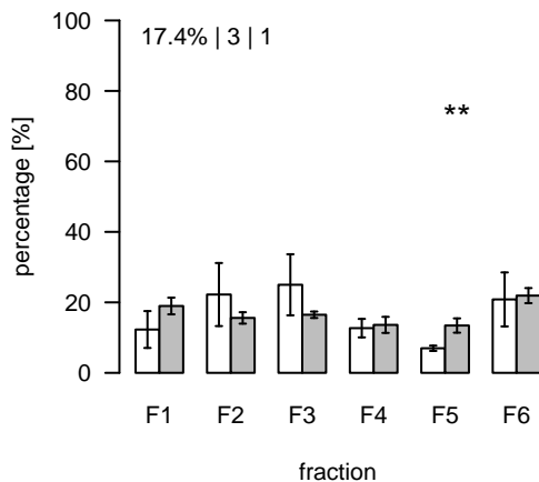
S875 (m/z=835.541657; rt=16.98974) T/S Cluster: S-17-11
