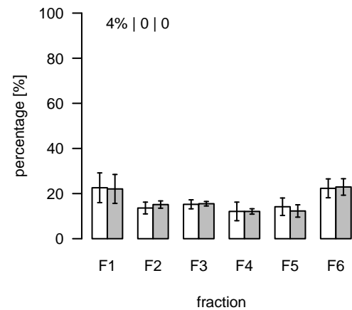
L1553 (m/z=785.583208; rt=8.05686) T/S Cluster: L-8.1-2
