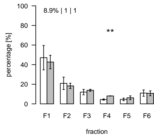
S692 (m/z=651.403592; rt=15.39067) T/S Cluster: S-15.4-1
