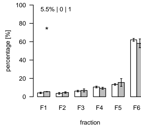
L794 (m/z=551.414595; rt=5.51041) T/S Cluster: L-5.5-2
