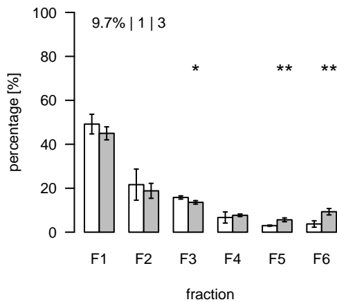
S205 (m/z=1174.367296; rt=7.19304) T/S Cluster: S-7.2-2
