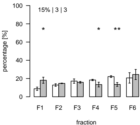
L2365 (m/z=1384.927902; rt=11.32866) T/S Cluster: L-11.3-23
