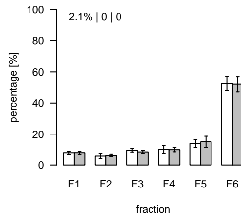
L835 (m/z=950.618069; rt=5.70319) T/S Cluster: L-5.7-1
