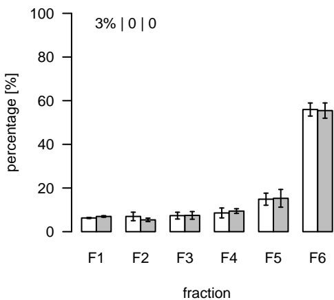
L92 (m/z=984.600309; rt=3.50095) T/S Cluster: L-3.5-1
