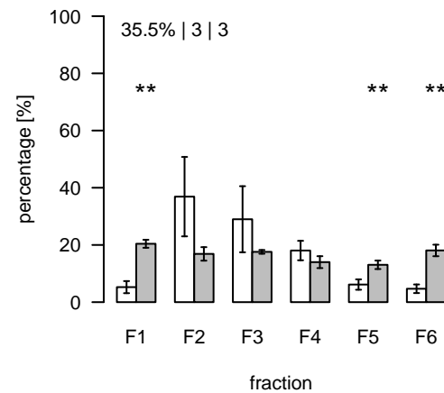
S883 (m/z=717.528996; rt=16.99959) T/S Cluster: S-17-15
