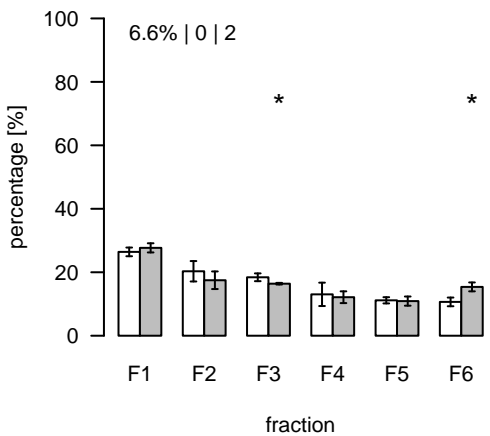
L2139 (m/z=816.638622; rt=10.58577) T/S Cluster: L-10.6-2
