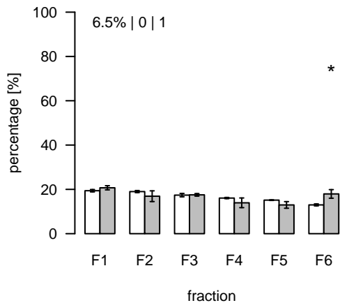
L2678 (m/z=924.313517; rt=15.84451) T/S Cluster: L-15.8-4
