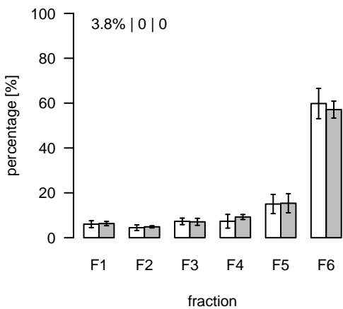
L916 (m/z=463.797187; rt=5.9589) T/S Cluster: L-6-1
