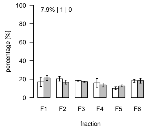
S729 (m/z=664.460749; rt=15.81597) T/S Cluster: S-15.8-6
