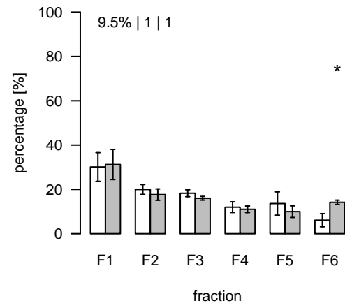
L1746 (m/z=784.556693; rt=8.87911) T/S Cluster: L-8.9-1
