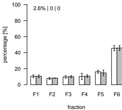
L1886 (m/z=468.833211; rt=9.52973) T/S Cluster: L-9.5-5
