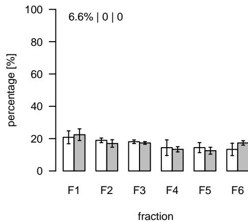
L1208 (m/z=388.293339; rt=6.69962) T/S Cluster: L-6.7-11
