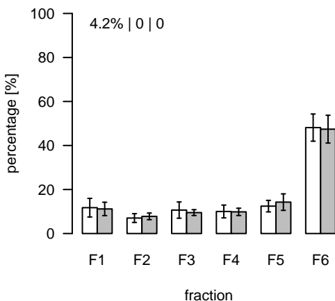
L1641 (m/z=901.554022; rt=8.62948) T/S Cluster: L-8.6-6
