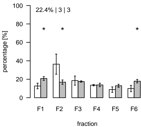
S888 (m/z=837.550518; rt=17.03846) T/S Cluster: S-17-19
