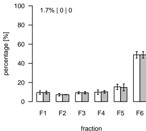
L1885 (m/z=312.226282; rt=9.52963) T/S Cluster: L-9.5-5
