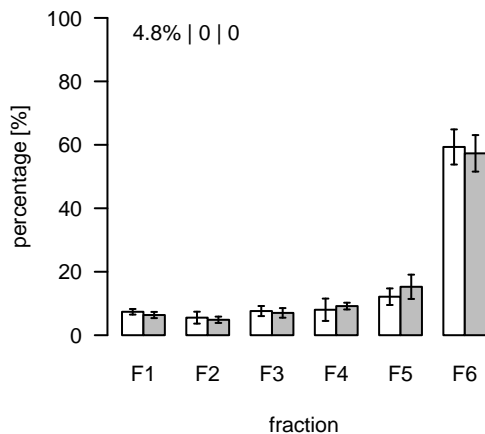
L1896 (m/z=772.597402; rt=9.5609) T/S Cluster: L-9.6-1
