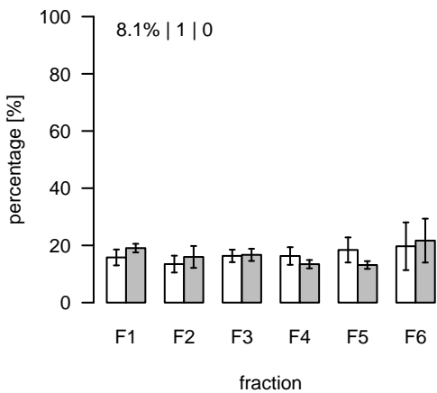
L1424 (m/z=953.541784; rt=7.8852) T/S Cluster: L-7.9-3
