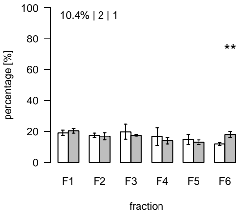
L2649 (m/z=851.806162; rt=15.82873) T/S Cluster: L-15.8-3
