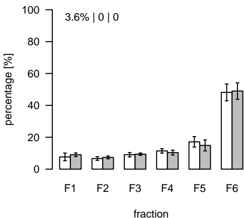
L1811 (m/z=961.672488; rt=8.96542) T/S Cluster: L-9-2
