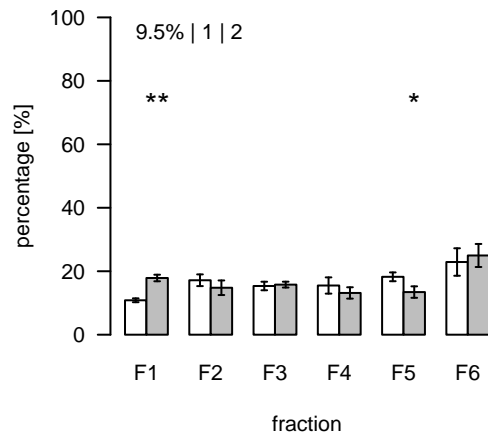
L2629 (m/z=985.280045; rt=15.80964) T/S Cluster: L-15.8-1
