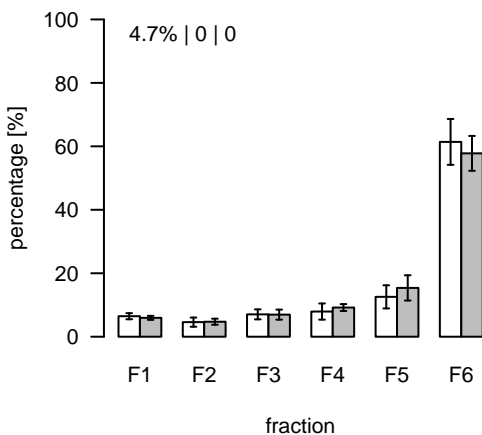
L1741 (m/z=796.598695; rt=8.84689) T/S Cluster: L-8.8-2
