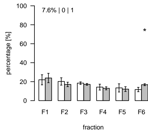
L301 (m/z=338.229676; rt=4.15457) T/S Cluster: L-4.2-4
