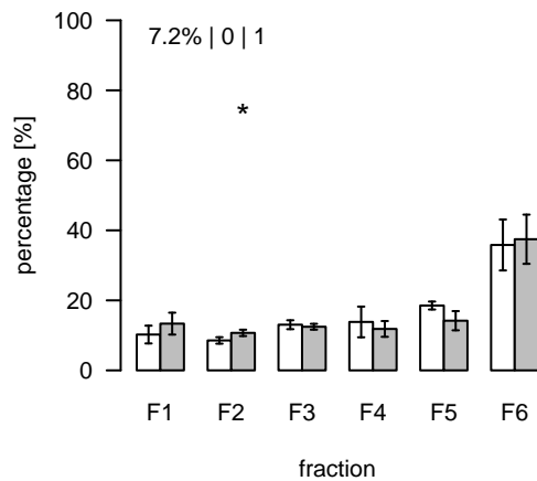
L1145 (m/z=958.634896; rt=6.65361) T/S Cluster: L-6.7-3
