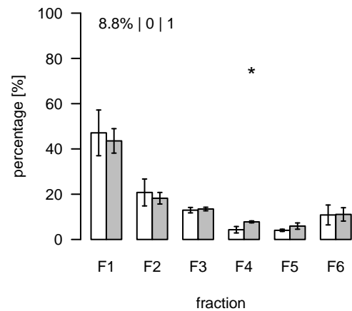
S680 (m/z=636.402912; rt=15.19723) T/S Cluster: S-15.2-1
