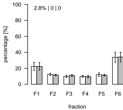
S844 (m/z=785.463024; rt=16.57796) T/S Cluster: S-16.6-1
