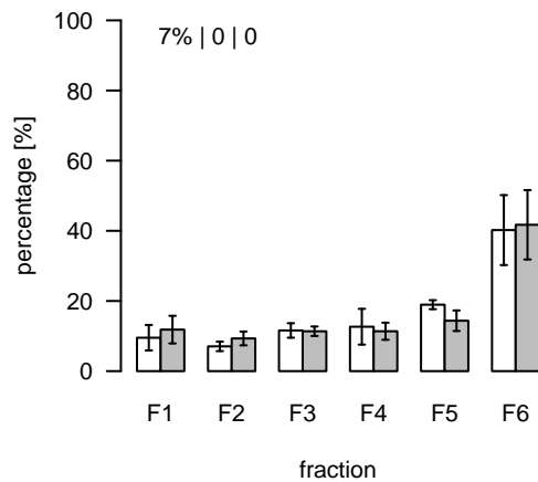
L1069 (m/z=255.188646; rt=6.54762) T/S Cluster: L-6.5-1
