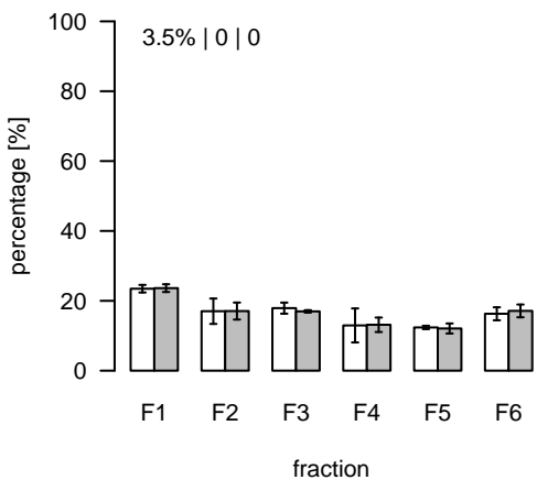
L2436 (m/z=422.35151; rt=11.74282) T/S Cluster: L-11.7-3
