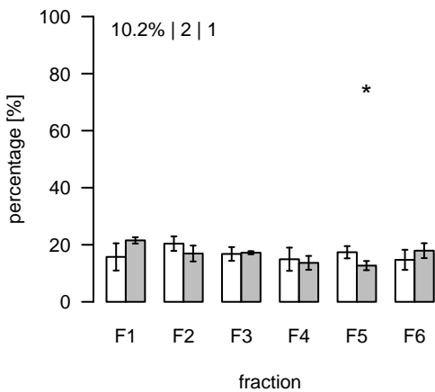
S910 (m/z=437.777035; rt=19.02028) T/S Cluster: S-19-1
