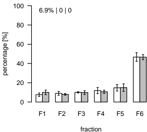
L1587 (m/z=923.486904; rt=8.20007) T/S Cluster: L-8.2-3
