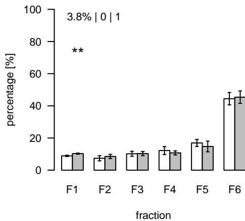
L856 (m/z=947.570531; rt=5.7143) T/S Cluster: L-5.7-1
