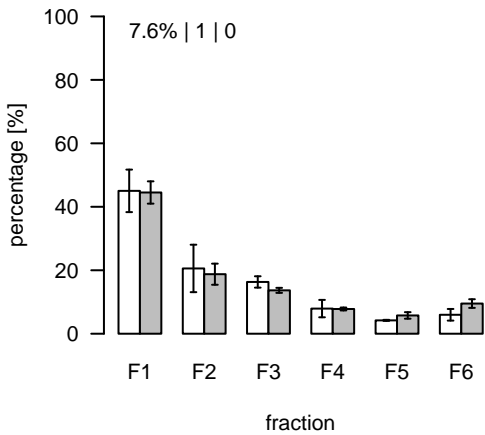
S183 (m/z=297.584273; rt=6.58032) T/S Cluster: S-6.6-2
