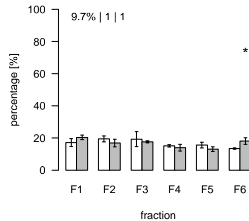
L2560 (m/z=806.726142; rt=15.17061) T/S Cluster: L-15.2-1
