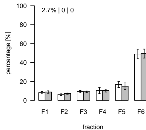
L1655 (m/z=935.578986; rt=8.64251) T/S Cluster: L-8.6-6
