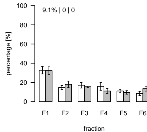
L768 (m/z=804.540482; rt=5.3383) T/S Cluster: L-5.3-7
