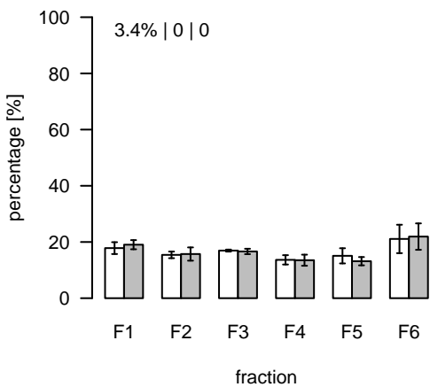
L996 (m/z=802.59213; rt=6.30747) T/S Cluster: L-6.3-1
