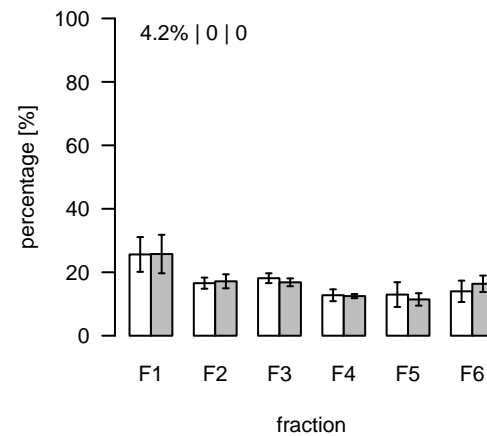
L805 (m/z=832.527223; rt=5.55428) T/S Cluster: L-5.6-3
