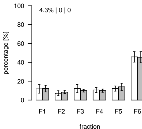
L1640 (m/z=901.52216; rt=8.62753) T/S Cluster: L-8.6-6
