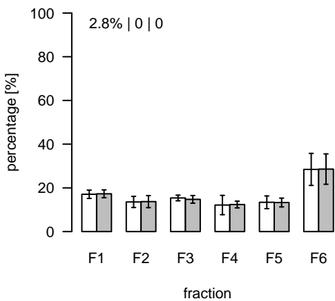
L993 (m/z=800.54395; rt=6.30598) T/S Cluster: L-6.3-1
