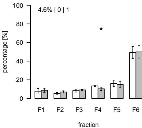
L1335 (m/z=795.577133; rt=7.34697) T/S Cluster: L-7.3-3
