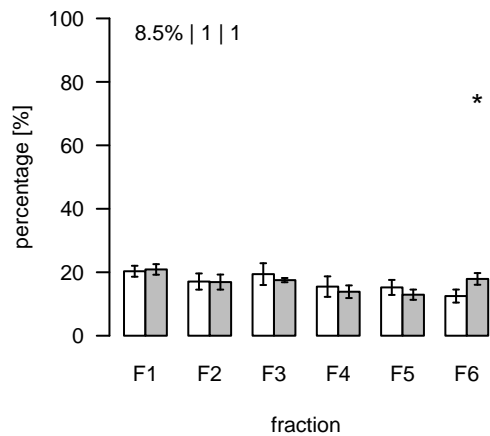
L2613 (m/z=876.801058; rt=15.58918) T/S Cluster: L-15.6-1
