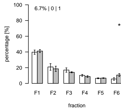
S92 (m/z=360.113923; rt=4.70422) T/S Cluster: S-4.7-1
