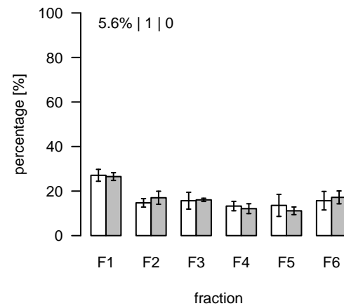
L820 (m/z=790.565291; rt=5.67597) T/S Cluster: L-5.7-2
