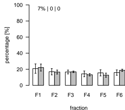
L2077 (m/z=865.517332; rt=10.48891) T/S Cluster: L-10.5-3
