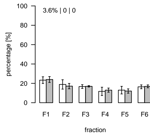
L389 (m/z=809.577932; rt=4.38891) T/S Cluster: L-4.4-9
