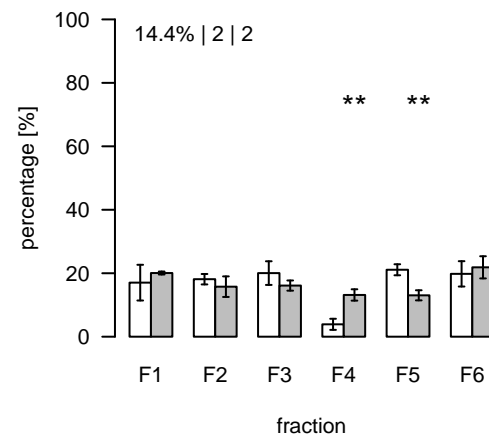
S310 (m/z=437.730124; rt=9.7917) T/S Cluster: S-9.8-2
