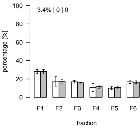
L1263 (m/z=366.78838; rt=7.16412) T/S Cluster: L-7.2-1
