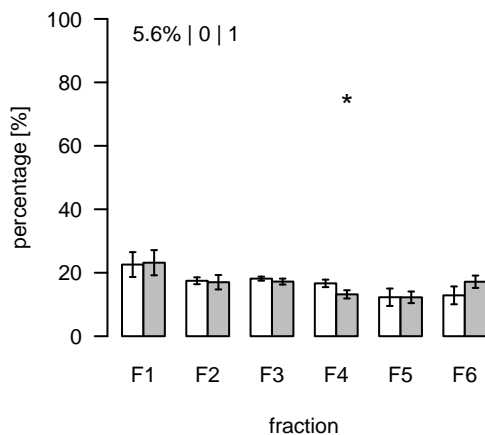
L1509 (m/z=378.264178; rt=7.94069) T/S Cluster: L-7.9-14
