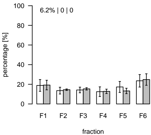
L142 (m/z=842.547932; rt=3.65278) T/S Cluster: L-3.7-3
