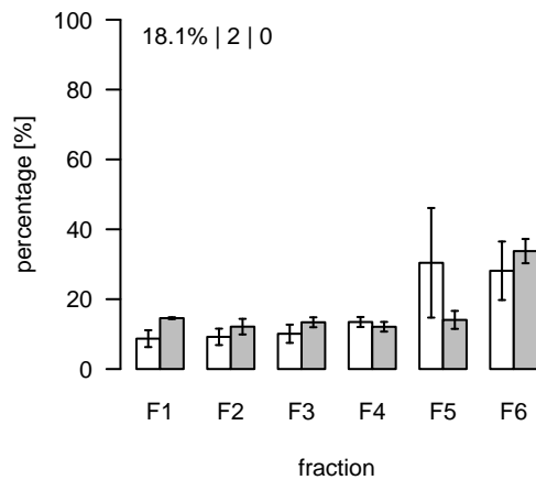
L1133 (m/z=761.499771; rt=6.64175) T/S Cluster: L-6.6-12
