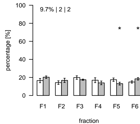
L778 (m/z=409.272152; rt=5.39959) T/S Cluster: L-5.4-3
