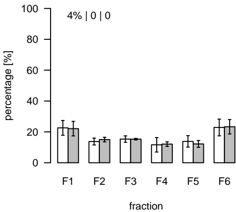
L1545 (m/z=261.19637; rt=8.05663) T/S Cluster: L-8.1-2
