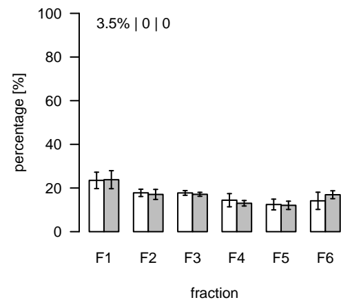
L1496 (m/z=252.855676; rt=7.93923) T/S Cluster: L-7.9-14
