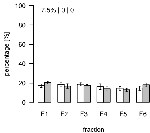
L2740 (m/z=934.883015; rt=16.54327) T/S Cluster: L-16.5-3
