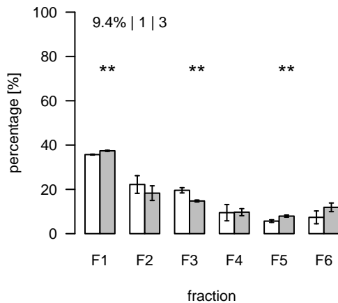
S231 (m/z=287.051025; rt=7.1968) T/S Cluster: S-7.2-2
