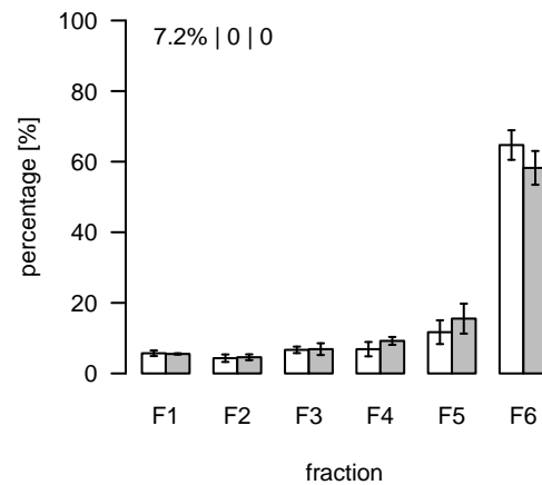
L2064 (m/z=776.619687; rt=10.38643) T/S Cluster: L-10.4-1
