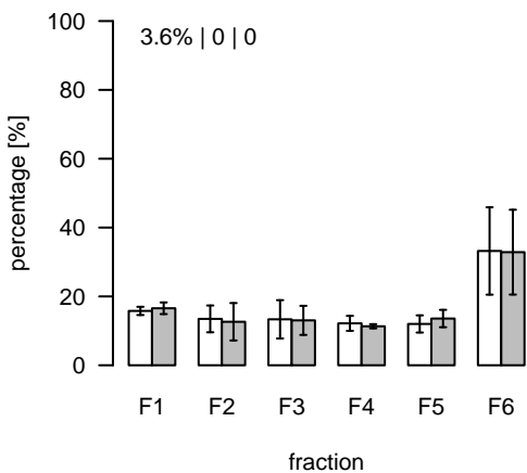
L154 (m/z=847.478578; rt=3.66853) T/S Cluster: L-3.7-13
