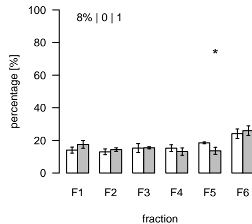
L513 (m/z=392.743865; rt=4.78876) T/S Cluster: L-4.8-8
