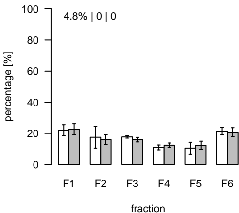
L1015 (m/z=777.585308; rt=6.44393) T/S Cluster: L-6.4-4
