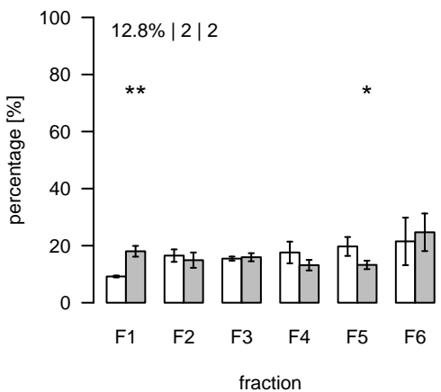
L2777 (m/z=1244.369564; rt=16.96598) T/S Cluster: L-17-2
