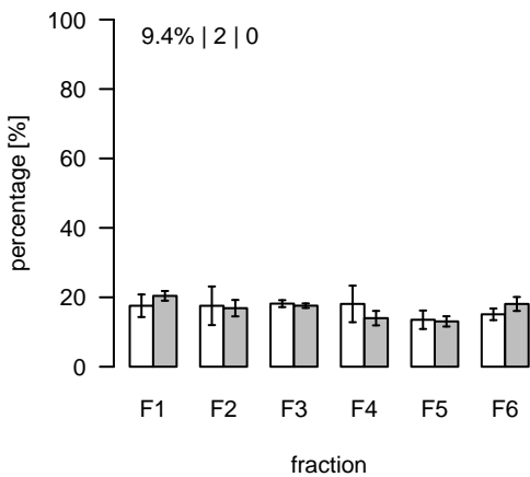
S907 (m/z=141.000467; rt=18.52528) T/S Cluster: S-18.5-2
