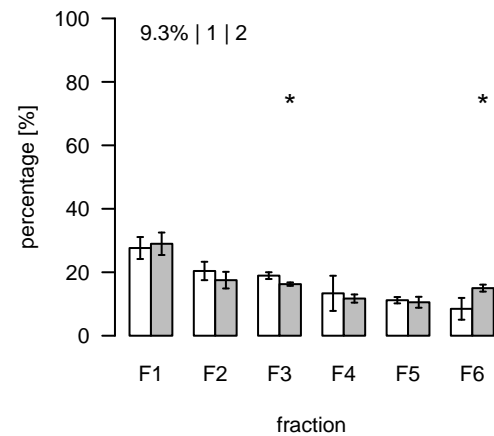
L1694 (m/z=252.861237; rt=8.70709) T/S Cluster: L-8.7-5
