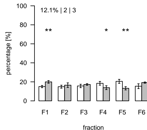
S797 (m/z=803.54631; rt=16.48865) T/S Cluster: S-16.5-2
