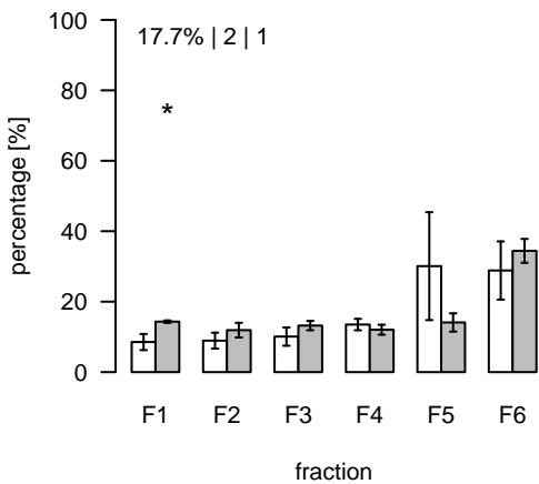
L1136 (m/z=761.521558; rt=6.6422) T/S Cluster: L-6.6-12
