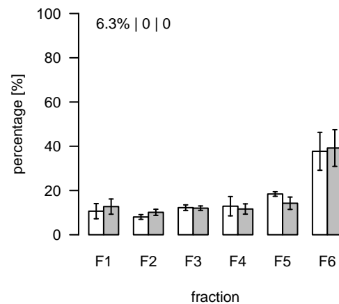
L1068 (m/z=585.45593; rt=6.54761) T/S Cluster: L-6.5-1
