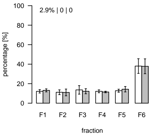
L404 (m/z=982.634197; rt=4.42422) T/S Cluster: L-4.4-14
