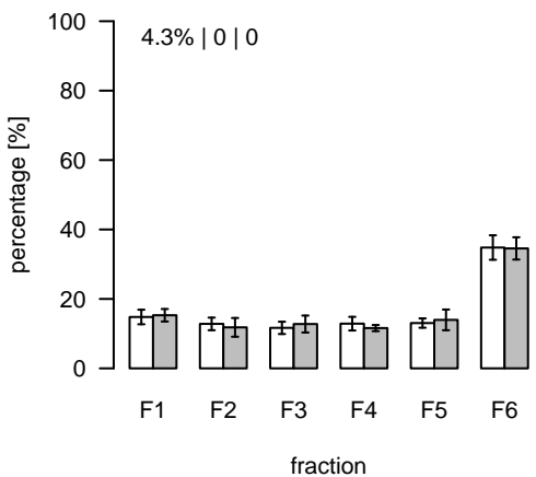
L2453 (m/z=874.588761; rt=11.84737) T/S Cluster: L-11.8-5
