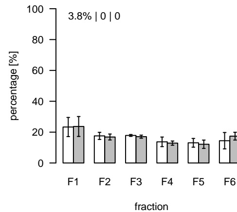
L1845 (m/z=773.593024; rt=9.27325) T/S Cluster: L-9.3-2
