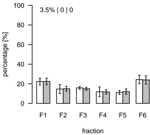
L491 (m/z=788.547762; rt=4.73069) T/S Cluster: L-4.7-7
