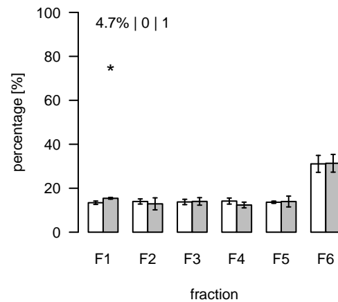
L2114 (m/z=893.546107; rt=10.50511) T/S Cluster: L-10.5-13
