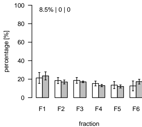
L1106 (m/z=800.587099; rt=6.56825) T/S Cluster: L-6.6-4
