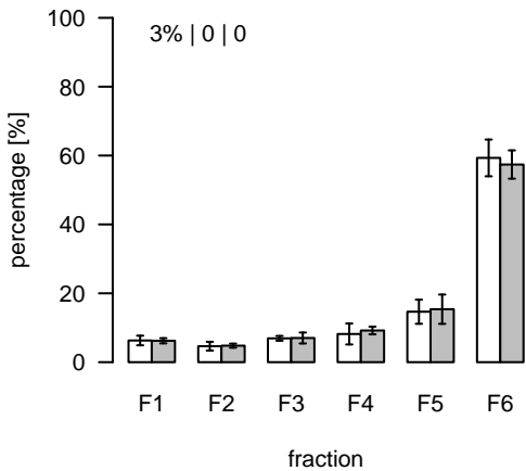
L1812 (m/z=960.666113; rt=9.01061) T/S Cluster: L-9-2
