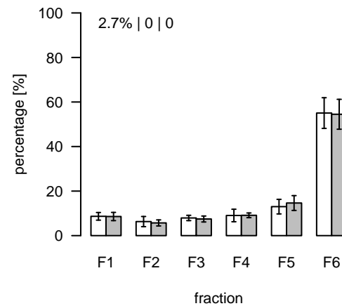
L660 (m/z=817.509592; rt=5.01432) T/S Cluster: L-5-1
