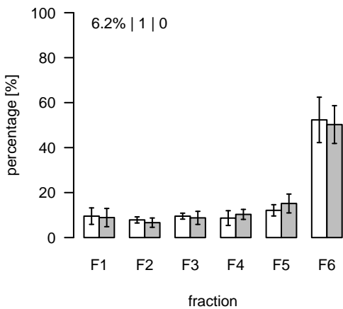
L1970 (m/z=888.554108; rt=9.87704) T/S Cluster: L-9.9-1
