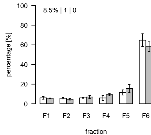
L1532 (m/z=795.546569; rt=8.04416) T/S Cluster: L-8-3
