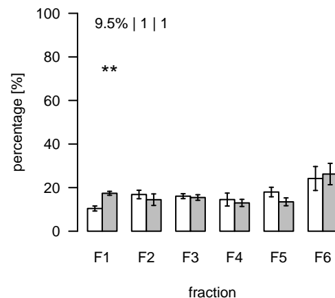
L2583 (m/z=907.265144; rt=15.36545) T/S Cluster: L-15.4-3
