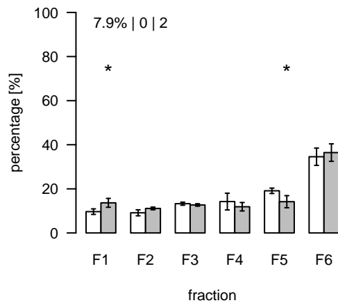
L1167 (m/z=318.202661; rt=6.6543) T/S Cluster: L-6.7-3
