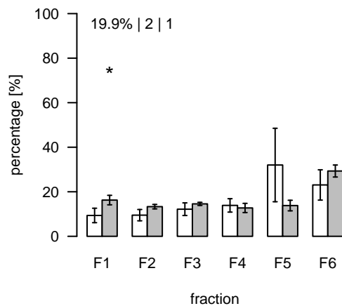
L1131 (m/z=762.525136; rt=6.64125) T/S Cluster: L-6.6-12
