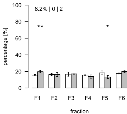
L2324 (m/z=793.613488; rt=11.32832) T/S Cluster: L-11.3-20
