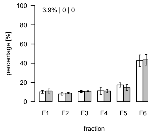
L1447 (m/z=932.636174; rt=7.90407) T/S Cluster: L-7.9-9
