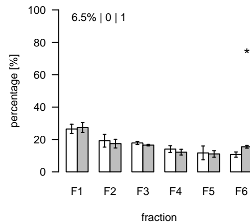
L1926 (m/z=253.863236; rt=9.59725) T/S Cluster: L-9.6-3
