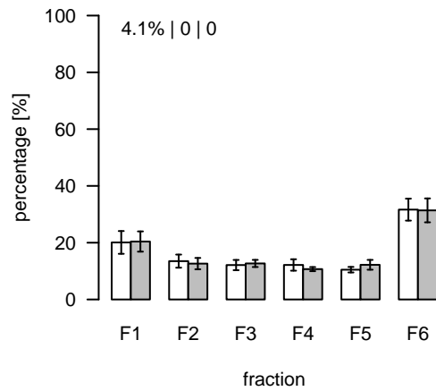
S437 (m/z=702.397915; rt=12.5817) T/S Cluster: S-12.6-14
