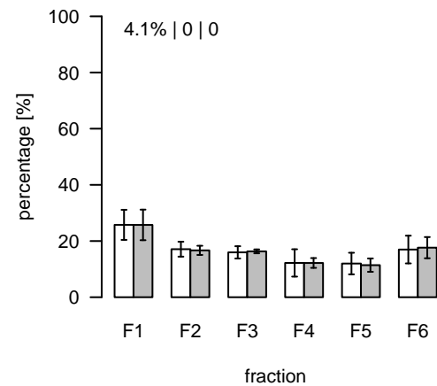
L1959 (m/z=787.608399; rt=9.82709) T/S Cluster: L-9.8-1
