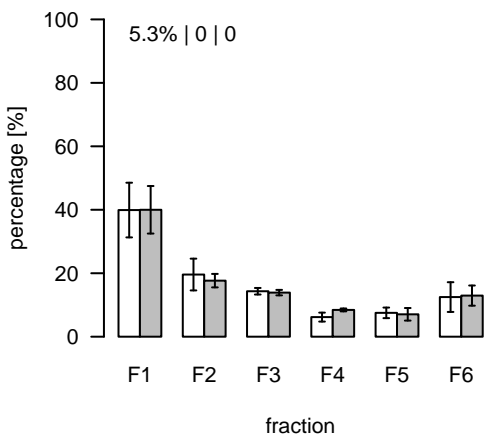
S603 (m/z=778.489647; rt=14.59585) T/S Cluster: S-14.6-1
