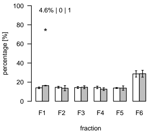
L2108 (m/z=447.276261; rt=10.50486) T/S Cluster: L-10.5-13
