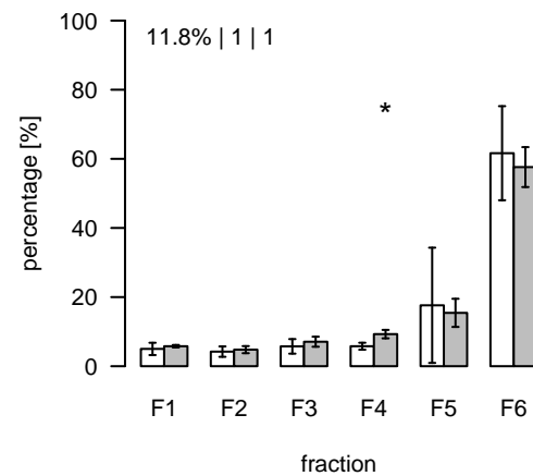
L2407 (m/z=443.78275; rt=11.5161) T/S Cluster: L-11.5-1
