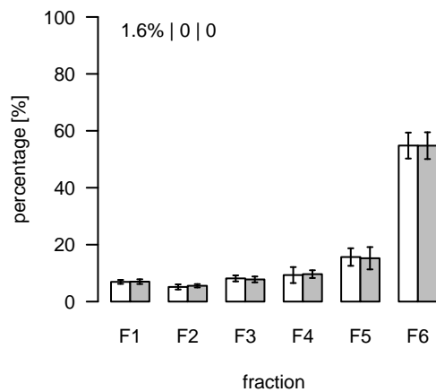
L612 (m/z=969.604967; rt=4.91092) T/S Cluster: L-4.9-9
