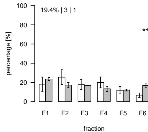
L2444 (m/z=894.566155; rt=11.83263) T/S Cluster: L-11.8-3
