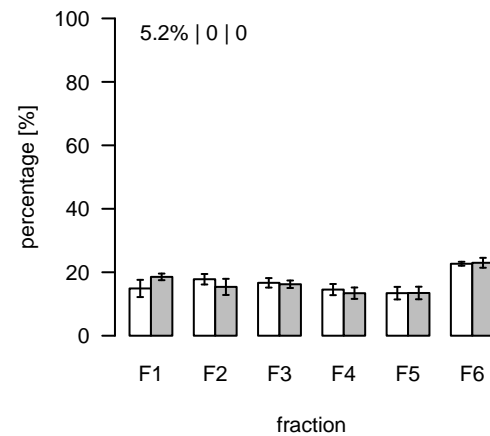
S588 (m/z=319.184642; rt=14.45667) T/S Cluster: S-14.5-2
