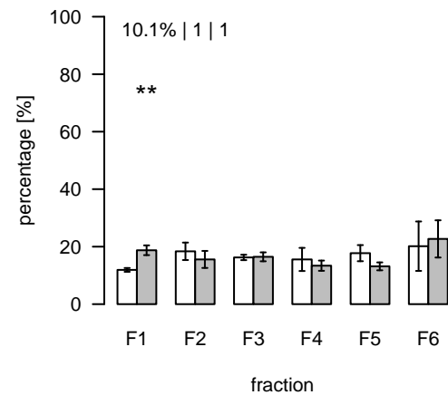
L2718 (m/z=1055.267851; rt=16.17884) T/S Cluster: L-16.2-5
