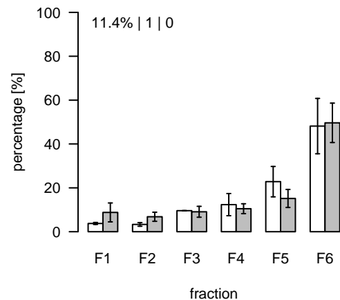
L2192 (m/z=896.526116; rt=10.91643) T/S Cluster: L-10.9-2
