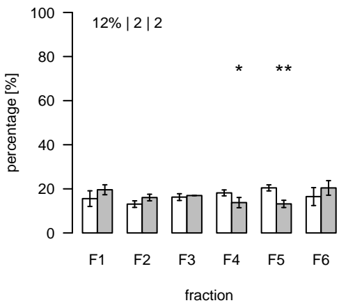
L1426 (m/z=468.797405; rt=7.88604) T/S Cluster: L-7.9-5
