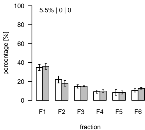
S635 (m/z=746.463658; rt=14.83897) T/S Cluster: S-14.8-2
