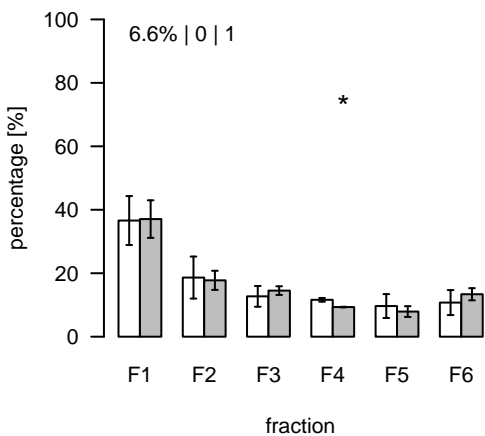
S247 (m/z=736.320097; rt=7.43214) T/S Cluster: S-7.4-2
