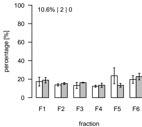
L1116 (m/z=837.559152; rt=6.60772) T/S Cluster: L-6.6-9
