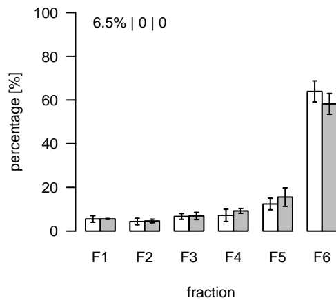
L775 (m/z=807.518998; rt=5.36222) T/S Cluster: L-5.4-2
