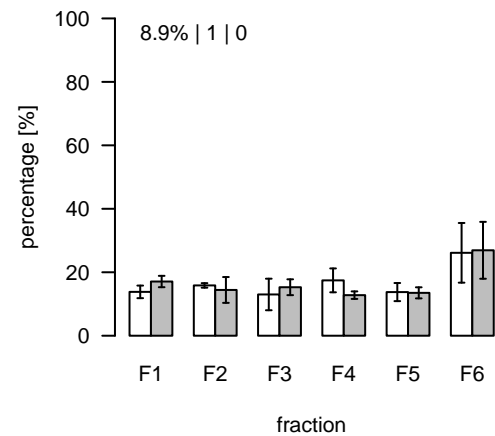
L1757 (m/z=903.569061; rt=8.9024) T/S Cluster: L-8.9-3
