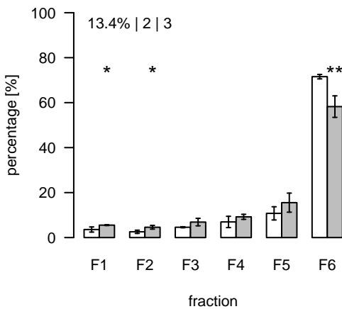
L1836 (m/z=909.507492; rt=9.19053) T/S Cluster: L-9.2-2
