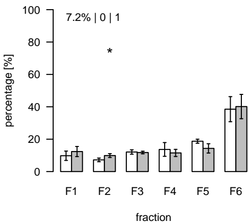
L1074 (m/z=255.513284; rt=6.54766) T/S Cluster: L-6.5-1
