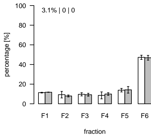
L94 (m/z=678.444946; rt=3.52915) T/S Cluster: L-3.5-8
