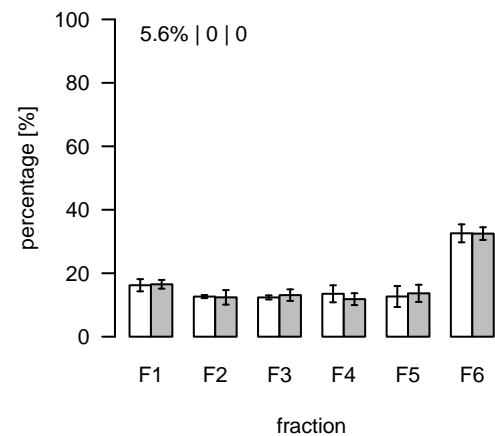
L2447 (m/z=437.289763; rt=11.84557) T/S Cluster: L-11.8-5
