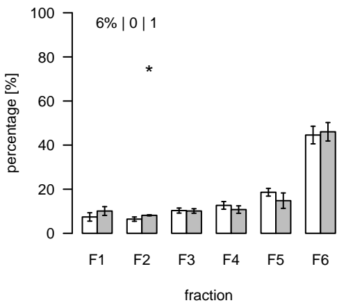
L218 (m/z=729.414044; rt=3.83972) T/S Cluster: L-3.8-5
