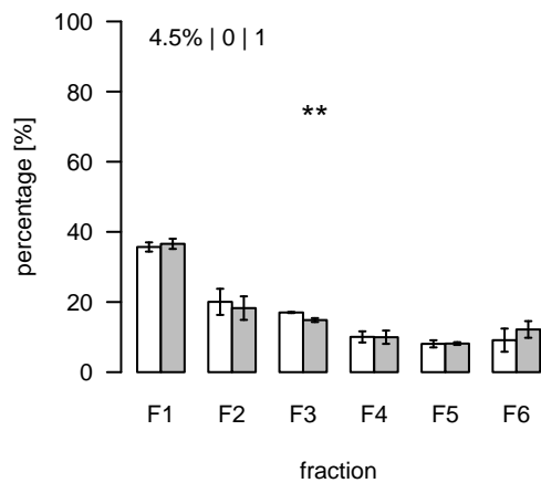
S74 ( m/z=103.532754 ; rt=4.70197 ) T/S Cluster: S-4.7-1
