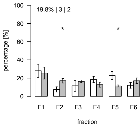
L2533 (m/z=759.225504; rt=14.06581) T/S Cluster: L-14.1-2
