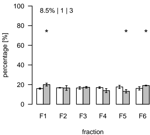
S22 (m/z=437.74927; rt=2.74676) T/S Cluster: S-2.7-1
