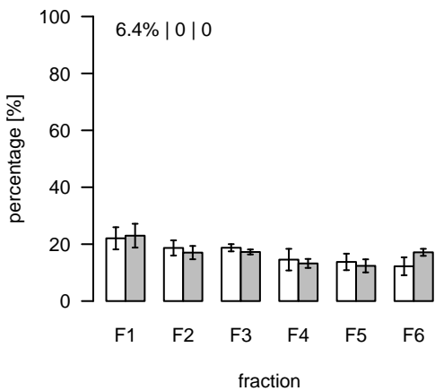
L1210 (m/z=776.539221; rt=6.69982) T/S Cluster: L-6.7-11
