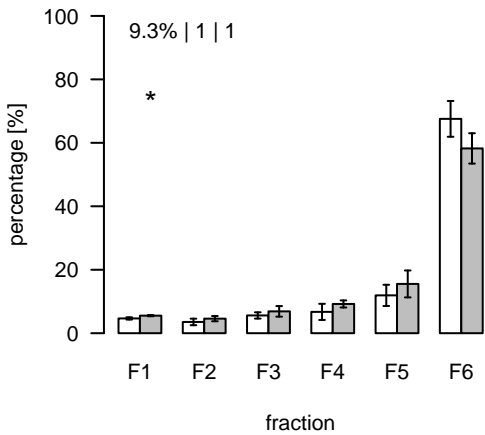
L421 (m/z=752.463855; rt=4.44574) T/S Cluster: L-4.4-2
