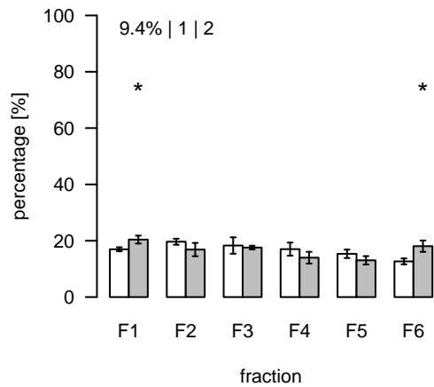
L2598 (m/z=834.757469; rt=15.47111) T/S Cluster: L-15.5-2
