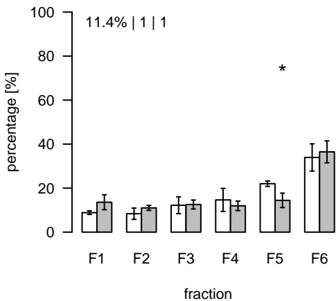
L1111 (m/z=942.537048; rt=6.5958) T/S Cluster: L-6.6-7
