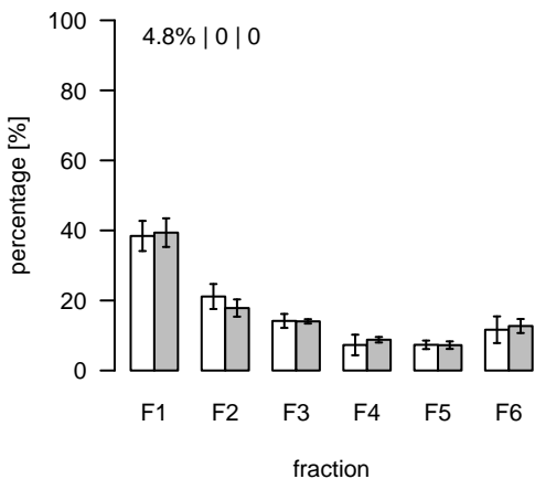
S651 (m/z=184.073441; rt=14.90541) T/S Cluster: S-14.9-2
