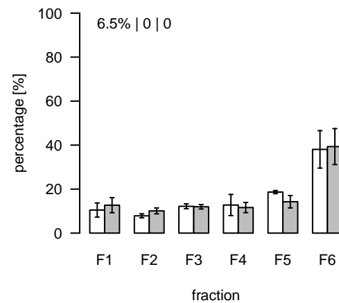
L1060 (m/z=292.730389; rt=6.54755) T/S Cluster: L-6.5-1
