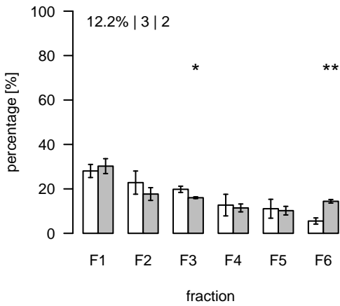
L1932 (m/z=782.573348; rt=9.59834) T/S Cluster: L-9.6-3
