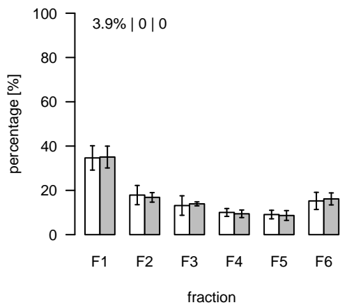
S665 (m/z=483.369643; rt=14.93415) T/S Cluster: S-14.9-5
