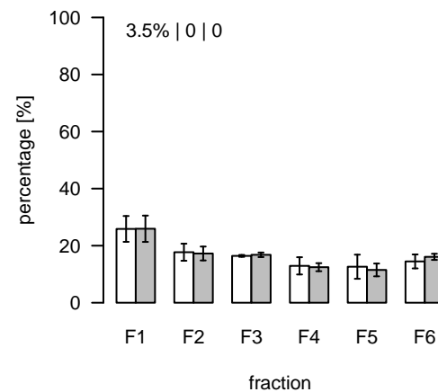
L1841 (m/z=772.572164; rt=9.2695) T/S Cluster: L-9.3-2
