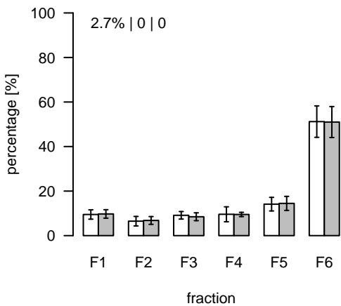
L663 (m/z=818.471707; rt=5.01516) T/S Cluster: L-5-1
