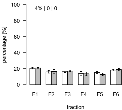
S487 (m/z=342.264794; rt=12.91227) T/S Cluster: S-12.9-18
