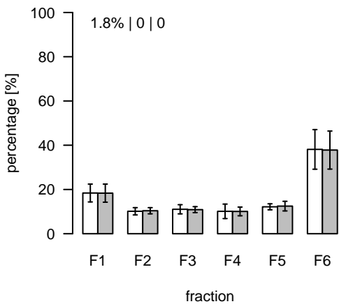
L1328 (m/z=820.558393; rt=7.33635) T/S Cluster: L-7.3-8
