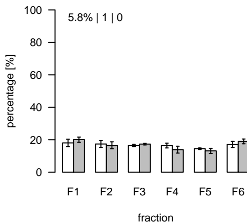
S418 (m/z=470.32333; rt=12.53996) T/S Cluster: S-12.5-10
