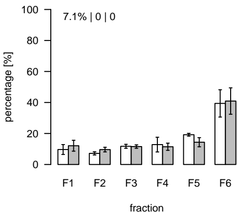
L1051 (m/z=255.517725; rt=6.5474) T/S Cluster: L-6.5-1
