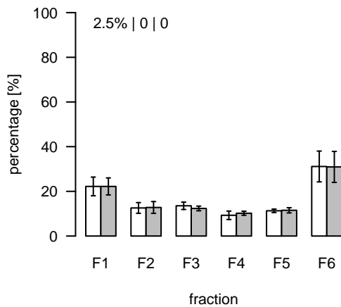
S305 (m/z=640.320822; rt=9.5758) T/S Cluster: S-9.6-2
