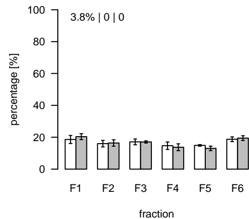
S518 (m/z=299.045914; rt=13.23136) T/S Cluster: S-13.2-4
