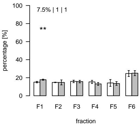
L2086 (m/z=954.611767; rt=10.49968) T/S Cluster: L-10.5-9
