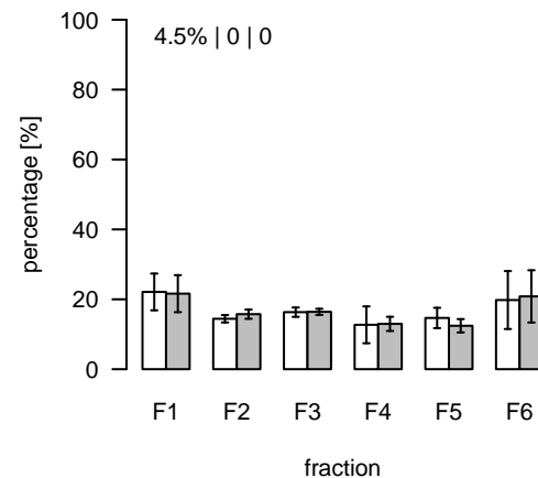
L1325 (m/z=390.280195; rt=7.32899) T/S Cluster: L-7.3-5
