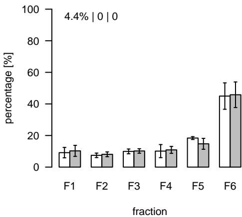
L770 (m/z=812.500817; rt=5.34444) T/S Cluster: L-5.3-5
