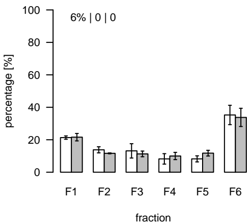
S577 (m/z=671.398567; rt=14.34832) T/S Cluster: S-14.3-4
