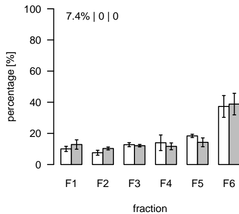
L1154 (m/z=478.815841; rt=6.65414) T/S Cluster: L-6.7-3
