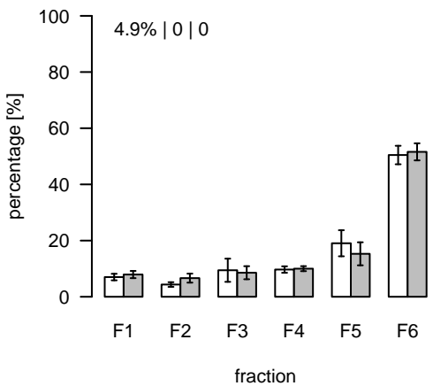
L2038 (m/z=926.491978; rt=10.21265) T/S Cluster: L-10.2-2
