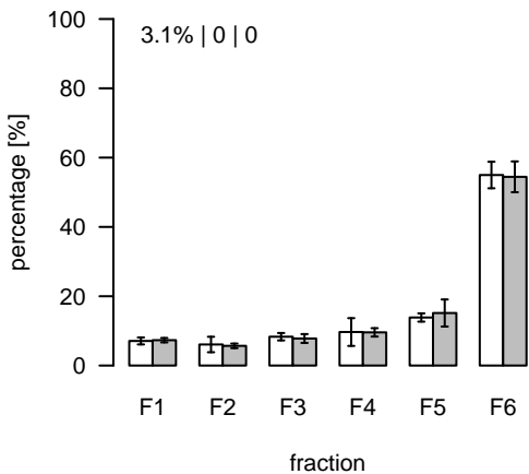
L931 (m/z=685.440282; rt=6.12608) T/S Cluster: L-6.1-1
