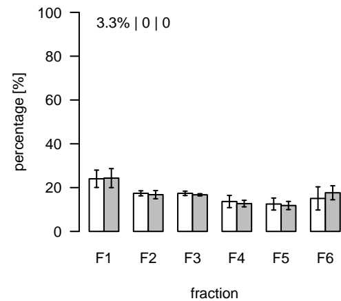
L1481 (m/z=379.784437; rt=7.93891) T/S Cluster: L-7.9-14
