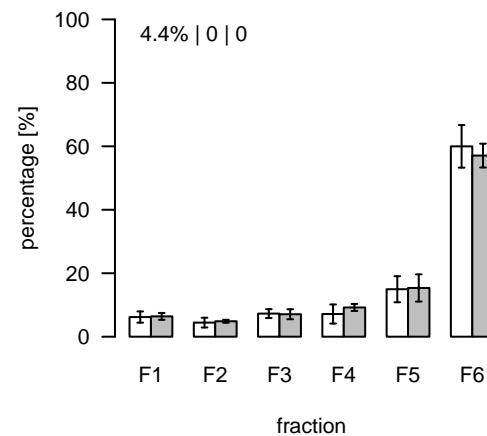
L917 (m/z=463.295319; rt=5.95916) T/S Cluster: L-6-1
