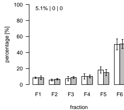
L1218 (m/z=769.494289; rt=6.77677) T/S Cluster: L-6.8-1
