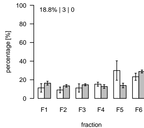
L1123 (m/z=835.517989; rt=6.63203) T/S Cluster: L-6.6-12
