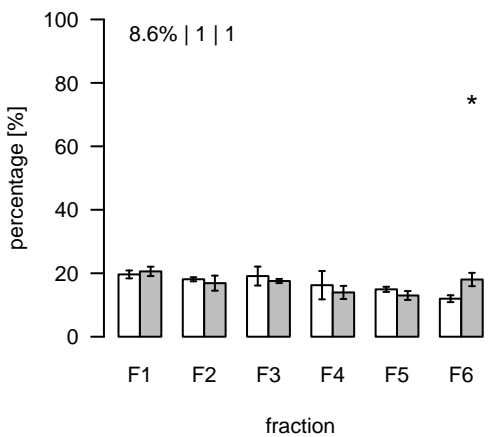
L2731 (m/z=906.851493; rt=16.28727) T/S Cluster: L-16.3-2
