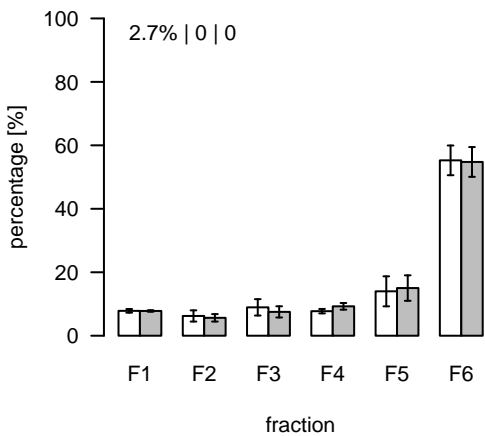
L1407 (m/z=906.587279; rt=7.65516) T/S Cluster: L-7.7-1
