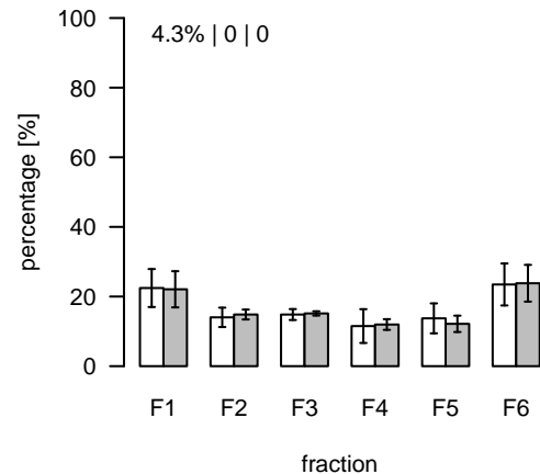
L1544 (m/z=784.580576; rt=8.0566) T/S Cluster: L-8.1-2
