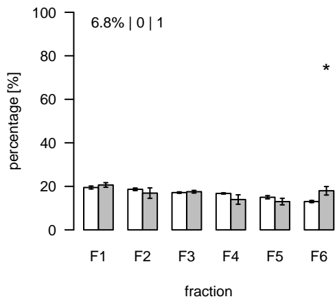
L2704 (m/z=998.332735; rt=16.15635) T/S Cluster: L-16.2-1
