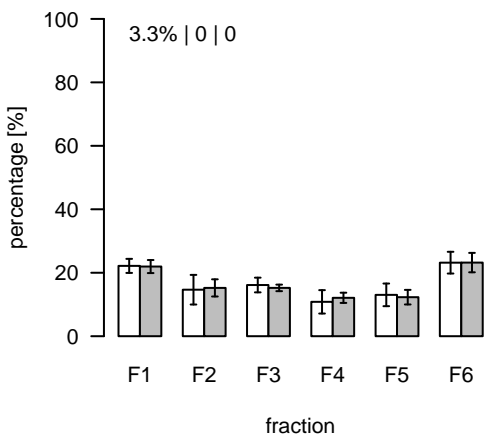
L445 (m/z=784.506199; rt=4.53304) T/S Cluster: L-4.5-6
