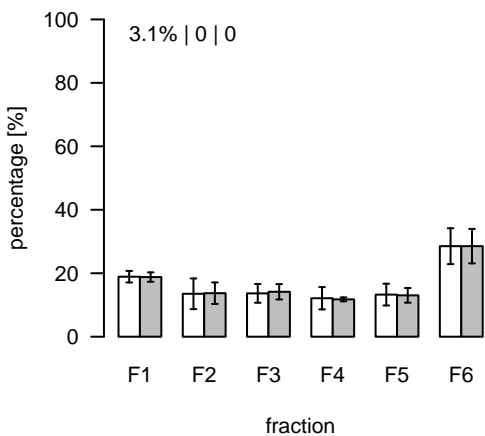
L179 (m/z=674.428876; rt=3.69505) T/S Cluster: L-3.7-8
