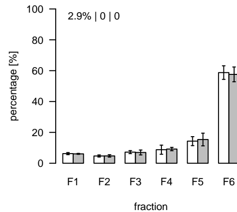
L367 (m/z=930.589661; rt=4.36508) T/S Cluster: L-4.4-2
