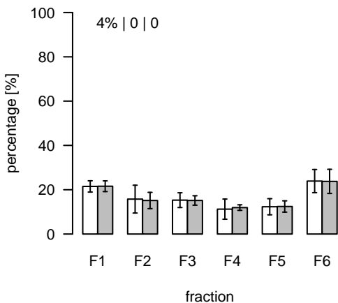
L280 (m/z=650.422665; rt=4.09564) T/S Cluster: L-4.1-2
