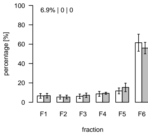
L198 (m/z=796.486399; rt=3.78858) T/S Cluster: L-3.8-5
