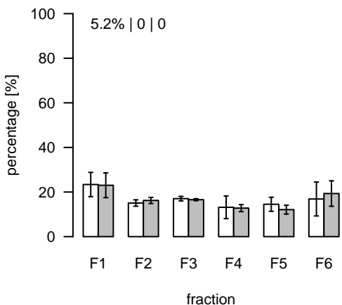
L1312 (m/z=260.183004; rt=7.32795) T/S Cluster: L-7.3-5
