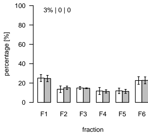
L2226 (m/z=857.694074; rt=11.15873) T/S Cluster: L-11.2-1
