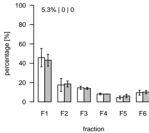
S257 (m/z=538.213867; rt=7.74468) T/S Cluster: S-7.7-1
