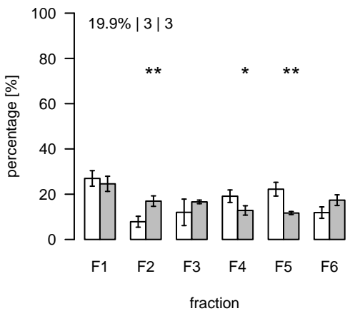
L2531 (m/z=758.224534; rt=14.0651) T/S Cluster: L-14.1-2
