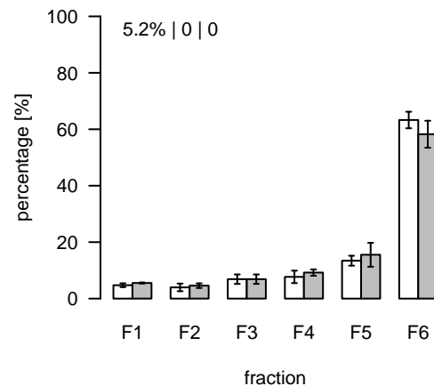
L2174 (m/z=951.593786; rt=10.68369) T/S Cluster: L-10.7-2
