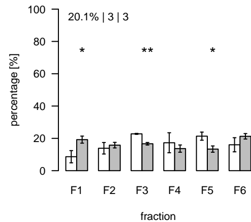
L2235 (m/z=1344.139125; rt=11.30904) T/S Cluster: L-11.3-5
