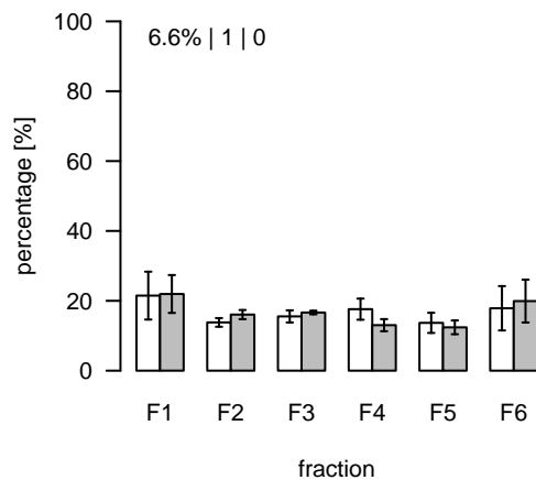
L1322 (m/z=260.189803; rt=7.32865) T/S Cluster: L-7.3-5
