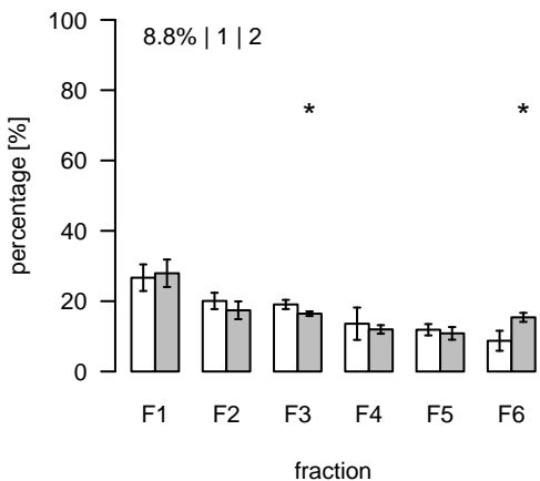
L1697 (m/z=253.189613; rt=8.70724) T/S Cluster: L-8.7-5
