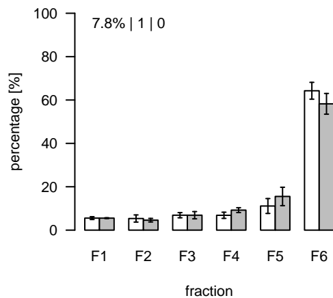
L74 (m/z=797.52938; rt=3.4503) T/S Cluster: L-3.5-1
