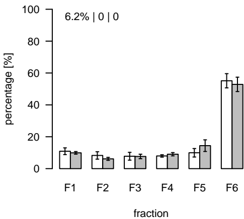
L1631 (m/z=887.575428; rt=8.59518) T/S Cluster: L-8.6-3
