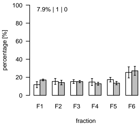
L2766 (m/z=602.173698; rt=16.96448) T/S Cluster: L-17-2
