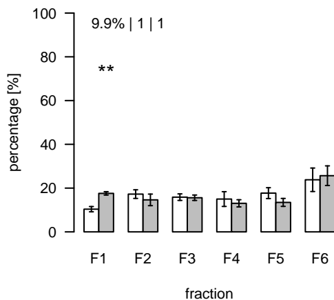
L2584 (m/z=908.263683; rt=15.36545) T/S Cluster: L-15.4-3
