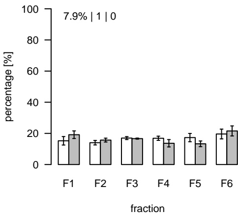
L1795 (m/z=968.587427; rt=8.91788) T/S Cluster: L-8.9-12
