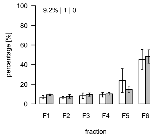
L622 (m/z=774.490816; rt=4.9215) T/S Cluster: L-4.9-11
