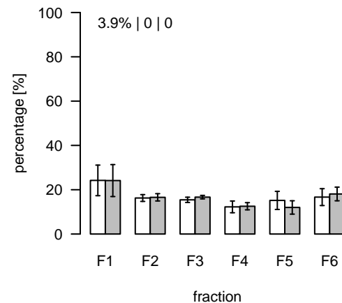
L1303 (m/z=800.557122; rt=7.31975) T/S Cluster: L-7.3-6
