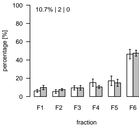
L1735 (m/z=447.762473; rt=8.74397) T/S Cluster: L-8.7-8
