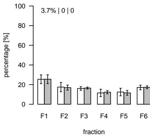
L2184 (m/z=789.622576; rt=10.74727) T/S Cluster: L-10.7-3
