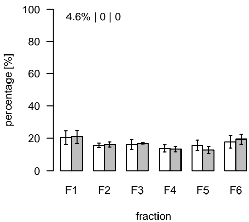
L1988 (m/z=761.595349; rt=10.05301) T/S Cluster: L-10.1-1
