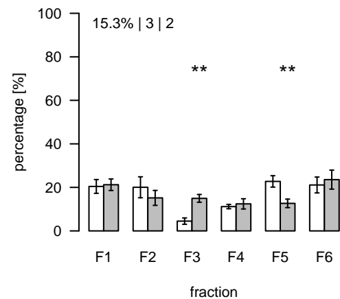
S357 (m/z=437.726429; rt=11.91956) T/S Cluster: S-11.9-1
