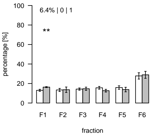
L2116 (m/z=223.387113; rt=10.5052) T/S Cluster: L-10.5-11
