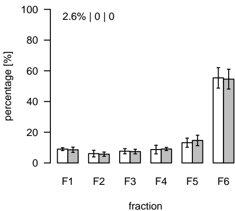
L665 (m/z=818.50693; rt=5.01555) T/S Cluster: L-5-1
