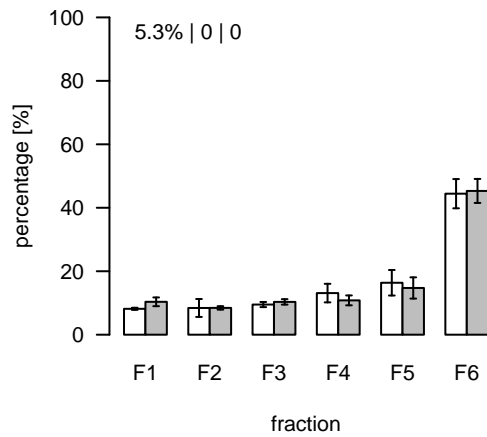
L201 (m/z=801.485579; rt=3.79138) T/S Cluster: L-3.8-5
