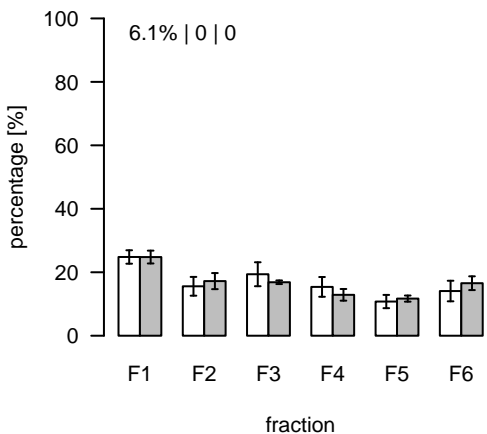
L2169 (m/z=860.676182; rt=10.66104) T/S Cluster: L-10.7-1
