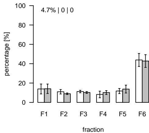
S686 (m/z=827.523684; rt=15.30498) T/S Cluster: S-15.3-3
