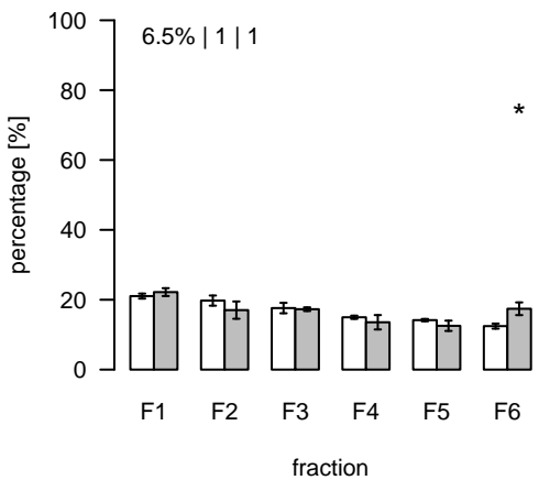
L2596 (m/z=847.297132; rt=15.46721) T/S Cluster: L-15.5-1
