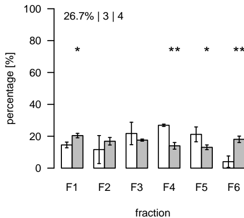
S5 (m/z=437.790096; rt=0.9975) T/S Cluster: S-1-1
