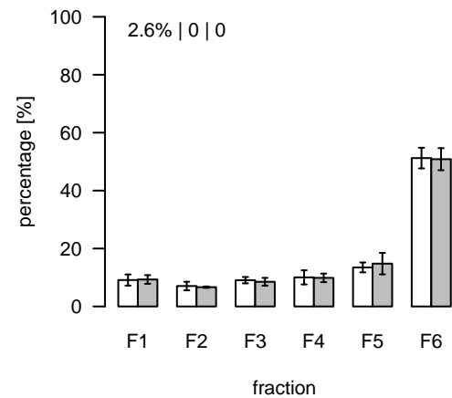
L1581 (m/z=892.571884; rt=8.18367) T/S Cluster: L-8.2-2
