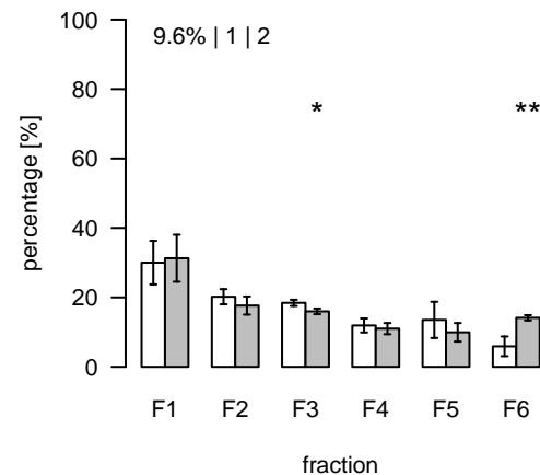
L1747 (m/z=785.570953; rt=8.87923) T/S Cluster: L-8.9-1
