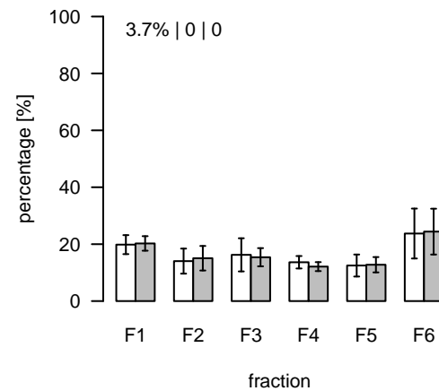
L77 (m/z=822.553506; rt=3.4779) T/S Cluster: L-3.5-3
