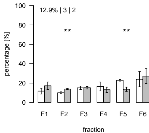
L910 (m/z=931.563788; rt=5.93428) T/S Cluster: L-5.9-5
