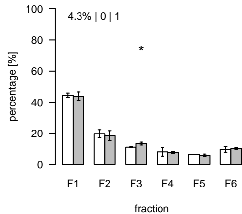
S675 (m/z=802.525435; rt=15.11617) T/S Cluster: S-15.1-2
