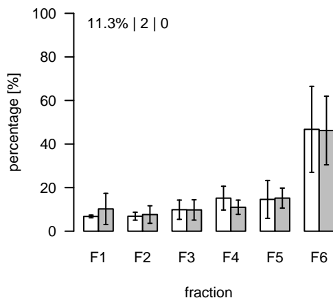
L1725 (m/z=911.550475; rt=8.72636) T/S Cluster: L-8.7-8
