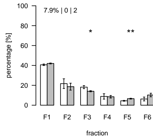
S215 (m/z=433.096403; rt=7.19527) T/S Cluster: S-7.2-2
