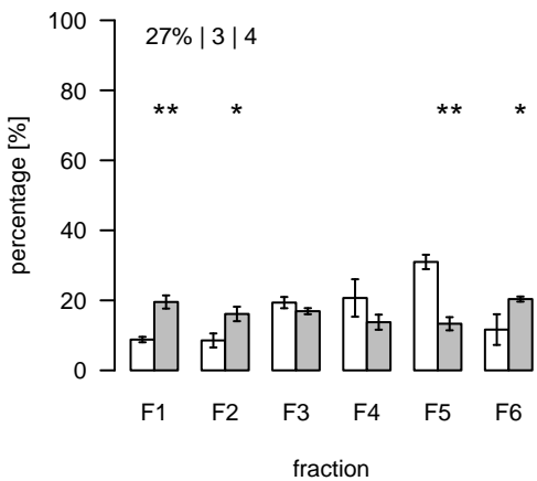
L2188 (m/z=916.561872; rt=10.91533) T/S Cluster: L-10.9-1
