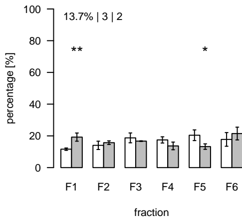
L2247 (m/z=170.373972; rt=11.32725) T/S Cluster: L-11.3-4
