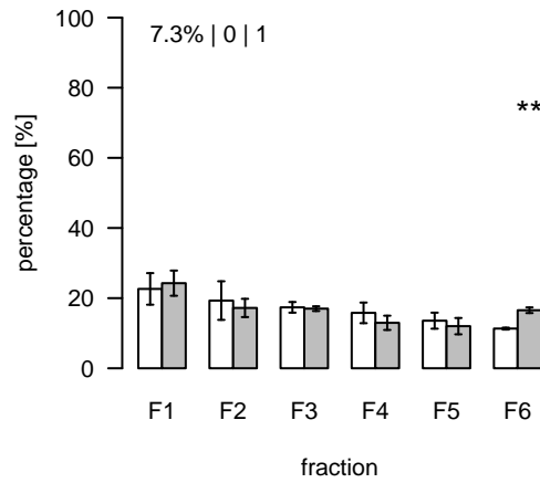
L495 (m/z=774.531637; rt=4.74897) T/S Cluster: L-4.7-9
