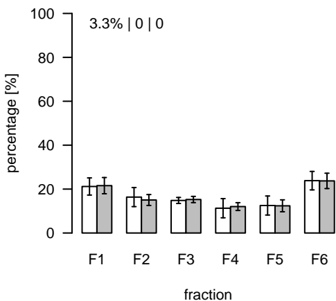
L479 (m/z=716.467353; rt=4.65931) T/S Cluster: L-4.7-1
