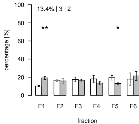
L2641 (m/z=1022.308847; rt=15.81099) T/S Cluster: L-15.8-2
