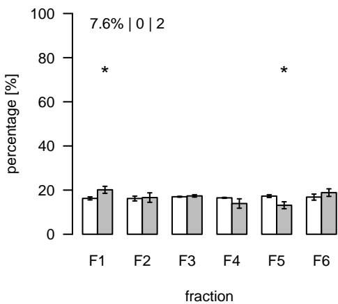
S28 (m/z=437.758718; rt=3.60429) T/S Cluster: S-3.6-2
