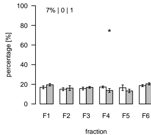
S3 (m/z=437.773809; rt=0.68232) T/S Cluster: S-0.7-1
