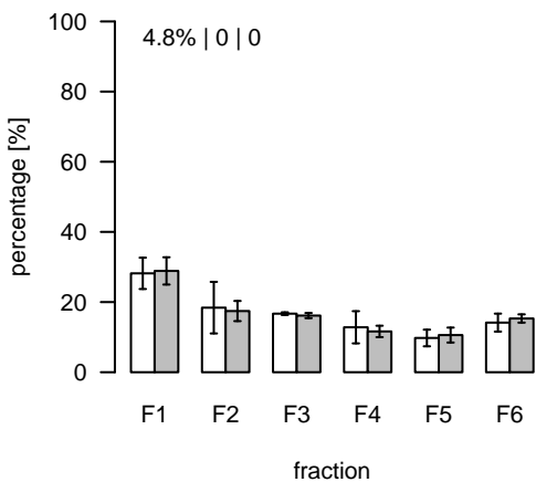
L455 (m/z=791.526549; rt=4.57265) T/S Cluster: L-4.6-1
