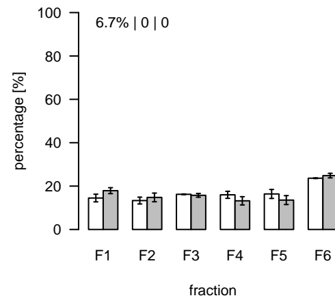
L1780 (m/z=907.464676; rt=8.91527) T/S Cluster: L-8.9-5
