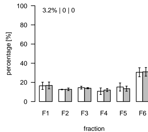
L728 (m/z=398.277468; rt=5.28564) T/S Cluster: L-5.3-1
