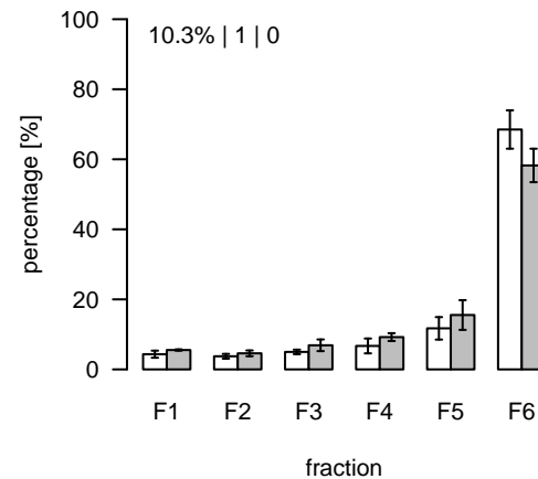
L222 (m/z=792.494005; rt=3.84578) T/S Cluster: L-3.8-5
