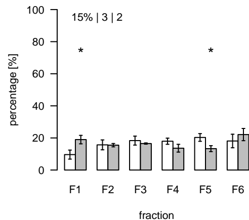
L2233 (m/z=136.097941; rt=11.30728) T/S Cluster: L-11.3-4
