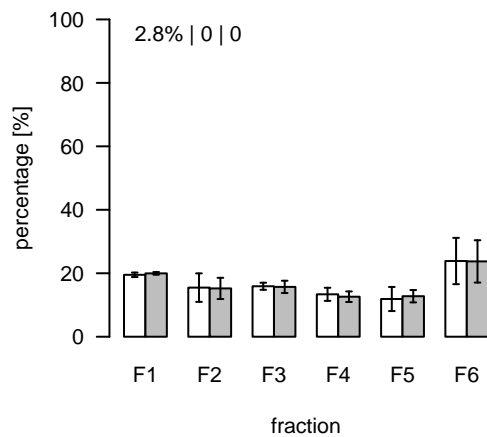
L463 (m/z=812.549016; rt=4.61247) T/S Cluster: L-4.6-5
