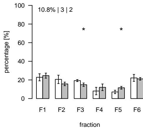
S902 (m/z=823.737916; rt=18.18814) T/S Cluster: S-18.2-1
