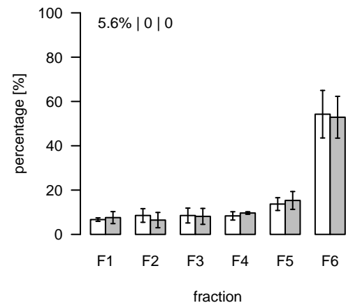
S398 (m/z=910.468927; rt=12.36861) T/S Cluster: S-12.4-4
