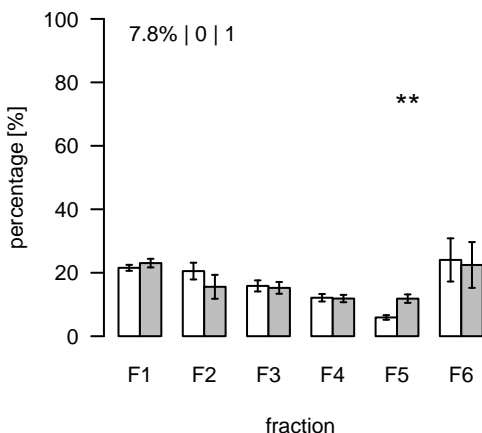
L1717 (m/z=796.533432; rt=8.71487) T/S Cluster: L-8.7-9
