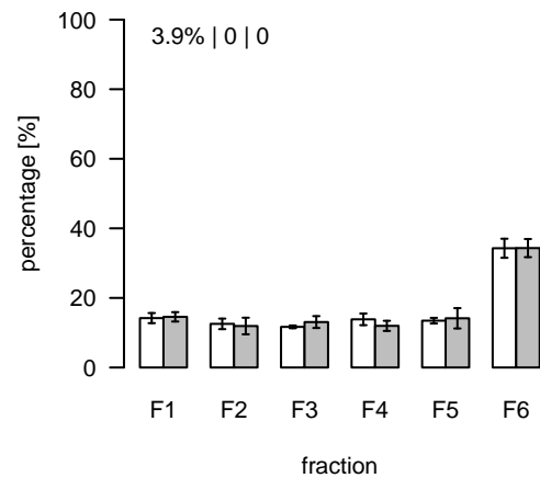
L2463 (m/z=290.859394; rt=11.84906) T/S Cluster: L-11.8-5
