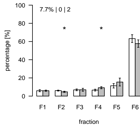
L2179 (m/z=892.531985; rt=10.68473) T/S Cluster: L-10.7-2
