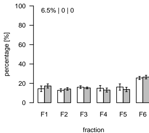
L1761 (m/z=629.227653; rt=8.91403) T/S Cluster: L-8.9-5
