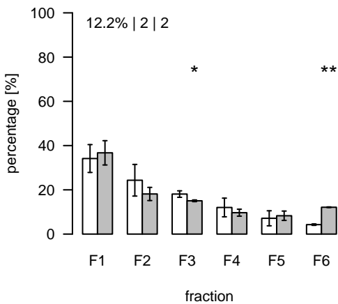
L160 (m/z=668.444418; rt=3.6749) T/S Cluster: L-3.7-14
