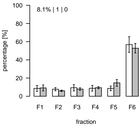
S559 (m/z=864.498753; rt=14.05099) T/S Cluster: S-14.1-1
