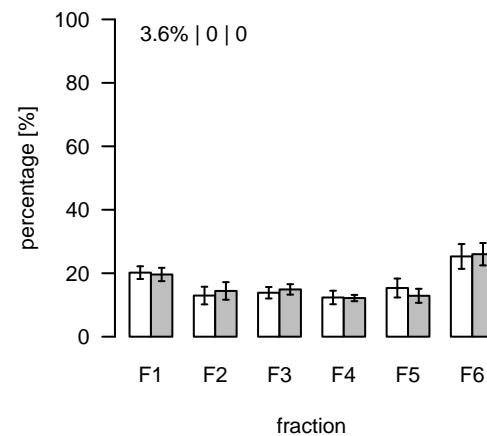
L749 (m/z=397.274583; rt=5.32431) T/S Cluster: L-5.3-1
