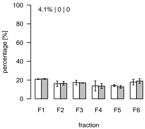
L2159 (m/z=844.661909; rt=10.61359) T/S Cluster: L-10.6-4
