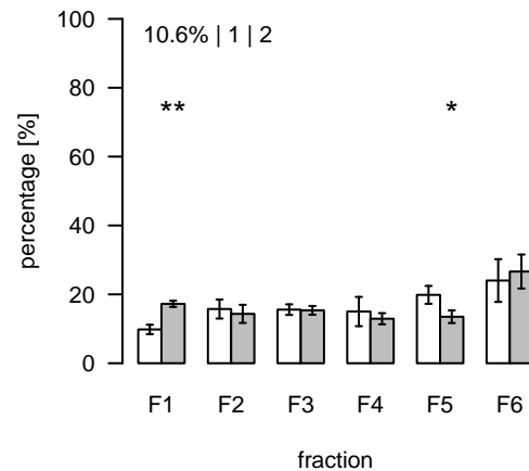
L2523 (m/z=758.225413; rt=14.00396) T/S Cluster: L-14-1
