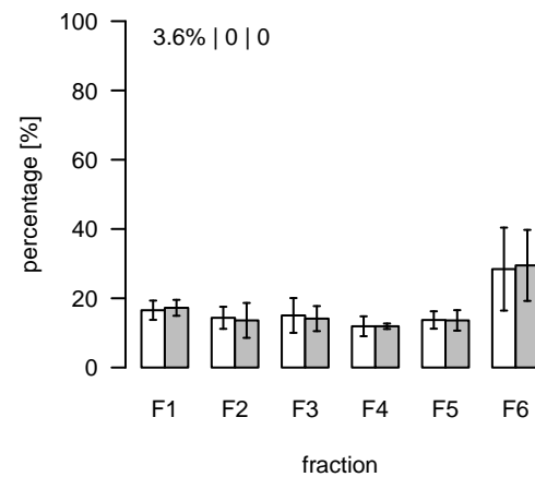
L130 (m/z=706.469389; rt=3.62959) T/S Cluster: L-3.6-8
