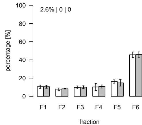
L1887 (m/z=468.840823; rt=9.53025) T/S Cluster: L-9.5-5
