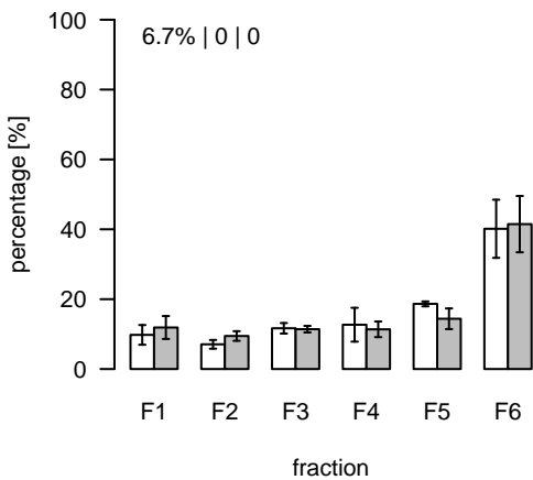
L1075 (m/z=152.908581; rt=6.54766) T/S Cluster: L-6.5-1
