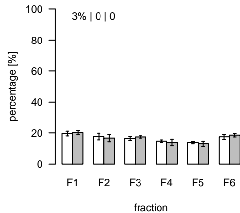
S292 (m/z=246.058657; rt=8.7245) T/S Cluster: S-8.7-2
