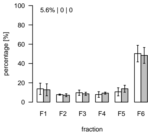
S778 (m/z=856.526911; rt=16.24273) T/S Cluster: S-16.2-6
