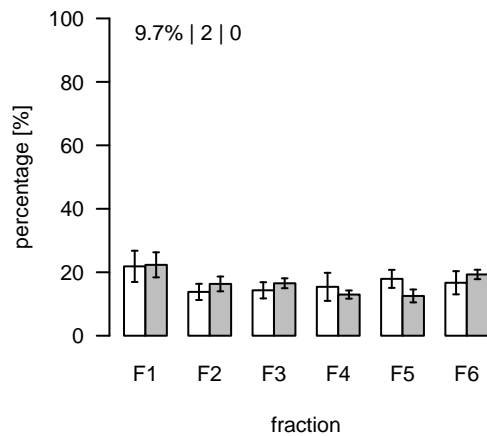
S72 (m/z=704.154486; rt=4.7008) T/S Cluster: S-4.7-5
