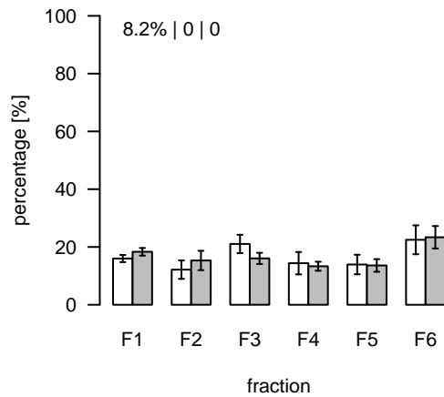
L294 (m/z=829.549097; rt=4.11294) T/S Cluster: L-4.1-8
