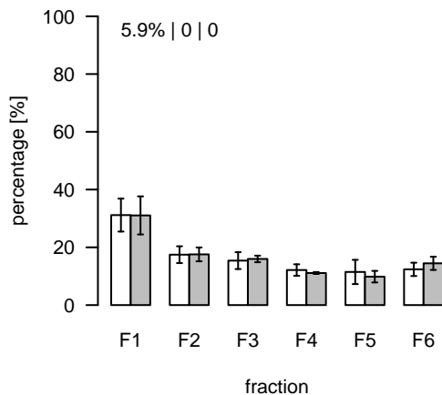
S503 (m/z=706.432773; rt=12.99644) T/S Cluster: S-13-3
