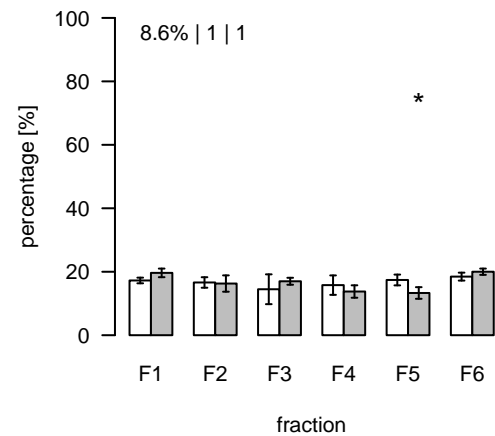
S351 (m/z=437.739811; rt=11.38715) T/S Cluster: S-11.4-2
