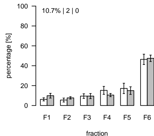
L1727 (m/z=447.769963; rt=8.74258) T/S Cluster: L-8.7-8
