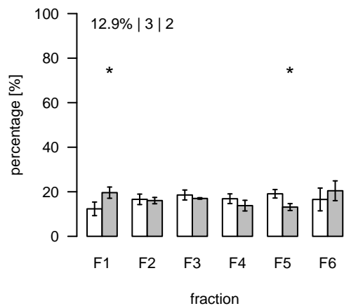
L2314 (m/z=221.155346; rt=11.32819) T/S Cluster: L-11.3-4
