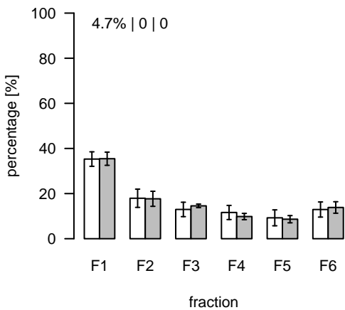
S676 (m/z=803.527813; rt=15.12401) T/S Cluster: S-15.1-3
