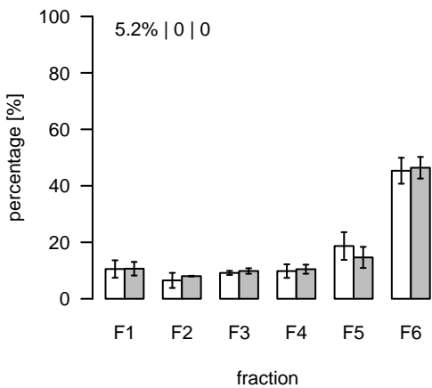
L212 (m/z=730.445864; rt=3.83337) T/S Cluster: L-3.8-5
