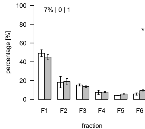
S135 (m/z=595.168375; rt=5.70155) T/S Cluster: S-5.7-1
