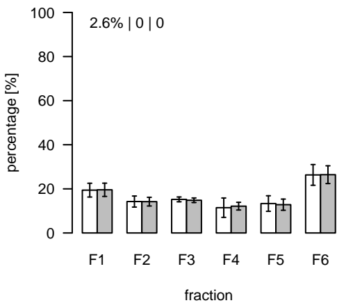
L968 (m/z=775.573129; rt=6.19001) T/S Cluster: L-6.2-5
