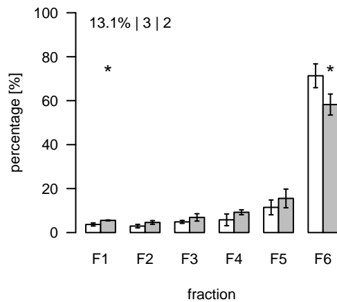
L216 (m/z=724.467184; rt=3.83772) T/S Cluster: L-3.8-5
