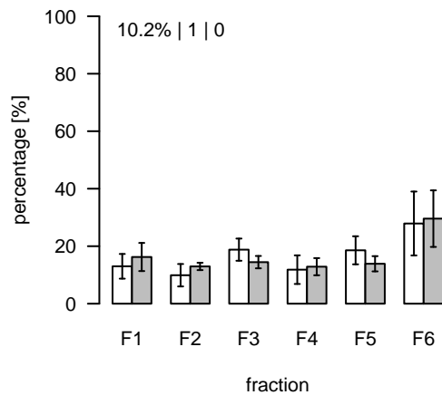
L1997 (m/z=886.533003; rt=10.08991) T/S Cluster: L-10.1-6
