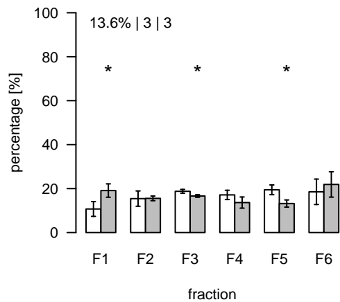
L2294 (m/z=724.51795; rt=11.32798) T/S Cluster: L-11.3-4
