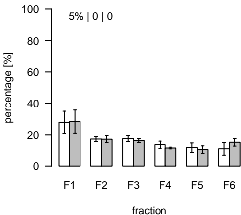
L1622 (m/z=770.57505; rt=8.48277) T/S Cluster: L-8.5-3
