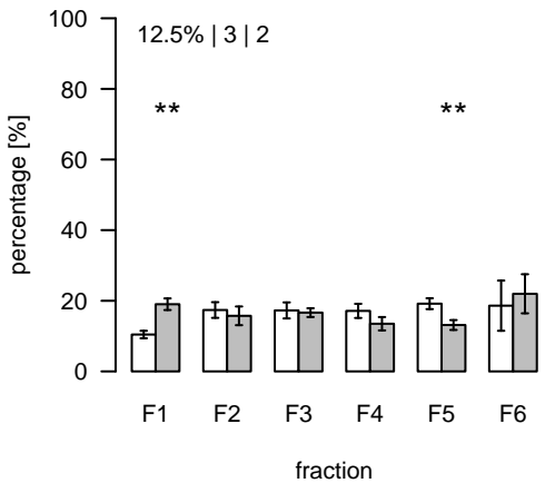
L2639 (m/z=1023.307804; rt=15.81082) T/S Cluster: L-15.8-2
