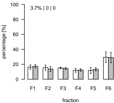
L68 (m/z=838.538327; rt=3.40692) T/S Cluster: L-3.4-6
