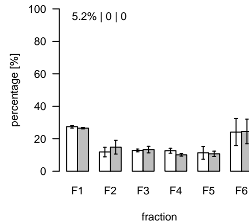
S447 (m/z=718.39483; rt=12.66275) T/S Cluster: S-12.7-2
