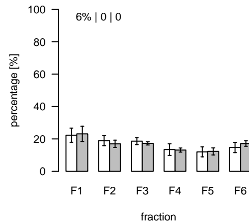
L959 (m/z=791.571987; rt=6.15337) T/S Cluster: L-6.2-2
