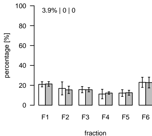
L283 (m/z=325.223766; rt=4.09569) T/S Cluster: L-4.1-2
