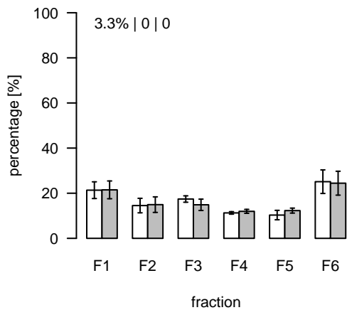
S377 (m/z=722.430685; rt=12.19378) T/S Cluster: S-12.2-7
