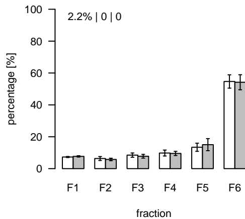
L239 (m/z=986.586679; rt=3.93529) T/S Cluster: L-3.9-7
