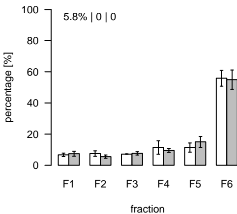
L1842 (m/z=908.528451; rt=9.27001) T/S Cluster: L-9.3-1
