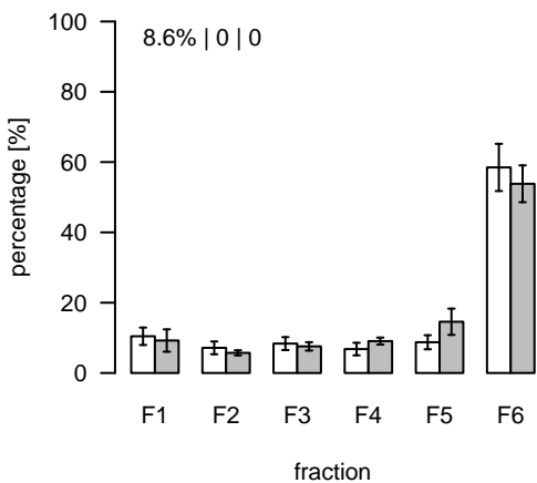
S715 (m/z=968.598738; rt=15.68854) T/S Cluster: S-15.7-3
