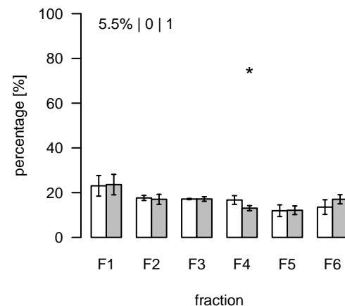
L1491 (m/z=379.280692; rt=7.93915) T/S Cluster: L-7.9-14
