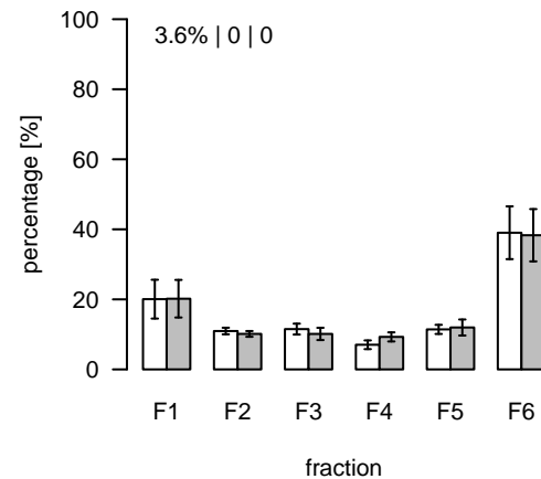
S636 (m/z=728.427707; rt=14.85118) T/S Cluster: S-14.9-1
