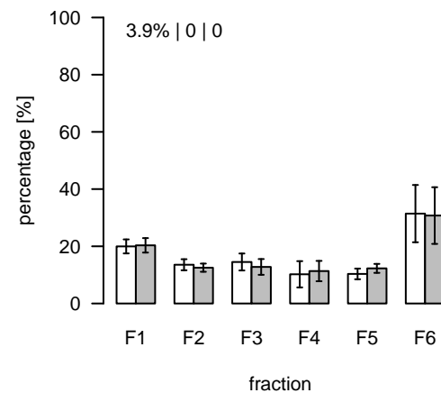
S581 (m/z=745.425417; rt=14.38501) T/S Cluster: S-14.4-1
