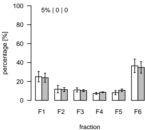
S265 (m/z=696.440768; rt=8.00195) T/S Cluster: S-8-2
