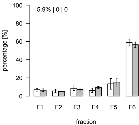
L104 (m/z=593.278874; rt=3.57045) T/S Cluster: L-3.6-2
