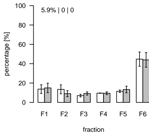
L78 (m/z=814.498689; rt=3.47805) T/S Cluster: L-3.5-2
