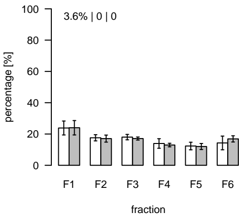
L1495 (m/z=151.313088; rt=7.93923) T/S Cluster: L-7.9-14
