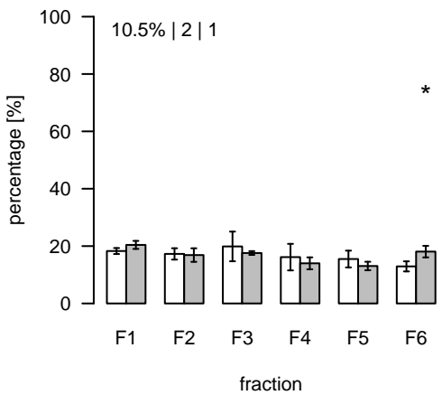
L2614 (m/z=848.774336; rt=15.5925) T/S Cluster: L-15.6-1
