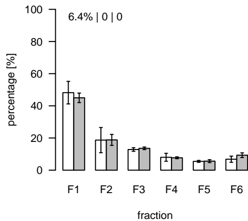
S136 (m/z=247.071511; rt=5.70156) T/S Cluster: S-5.7-1
