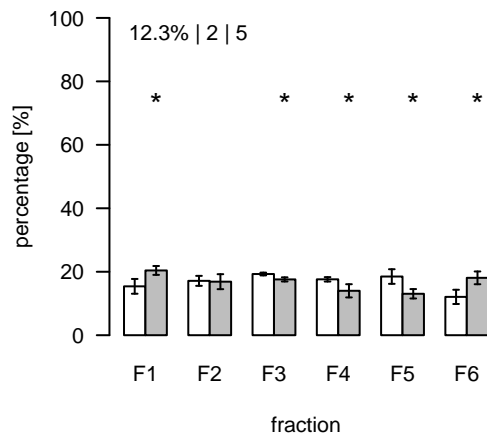
L1038 (m/z=769.495591; rt=6.54578) T/S Cluster: L-6.5-6
