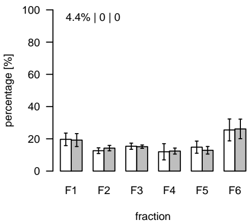
L747 (m/z=795.517665; rt=5.32408) T/S Cluster: L-5.3-1
