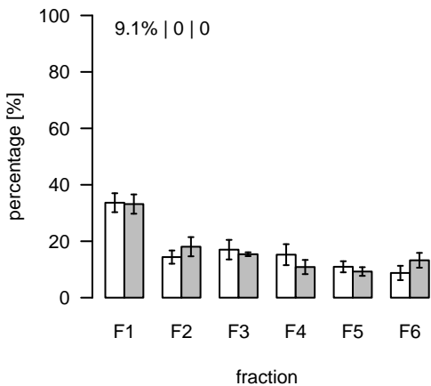
L767 (m/z=804.534016; rt=5.33801) T/S Cluster: L-5.3-7
