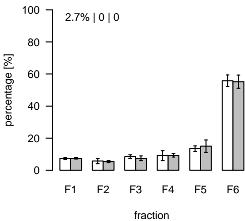
L935 (m/z=684.462244; rt=6.12661) T/S Cluster: L-6.1-1
