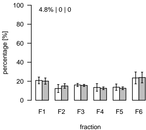
L2534 (m/z=812.65814; rt=14.11528) T/S Cluster: L-14.1-3
