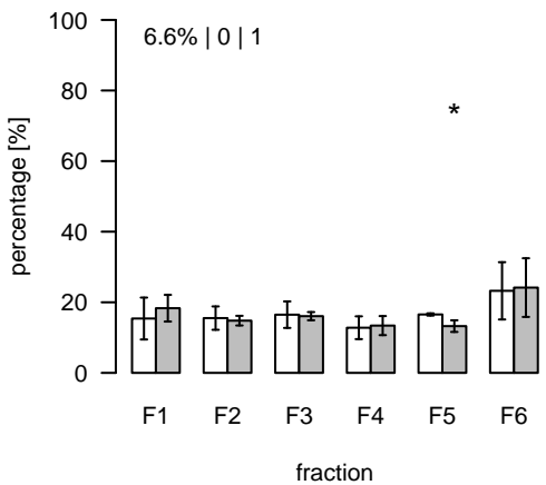
L2618 (m/z=1425.41018; rt=15.60846) T/S Cluster: L-15.6-5
