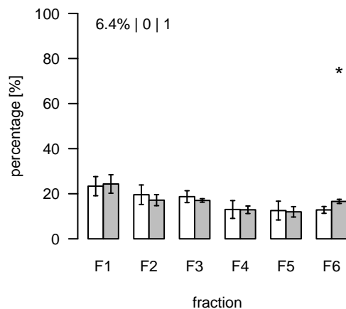
L305 (m/z=677.449712; rt=4.15479) T/S Cluster: L-4.2-4
