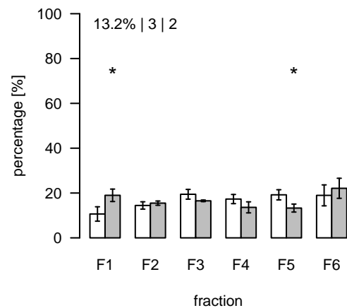
L2307 (m/z=170.123387; rt=11.3281) T/S Cluster: L-11.3-4
