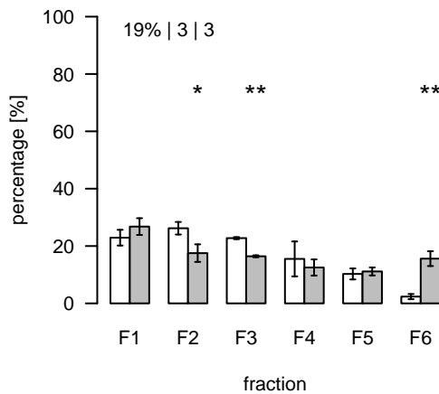
L1671 (m/z=780.535129; rt=8.70509) T/S Cluster: L-8.7-4
