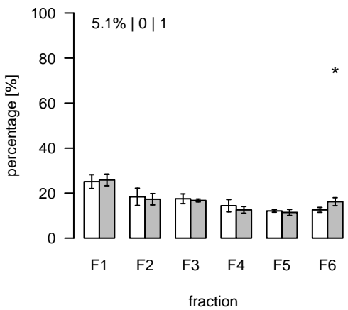
L2513 (m/z=895.706831; rt=12.79005) T/S Cluster: L-12.8-3
