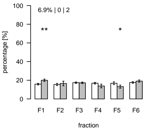
L1772 (m/z=908.611069; rt=8.91495) T/S Cluster: L-8.9-7
