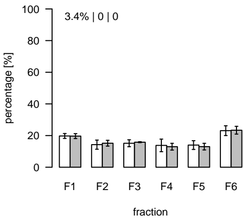
L497 (m/z=718.486128; rt=4.75589) T/S Cluster: L-4.8-2
