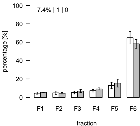
L17 (m/z=812.519897; rt=2.61006) T/S Cluster: L-2.6-2
