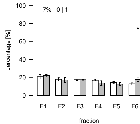
L2728 (m/z=952.893535; rt=16.26236) T/S Cluster: L-16.3-1
