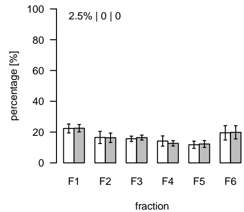
L944 (m/z=772.606223; rt=6.14022) T/S Cluster: L-6.1-6
