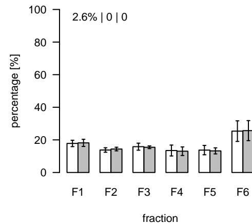
L863 (m/z=386.778878; rt=5.71578) T/S Cluster: L-5.7-4
