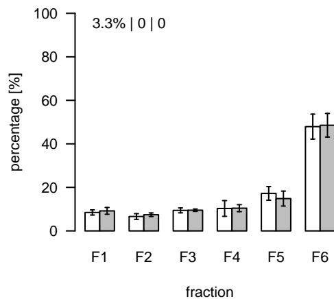
L1653 (m/z=467.827005; rt=8.64247) T/S Cluster: L-8.6-6
