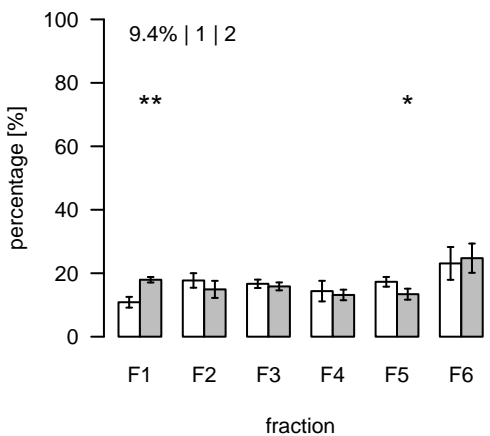
L2744 (m/z=564.163418; rt=16.54654) T/S Cluster: L-16.5-6
