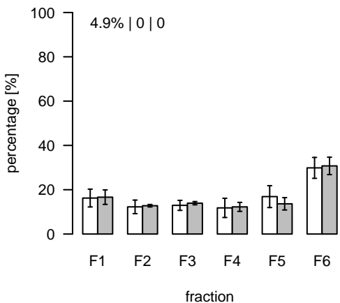
L136 (m/z=842.513579; rt=3.65223) T/S Cluster: L-3.7-3
