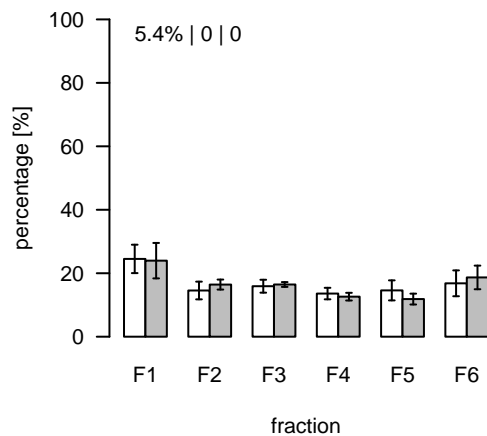
L1044 (m/z=396.284479; rt=6.54649) T/S Cluster: L-6.5-5
