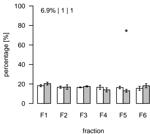
S374 (m/z=249.103192; rt=12.16165) T/S Cluster: S-12.2-4
