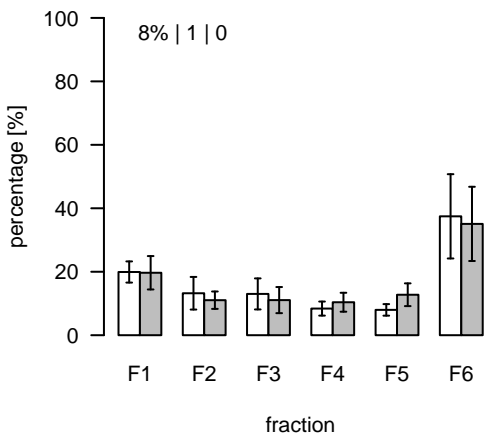
S860 (m/z=571.452411; rt=16.97576) T/S Cluster: S-17-3
