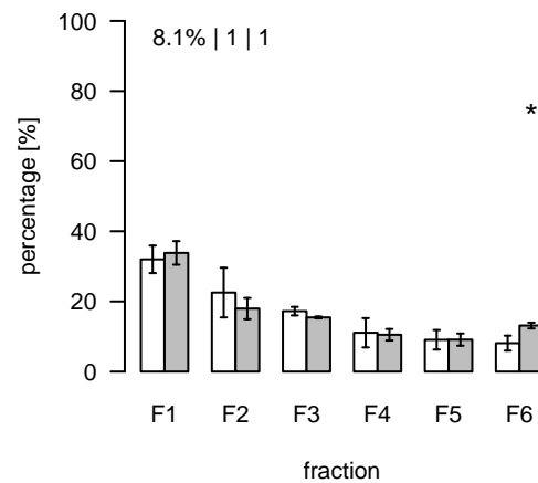
L792 (m/z=622.432026; rt=5.48551) T/S Cluster: L-5.5-1
