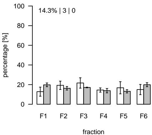
L2413 (m/z=709.497356; rt=11.588) T/S Cluster: L-11.6-2
