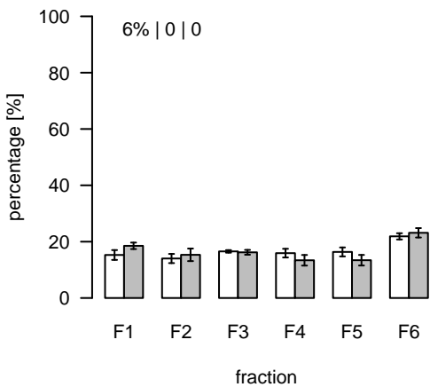
L1783 (m/z=909.528911; rt=8.91609) T/S Cluster: L-8.9-5
