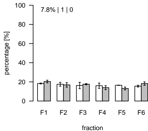
S761 (m/z=437.770233; rt=16.15265) T/S Cluster: S-16.2-2
