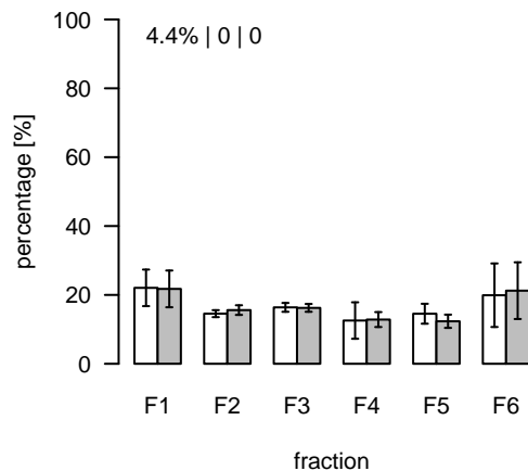
L1319 (m/z=781.561556; rt=7.32848) T/S Cluster: L-7.3-5
