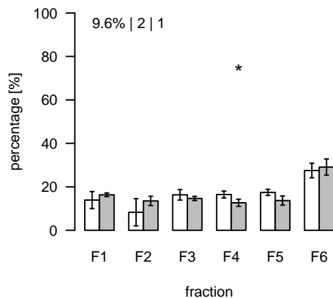
L1784 (m/z=302.523112; rt=8.91701) T/S Cluster: L-8.9-8
