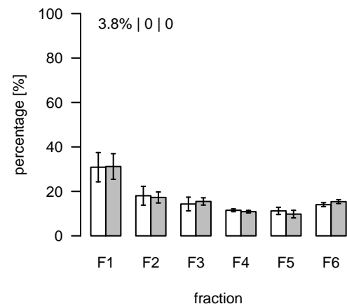
S393 (m/z=770.364877; rt=12.34045) T/S Cluster: S-12.3-8
