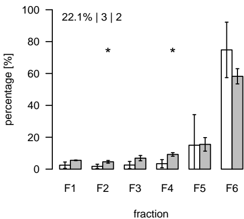
L1625 (m/z=923.522508; rt=8.492) T/S Cluster: L-8.5-4
