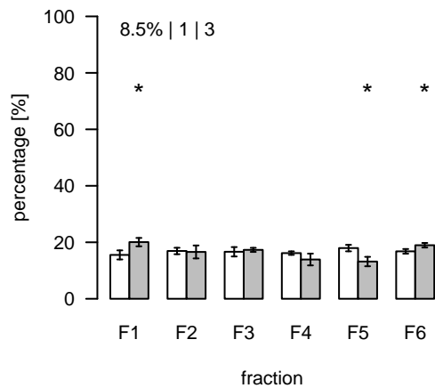
S353 (m/z=437.770462; rt=11.54149) T/S Cluster: S-11.5-1
