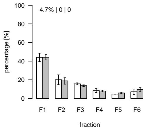
S115 (m/z=358.1137; rt=4.91112) T/S Cluster: S-4.9-1
