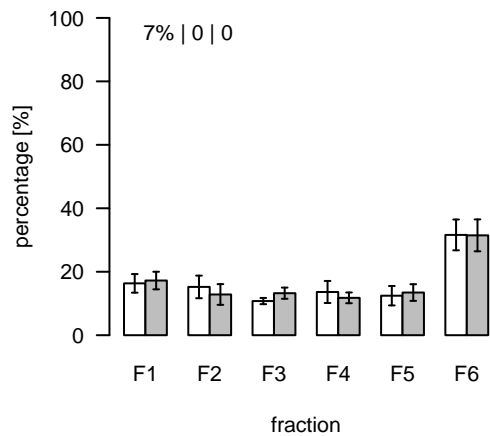
L2446 (m/z=217.898746; rt=11.84515) T/S Cluster: L-11.8-5
