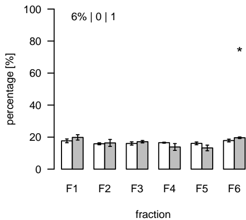
S485 (m/z=289.216643; rt=12.91196) T/S Cluster: S-12.9-16
