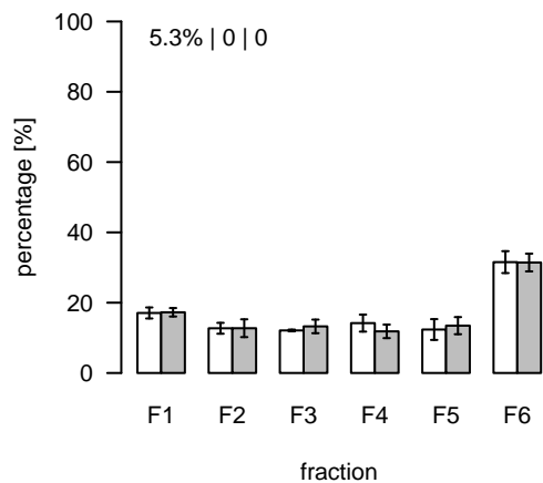
L2448 (m/z=437.29867; rt=11.84559) T/S Cluster: L-11.8-5
