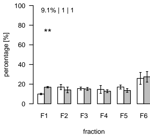
L2772 (m/z=1205.300515; rt=16.96565) T/S Cluster: L-17-2
