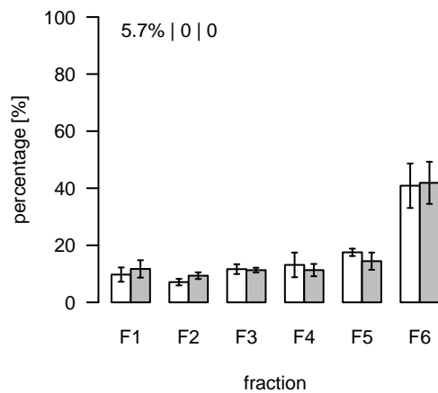
L1097 (m/z=152.90724; rt=6.54818) T/S Cluster: L-6.5-1
