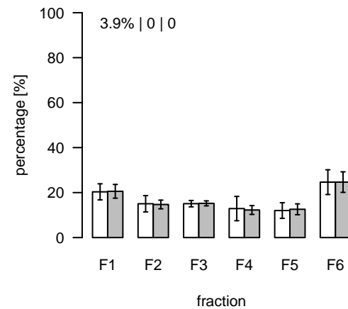
L824 (m/z=797.558037; rt=5.69244) T/S Cluster: L-5.7-4
