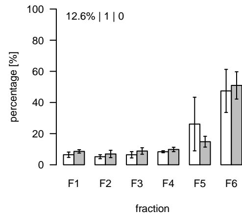
L1238 (m/z=762.499191; rt=6.93733) T/S Cluster: L-6.9-5
