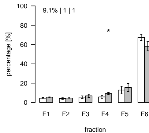
L521 (m/z=824.559558; rt=4.80697) T/S Cluster: L-4.8-10
