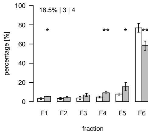
L1977 (m/z=907.487693; rt=9.88116) T/S Cluster: L-9.9-2
