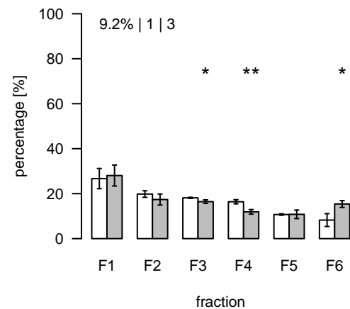
L1690 (m/z=758.572754; rt=8.70703) T/S Cluster: L-8.7-5
