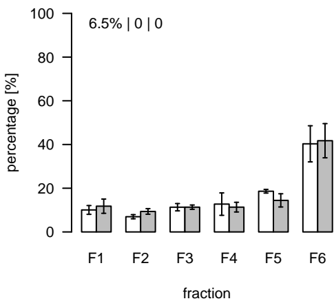
L1056 (m/z=191.384475; rt=6.54751) T/S Cluster: L-6.5-1
