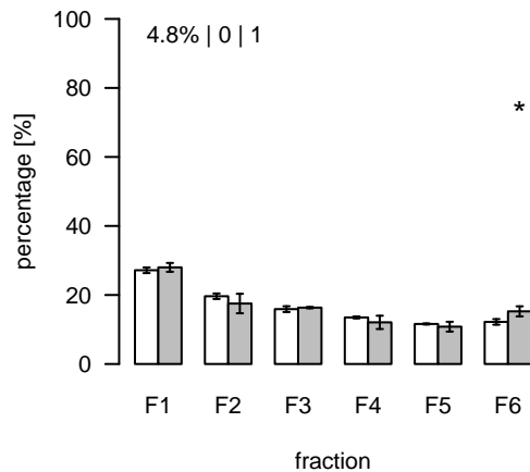
L2290 (m/z=354.255784; rt=11.32794) T/S Cluster: L-11.3-11
