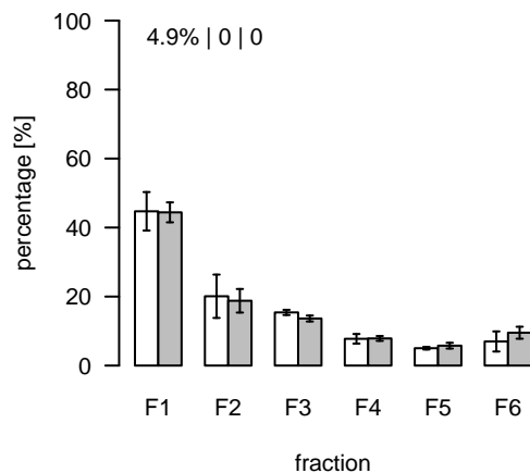
S114 (m/z=179.057143; rt=4.91102) T/S Cluster: S-4.9-1
