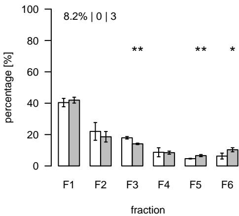
S220 (m/z=579.172002; rt=7.19576) T/S Cluster: S-7.2-2
