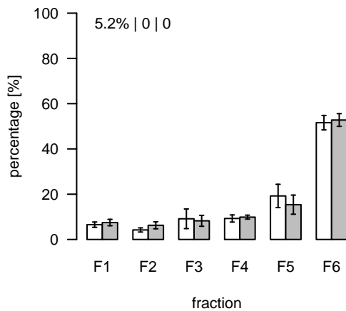
L2039 (m/z=462.775013; rt=10.21267) T/S Cluster: L-10.2-2
