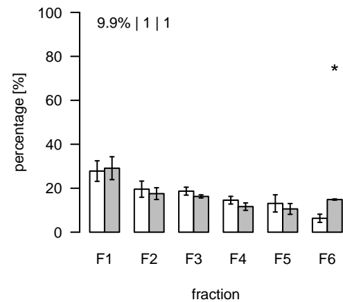
L1754 (m/z=787.598693; rt=8.88016) T/S Cluster: L-8.9-1
