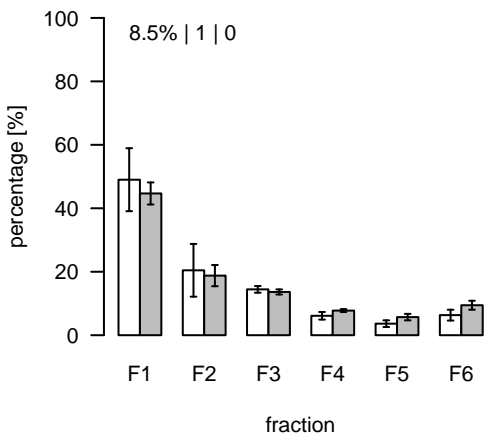
S170 (m/z=1209.370802; rt=6.57516) T/S Cluster: S-6.6-2
