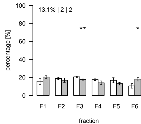
L1179 (m/z=961.584171; rt=6.66074) T/S Cluster: L-6.7-6
