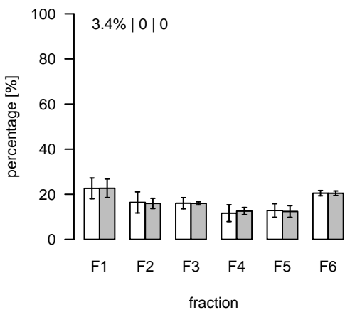
L63 (m/z=722.491438; rt=3.39937) T/S Cluster: L-3.4-5
