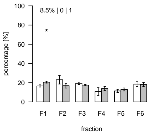
S788 (m/z=660.544253; rt=16.40128) T/S Cluster: S-16.4-1
