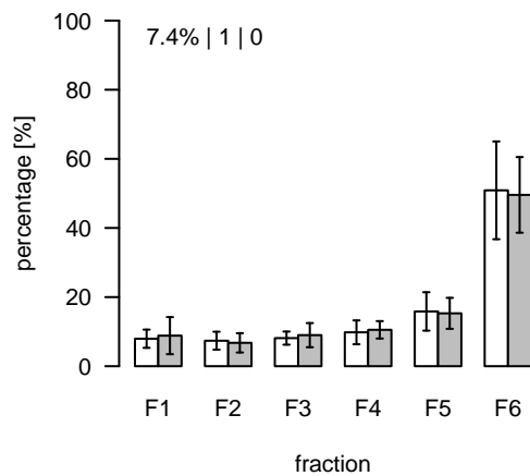
L1603 (m/z=891.568964; rt=8.29586) T/S Cluster: L-8.3-3
