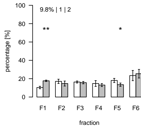
L2582 (m/z=909.241436; rt=15.36536) T/S Cluster: L-15.4-3
