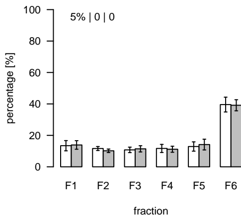
L2488 (m/z=436.289353; rt=12.38414) T/S Cluster: L-12.4-3
