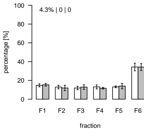
L2452 (m/z=874.550347; rt=11.84729) T/S Cluster: L-11.8-5
