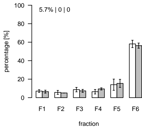
L105 (m/z=593.259852; rt=3.57047) T/S Cluster: L-3.6-2
