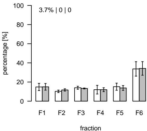
L584 (m/z=795.54141; rt=4.8972) T/S Cluster: L-4.9-10
