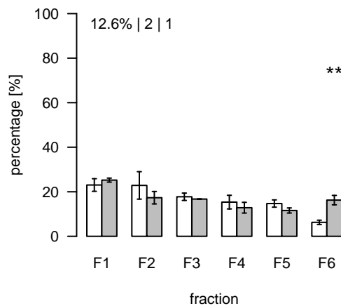
L780 (m/z=416.369805; rt=5.39997) T/S Cluster: L-5.4-4
