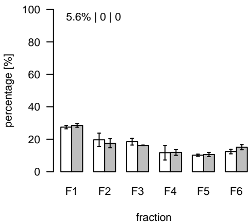
L1473 (m/z=717.576433; rt=7.93871) T/S Cluster: L-7.9-13
