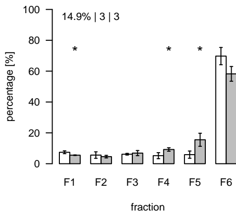
L232 (m/z=810.508967; rt=3.90109) T/S Cluster: L-3.9-5
