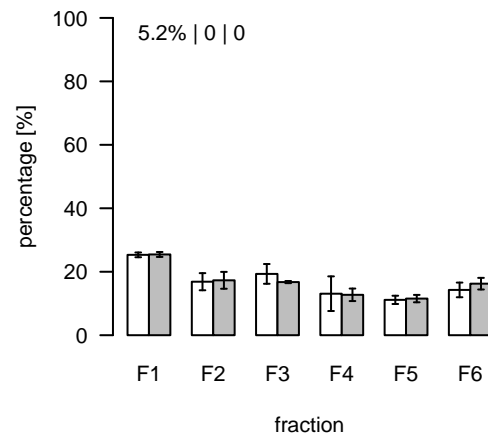
L2171 (m/z=421.840377; rt=10.66197) T/S Cluster: L-10.7-1
