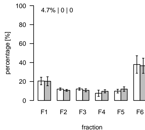
S576 (m/z=670.395613; rt=14.34756) T/S Cluster: S-14.3-4
