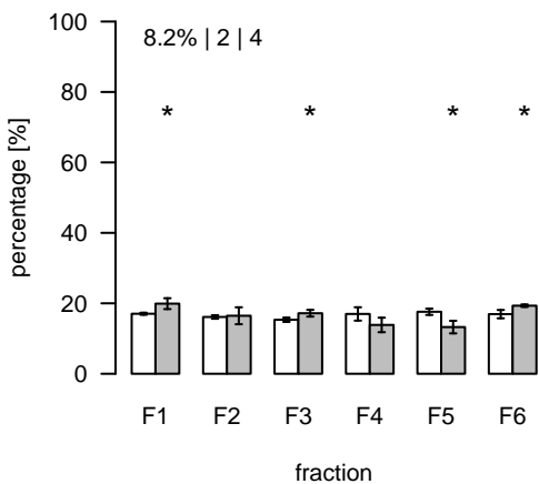
S535 (m/z=437.769042; rt=13.50714) T/S Cluster: S-13.5-2
