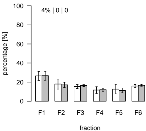
L2182 (m/z=788.601513; rt=10.7472) T/S Cluster: L-10.7-3
