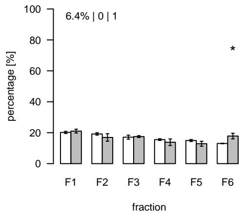
L2677 (m/z=921.27974; rt=15.84438) T/S Cluster: L-15.8-4
