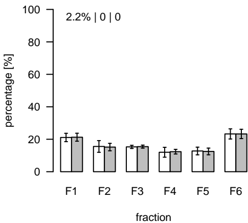
L1270 (m/z=754.546397; rt=7.18767) T/S Cluster: L-7.2-2
