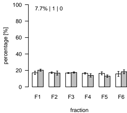
S683 (m/z=437.781498; rt=15.23024) T/S Cluster: S-15.2-2
