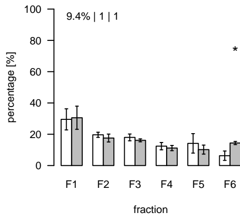
L1748 (m/z=786.598216; rt=8.87933) T/S Cluster: L-8.9-1
