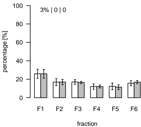
L461 (m/z=702.473921; rt=4.59548) T/S Cluster: L-4.6-3
