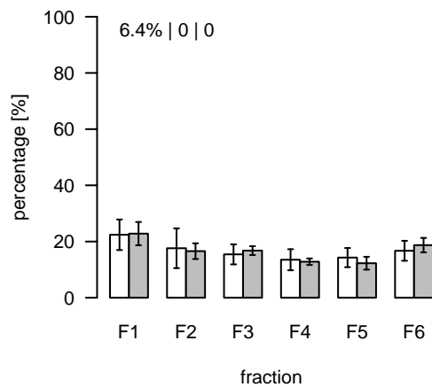
L458 (m/z=690.473676; rt=4.58216) T/S Cluster: L-4.6-3
