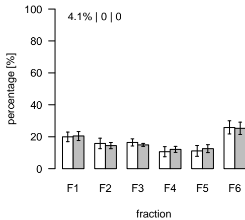
L310 (m/z=810.554037; rt=4.18369) T/S Cluster: L-4.2-7
