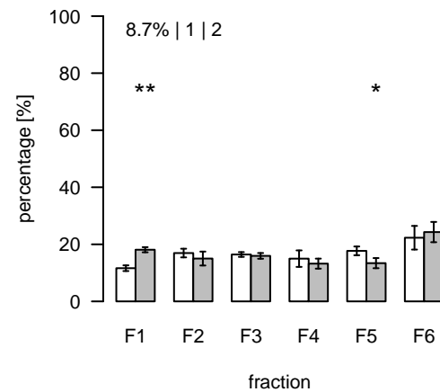
L2635 (m/z=982.246206; rt=15.81029) T/S Cluster: L-15.8-1
