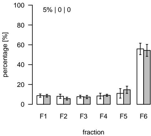
S442 (m/z=894.474351; rt=12.64522) T/S Cluster: S-12.6-18
