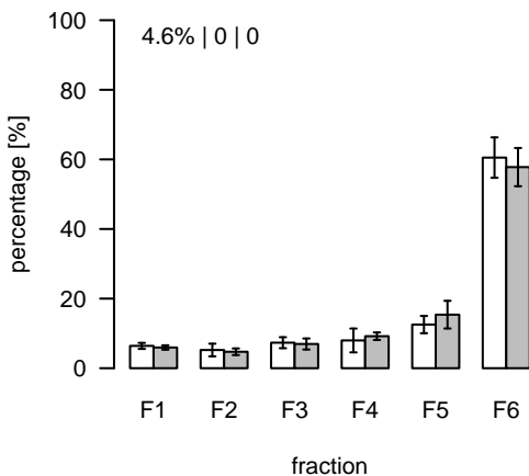
L1891 (m/z=772.559599; rt=9.56004) T/S Cluster: L-9.6-1
