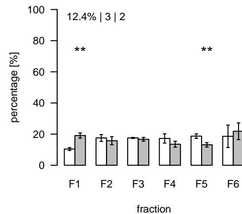
L2727 (m/z=1097.328083; rt=16.18005) T/S Cluster: L-16.2-6
