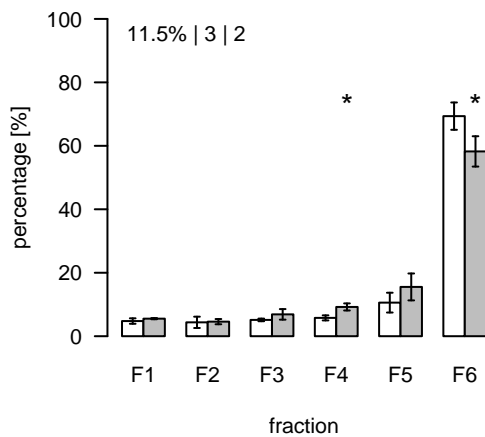
L117 (m/z=792.494438; rt=3.60603) T/S Cluster: L-3.6-5
