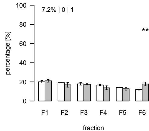
L2668 (m/z=925.312678; rt=15.84396) T/S Cluster: L-15.8-4
