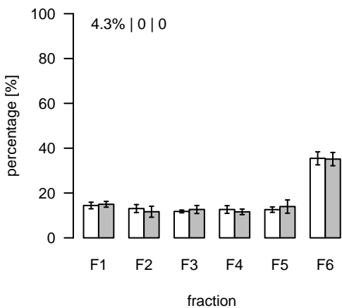
L2470 (m/z=290.523863; rt=11.85026) T/S Cluster: L-11.9-1
