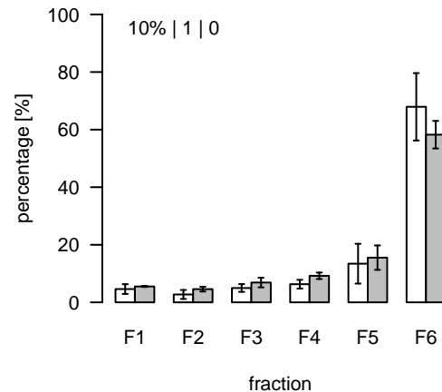
L1611 (m/z=941.564783; rt=8.42457) T/S Cluster: L-8.4-4
