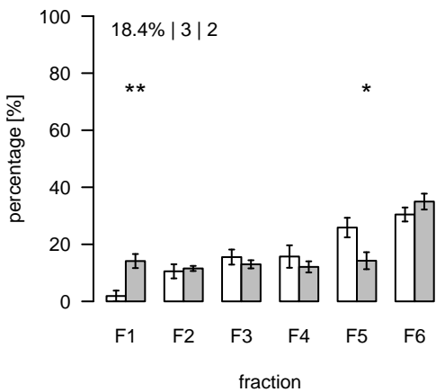
L833 (m/z=953.635954; rt=5.70317) T/S Cluster: L-5.7-9
