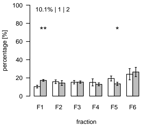
L2519 (m/z=379.613469; rt=14.00343) T/S Cluster: L-14-1
