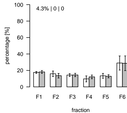
L718 (m/z=794.508086; rt=5.23126) T/S Cluster: L-5.2-7
