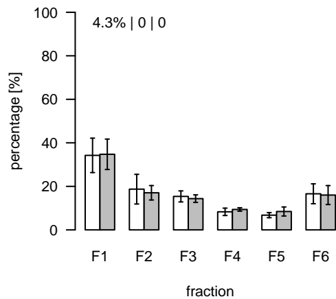
S316 (m/z=600.29045; rt=10.05942) T/S Cluster: S-10.1-1
