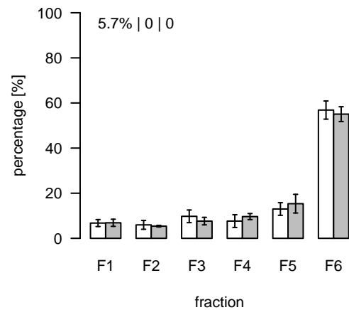
L2209 (m/z=869.562042; rt=11.0044) T/S Cluster: L-11-2
