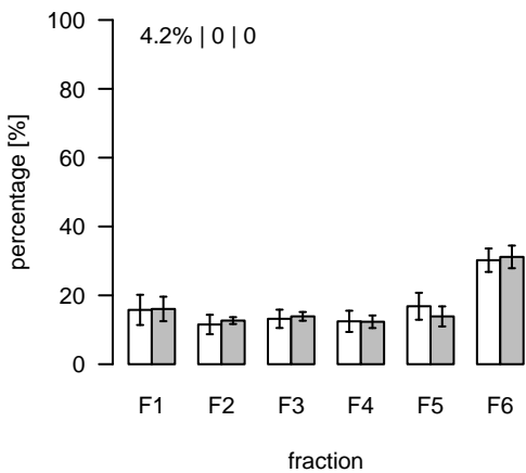
L101 (m/z=421.258625; rt=3.54877) T/S Cluster: L-3.5-8
