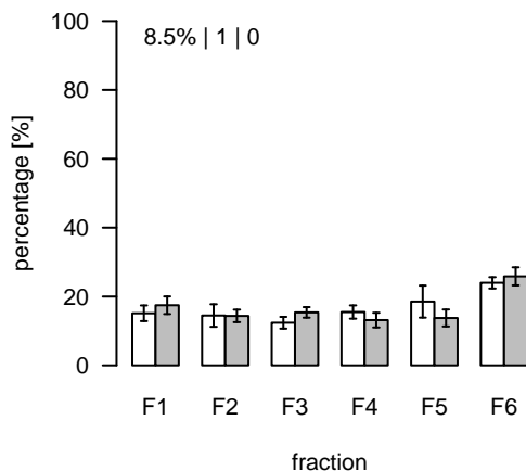
L635 (m/z=849.527124; rt=4.94971) T/S Cluster: L-4.9-17
