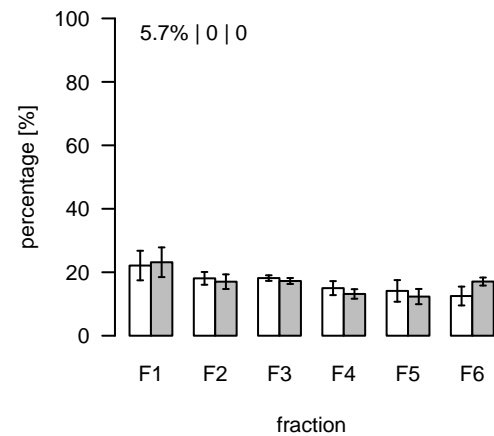
L1206 (m/z=388.794852; rt=6.69782) T/S Cluster: L-6.7-11
