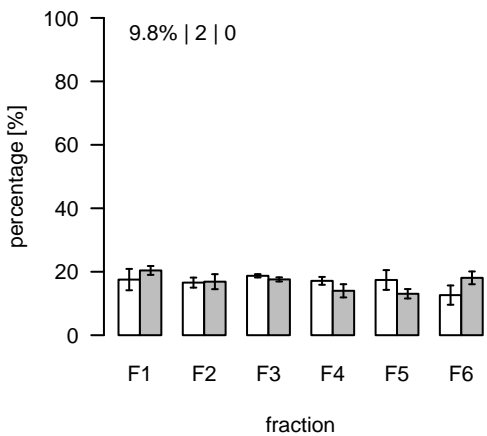
L1045 (m/z=786.468917; rt=6.54666) T/S Cluster: L-6.5-7
