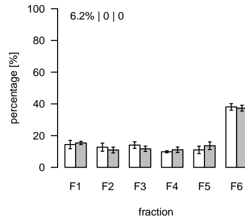
S401 (m/z=824.427303; rt=12.39453) T/S Cluster: S-12.4-7
