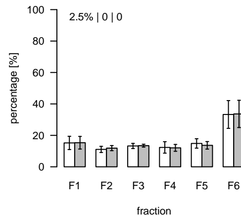
L587 (m/z=397.269964; rt=4.89811) T/S Cluster: L-4.9-10
