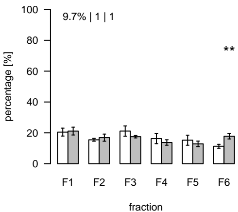
L2561 (m/z=768.710425; rt=15.24836) T/S Cluster: L-15.2-2
