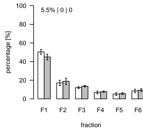
S52 (m/z=512.130114; rt=4.64473) T/S Cluster: S-4.6-1
