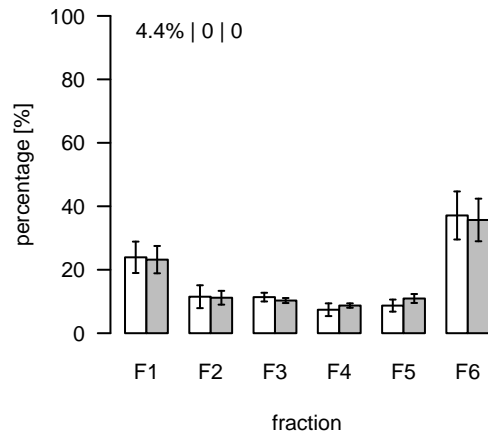
S260 (m/z=652.413965; rt=7.7598) T/S Cluster: S-7.8-1
