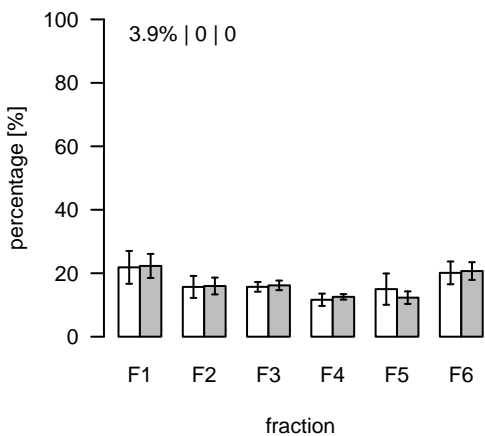
L1597 (m/z=757.559344; rt=8.2746) T/S Cluster: L-8.3-1
