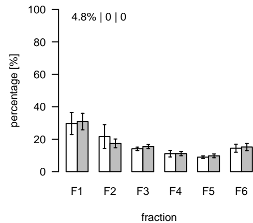
S325 (m/z=184.073387; rt=10.06364) T/S Cluster: S-10.1-1
