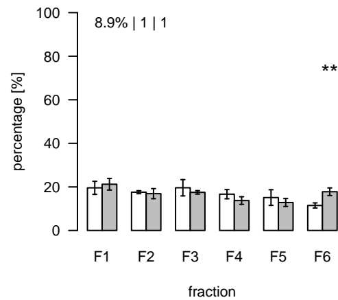
L2602 (m/z=797.74569; rt=15.55463) T/S Cluster: L-15.6-1
