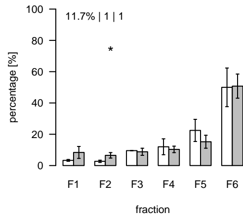
L2202 (m/z=893.54611; rt=10.91704) T/S Cluster: L-10.9-2
