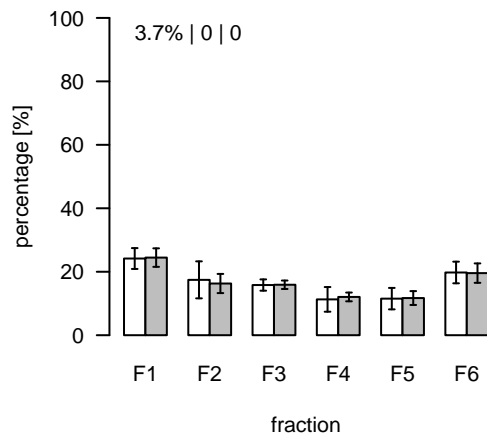
L947 (m/z=773.555626; rt=6.14153) T/S Cluster: L-6.1-6
