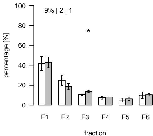
S641 (m/z=652.421196; rt=14.87387) T/S Cluster: S-14.9-2
