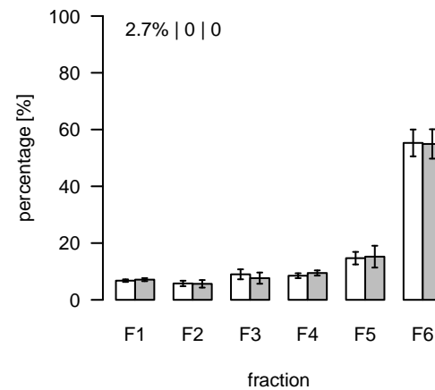
L740 (m/z=972.594867; rt=5.3013) T/S Cluster: L-5.3-5
