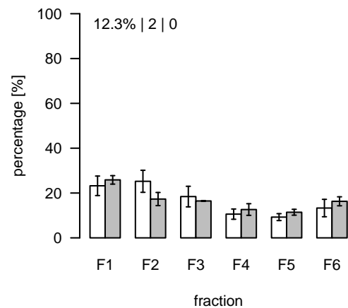
S852 (m/z=1194.826114; rt=16.95159) T/S Cluster: S-17-1
