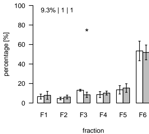
L1862 (m/z=908.46245; rt=9.43485) T/S Cluster: L-9.4-1
