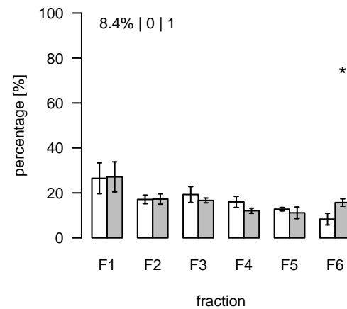
L378 (m/z=839.533048; rt=4.37985) T/S Cluster: L-4.4-8
