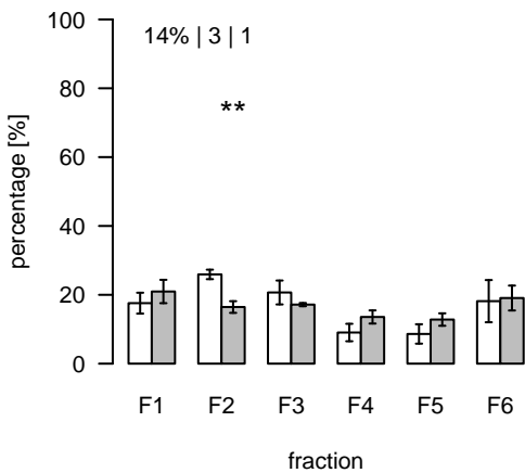
S790 (m/z=229.143892; rt=16.45352) T/S Cluster: S-16.5-1
