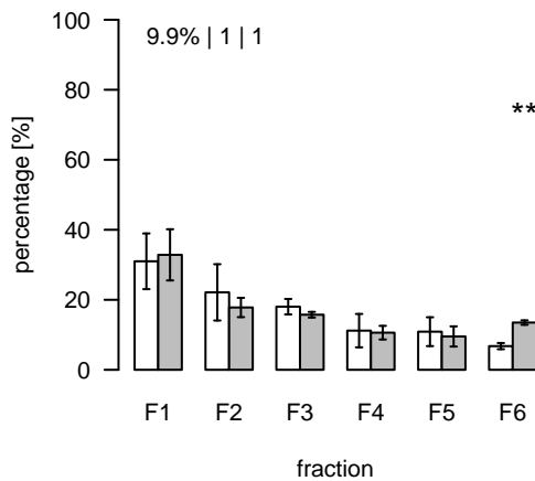
L233 (m/z=680.434786; rt=3.90204) T/S Cluster: L-3.9-6
