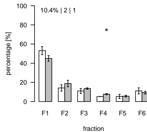
S54 (m/z=494.100671; rt=4.6453) T/S Cluster: S-4.6-1
