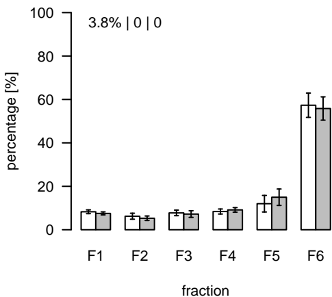
L272 (m/z=826.524257; rt=4.05438) T/S Cluster: L-4.1-1
