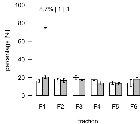
L1457 (m/z=388.343832; rt=7.91226) T/S Cluster: L-7.9-11
