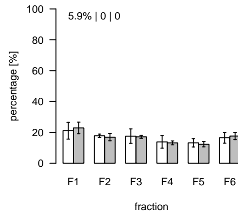
L828 (m/z=815.576556; rt=5.69693) T/S Cluster: L-5.7-7
