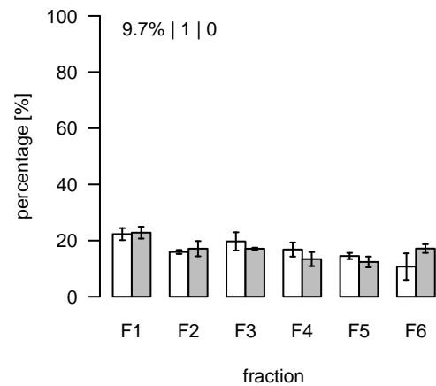
S432 (m/z=437.229836; rt=12.55419) T/S Cluster: S-12.6-9
