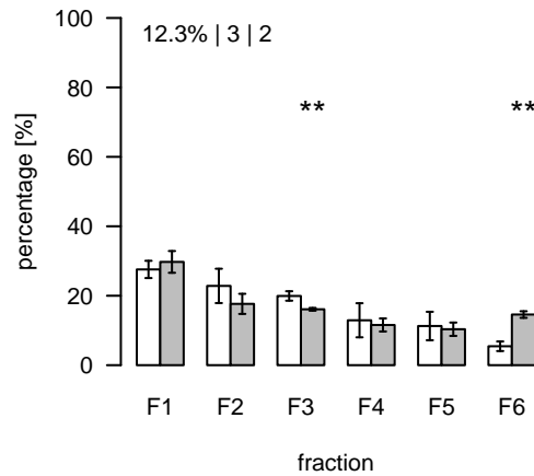
L1933 (m/z=782.548166; rt=9.59856) T/S Cluster: L-9.6-3
