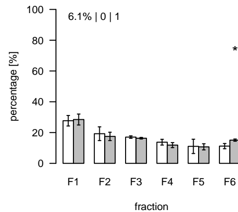
L1918 (m/z=761.592184; rt=9.59703) T/S Cluster: L-9.6-3
