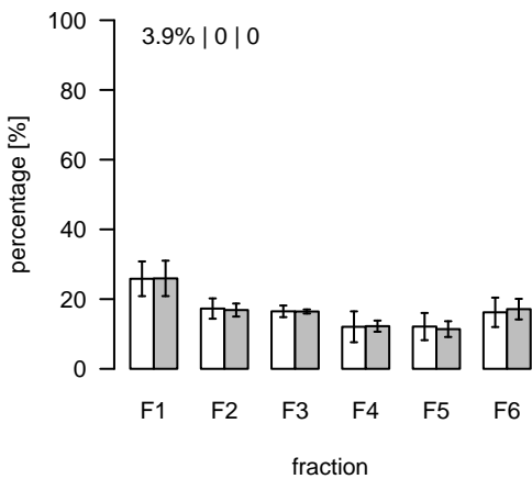
L1962 (m/z=786.604757; rt=9.82717) T/S Cluster: L-9.8-1
