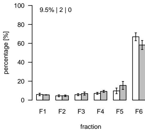
L636 (m/z=583.438992; rt=4.95077) T/S Cluster: L-5-1
