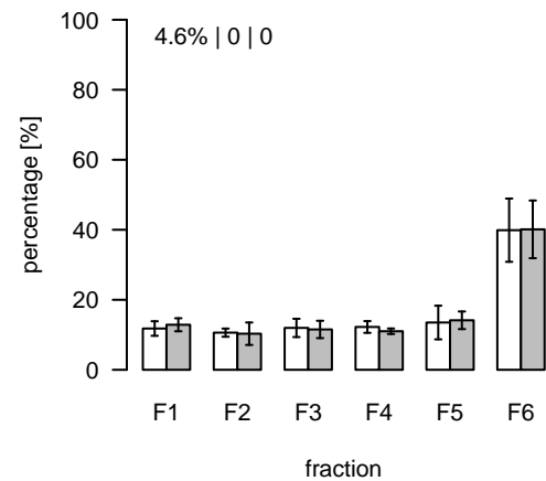
S368 (m/z=708.418704; rt=12.08746) T/S Cluster: S-12.1-4
