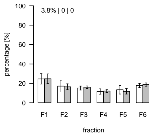
L186 (m/z=695.471953; rt=3.74089) T/S Cluster: L-3.7-22
