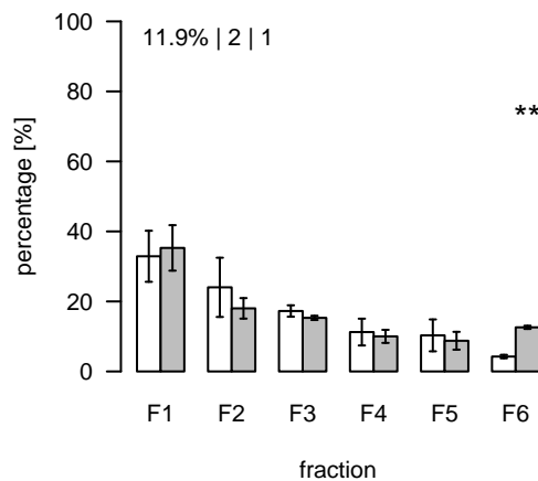
L159 (m/z=666.436865; rt=3.67489) T/S Cluster: L-3.7-14
