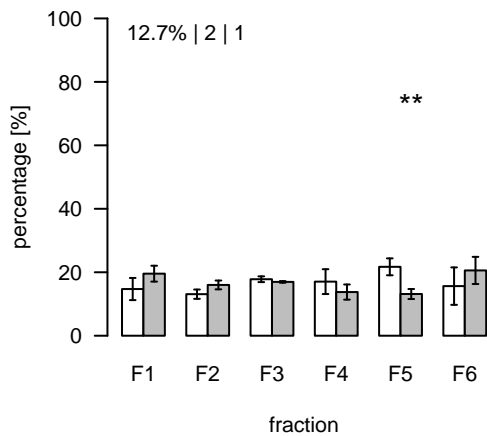
L1352 (m/z=813.523604; rt=7.3489) T/S Cluster: L-7.3-11
