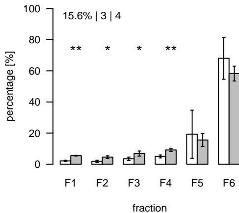
L2047 (m/z=911.544359; rt=10.29426) T/S Cluster: L-10.3-1
