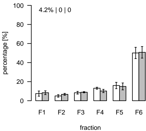
L1336 (m/z=794.573786; rt=7.34701) T/S Cluster: L-7.3-3
