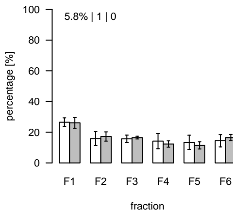
L1945 (m/z=381.298183; rt=9.6509) T/S Cluster: L-9.7-1
