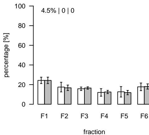
L1634 (m/z=732.537958; rt=8.6011) T/S Cluster: L-8.6-5
