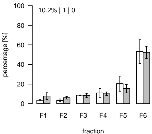
L2203 (m/z=893.474686; rt=10.91718) T/S Cluster: L-10.9-2
