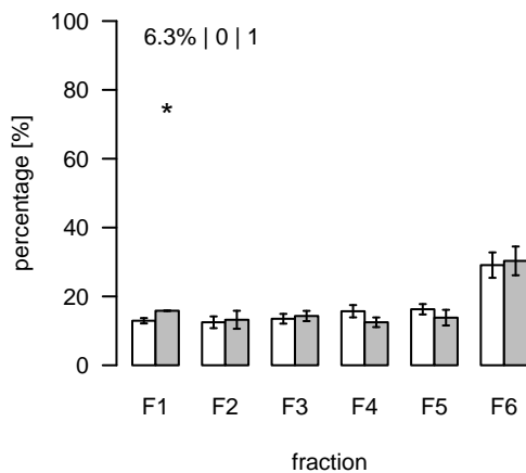
L2122 (m/z=446.746174; rt=10.50593) T/S Cluster: L-10.5-11
