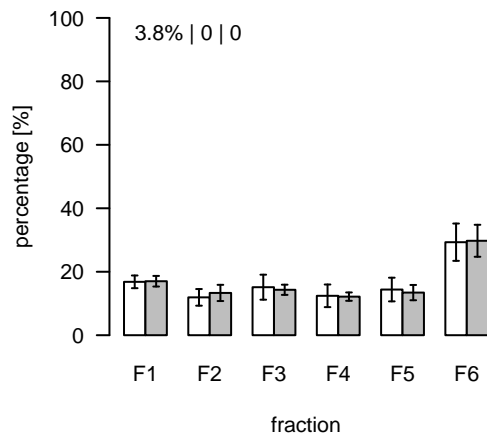
L843 (m/z=800.550725; rt=5.7092) T/S Cluster: L-5.7-10
