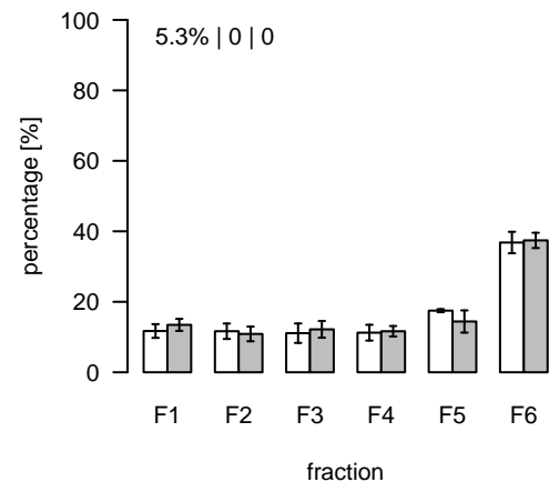
S386 (m/z=704.38868; rt=12.28762) T/S Cluster: S-12.3-3
