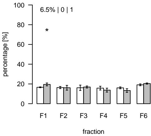
S439 (m/z=426.28605; rt=12.61797) T/S Cluster: S-12.6-16
