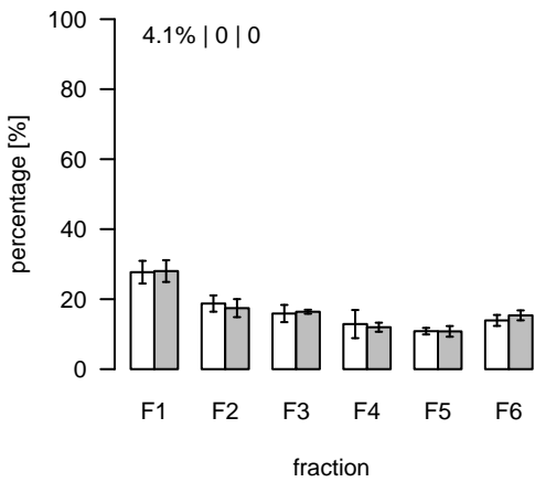
S436 (m/z=882.57329; rt=12.57246) T/S Cluster: S-12.6-13
