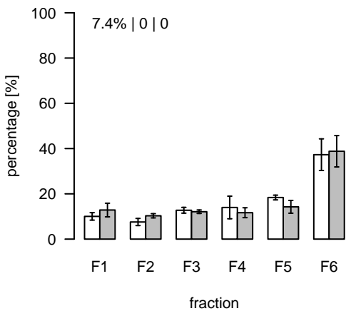
L1151 (m/z=478.821194; rt=6.65409) T/S Cluster: L-6.7-3
