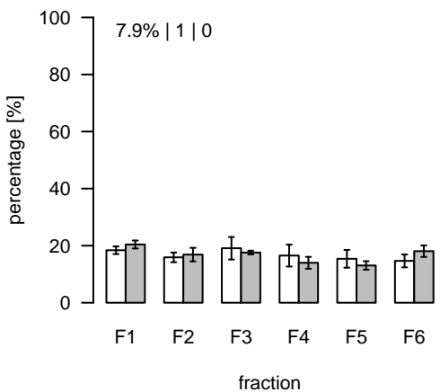
L2617 (m/z=874.789437; rt=15.59536) T/S Cluster: L-15.6-1
