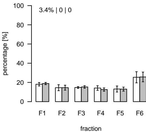
L1254 (m/z=802.600881; rt=7.1232) T/S Cluster: L-7.1-5
