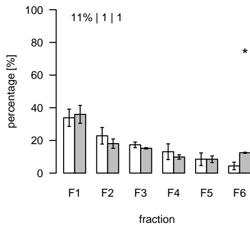
L1376 (m/z=738.511213; rt=7.50026) T/S Cluster: L-7.5-4
