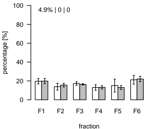
L892 (m/z=797.532109; rt=5.86987) T/S Cluster: L-5.9-1
