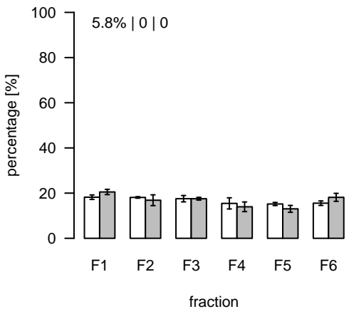
L2741 (m/z=960.895814; rt=16.54507) T/S Cluster: L-16.5-5
