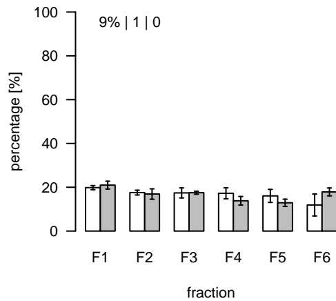
L971 (m/z=797.552708; rt=6.19016) T/S Cluster: L-6.2-8
