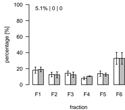
S372 (m/z=722.398853; rt=12.16149) T/S Cluster: S-12.2-2
