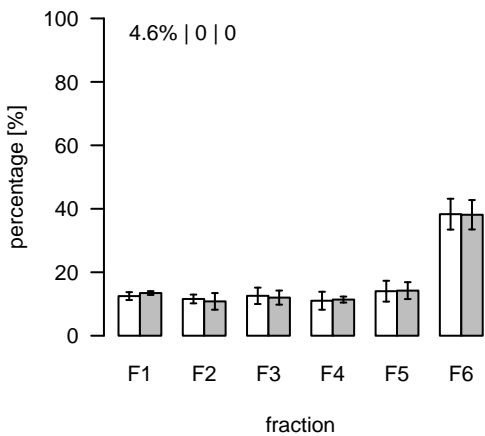
S412 (m/z=1048.573305; rt=12.5224) T/S Cluster: S-12.5-6
