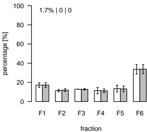
L848 (m/z=399.28909; rt=5.71169) T/S Cluster: L-5.7-4
