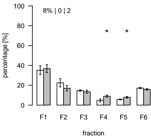
S700 (m/z=808.542853; rt=15.44717) T/S Cluster: S-15.4-4
