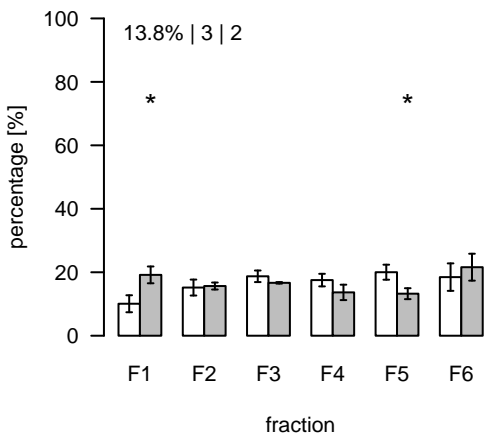
L2304 (m/z=340.732909; rt=11.32806) T/S Cluster: L-11.3-4
