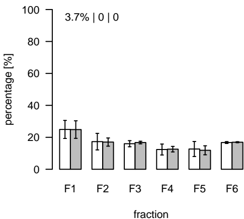
L126 (m/z=638.444823; rt=3.61746) T/S Cluster: L-3.6-7
