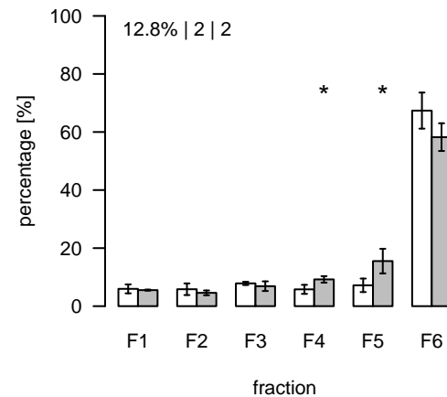
S762 (m/z=926.587194; rt=16.16484) T/S Cluster: S-16.2-3
