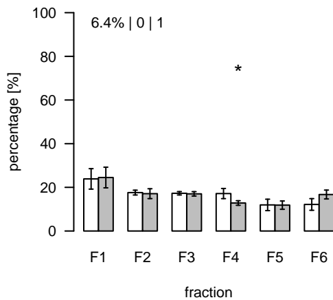
L1504 (m/z=378.767913; rt=7.93996) T/S Cluster: L-7.9-14
