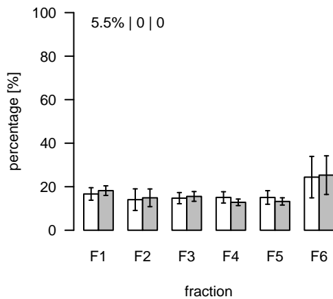
L2072 (m/z=907.527807; rt=10.4285) T/S Cluster: L-10.4-2
