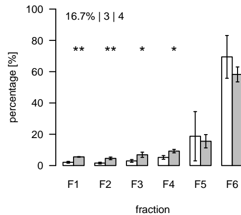
L2051 (m/z=909.541249; rt=10.29466) T/S Cluster: L-10.3-1
