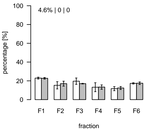
L2424 (m/z=872.715793; rt=11.73938) T/S Cluster: L-11.7-3
