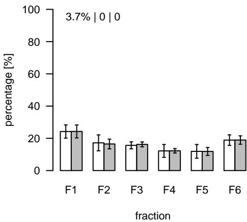
L949 (m/z=386.275206; rt=6.14158) T/S Cluster: L-6.1-6
