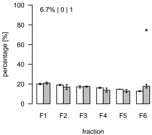
L2666 (m/z=461.158572; rt=15.8436) T/S Cluster: L-15.8-4
