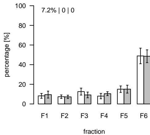
L2486 (m/z=871.577213; rt=12.3835) T/S Cluster: L-12.4-1
