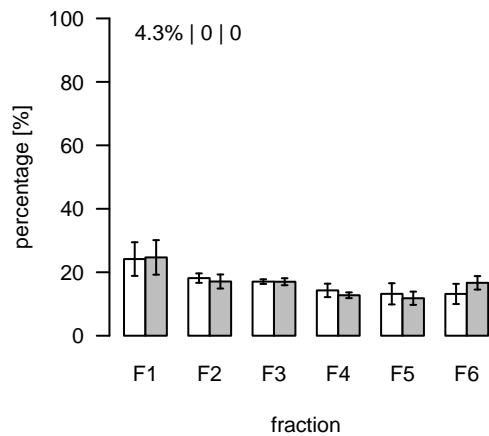
L1488 (m/z=189.390513; rt=7.93905) T/S Cluster: L-7.9-14
