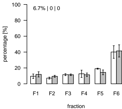
L1061 (m/z=767.545717; rt=6.54755) T/S Cluster: L-6.5-1
