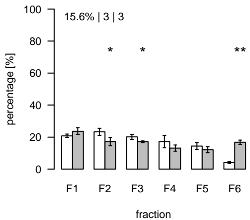
L2085 (m/z=916.549127; rt=10.49953) T/S Cluster: L-10.5-8
