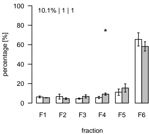
L325 (m/z=798.536792; rt=4.25506) T/S Cluster: L-4.3-1
