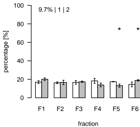
S427 (m/z=210.628363; rt=12.55145) T/S Cluster: S-12.6-3
