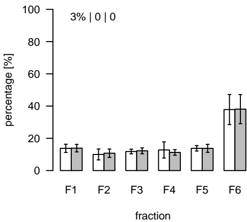
L605 (m/z=843.527252; rt=4.90645) T/S Cluster: L-4.9-15
