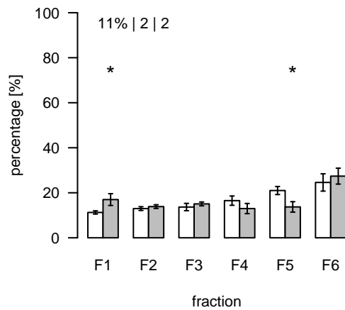
L512 (m/z=787.486257; rt=4.78656) T/S Cluster: L-4.8-3
