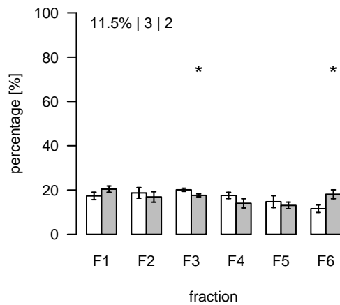
L1178 (m/z=975.551241; rt=6.66073) T/S Cluster: L-6.7-7
