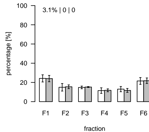
L2225 (m/z=830.675648; rt=11.15537) T/S Cluster: L-11.2-1
