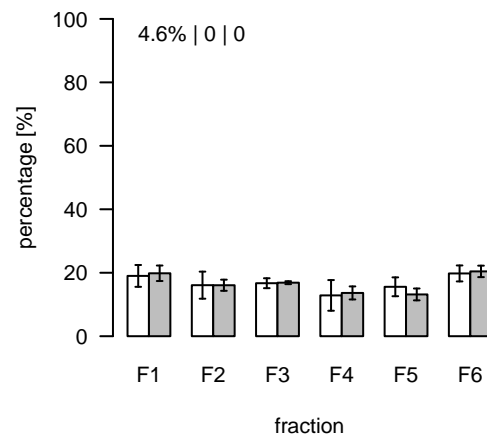
L565 (m/z=742.513855; rt=4.87059) T/S Cluster: L-4.9-3
