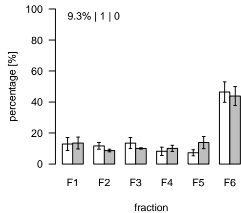
S614 (m/z=842.513989; rt=14.68184) T/S Cluster: S-14.7-4
