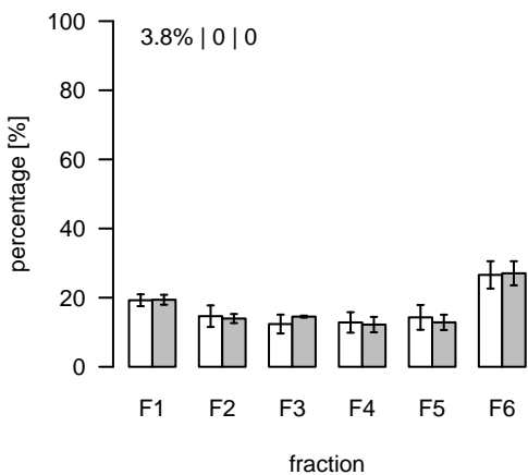
L412 (m/z=805.546295; rt=4.43073) T/S Cluster: L-4.4-1
