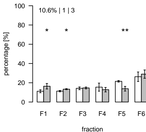
L1646 (m/z=940.611341; rt=8.63636) T/S Cluster: L-8.6-8
