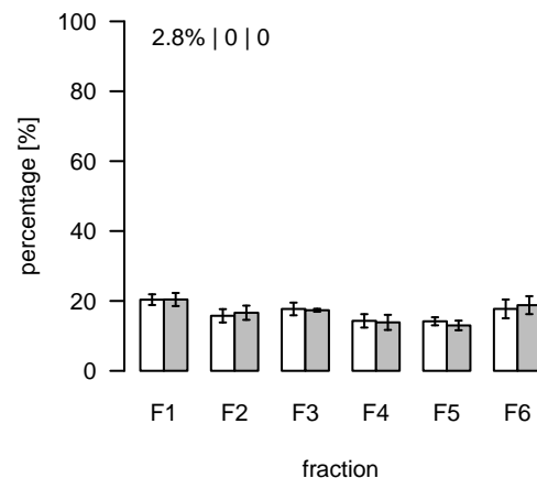
L2140 (m/z=429.852138; rt=10.60934) T/S Cluster: L-10.6-3
