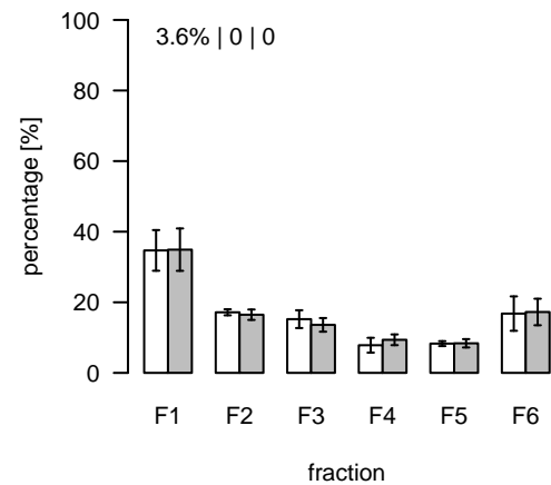
S684 (m/z=524.372504; rt=15.25043) T/S Cluster: S-15.3-1
