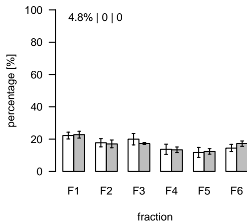
L309 (m/z=750.496153; rt=4.18119) T/S Cluster: L-4.2-3
