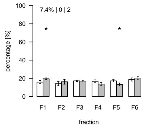
L1798 (m/z=455.275245; rt=8.91855) T/S Cluster: L-8.9-11
