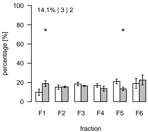
L2322 (m/z=340.22938; rt=11.32829) T/S Cluster: L-11.3-4
