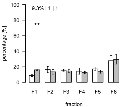
L2798 (m/z=1352.385961; rt=18.07315) T/S Cluster: L-18.1-1
