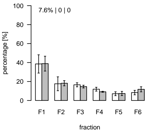
S151 (m/z=428.205446; rt=5.84812) T/S Cluster: S-5.8-2
