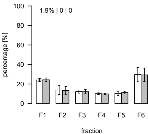
S417 (m/z=720.401855; rt=12.53936) T/S Cluster: S-12.5-9
