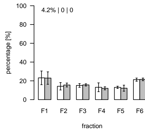
L2220 (m/z=842.675239; rt=11.03921) T/S Cluster: L-11-4
