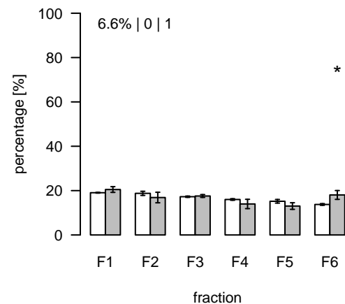
L2700 (m/z=995.338274; rt=16.15619) T/S Cluster: L-16.2-1
