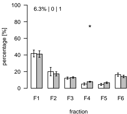
S705 (m/z=808.573615; rt=15.51055) T/S Cluster: S-15.5-1
