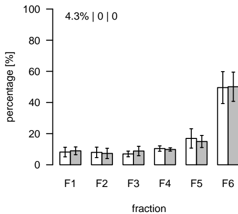
L129 (m/z=806.48662; rt=3.62504) T/S Cluster: L-3.6-5
