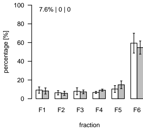
L707 (m/z=782.504885; rt=5.2137) T/S Cluster: L-5.2-5
