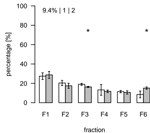
L1688 (m/z=253.196352; rt=8.70695) T/S Cluster: L-8.7-5
