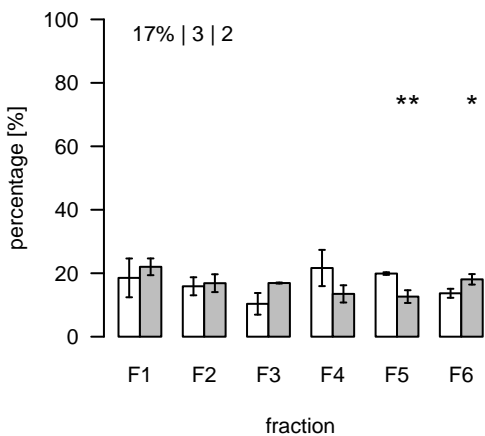
S850 (m/z=520.437709; rt=16.84106) T/S Cluster: S-16.8-2
