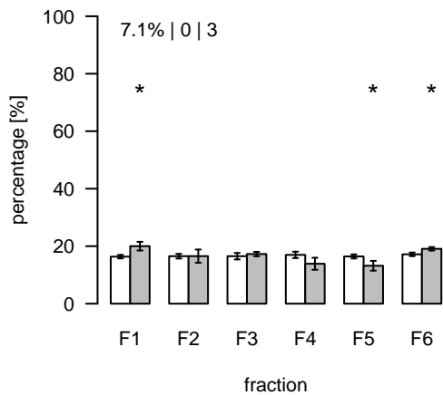
S492 (m/z=153.613887; rt=12.91265) T/S Cluster: S-12.9-22
