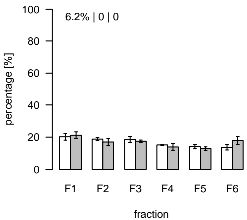
L2557 (m/z=774.276005; rt=14.97215) T/S Cluster: L-15-1
