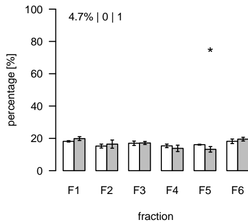
S467 (m/z=108.413383; rt=12.9093) T/S Cluster: S-12.9-5
