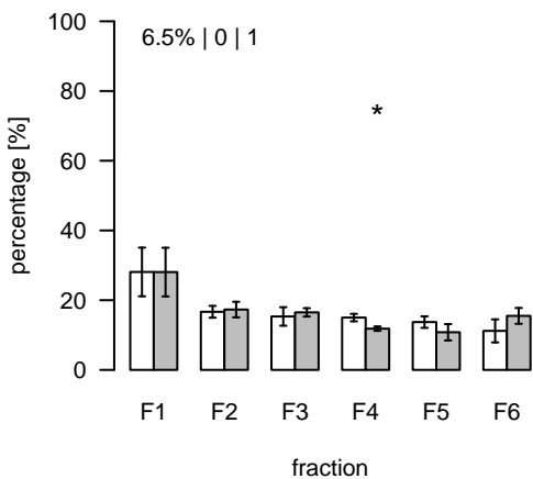
S148 (m/z=382.144032; rt=5.79654) T/S Cluster: S-5.8-1
