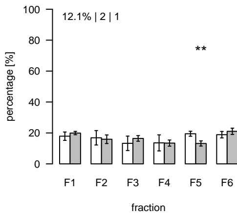
S296 (m/z=437.736581; rt=9.01797) T/S Cluster: S-9-2
