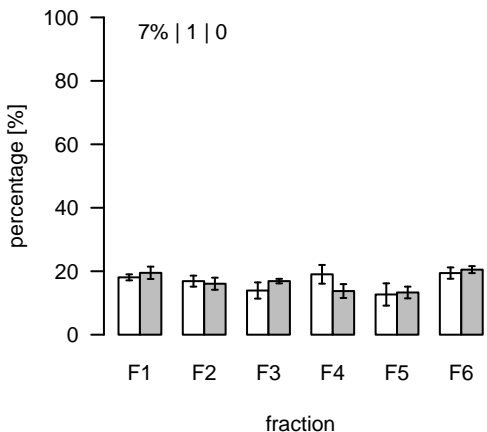
L1607 (m/z=437.752312; rt=8.39698) T/S Cluster: L-8.4-3
