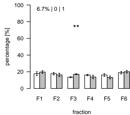
S513 (m/z=400.234576; rt=13.11391) T/S Cluster: S-13.1-5
