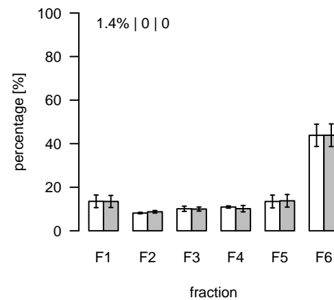
L557 (m/z=808.55929; rt=4.84721) T/S Cluster: L-4.8-10
