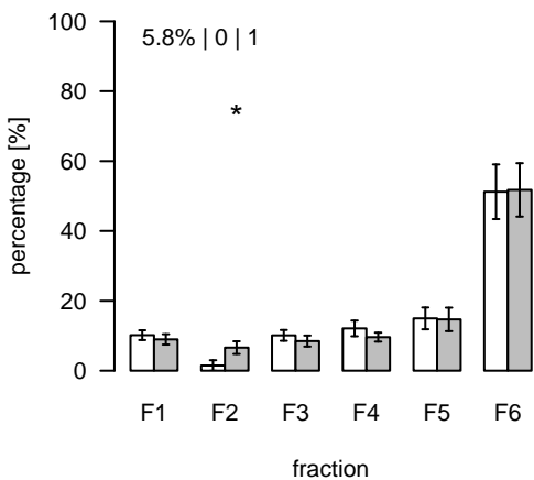
L661 (m/z=818.554508; rt=5.01452) T/S Cluster: L-5-1
