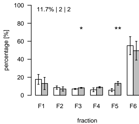
S833 (m/z=586.439884; rt=16.57441) T/S Cluster: S-16.6-1
