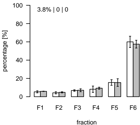
L524 (m/z=782.504008; rt=4.80826) T/S Cluster: L-4.8-10
