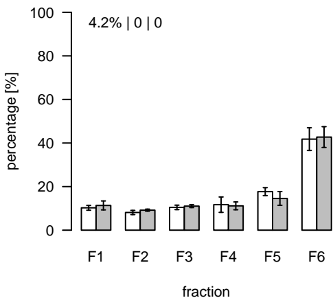
L1440 (m/z=934.608819; rt=7.90233) T/S Cluster: L-7.9-9
