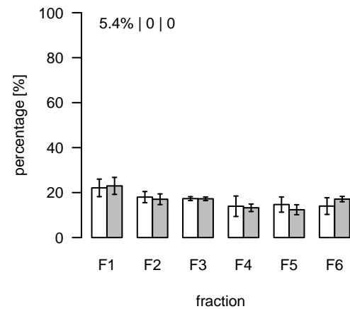
L1207 (m/z=777.588171; rt=6.69893) T/S Cluster: L-6.7-11
