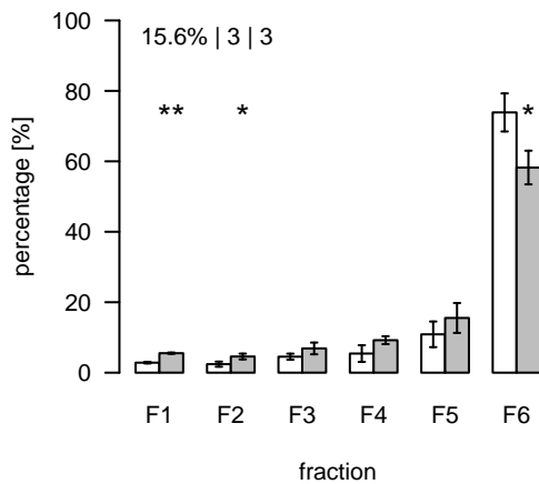
L244 (m/z=724.467471; rt=3.93953) T/S Cluster: L-3.9-7
