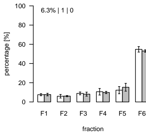
L1393 (m/z=909.506812; rt=7.5888) T/S Cluster: L-7.6-1
