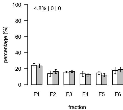
L90 (m/z=836.537757; rt=3.49571) T/S Cluster: L-3.5-7
