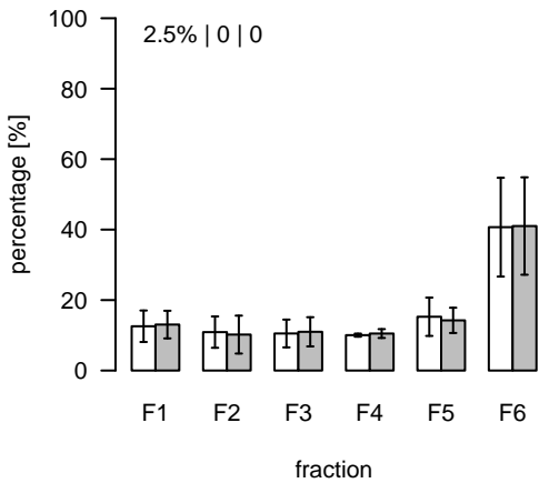
L143 (m/z=806.532826; rt=3.65303) T/S Cluster: L-3.7-6
