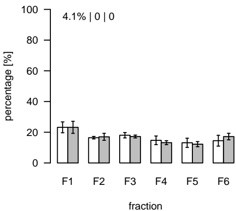
L1507 (m/z=151.311605; rt=7.94023) T/S Cluster: L-7.9-14
