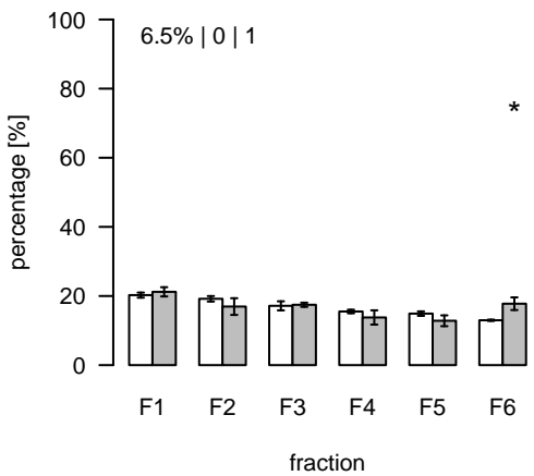
L2672 (m/z=921.317847; rt=15.84422) T/S Cluster: L-15.8-4
