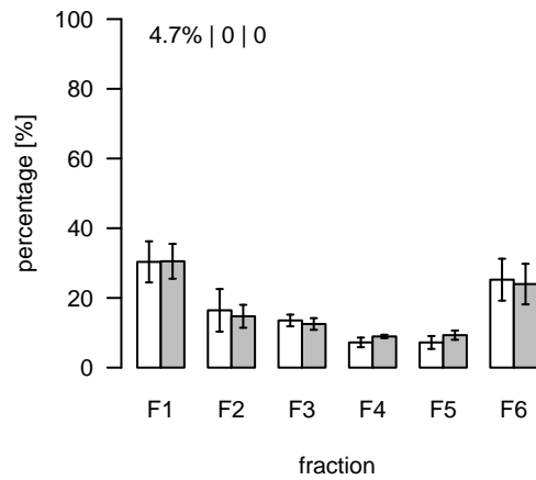
S202 (m/z=453.344711; rt=7.15643) T/S Cluster: S-7.2-1
