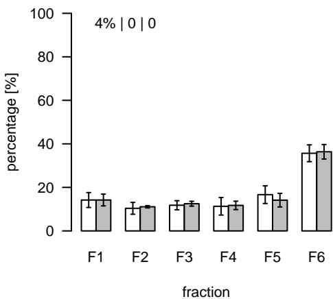
L97 (m/z=842.549188; rt=3.54747) T/S Cluster: L-3.5-8
