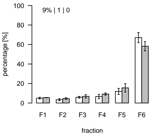
L773 (m/z=806.545904; rt=5.36047) T/S Cluster: L-5.4-2
