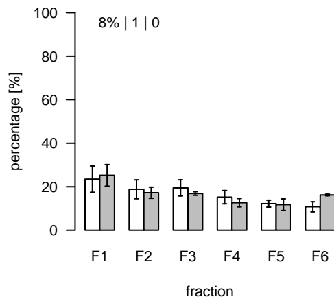
S21 (m/z=146.063461; rt=2.60719) T/S Cluster: S-2.6-1
