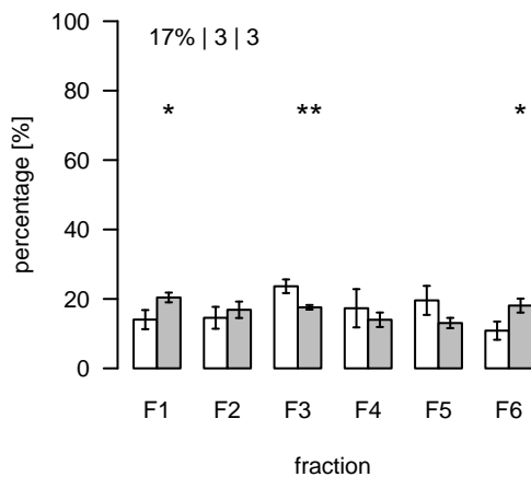
L1868 (m/z=930.51098; rt=9.43749) T/S Cluster: L-9.4-2
