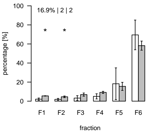
L2008 (m/z=910.544409; rt=10.09393) T/S Cluster: L-10.1-9
