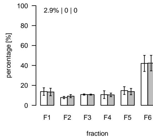
L914 (m/z=750.492831; rt=5.93789) T/S Cluster: L-5.9-4
