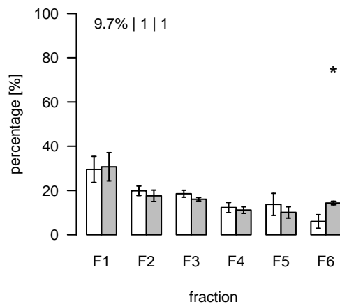
L1755 (m/z=392.298973; rt=8.8805) T/S Cluster: L-8.9-1
