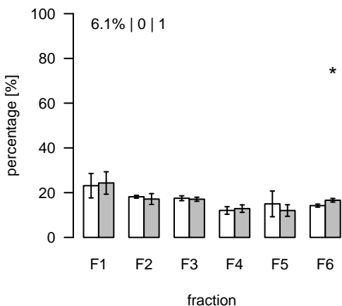
L2076 (m/z=938.67907; rt=10.48399) T/S Cluster: L-10.5-2
