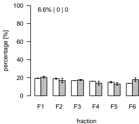
L2701 (m/z=996.303748; rt=16.15622) T/S Cluster: L-16.2-1
