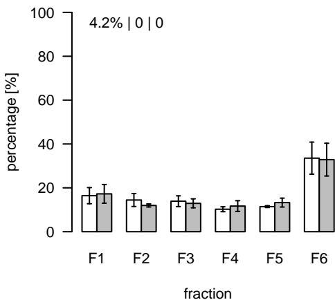
S637 (m/z=729.430537; rt=14.85201) T/S Cluster: S-14.9-1
