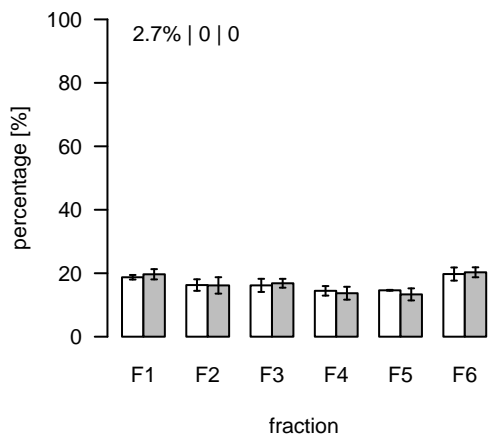
S482 (m/z=673.458431; rt=12.91163) T/S Cluster: S-12.9-13
