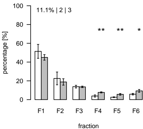
S649 (m/z=688.41805; rt=14.90257) T/S Cluster: S-14.9-2
