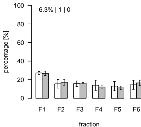
L1949 (m/z=380.794792; rt=9.65142) T/S Cluster: L-9.7-1
