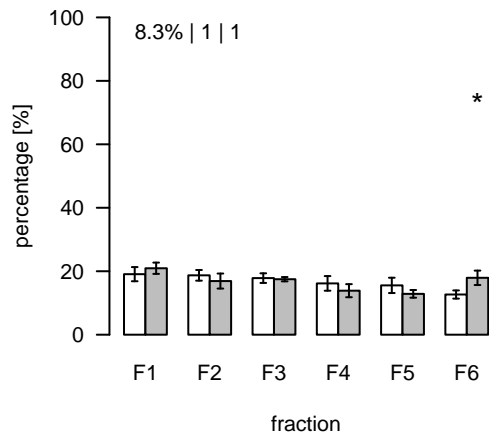
L2588 (m/z=782.725977; rt=15.38703) T/S Cluster: L-15.4-4
