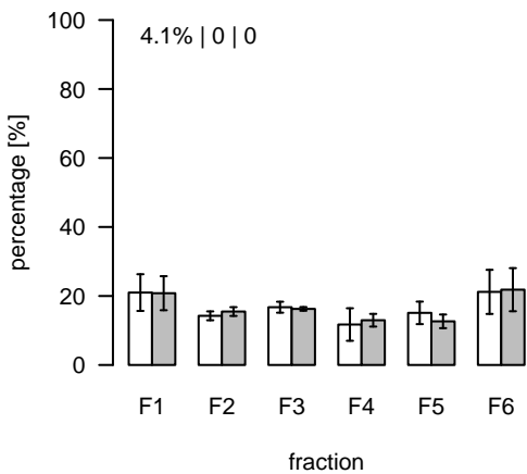
L1200 (m/z=259.84981; rt=6.66783) T/S Cluster: L-6.7-8
