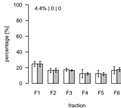
L784 (m/z=790.564333; rt=5.43042) T/S Cluster: L-5.4-5
