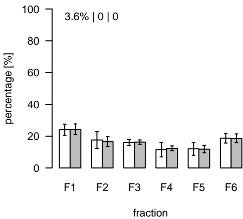
L945 (m/z=772.529948; rt=6.14147) T/S Cluster: L-6.1-6
