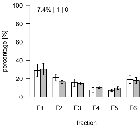
S721 (m/z=593.278104; rt=15.76523) T/S Cluster: S-15.8-2
