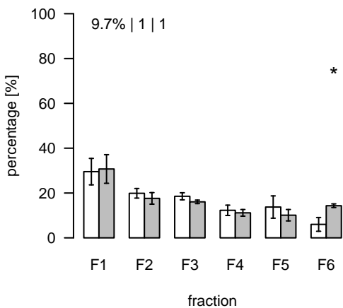
L1752 (m/z=392.292908; rt=8.88001) T/S Cluster: L-8.9-1
