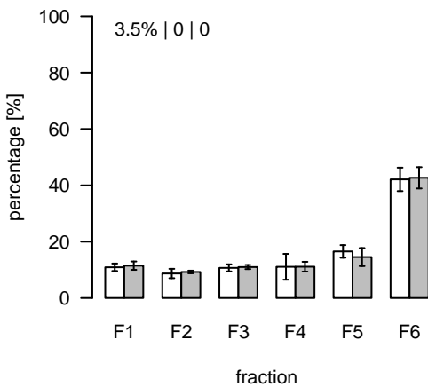
L1876 (m/z=938.628773; rt=9.52831) T/S Cluster: L-9.5-5
