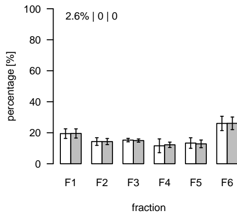
L970 (m/z=775.548871; rt=6.19013) T/S Cluster: L-6.2-5
