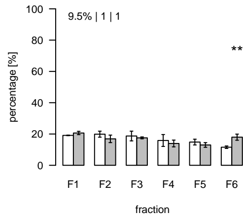
L2682 (m/z=865.808442; rt=15.94687) T/S Cluster: L-15.9-1
