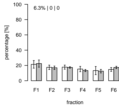
L1109 (m/z=801.587851; rt=6.58541) T/S Cluster: L-6.6-4
