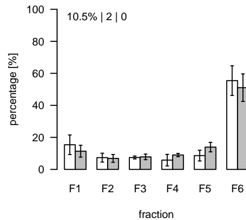
L586 (m/z=788.613377; rt=4.89771) T/S Cluster: L-4.9-4
