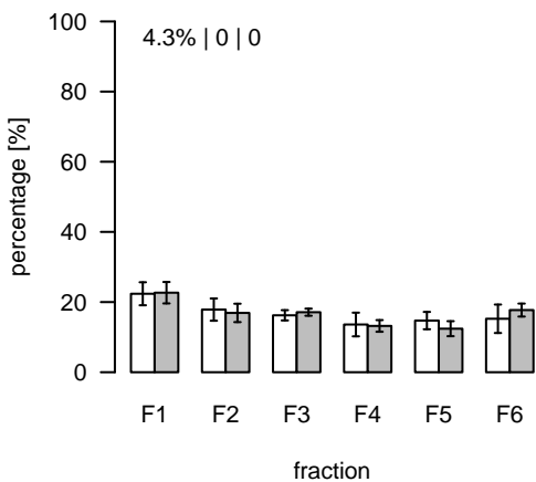
L786 (m/z=792.5734; rt=5.43054) T/S Cluster: L-5.4-7
