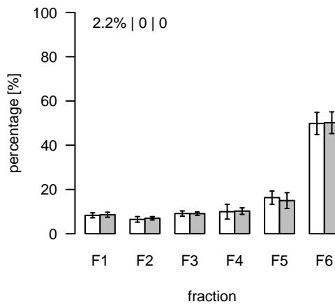
L1652 (m/z=935.655344; rt=8.64246) T/S Cluster: L-8.6-6
