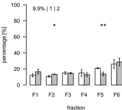
L1645 (m/z=939.608755; rt=8.63608) T/S Cluster: L-8.6-8
