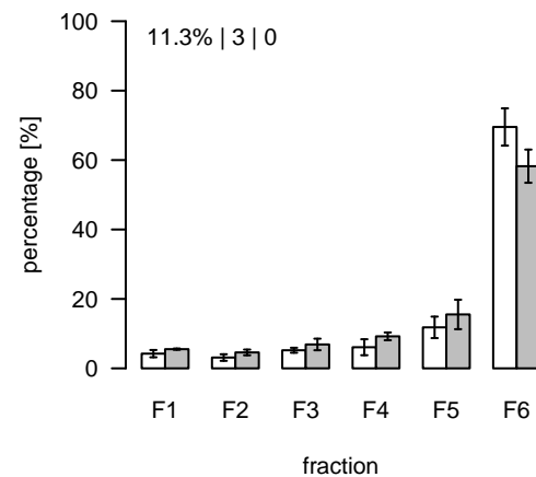
L1271 (m/z=767.553517; rt=7.18875) T/S Cluster: L-7.2-3
