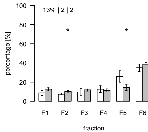
L618 (m/z=832.526833; rt=4.91642) T/S Cluster: L-4.9-16
