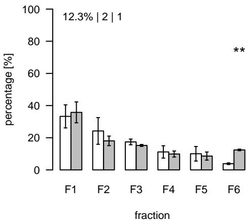
L158 (m/z=666.403687; rt=3.67489) T/S Cluster: L-3.7-14
