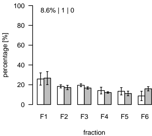
L1541 (m/z=804.553813; rt=8.05645) T/S Cluster: L-8.1-3
