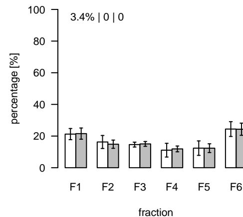
L480 (m/z=716.490424; rt=4.6594) T/S Cluster: L-4.7-1
