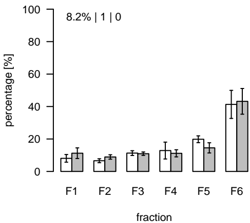
L1279 (m/z=771.509089; rt=7.18994) T/S Cluster: L-7.2-3
