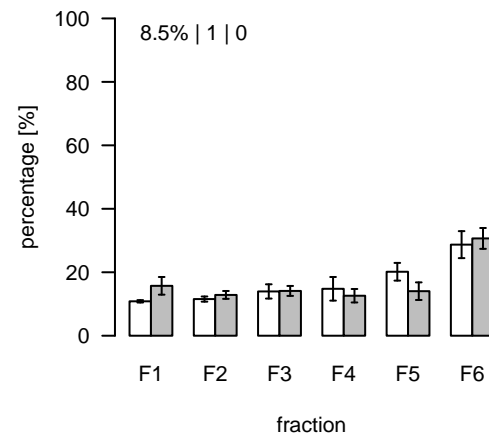
L926 (m/z=689.41694; rt=6.12405) T/S Cluster: L-6.1-3
