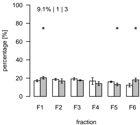
L2164 (m/z=864.65724; rt=10.62534) T/S Cluster: L-10.6-7
