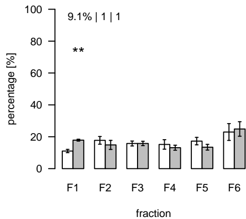
L2711 (m/z=528.152414; rt=16.1777) T/S Cluster: L-16.2-5
