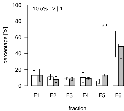
L1568 (m/z=925.495717; rt=8.11728) T/S Cluster: L-8.1-5
