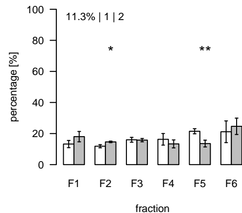
L1649 (m/z=939.567561; rt=8.64015) T/S Cluster: L-8.6-8
