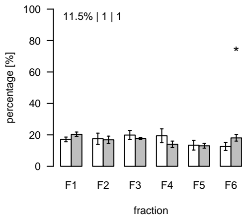
L2568 (m/z=898.788584; rt=15.33191) T/S Cluster: L-15.3-4
