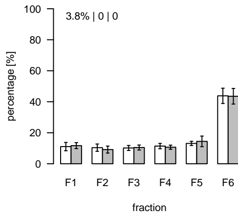
S410 (m/z=896.488146; rt=12.51678) T/S Cluster: S-12.5-5
