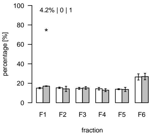
L2092 (m/z=897.55662; rt=10.50423) T/S Cluster: L-10.5-4
