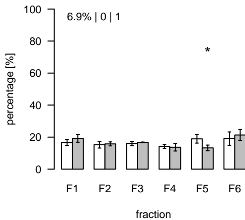
L2205 (m/z=565.568501; rt=10.95051) T/S Cluster: L-11-1
