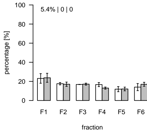
L1470 (m/z=758.606611; rt=7.93839) T/S Cluster: L-7.9-14
