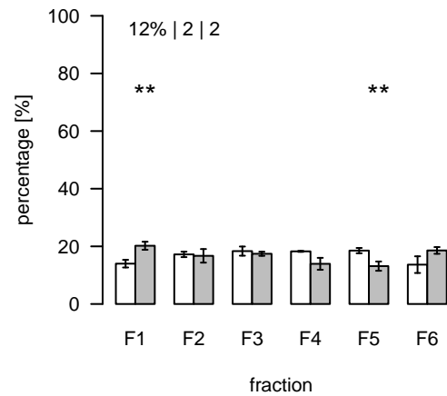
L2379 (m/z=726.466195; rt=11.32905) T/S Cluster: L-11.3-33
