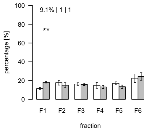
L2722 (m/z=1054.26999; rt=16.17899) T/S Cluster: L-16.2-5
