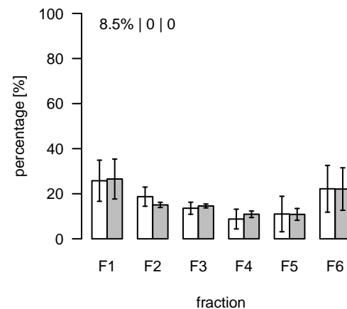
L1595 (m/z=740.542361; rt=8.24757) T/S Cluster: L-8.2-5
