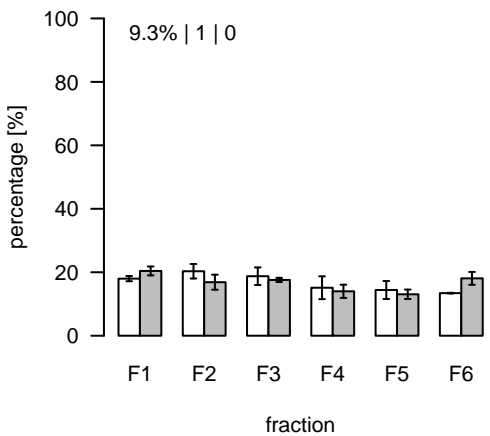
L2684 (m/z=890.819122; rt=15.95836) T/S Cluster: L-16-1
