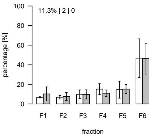
L1724 (m/z=911.551682; rt=8.72635) T/S Cluster: L-8.7-8
