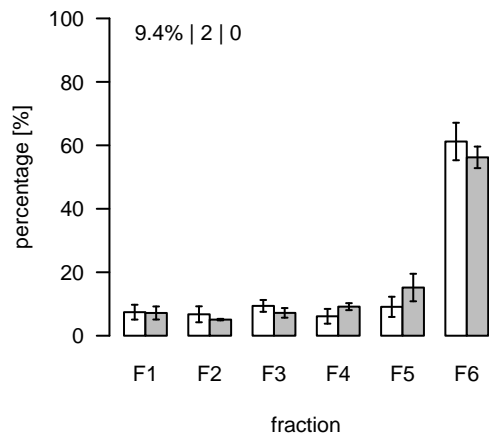
S818 (m/z=957.627932; rt=16.57017) T/S Cluster: S-16.6-2
