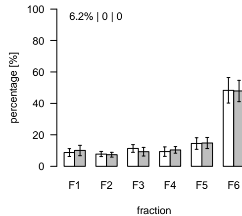
L2483 (m/z=872.580465; rt=12.38343) T/S Cluster: L-12.4-1
