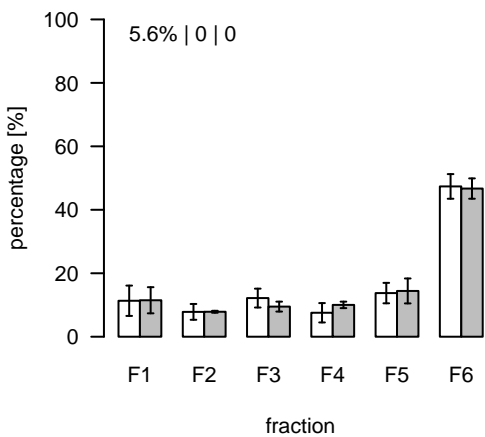
L1903 (m/z=886.561762; rt=9.57775) T/S Cluster: L-9.6-2
