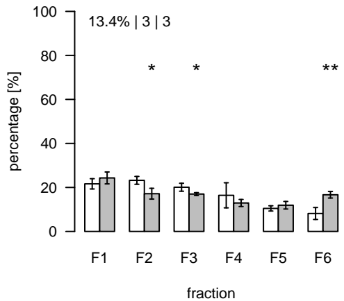
L2128 (m/z=931.50367; rt=10.51219) T/S Cluster: L-10.5-8
