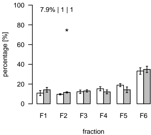
L1438 (m/z=935.587552; rt=7.89946) T/S Cluster: L-7.9-9
