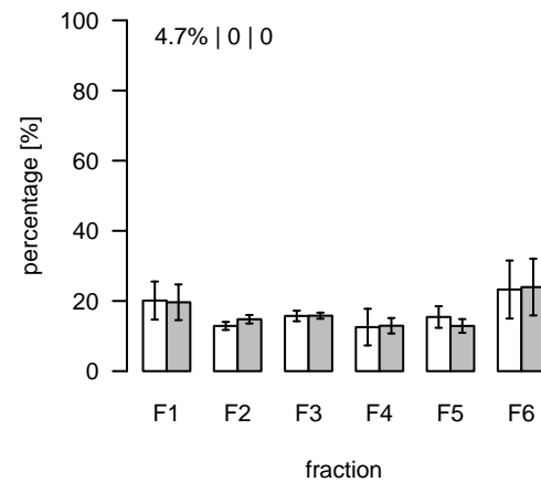
L1193 (m/z=259.518178; rt=6.66678) T/S Cluster: L-6.7-8
