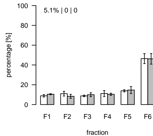
S415 (m/z=896.486887; rt=12.53737) T/S Cluster: S-12.5-5
