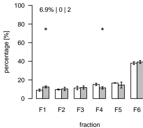
L708 (m/z=787.490463; rt=5.21379) T/S Cluster: L-5.2-4
