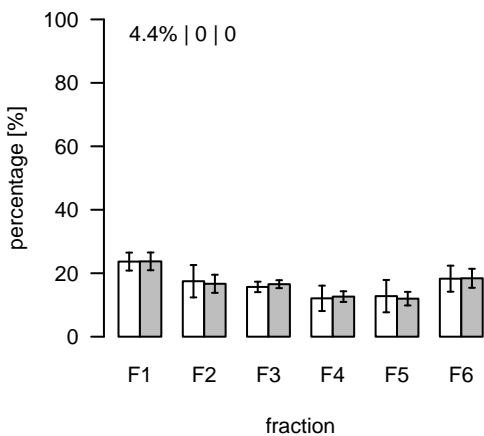
L1636 (m/z=732.559326; rt=8.60172) T/S Cluster: L-8.6-5
