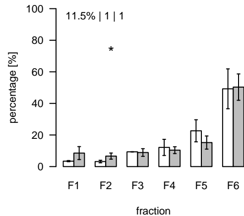
L2193 (m/z=896.551648; rt=10.91644) T/S Cluster: L-10.9-2
