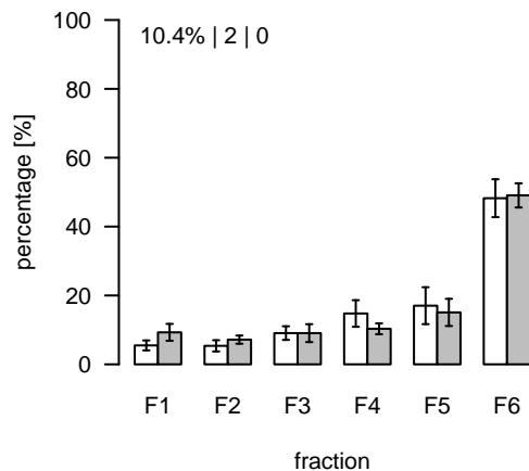
L1733 (m/z=448.26375; rt=8.74374) T/S Cluster: L-8.7-8
