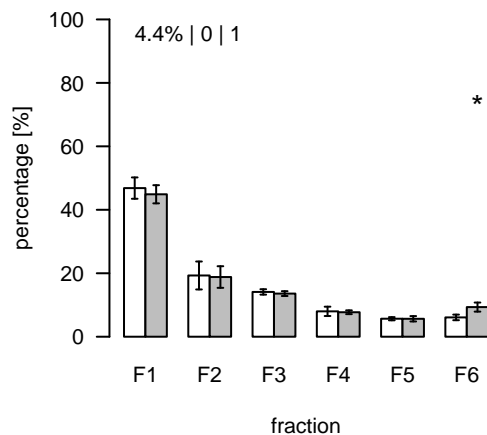
S102 (m/z=571.197514; rt=4.70733) T/S Cluster: S-4.7-1
