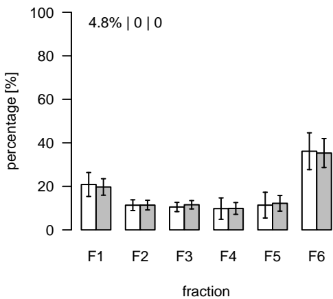
S268 (m/z=697.413224; rt=8.00757) T/S Cluster: S-8-2
