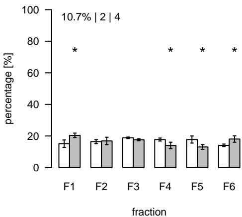
L1033 (m/z=385.248206; rt=6.54517) T/S Cluster: L-6.5-6
