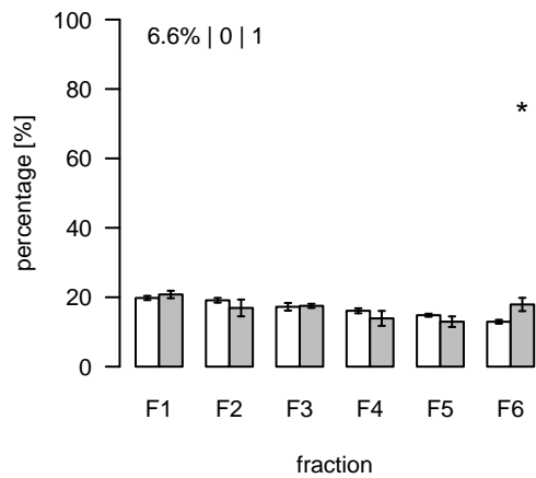
L2670 (m/z=922.318411; rt=15.84417) T/S Cluster: L-15.8-4
