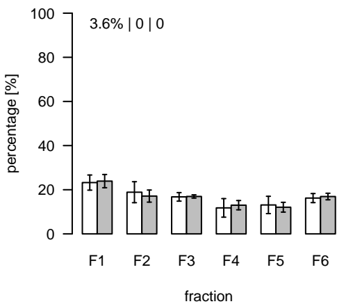
L390 (m/z=809.559042; rt=4.38898) T/S Cluster: L-4.4-9
