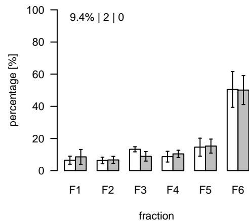
L1866 (m/z=908.589221; rt=9.43549) T/S Cluster: L-9.4-1
