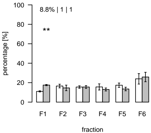
L2575 (m/z=911.259746; rt=15.36475) T/S Cluster: L-15.4-3
