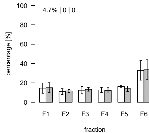
L330 (m/z=814.532546; rt=4.26275) T/S Cluster: L-4.3-3
