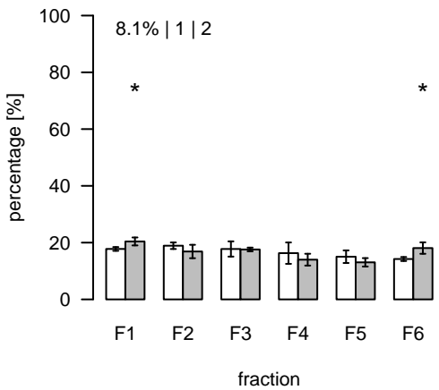
L2589 (m/z=808.741943; rt=15.43141) T/S Cluster: L-15.4-4
