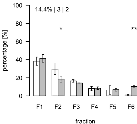
L1787 (m/z=716.50476; rt=8.91733) T/S Cluster: L-8.9-1
