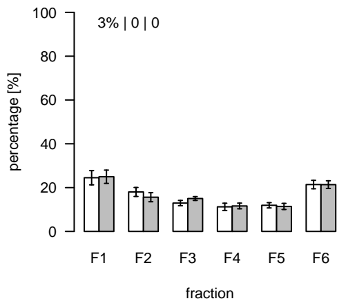
S552 (m/z=323.219716; rt=13.72196) T/S Cluster: S-13.7-1
