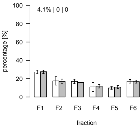
L1261 (m/z=734.571623; rt=7.16406) T/S Cluster: L-7.2-1
