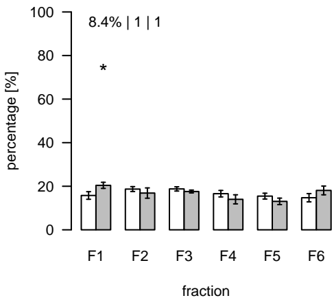
L2804 (m/z=1191.127696; rt=18.41561) T/S Cluster: L-18.4-2
