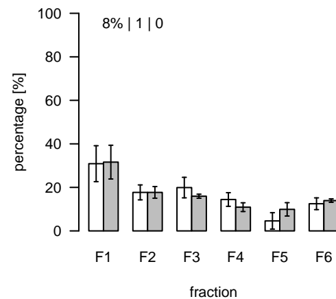
L118 (m/z=690.463634; rt=3.61108) T/S Cluster: L-3.6-6
