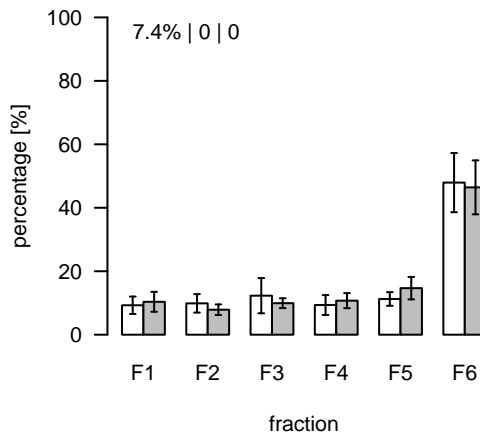
S632 (m/z=843.517811; rt=14.8138) T/S Cluster: S-14.8-8
