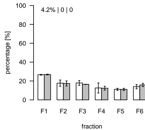
L2516 (m/z=900.753482; rt=13.7002) T/S Cluster: L-13.7-2
