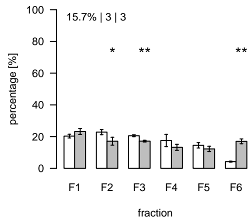
L2084 (m/z=915.512351; rt=10.49928) T/S Cluster: L-10.5-8
