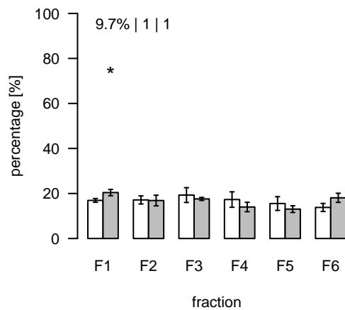
L2657 (m/z=902.799423; rt=15.83166) T/S Cluster: L-15.8-3
