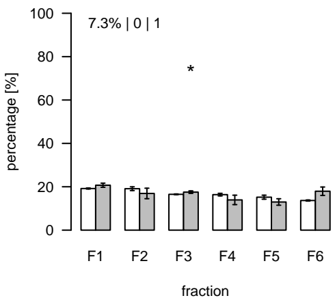
L2692 (m/z=498.668636; rt=16.15467) T/S Cluster: L-16.2-1
