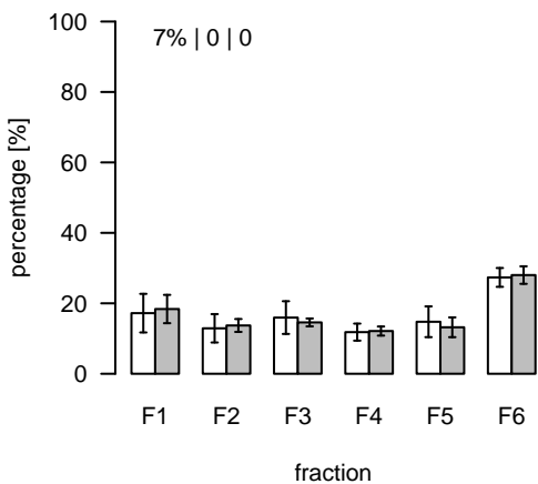
L1759 (m/z=887.573742; rt=8.91291) T/S Cluster: L-8.9-4
