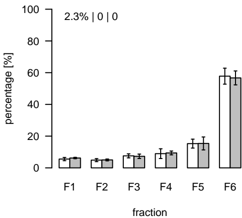
L578 (m/z=971.619572; rt=4.89653) T/S Cluster: L-4.9-9
