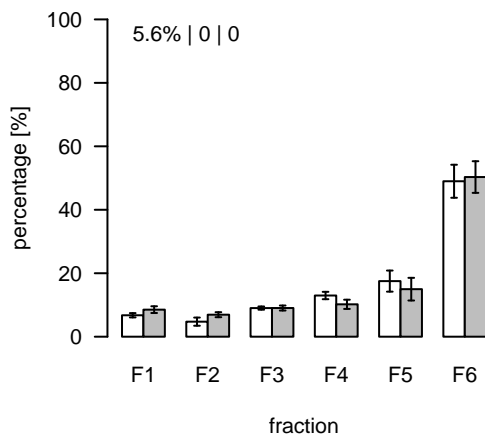
L771 (m/z=811.5569; rt=5.34466) T/S Cluster: L-5.3-5
