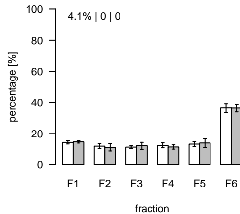
L2466 (m/z=290.530423; rt=11.84911) T/S Cluster: L-11.8-5
