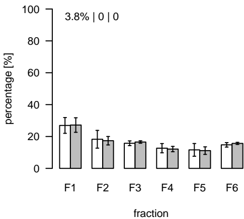
L87 (m/z=680.452926; rt=3.48321) T/S Cluster: L-3.5-6
