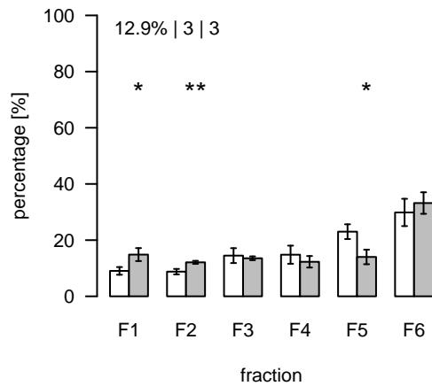
L510 (m/z=786.507196; rt=4.78247) T/S Cluster: L-4.8-3
