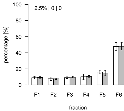
L493 (m/z=892.57477; rt=4.74184) T/S Cluster: L-4.7-8
