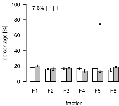
S431 (m/z=421.257169; rt=12.55213) T/S Cluster: S-12.6-8
