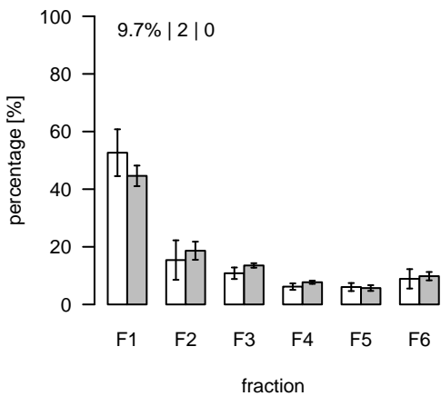
S65 (m/z=1208.336651; rt=4.68743) T/S Cluster: S-4.7-1
