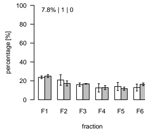
L958 (m/z=790.564346; rt=6.15282) T/S Cluster: L-6.2-2
