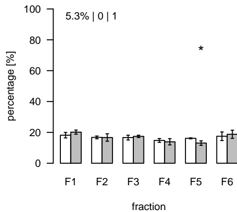
S245 (m/z=239.042175; rt=7.40468) T/S Cluster: S-7.4-1
