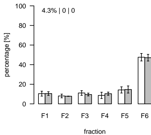
L1901 (m/z=885.527552; rt=9.57692) T/S Cluster: L-9.6-2
