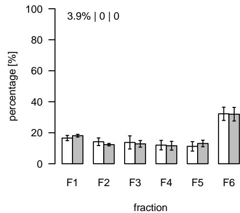
S610 (m/z=810.515164; rt=14.6549) T/S Cluster: S-14.7-2
