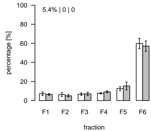
L382 (m/z=824.556741; rt=4.38466) T/S Cluster: L-4.4-2
