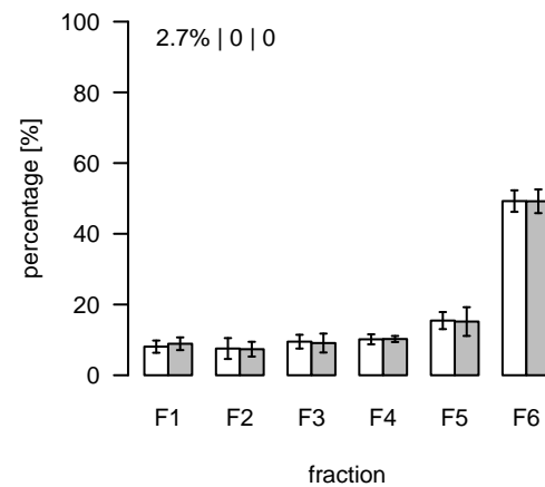
L264 (m/z=978.6078; rt=4.00658) T/S Cluster: L-4-2
