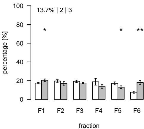
L1789 (m/z=930.511793; rt=8.91748) T/S Cluster: L-8.9-9
