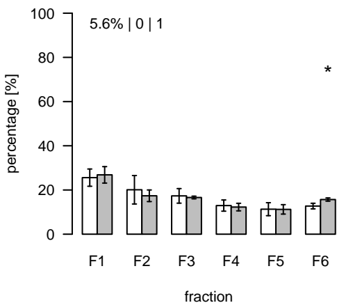
L626 (m/z=787.538077; rt=4.93435) T/S Cluster: L-4.9-18
