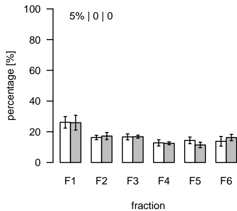
L1037 (m/z=793.558529; rt=6.54572) T/S Cluster: L-6.5-5
