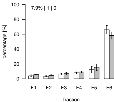
L640 (m/z=782.535505; rt=4.95227) T/S Cluster: L-5-1
