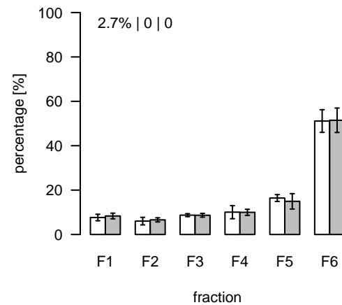
L1461 (m/z=769.53583; rt=7.91783) T/S Cluster: L-7.9-9
