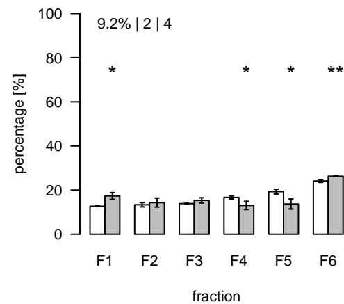
L2317 (m/z=722.514378; rt=11.32823) T/S Cluster: L-11.3-19
