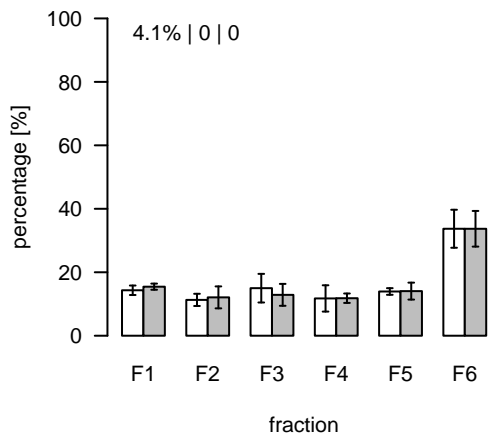
S389 (m/z=894.489496; rt=12.32224) T/S Cluster: S-12.3-5
