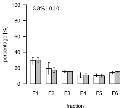
L1012 (m/z=812.546212; rt=6.42238) T/S Cluster: L-6.4-3
