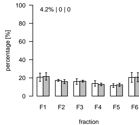
L703 (m/z=812.552043; rt=5.19169) T/S Cluster: L-5.2-2
