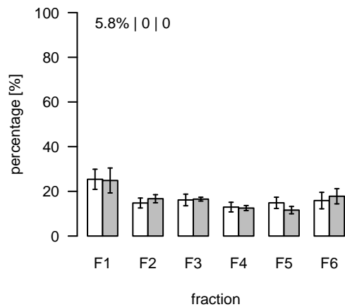
L1054 (m/z=792.56931; rt=6.54743) T/S Cluster: L-6.5-5
