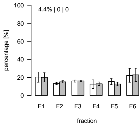
L1199 (m/z=389.771084; rt=6.66741) T/S Cluster: L-6.7-8
