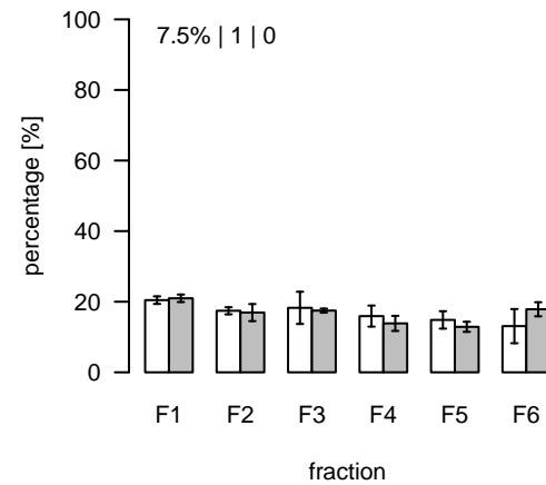
L966 (m/z=797.535445; rt=6.18961) T/S Cluster: L-6.2-8
