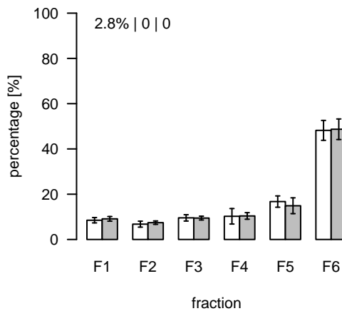
L1651 (m/z=936.623615; rt=8.64135) T/S Cluster: L-8.6-6
