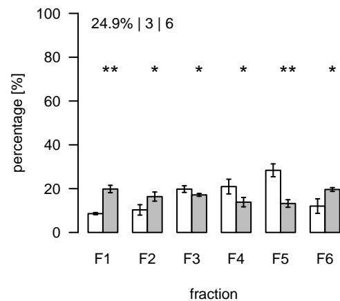
L2186 (m/z=915.537338; rt=10.91521) T/S Cluster: L-10.9-1
