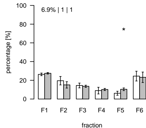
L1936 (m/z=798.582547; rt=9.61291) T/S Cluster: L-9.6-4
