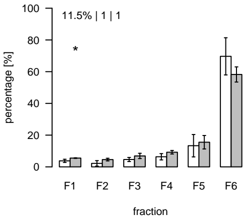
L1609 (m/z=940.576795; rt=8.42258) T/S Cluster: L-8.4-4
