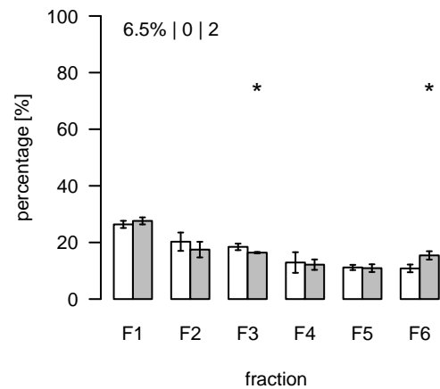
L2136 (m/z=816.662962; rt=10.58508) T/S Cluster: L-10.6-2
