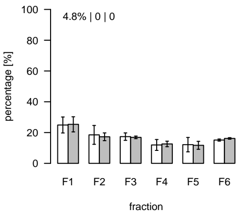
L125 (m/z=639.45025; rt=3.61718) T/S Cluster: L-3.6-7
