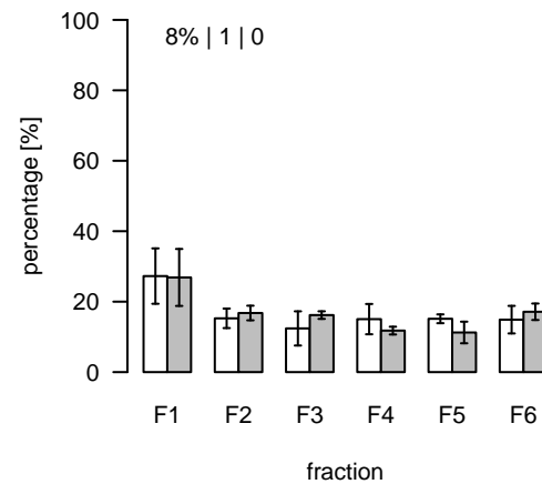
S17 (m/z=231.116489; rt=1.62613) T/S Cluster: S-1.6-2
