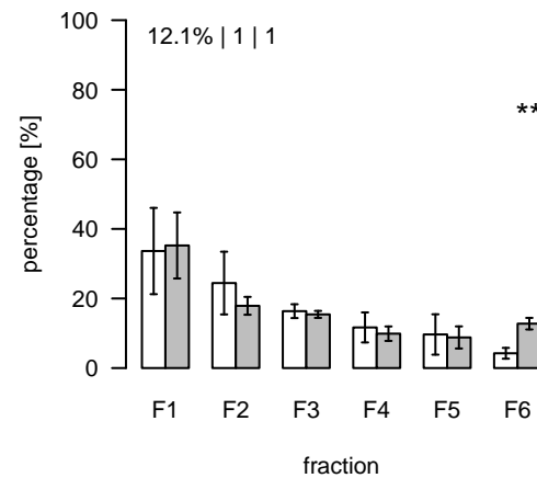
L47 (m/z=722.466054; rt=3.2742) T/S Cluster: L-3.3-5
