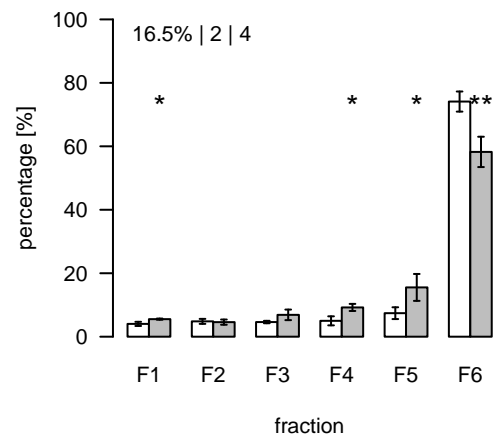
L1979 (m/z=909.532741; rt=9.89855) T/S Cluster: L-9.9-2
