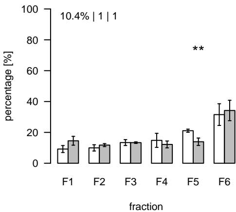
L642 (m/z=785.484747; rt=4.9527) T/S Cluster: L-5-2
