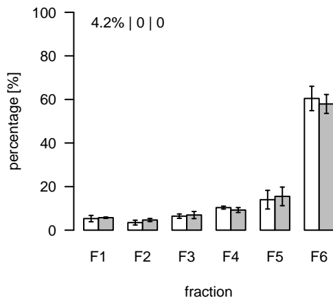
L547 (m/z=778.455723; rt=4.83541) T/S Cluster: L-4.8-10
