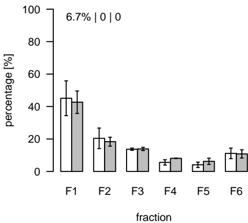
S681 (m/z=637.429858; rt=15.19777) T/S Cluster: S-15.2-1
