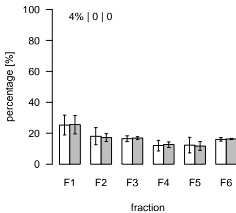
L122 (m/z=319.221655; rt=3.61677) T/S Cluster: L-3.6-7
