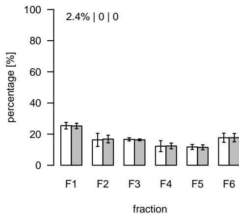
L1256 (m/z=749.592436; rt=7.16143) T/S Cluster: L-7.2-1
