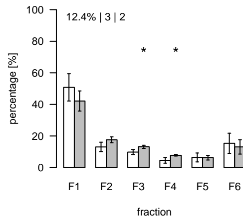
S573 (m/z=760.427233; rt=14.30653) T/S Cluster: S-14.3-1
