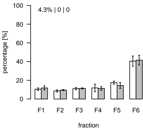
L1441 (m/z=466.817917; rt=7.90291) T/S Cluster: L-7.9-9
