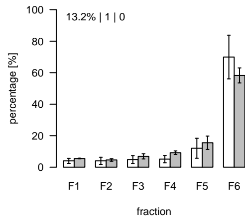
L1739 (m/z=891.532698; rt=8.81155) T/S Cluster: L-8.8-2
