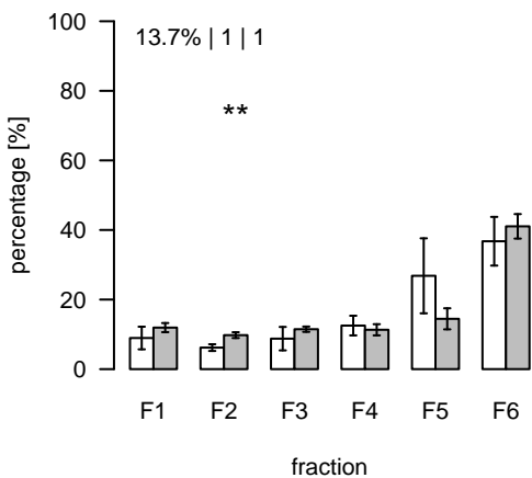
L1292 (m/z=836.55925; rt=7.27801) T/S Cluster: L-7.3-2
