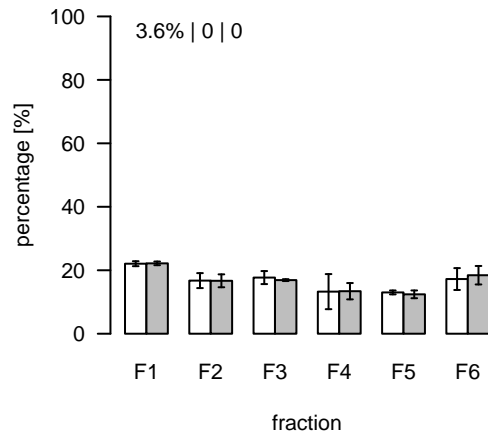
L2145 (m/z=680.621903; rt=10.612) T/S Cluster: L-10.6-4
