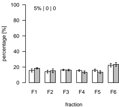
L1791 (m/z=454.773921; rt=8.91767) T/S Cluster: L-8.9-5
