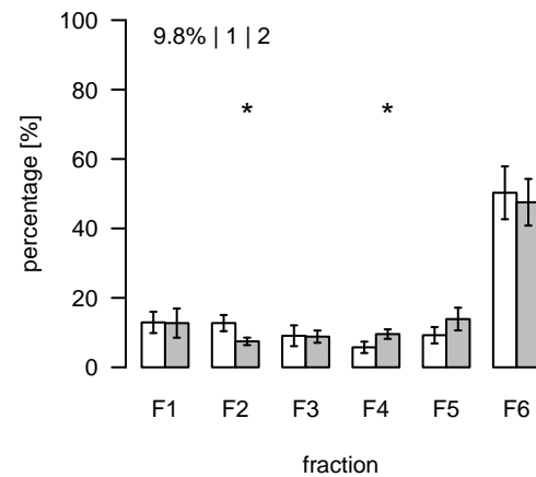
S869 (m/z=741.476035; rt=16.9814) T/S Cluster: S-17-5
