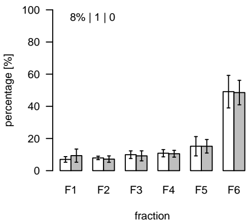
L1981 (m/z=904.570303; rt=9.97411) T/S Cluster: L-10-2
