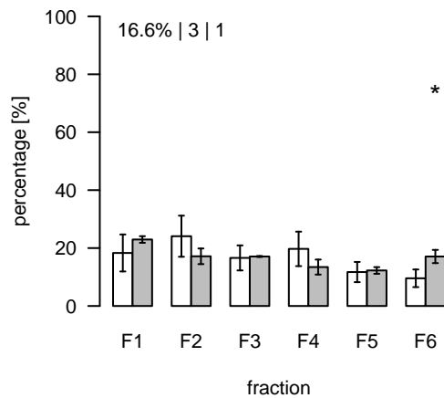
L2473 (m/z=894.543346; rt=11.85683) T/S Cluster: L-11.9-2
