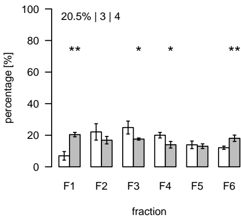
S870 (m/z=766.564039; rt=16.98173) T/S Cluster: S-17-8
