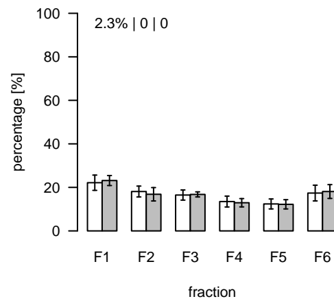
L789 (m/z=394.274074; rt=5.4369) T/S Cluster: L-5.4-9
