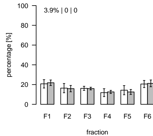
L297 (m/z=806.5586; rt=4.15123) T/S Cluster: L-4.2-2
