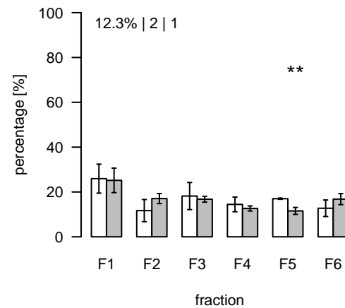
L2530 (m/z=761.224584; rt=14.06408) T/S Cluster: L-14.1-1
