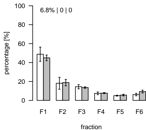
S89 ( m/z=1038.275955 ; rt=4.70375 ) T/S Cluster: S-4.7-1
