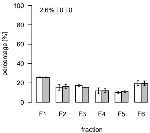
L2511 (m/z=874.728608; rt=12.7885) T/S Cluster: L-12.8-2
