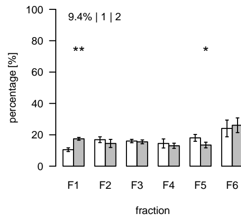
L2586 (m/z=907.227608; rt=15.36564) T/S Cluster: L-15.4-3
