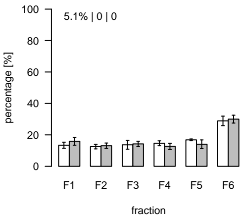
L1118 (m/z=953.659222; rt=6.61367) T/S Cluster: L-6.6-11
