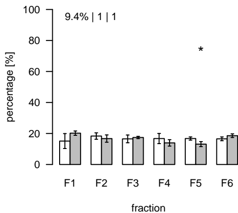
S806 (m/z=437.776845; rt=16.52788) T/S Cluster: S-16.5-9
