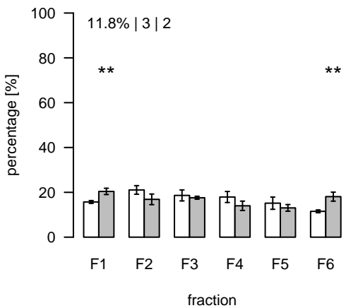
L2567 (m/z=821.745666; rt=15.32287) T/S Cluster: L-15.3-3
