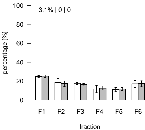
L1225 (m/z=775.572513; rt=6.79827) T/S Cluster: L-6.8-2
