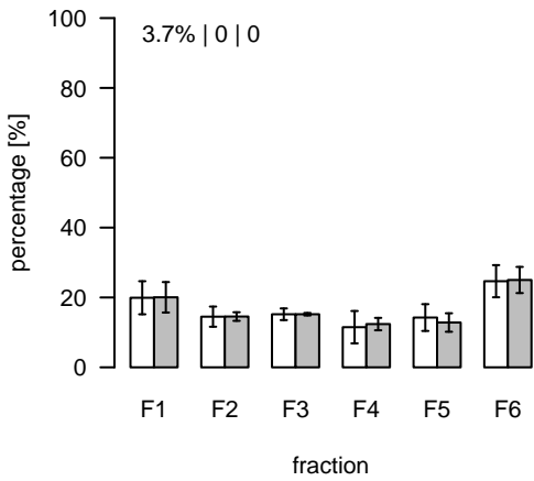
L504 (m/z=716.490613; rt=4.75652) T/S Cluster: L-4.8-2
