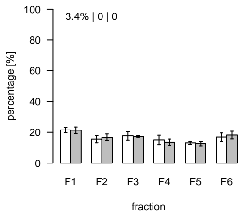
L2148 (m/z=422.342082; rt=10.61227) T/S Cluster: L-10.6-4
