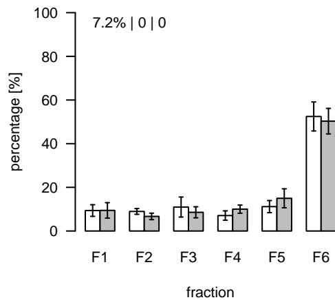
L2 (m/z=433.238775; rt=1.36419) T/S Cluster: L-1.4-1
