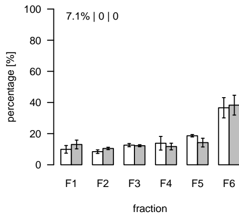
L1159 (m/z=955.624378; rt=6.65422) T/S Cluster: L-6.7-3
