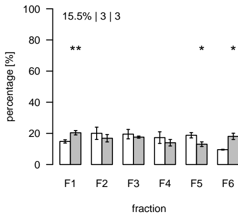
L1664 (m/z=388.344284; rt=8.68742) T/S Cluster: L-8.7-2
