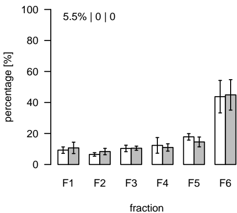
L1098 (m/z=382.748376; rt=6.54819) T/S Cluster: L-6.5-1
