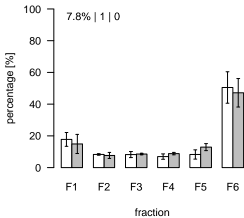
S832 (m/z=765.538344; rt=16.57432) T/S Cluster: S-16.6-1
