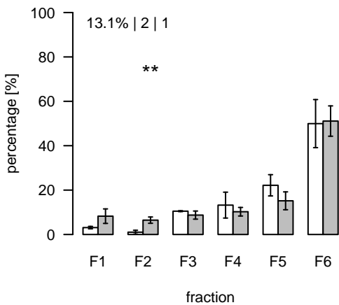
L2191 (m/z=895.617553; rt=10.91627) T/S Cluster: L-10.9-2
