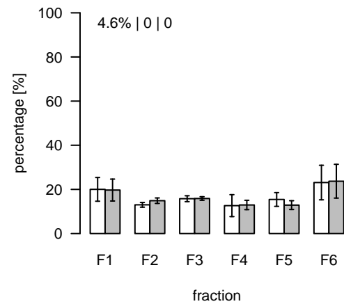
L1192 (m/z=778.543084; rt=6.66672) T/S Cluster: L-6.7-8
