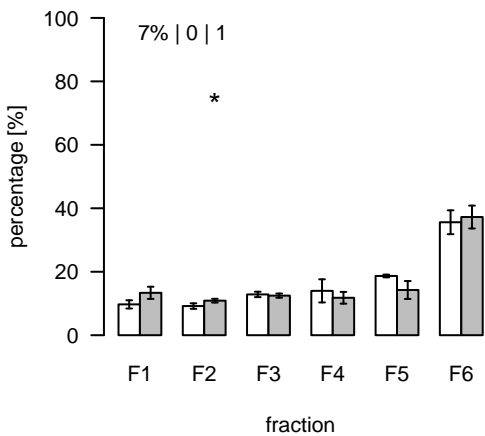
L1149 (m/z=318.539822; rt=6.65397) T/S Cluster: L-6.7-3
