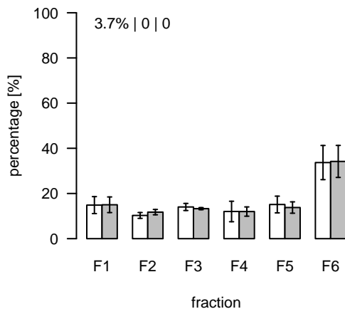
L592 (m/z=795.543285; rt=4.90003) T/S Cluster: L-4.9-10
