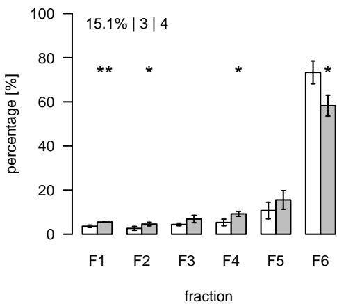
L339 (m/z=796.524292; rt=4.27783) T/S Cluster: L-4.3-1
