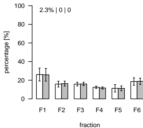
L1825 (m/z=392.292751; rt=9.06091) T/S Cluster: L-9.1-1
