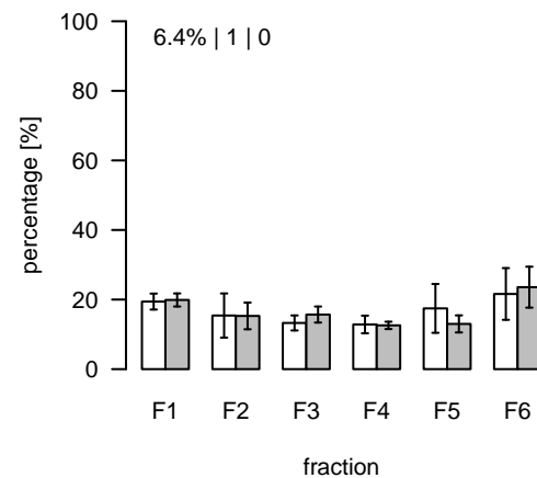
L287 (m/z=325.723394; rt=4.09595) T/S Cluster: L-4.1-2
