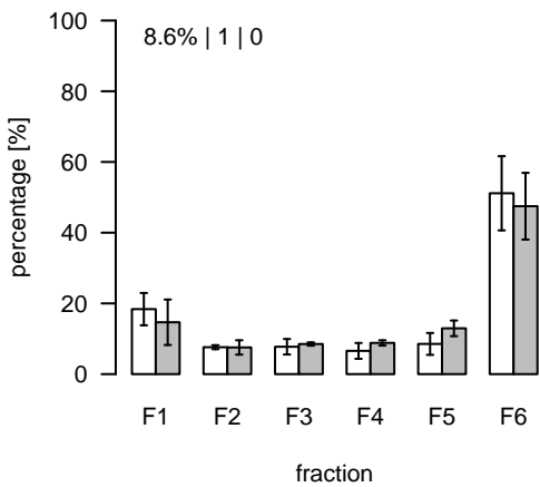
S828 (m/z=382.774091; rt=16.57421) T/S Cluster: S-16.6-1
