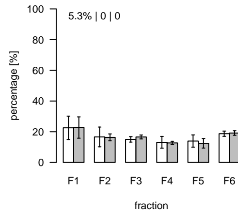
L277 (m/z=662.44363; rt=4.07434) T/S Cluster: L-4.1-2
