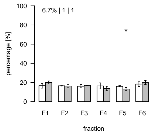
S384 (m/z=331.148217; rt=12.25789) T/S Cluster: S-12.3-1
