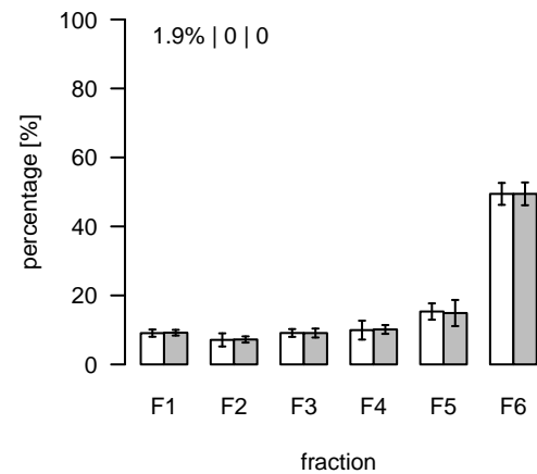
L1855 (m/z=911.654746; rt=9.34441) T/S Cluster: L-9.3-6
