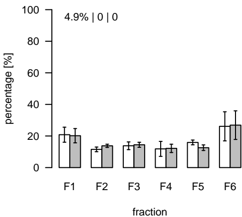
L1361 (m/z=820.602716; rt=7.35213) T/S Cluster: L-7.4-2
