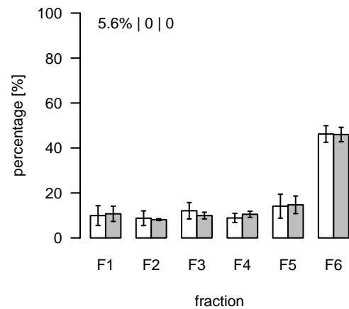
L2219 (m/z=885.525981; rt=11.02765) T/S Cluster: L-11-2
