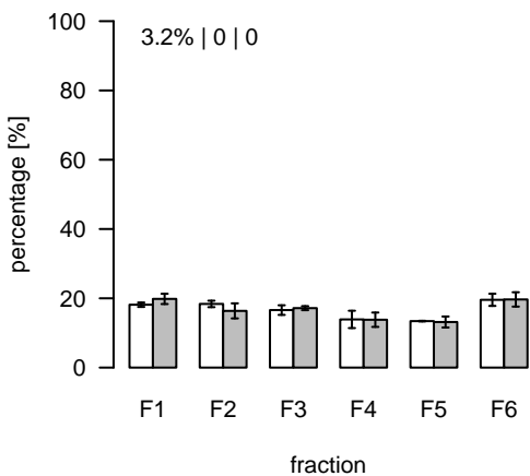
S543 (m/z=597.483554; rt=13.64733) T/S Cluster: S-13.6-6
