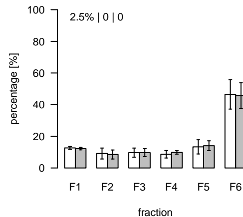
L22 (m/z=688.425974; rt=2.74915) T/S Cluster: L-2.7-3
