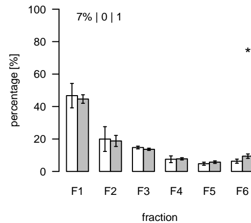
S137 (m/z=433.10254; rt=5.70226) T/S Cluster: S-5.7-1
