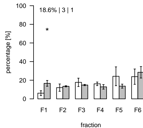
L2410 (m/z=680.482781; rt=11.5809) T/S Cluster: L-11.6-1
