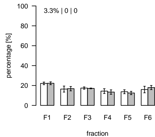
L2142 (m/z=861.709267; rt=10.61043) T/S Cluster: L-10.6-5
