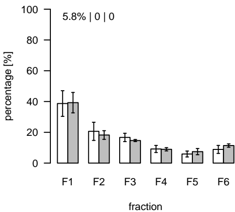
S196 (m/z=595.167925; rt=6.90063) T/S Cluster: S-6.9-2
