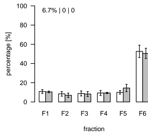
L1628 (m/z=904.572552; rt=8.55178) T/S Cluster: L-8.6-1
