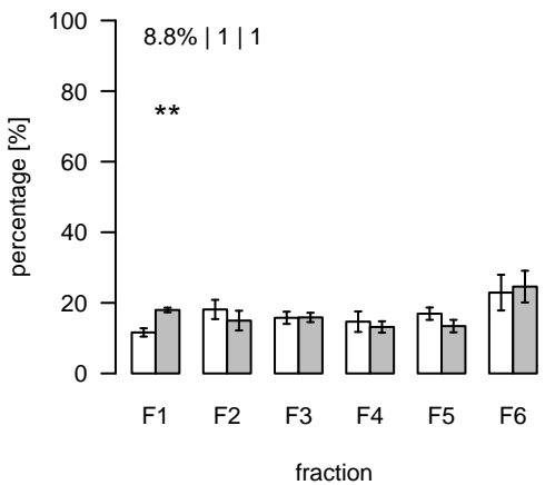
L2710 (m/z=527.653239; rt=16.17764) T/S Cluster: L-16.2-5
