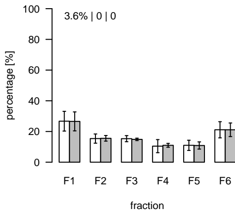
L1821 (m/z=785.594111; rt=9.06051) T/S Cluster: L-9.1-1
