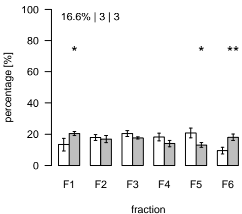
L2265 (m/z=1399.00331; rt=11.32772) T/S Cluster: L-11.3-4
