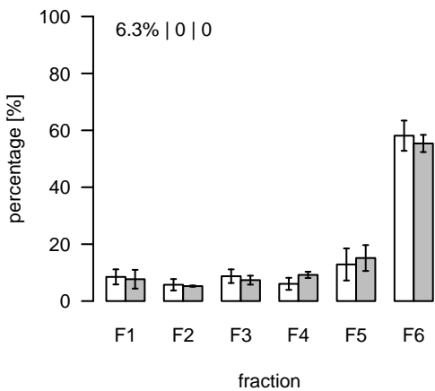
L107 (m/z=594.274306; rt=3.57068) T/S Cluster: L-3.6-2
