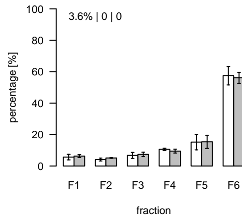
L533 (m/z=583.439282; rt=4.81096) T/S Cluster: L-4.8-10
