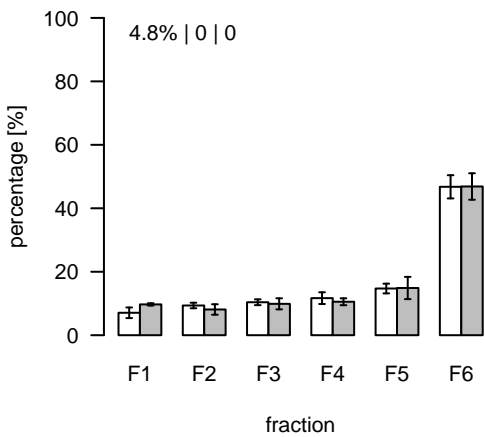
L796 (m/z=569.434411; rt=5.51201) T/S Cluster: L-5.5-2
