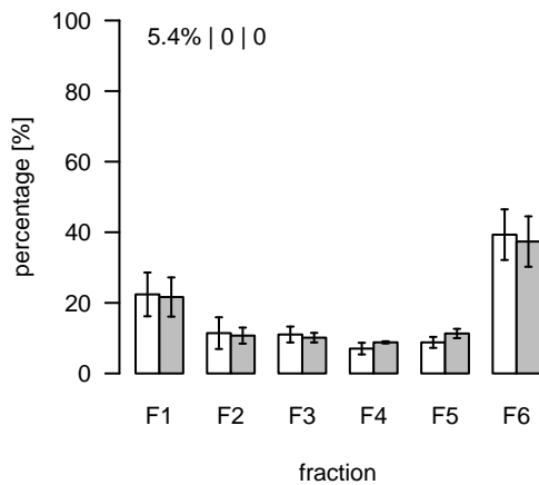
S299 (m/z=584.293593; rt=9.40551) T/S Cluster: S-9.4-1
