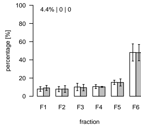
L365 (m/z=984.598244; rt=4.34507) T/S Cluster: L-4.3-14
