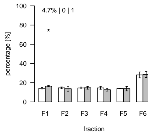
L2111 (m/z=895.496217; rt=10.50494) T/S Cluster: L-10.5-13
