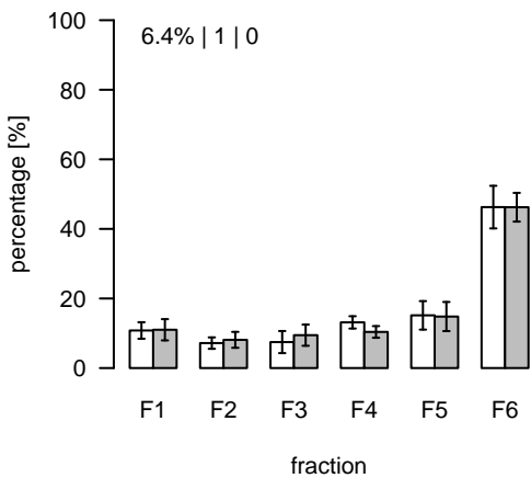
L356 (m/z=841.474169; rt=4.29828) T/S Cluster: L-4.3-13
