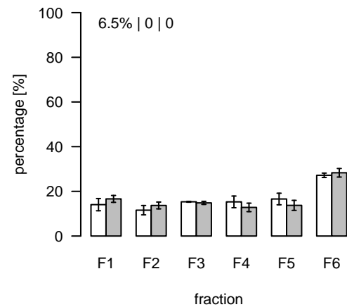
L1770 (m/z=303.183901; rt=8.91483) T/S Cluster: L-8.9-5
