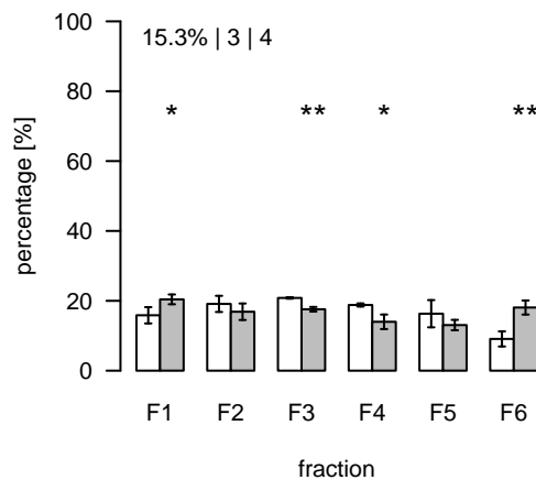
L1177 (m/z=959.582032; rt=6.66037) T/S Cluster: L-6.7-6
