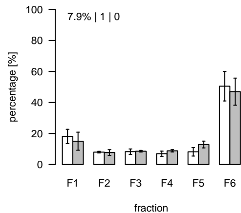
S837 (m/z=764.533664; rt=16.57449) T/S Cluster: S-16.6-1
