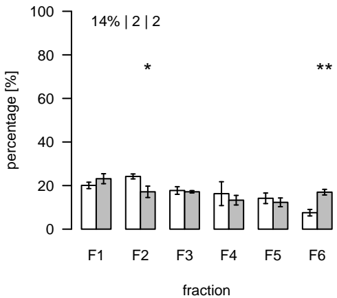
L2127 (m/z=1091.731047; rt=10.5106) T/S Cluster: L-10.5-8
