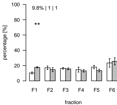
L2580 (m/z=909.269026; rt=15.36525) T/S Cluster: L-15.4-3
