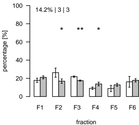
S805 (m/z=313.274143; rt=16.51683) T/S Cluster: S-16.5-8
