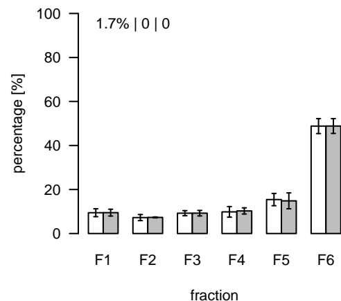
L1888 (m/z=312.229203; rt=9.53035) T/S Cluster: L-9.5-5
