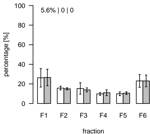
S767 (m/z=304.151404; rt=16.21574) T/S Cluster: S-16.2-5
