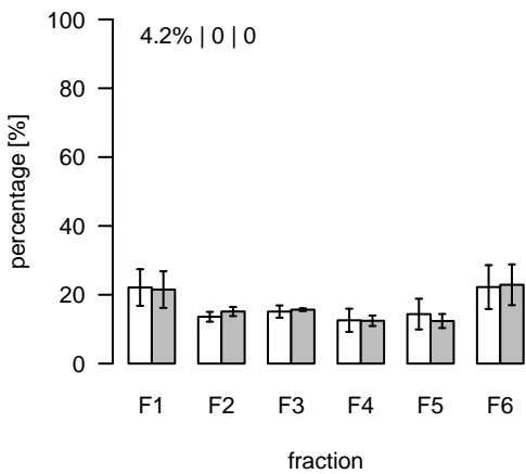
L1550 (m/z=391.273037; rt=8.05672) T/S Cluster: L-8.1-2
