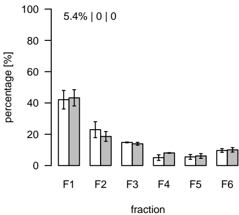
S612 (m/z=738.457985; rt=14.66602) T/S Cluster: S-14.7-3
