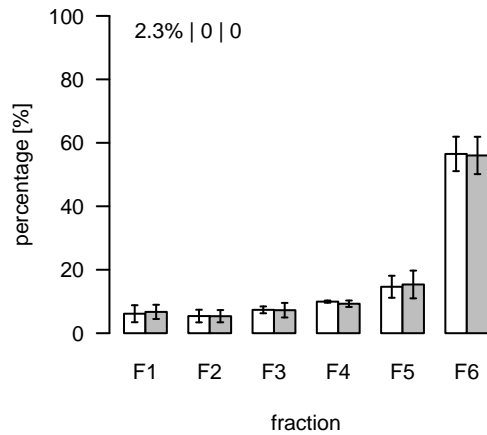
L396 (m/z=980.625636; rt=4.39259) T/S Cluster: L-4.4-2
