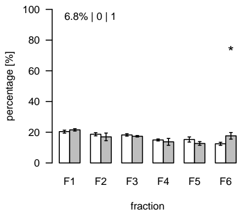
L2664 (m/z=926.312827; rt=15.84248) T/S Cluster: L-15.8-4
