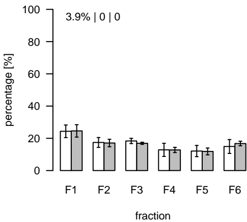
L782 (m/z=791.549627; rt=5.42587) T/S Cluster: L-5.4-5
