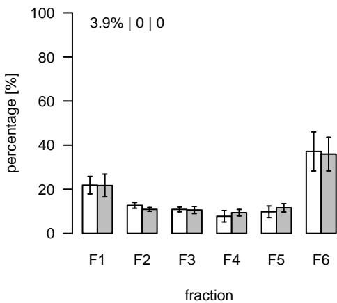
S580 (m/z=481.353719; rt=14.34939) T/S Cluster: S-14.3-4
