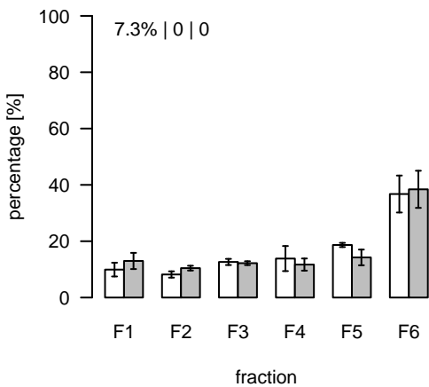
L1166 (m/z=318.212707; rt=6.65429) T/S Cluster: L-6.7-3
