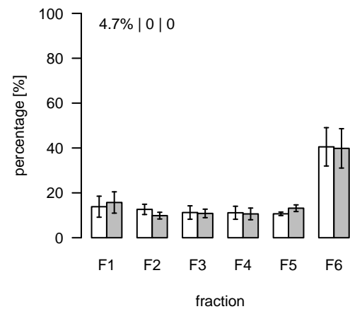
S747 (m/z=848.52352; rt=15.9723) T/S Cluster: S-16-3
