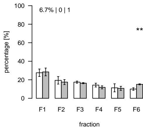
L1928 (m/z=380.7844; rt=9.59738) T/S Cluster: L-9.6-3
