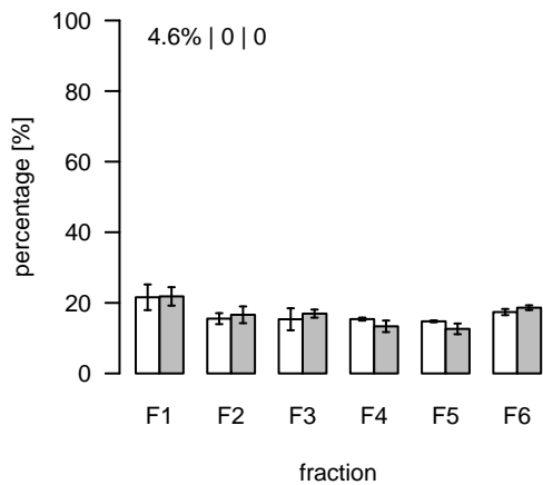
S191 (m/z=617.150093; rt=6.5895) T/S Cluster: S-6.6-5
