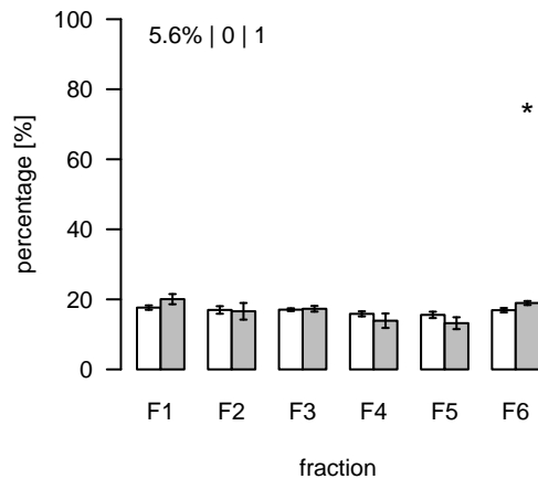
S463 (m/z=263.11771; rt=12.86912) T/S Cluster: S-12.9-2
