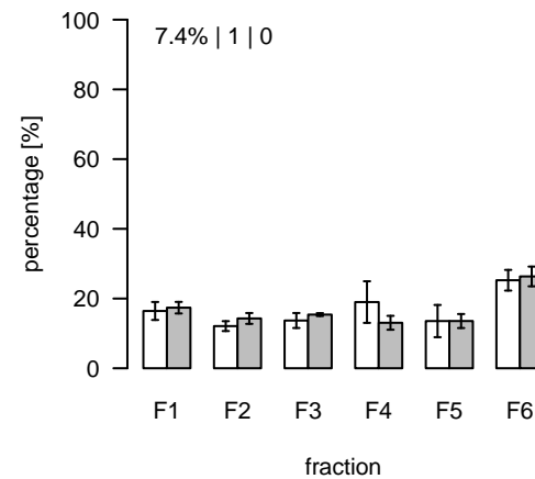
L405 (m/z=804.547476; rt=4.42583) T/S Cluster: L-4.4-1
