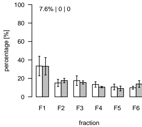
S161 (m/z=428.20523; rt=6.18741) T/S Cluster: S-6.2-1
