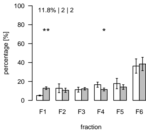
L2240 (m/z=610.187215; rt=11.32321) T/S Cluster: L-11.3-9
