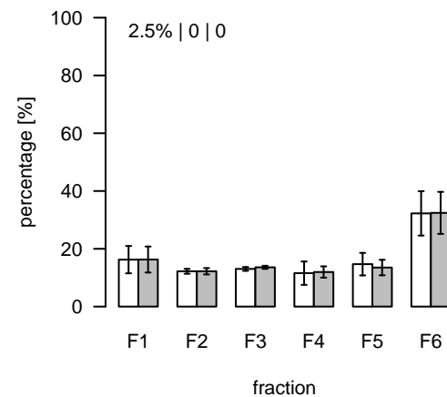
L731 (m/z=797.531631; rt=5.28682) T/S Cluster: L-5.3-1
