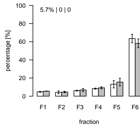
L128 (m/z=1002.610012; rt=3.62033) T/S Cluster: L-3.6-5
