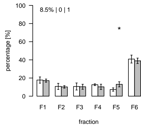
S666 (m/z=808.49999; rt=14.94961) T/S Cluster: S-14.9-6
