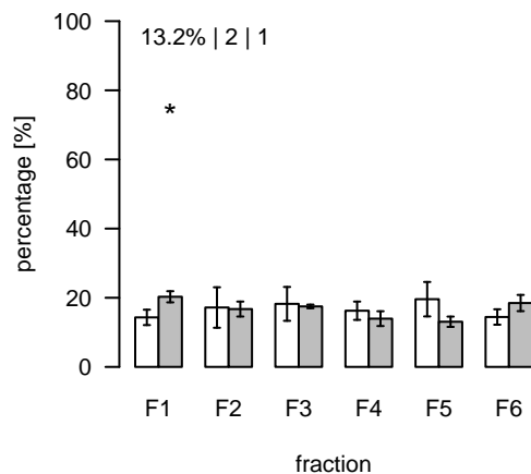
L851 (m/z=389.34674; rt=5.71319) T/S Cluster: L-5.7-11
