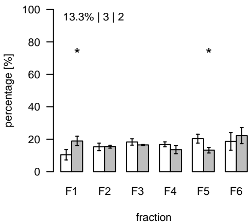
L2296 (m/z=680.44165; rt=11.32798) T/S Cluster: L-11.3-4
