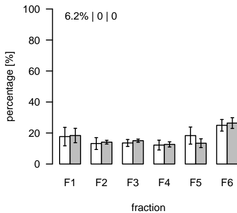
L140 (m/z=843.547498; rt=3.65242) T/S Cluster: L-3.7-3
