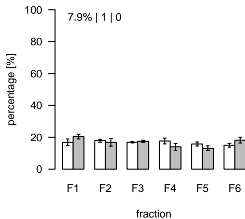
L2796 (m/z=1164.099886; rt=17.94436) T/S Cluster: L-17.9-1
