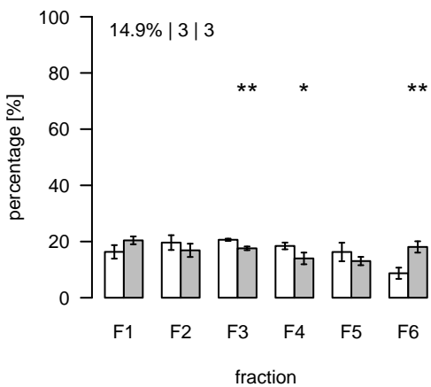
L1175 (m/z=960.585945; rt=6.65986) T/S Cluster: L-6.7-6
