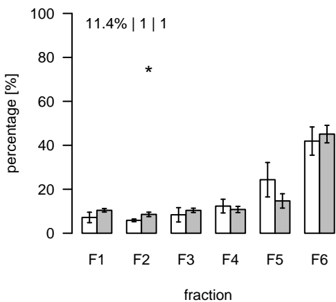
L817 (m/z=856.495816; rt=5.66095) T/S Cluster: L-5.7-1
