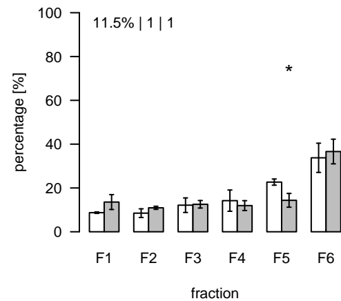
L1114 (m/z=941.533861; rt=6.59733) T/S Cluster: L-6.6-7
