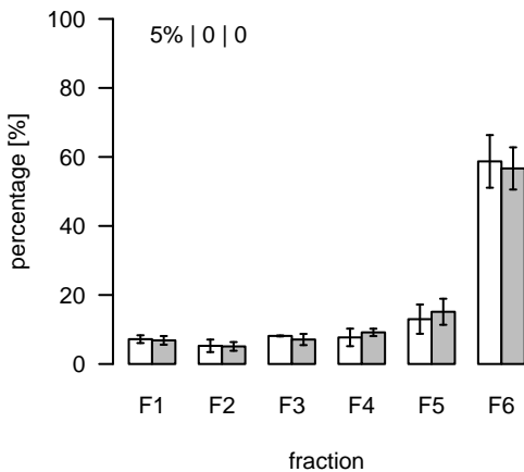
L1742 (m/z=797.602325; rt=8.84813) T/S Cluster: L-8.8-2
