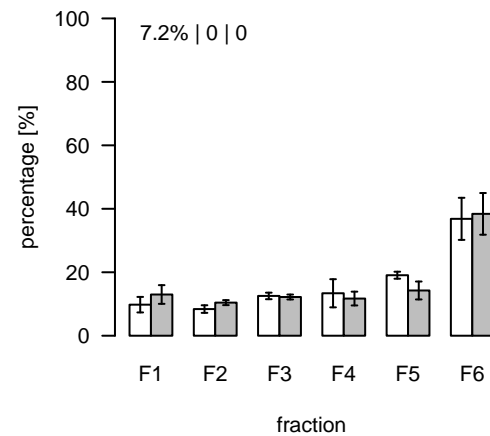
L1146 (m/z=318.879084; rt=6.65381) T/S Cluster: L-6.7-3
