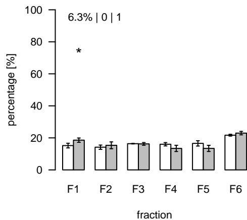
L1773 (m/z=453.770355; rt=8.91495) T/S Cluster: L-8.9-5
