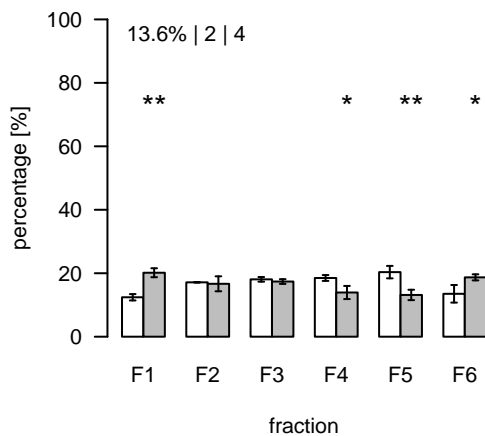
L2341 (m/z=727.469583; rt=11.32848) T/S Cluster: L-11.3-24
