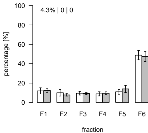
L1632 (m/z=887.545378; rt=8.59721) T/S Cluster: L-8.6-3
