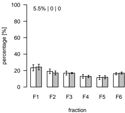
L664 (m/z=828.509645; rt=5.01521) T/S Cluster: L-5-5
