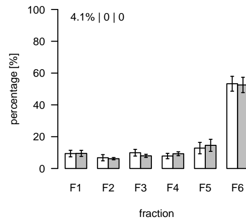
L1907 (m/z=888.555099; rt=9.58502) T/S Cluster: L-9.6-2
