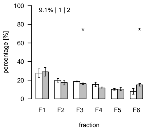
L1672 (m/z=380.796789; rt=8.70611) T/S Cluster: L-8.7-5
