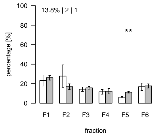
S741 (m/z=770.580618; rt=15.92413) T/S Cluster: S-15.9-6
