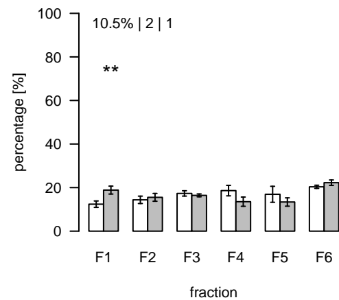
L1796 (m/z=1104.707104; rt=8.91793) T/S Cluster: L-8.9-10
