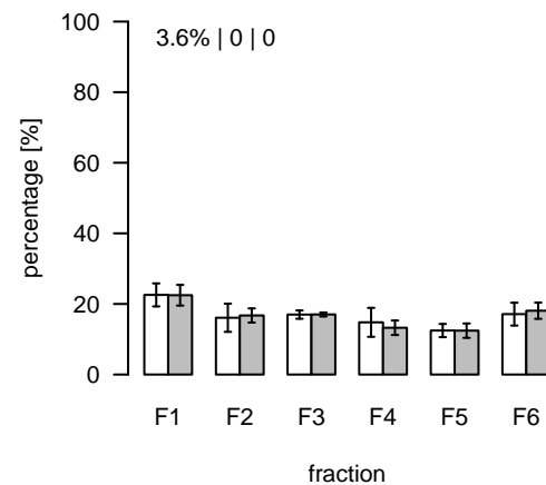
L2423 (m/z=862.72174; rt=11.73858) T/S Cluster: L-11.7-3
