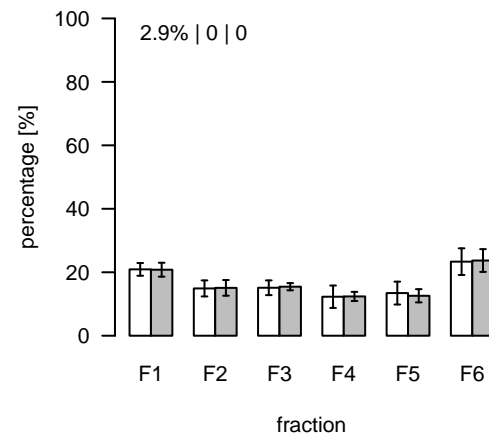
L1269 (m/z=755.551654; rt=7.1874) T/S Cluster: L-7.2-2
