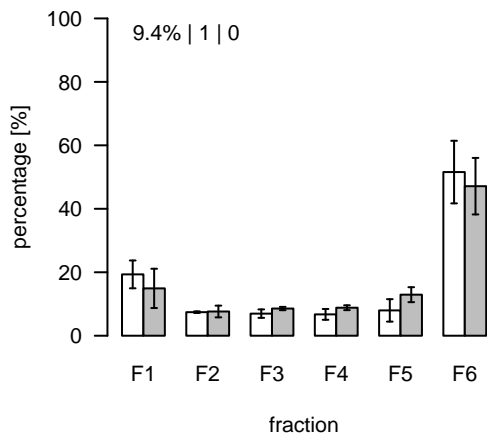
S823 (m/z=766.538433; rt=16.57395) T/S Cluster: S-16.6-1
