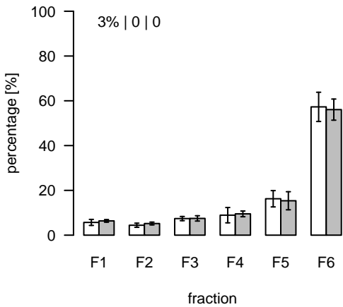
L904 (m/z=928.596437; rt=5.93358) T/S Cluster: L-5.9-4
