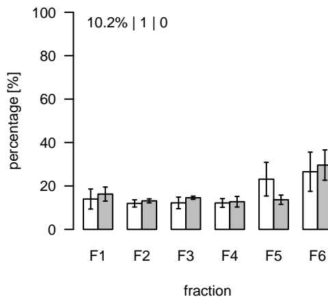
L1944 (m/z=903.569014; rt=9.64593) T/S Cluster: L-9.6-6
