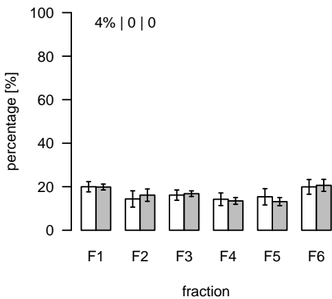
L1397 (m/z=730.540982; rt=7.62448) T/S Cluster: L-7.6-2
