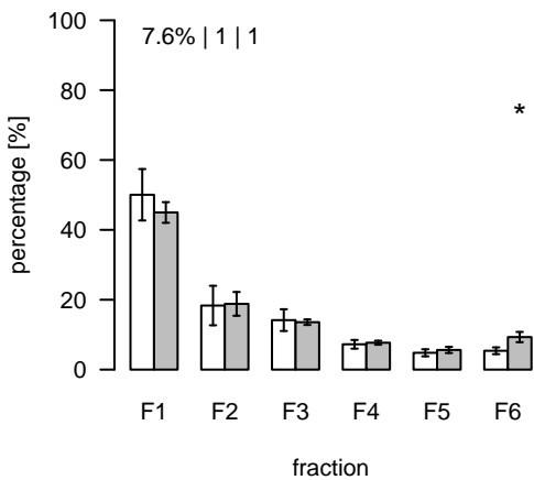
S93 (m/z=519.14016; rt=4.70433) T/S Cluster: S-4.7-1
