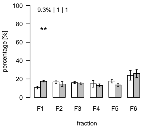
L2579 (m/z=906.231112; rt=15.36524) T/S Cluster: L-15.4-3
