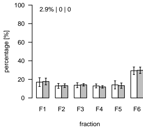
L267 (m/z=832.575809; rt=4.00906) T/S Cluster: L-4-7
