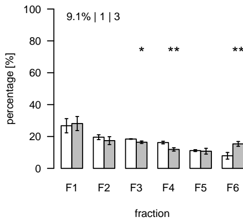
L1681 (m/z=253.530561; rt=8.70678) T/S Cluster: L-8.7-5
