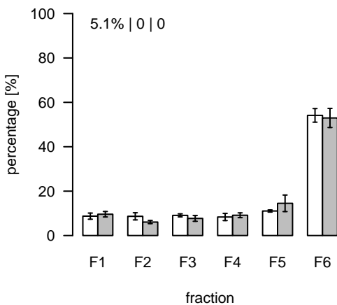
L1830 (m/z=888.576609; rt=9.15903) T/S Cluster: L-9.2-1
