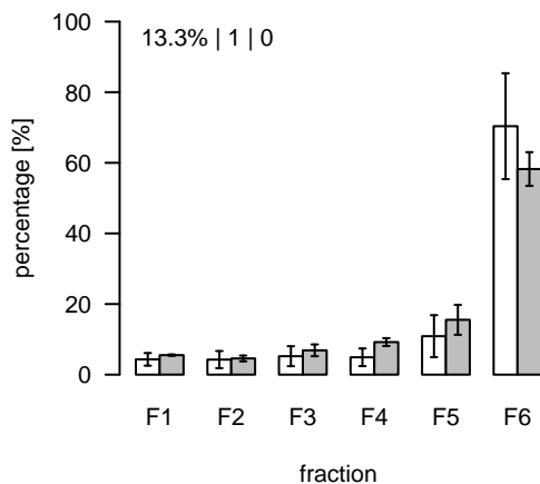
L1740 (m/z=891.568987; rt=8.81159) T/S Cluster: L-8.8-2
