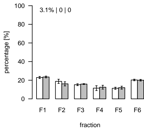
S565 (m/z=349.235656; rt=14.11394) T/S Cluster: S-14.1-2
