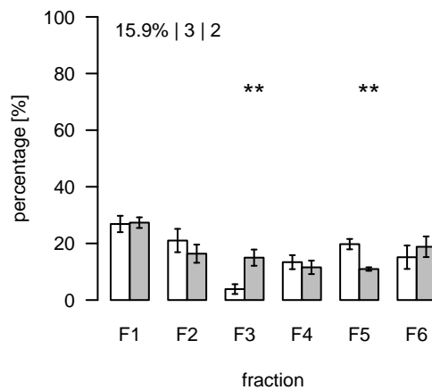
S845 (m/z=437.732862; rt=16.65029) T/S Cluster: S-16.7-1
