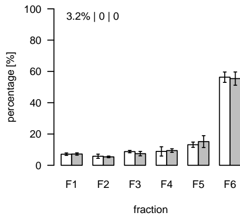
L936 (m/z=342.234516; rt=6.12675) T/S Cluster: L-6.1-1
