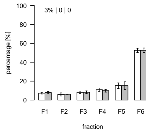
L715 (m/z=786.509096; rt=5.22488) T/S Cluster: L-5.2-4
