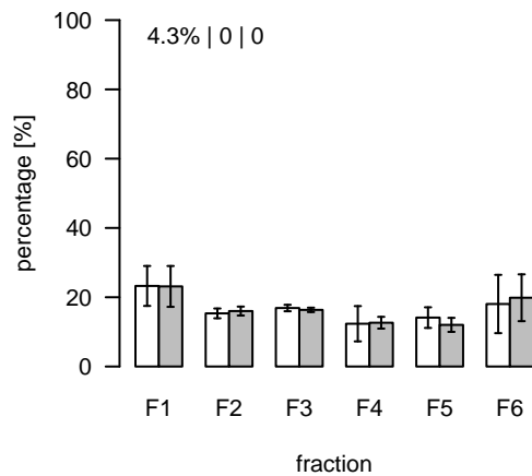
L1311 (m/z=390.76957; rt=7.32757) T/S Cluster: L-7.3-5
