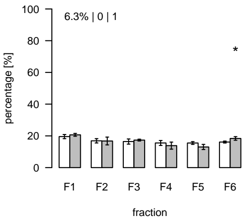
S502 (m/z=344.179703; rt=12.98455) T/S Cluster: S-13-2
