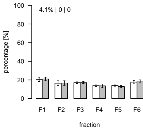
S289 (m/z=305.102564; rt=8.72237) T/S Cluster: S-8.7-1
