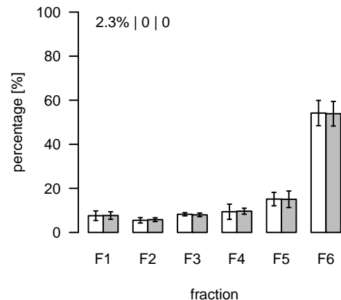
L1534 (m/z=959.657687; rt=8.05104) T/S Cluster: L-8.1-1
