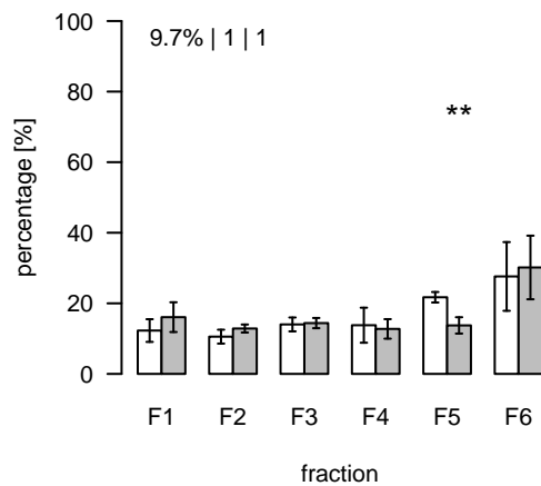
L919 (m/z=931.543653; rt=5.96081) T/S Cluster: L-6-2
