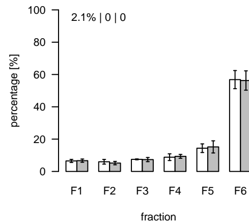
L393 (m/z=942.585674; rt=4.38964) T/S Cluster: L-4.4-2
