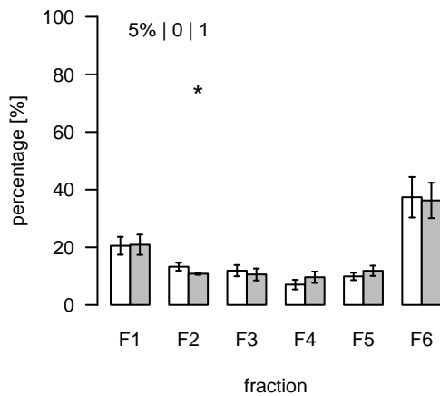
S578 (m/z=653.368505; rt=14.34934) T/S Cluster: S-14.3-4
