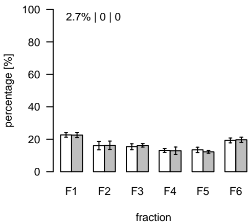
S532 (m/z=307.227236; rt=13.44778) T/S Cluster: S-13.4-5
