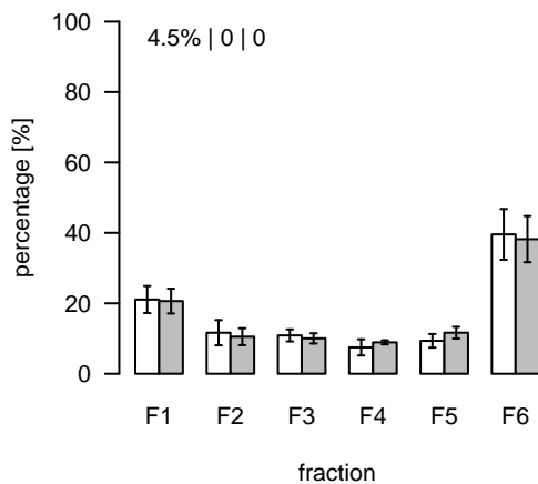
S293 (m/z=872.545735; rt=8.80174) T/S Cluster: S-8.8-1
