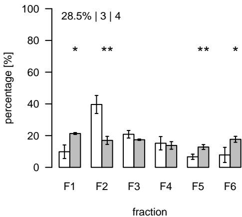
S864 (m/z=764.547829; rt=16.9773) T/S Cluster: S-17-6
