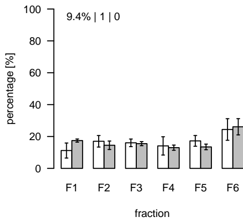
L2767 (m/z=601.674221; rt=16.96478) T/S Cluster: L-17-2
