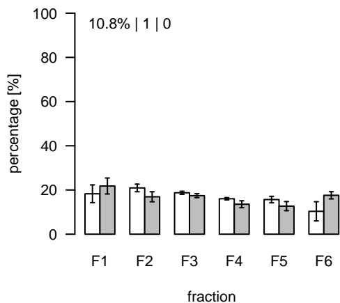
L2367 (m/z=686.491277; rt=11.32869) T/S Cluster: L-11.3-17
