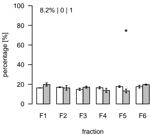
S343 (m/z=437.750499; rt=10.8718) T/S Cluster: S-10.9-2
