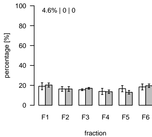
L429 (m/z=835.594523; rt=4.4844) T/S Cluster: L-4.5-4
