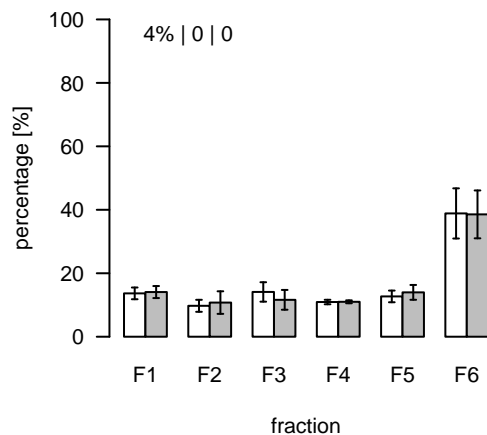
L488 (m/z=820.515641; rt=4.70551) T/S Cluster: L-4.7-5
