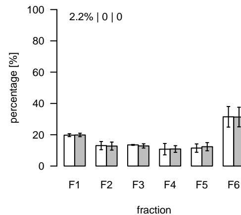
L701 (m/z=788.546324; rt=5.12672) T/S Cluster: L-5.1-9
