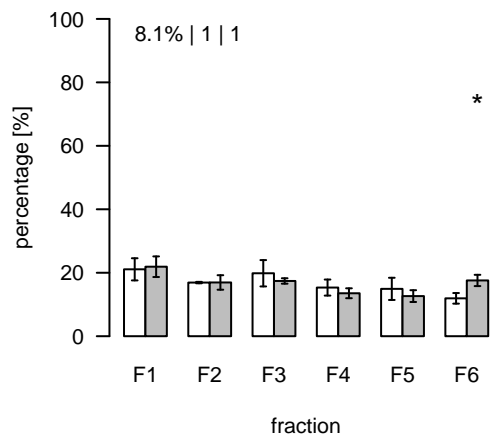
L2603 (m/z=824.767348; rt=15.56767) T/S Cluster: L-15.6-1
