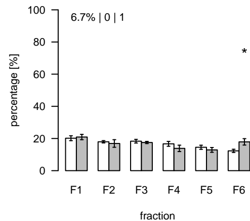
L2707 (m/z=866.821291; rt=16.16538) T/S Cluster: L-16.2-3
