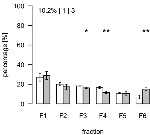
L1682 (m/z=380.293379; rt=8.70679) T/S Cluster: L-8.7-5
