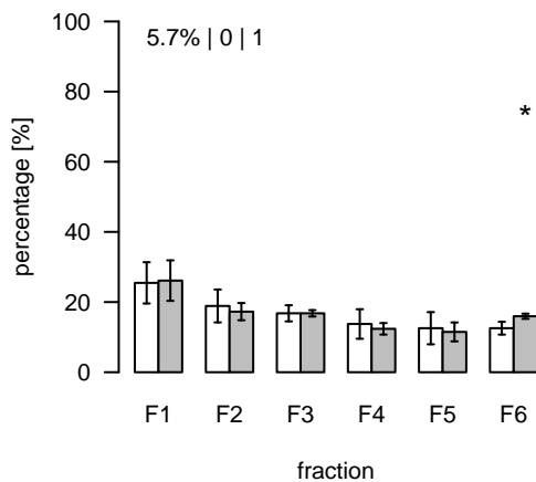
L121 (m/z=690.426556; rt=3.61581) T/S Cluster: L-3.6-6
