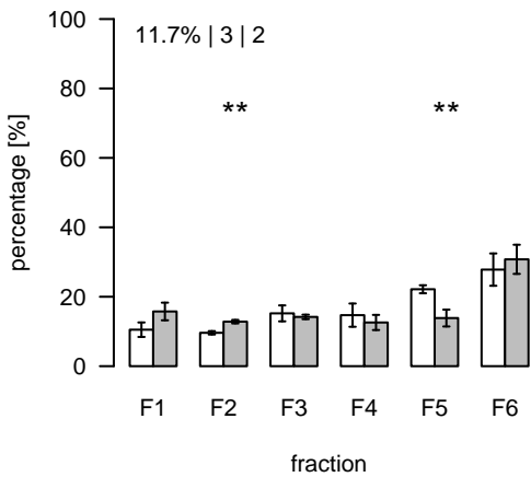
L515 (m/z=786.483892; rt=4.79151) T/S Cluster: L-4.8-3
