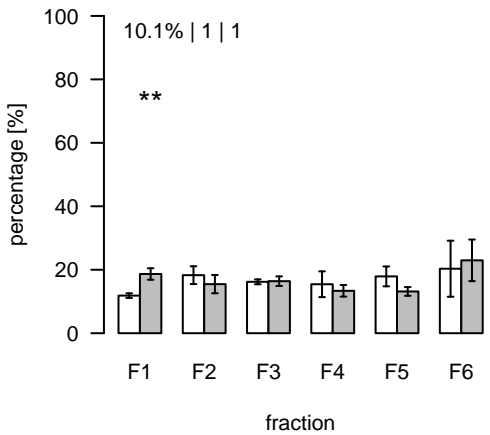
L2719 (m/z=1058.300589; rt=16.17896) T/S Cluster: L-16.2-5
