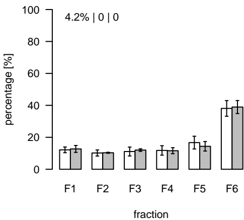
L320 (m/z=854.526705; rt=4.22487) T/S Cluster: L-4.2-11
