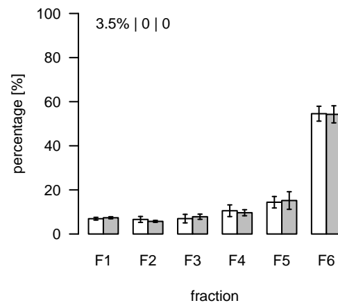
L530 (m/z=391.269306; rt=4.8107) T/S Cluster: L-4.8-10
