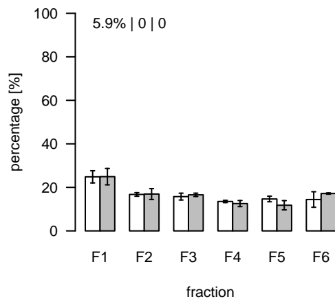
L1140 (m/z=982.602641; rt=6.64963) T/S Cluster: L-6.6-13
