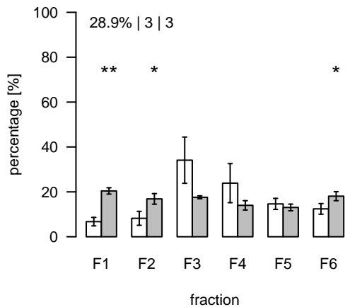
S879 (m/z=761.589933; rt=16.99719) T/S Cluster: S-17-13
