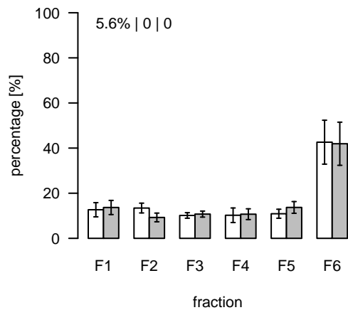
S566 (m/z=1002.604683; rt=14.14891) T/S Cluster: S-14.1-3
