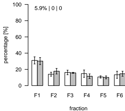
L769 (m/z=804.55613; rt=5.34019) T/S Cluster: L-5.3-7
