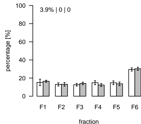
L1638 (m/z=552.499971; rt=8.61582) T/S Cluster: L-8.6-7
