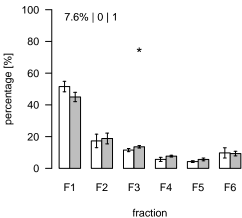
S62 (m/z=494.119748; rt=4.64609) T/S Cluster: S-4.6-1
