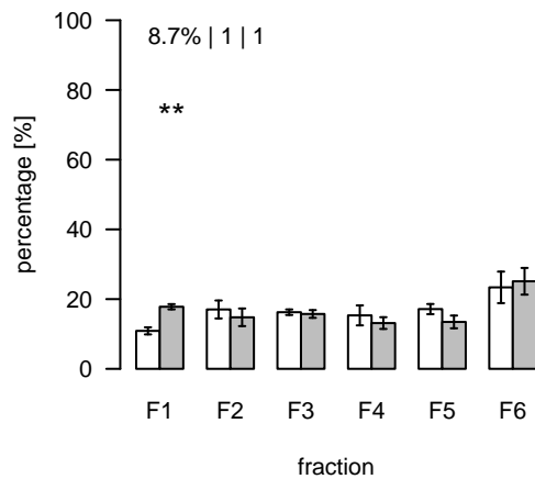
L2755 (m/z=1129.26618; rt=16.54777) T/S Cluster: L-16.5-6
