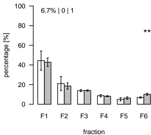
S175 (m/z=198.395367; rt=6.57809) T/S Cluster: S-6.6-2
