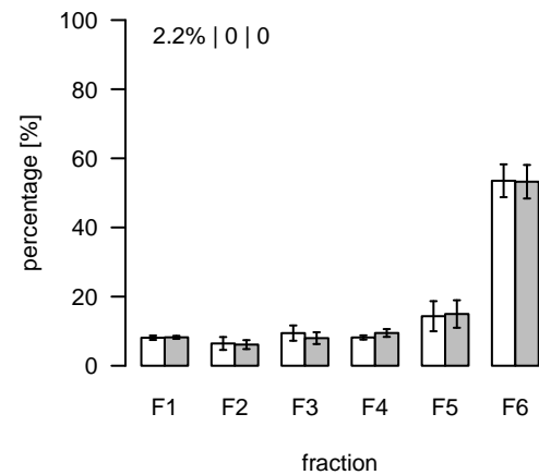
L1410 (m/z=906.550328; rt=7.65543) T/S Cluster: L-7.7-1
