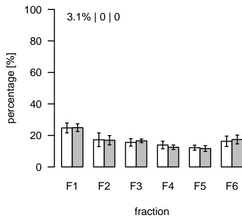
L658 (m/z=827.539411; rt=5.01399) T/S Cluster: L-5-4
