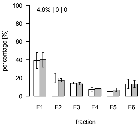
S594 (m/z=740.473958; rt=14.47245) T/S Cluster: S-14.5-4
