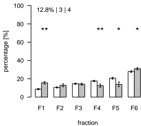
L2335 (m/z=721.512105; rt=11.3284) T/S Cluster: L-11.3-19
