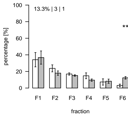
L1573 (m/z=715.497715; rt=8.13092) T/S Cluster: L-8.1-3
