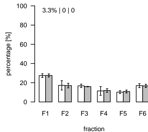
L1262 (m/z=733.569331; rt=7.16409) T/S Cluster: L-7.2-1
