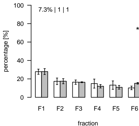
L1951 (m/z=782.570671; rt=9.65186) T/S Cluster: L-9.7-3
