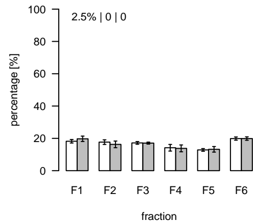
S546 (m/z=310.23574; rt=13.65218) T/S Cluster: S-13.7-2
