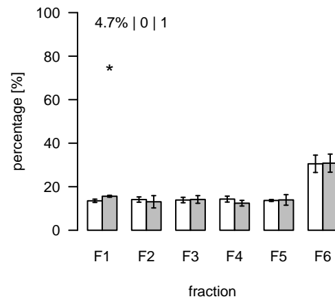
L2115 (m/z=446.774522; rt=10.50511) T/S Cluster: L-10.5-13
