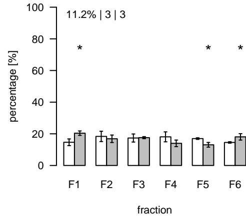
L2389 (m/z=550.632; rt=11.34431) T/S Cluster: L-11.3-39
