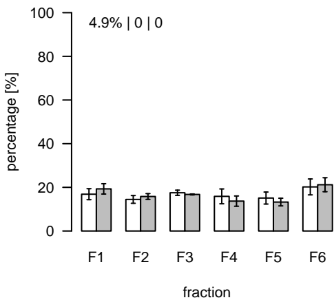
L567 (m/z=743.510116; rt=4.87535) T/S Cluster: L-4.9-3
