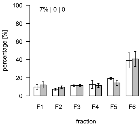
L1057 (m/z=766.541752; rt=6.54753) T/S Cluster: L-6.5-1
