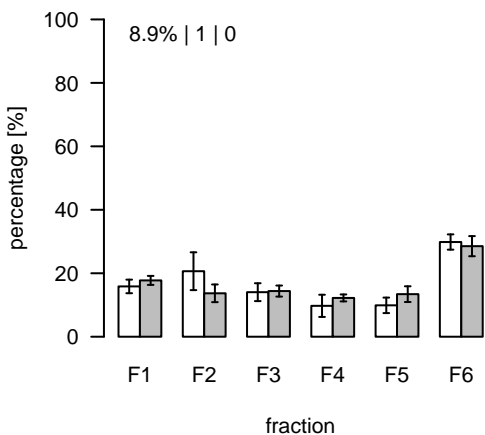
L470 (m/z=682.366845; rt=4.62285) T/S Cluster: L-4.6-7
