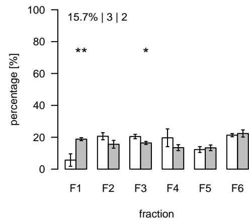
S727 (m/z=680.483317; rt=15.81148) T/S Cluster: S-15.8-5
