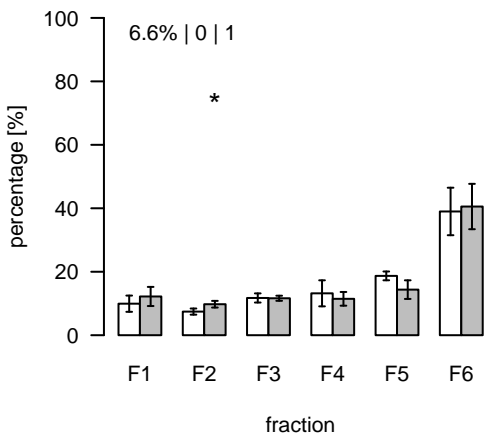
L1089 (m/z=254.841967; rt=6.54778) T/S Cluster: L-6.5-1
