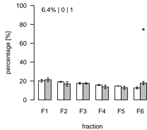
L2676 (m/z=923.294113; rt=15.84434) T/S Cluster: L-15.8-4
