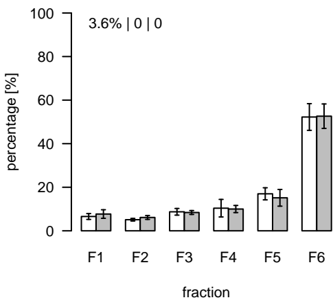
L1020 (m/z=929.611525; rt=6.49643) T/S Cluster: L-6.5-1
