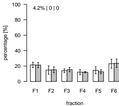
L289 (m/z=216.814993; rt=4.09623) T/S Cluster: L-4.1-2
