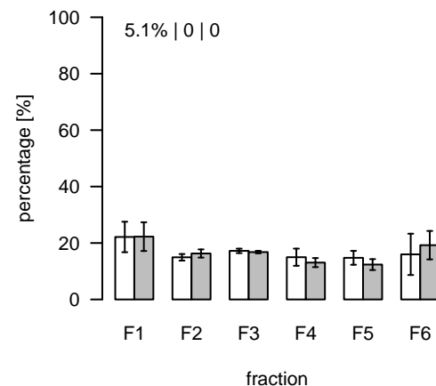
L1313 (m/z=390.261971; rt=7.32797) T/S Cluster: L-7.3-5
