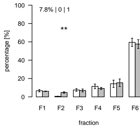
L638 (m/z=781.589073; rt=4.95185) T/S Cluster: L-5-1
