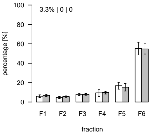
L908 (m/z=928.554717; rt=5.93364) T/S Cluster: L-5.9-4
