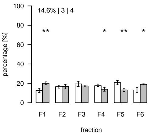
L2287 (m/z=1411.003668; rt=11.3279) T/S Cluster: L-11.3-4
