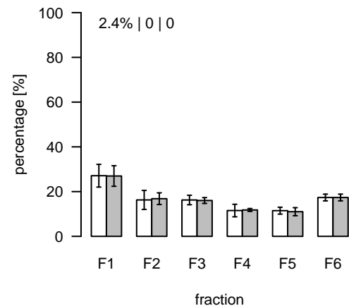
S396 (m/z=725.446012; rt=12.36346) T/S Cluster: S-12.4-2
