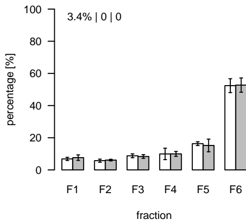
L1709 (m/z=771.563063; rt=8.70932) T/S Cluster: L-8.7-7
