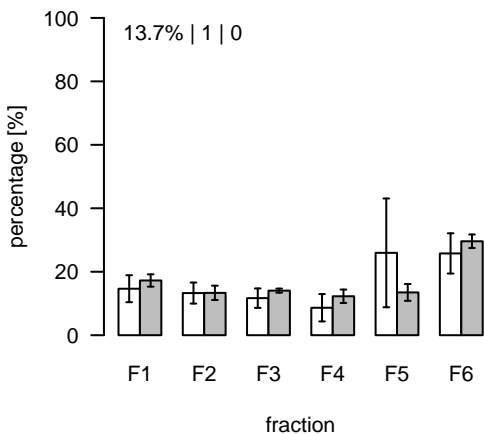
L1466 (m/z=738.537995; rt=7.9195) T/S Cluster: L-7.9-12
