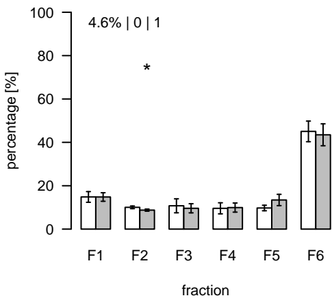
S671 (m/z=656.416084; rt=14.97841) T/S Cluster: S-15-3
