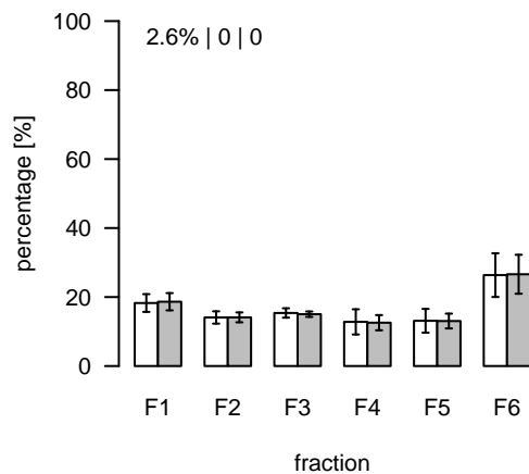
L859 (m/z=257.521284; rt=5.71476) T/S Cluster: L-5.7-4
