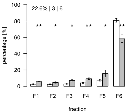
L1974 (m/z=907.525651; rt=9.87991) T/S Cluster: L-9.9-2
