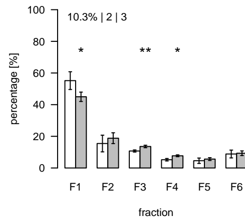
S33 (m/z=497.130775; rt=3.71976) T/S Cluster: S-3.7-1
