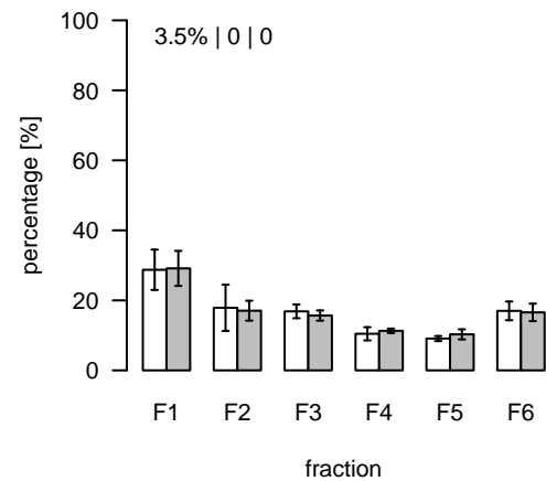
S364 (m/z=741.441077; rt=12.06072) T/S Cluster: S-12.1-2
