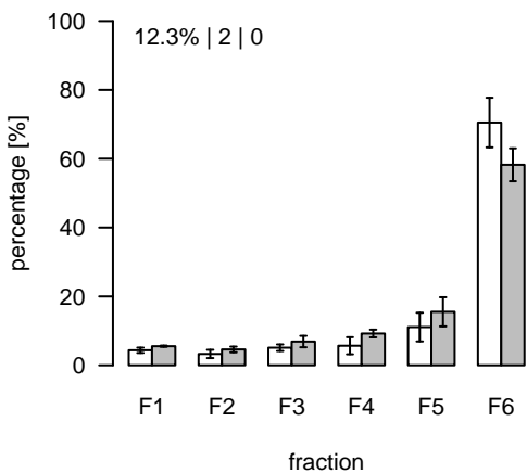
L14 (m/z=674.38601; rt=2.50455) T/S Cluster: L-2.5-1
