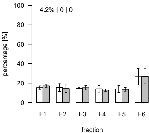
L266 (m/z=833.576018; rt=4.00771) T/S Cluster: L-4-6
