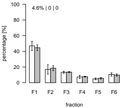
S258 (m/z=538.230008; rt=7.74501) T/S Cluster: S-7.7-1
