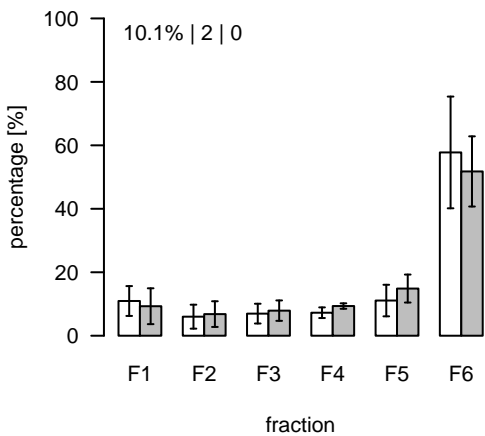
L290 (m/z=841.555272; rt=4.09698) T/S Cluster: L-4.1-4
