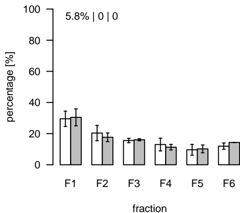
L1927 (m/z=761.673501; rt=9.59737) T/S Cluster: L-9.6-3
