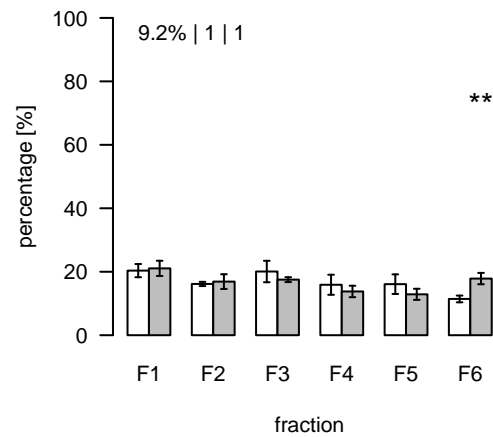
L2601 (m/z=796.742038; rt=15.55342) T/S Cluster: L-15.6-1
