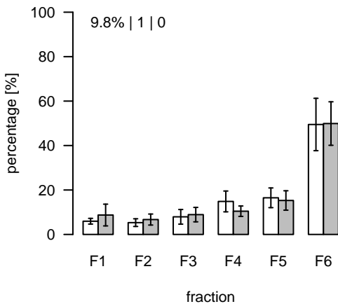
L1938 (m/z=910.550883; rt=9.61903) T/S Cluster: L-9.6-5
