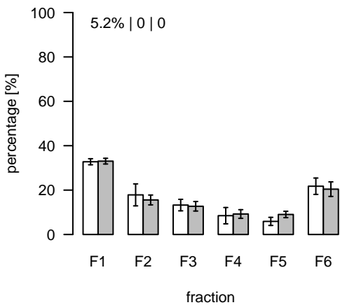
S609 (m/z=655.38624; rt=14.65472) T/S Cluster: S-14.7-1
