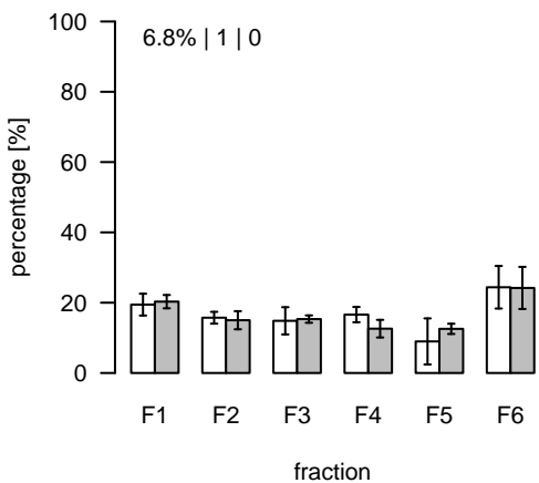
L698 (m/z=789.587463; rt=5.1255) T/S Cluster: L-5.1-7
