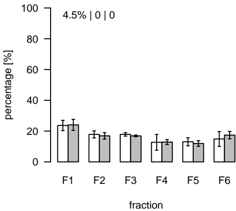
L1494 (m/z=252.189377; rt=7.93917) T/S Cluster: L-7.9-14
