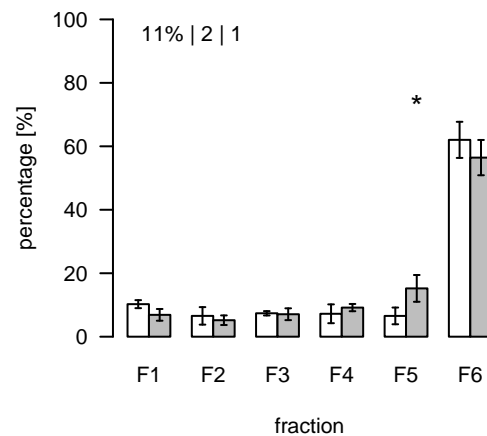
L231 (m/z=811.512457; rt=3.8994) T/S Cluster: L-3.9-5
