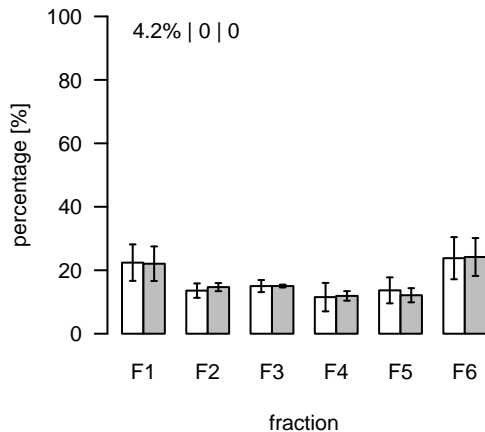
L1546 (m/z=783.576718; rt=8.05664) T/S Cluster: L-8.1-2
