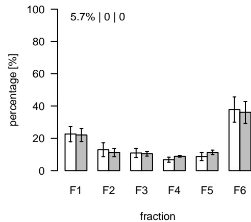
S288 (m/z=828.519036; rt=8.61841) T/S Cluster: S-8.6-3
