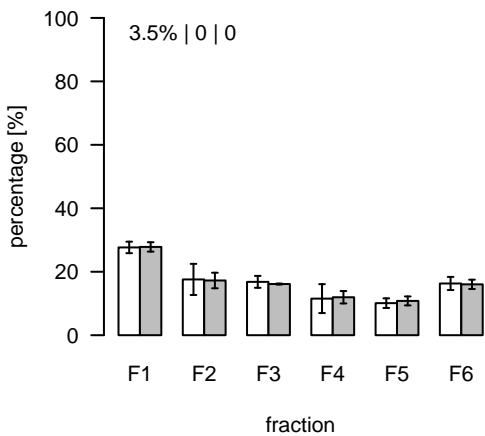
L1257 (m/z=733.542083; rt=7.16388) T/S Cluster: L-7.2-1
