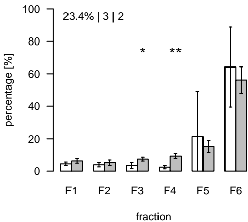
L2229 (m/z=903.567442; rt=11.231) T/S Cluster: L-11.2-2
