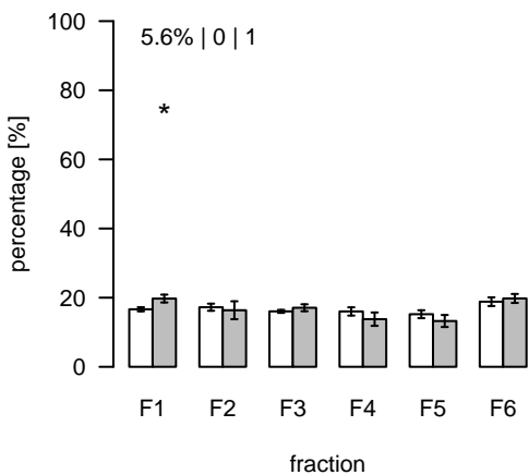
S479 (m/z=290.219843; rt=12.91121) T/S Cluster: S-12.9-12
