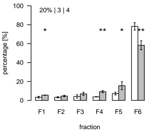
L1973 (m/z=908.532285; rt=9.87985) T/S Cluster: L-9.9-2
