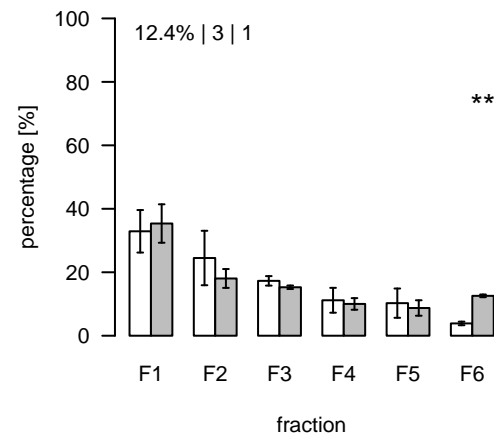
L157 (m/z=333.721047; rt=3.67488) T/S Cluster: L-3.7-14
