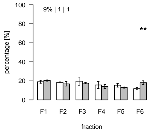
L2644 (m/z=825.777321; rt=15.82297) T/S Cluster: L-15.8-3
