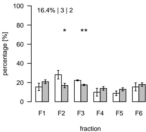
S750 (m/z=518.406788; rt=16.0437) T/S Cluster: S-16-4
