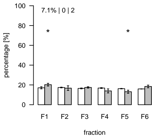
S496 (m/z=173.610324; rt=12.91293) T/S Cluster: S-12.9-25
