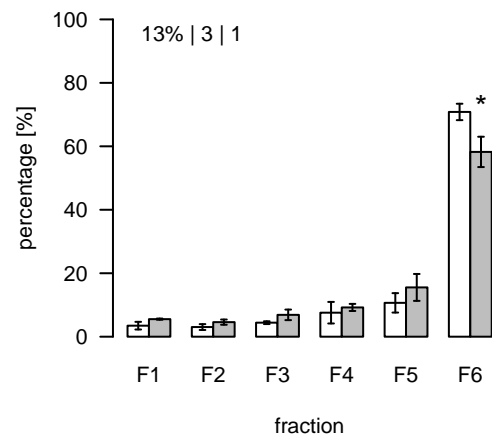
L1834 (m/z=910.545805; rt=9.18792) T/S Cluster: L-9.2-2
