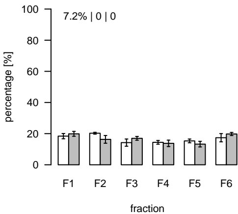
S801 (m/z=392.288689; rt=16.49223) T/S Cluster: S-16.5-5
