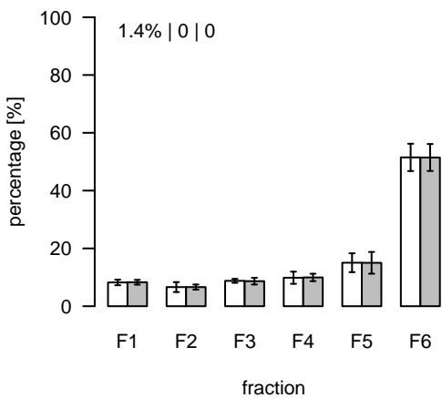
L854 (m/z=946.620335; rt=5.71383) T/S Cluster: L-5.7-1
