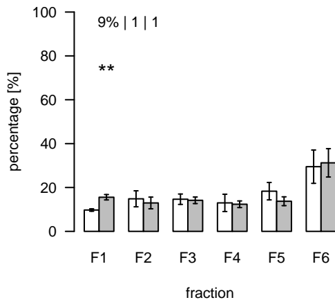
L2504 (m/z=684.188612; rt=12.76663) T/S Cluster: L-12.8-1
