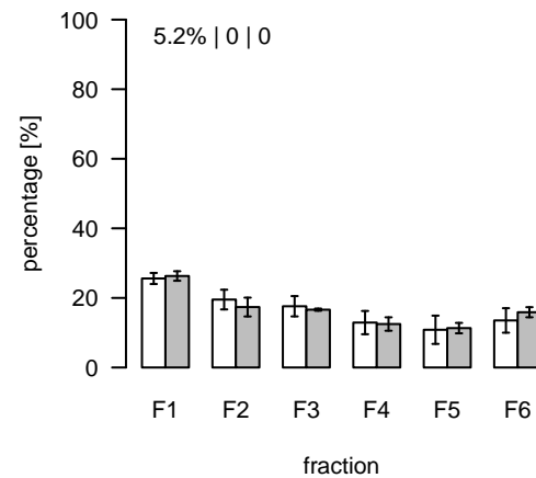
L1222 (m/z=775.537098; rt=6.7827) T/S Cluster: L-6.8-2
