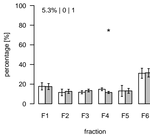
L1395 (m/z=780.557237; rt=7.61583) T/S Cluster: L-7.6-2
