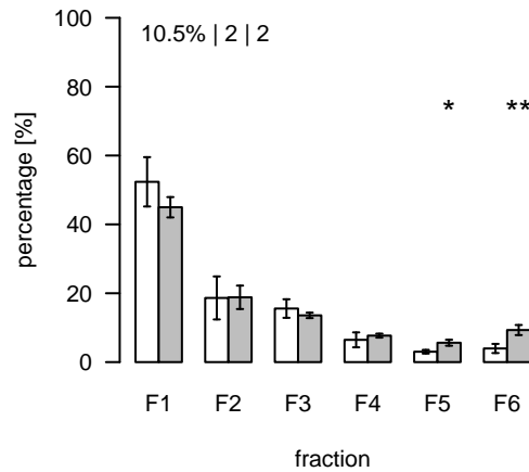
S173 (m/z=1206.360419; rt=6.57793) T/S Cluster: S-6.6-2
