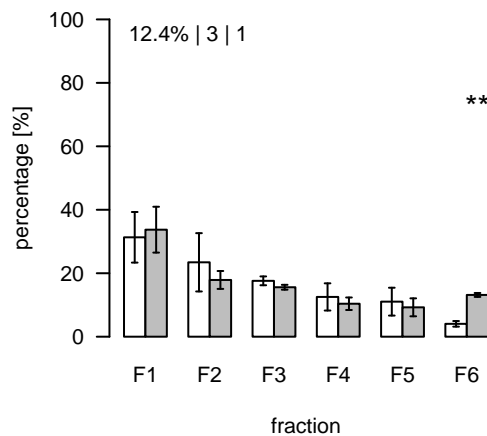
L81 (m/z=652.407087; rt=3.48112) T/S Cluster: L-3.5-4
