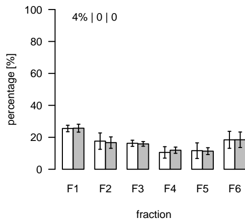
L788 (m/z=788.547131; rt=5.43688) T/S Cluster: L-5.4-5
