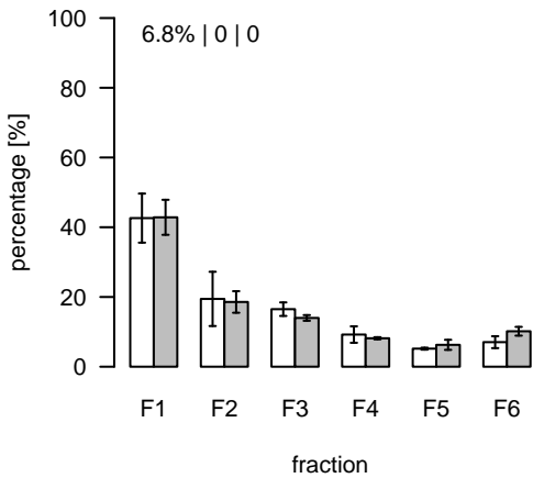
S178 (m/z=597.154557; rt=6.57952) T/S Cluster: S-6.6-2
