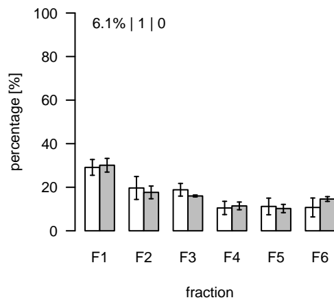
L801 (m/z=788.547006; rt=5.53665) T/S Cluster: L-5.5-1
