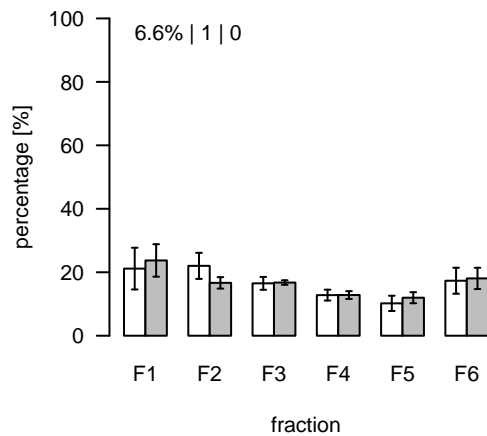
L885 (m/z=789.553753; rt=5.75745) T/S Cluster: L-5.8-2
