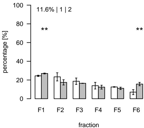
L1908 (m/z=391.283613; rt=9.59492) T/S Cluster: L-9.6-3
