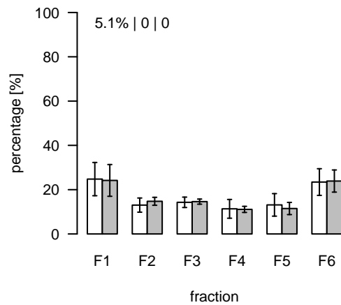
L1538 (m/z=392.295469; rt=8.05554) T/S Cluster: L-8.1-2
