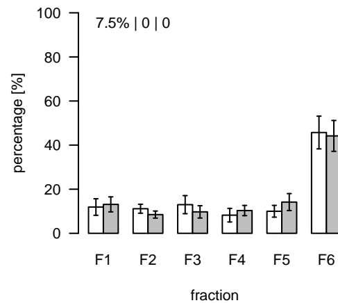
L3 (m/z=415.213114; rt=1.36432) T/S Cluster: L-1.4-1
