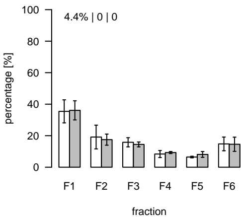
S324 (m/z=598.301129; rt=10.06174) T/S Cluster: S-10.1-1
