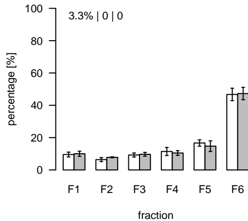
L1459 (m/z=770.542739; rt=7.91704) T/S Cluster: L-7.9-9
