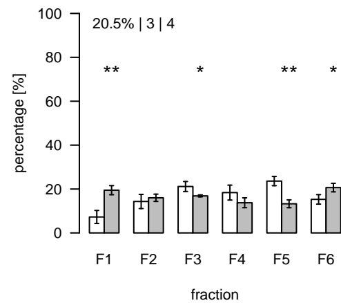
L2362 (m/z=671.473439; rt=11.32863) T/S Cluster: L-11.3-4
