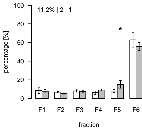
S709 (m/z=971.616914; rt=15.59826) T/S Cluster: S-15.6-2
