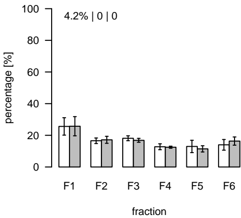
L806 (m/z=832.526938; rt=5.55439) T/S Cluster: L-5.6-3
