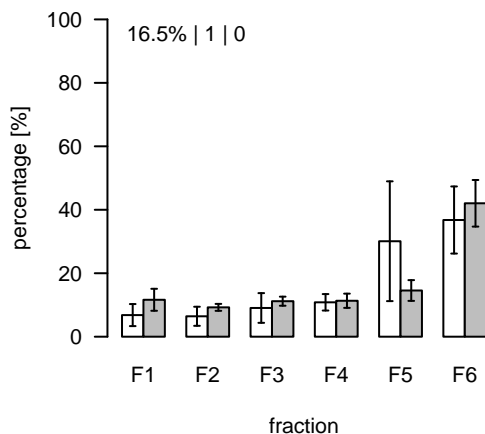
L1615 (m/z=767.547125; rt=8.43303) T/S Cluster: L-8.4-5
