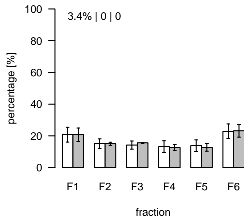
L228 (m/z=702.473626; rt=3.86527) T/S Cluster: L-3.9-3
