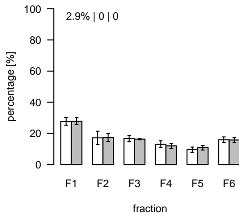
L1266 (m/z=366.281817; rt=7.16428) T/S Cluster: L-7.2-1
