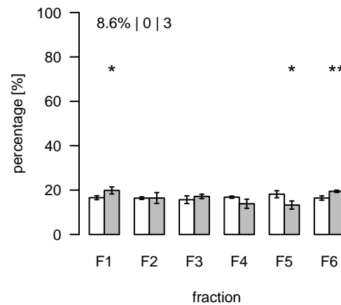
L2361 (m/z=792.609465; rt=11.3286) T/S Cluster: L-11.3-28
