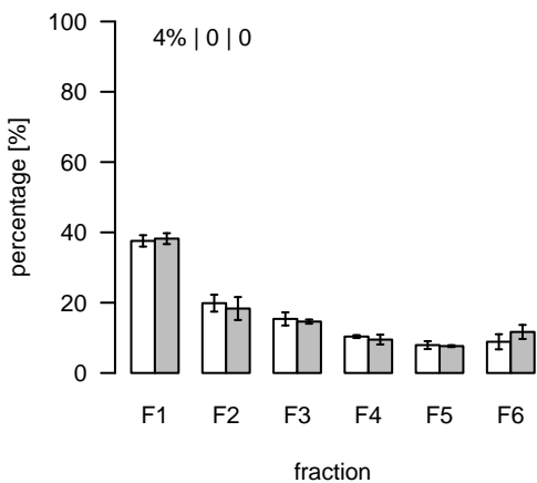
S110 (m/z=103.532803; rt=4.91058) T/S Cluster: S-4.9-1
