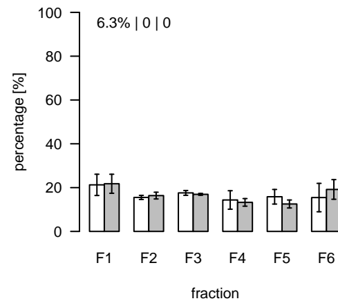
L1326 (m/z=391.281617; rt=7.33026) T/S Cluster: L-7.3-5
