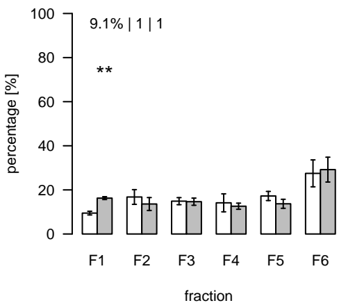
L2793 (m/z=1276.330256; rt=17.44945) T/S Cluster: L-17.4-1
