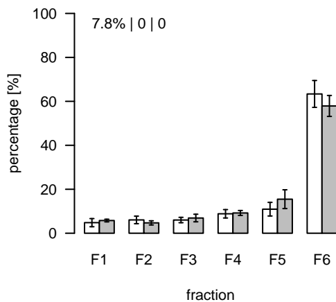
L112 (m/z=795.488414; rt=3.58165) T/S Cluster: L-3.6-3
