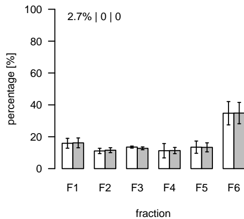
L846 (m/z=799.553841; rt=5.71124) T/S Cluster: L-5.7-4
