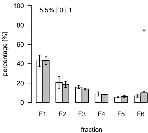
S143 (m/z=743.232701; rt=5.7031) T/S Cluster: S-5.7-1
