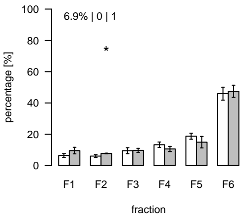
L247 (m/z=729.424936; rt=3.94037) T/S Cluster: L-3.9-7
