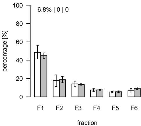
S94 (m/z=1040.282221; rt=4.70495) T/S Cluster: S-4.7-1
