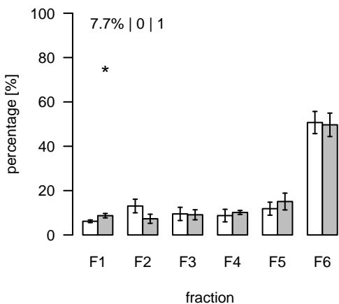
L469 (m/z=654.3202; rt=4.62222) T/S Cluster: L-4.6-6
