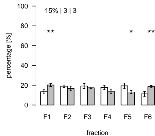
S717 (m/z=823.628113; rt=15.70538) T/S Cluster: S-15.7-5
