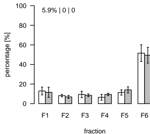
S777 (m/z=857.531196; rt=16.24222) T/S Cluster: S-16.2-6
