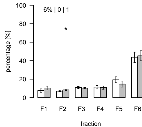
L219 (m/z=730.423129; rt=3.84015) T/S Cluster: L-3.8-5
