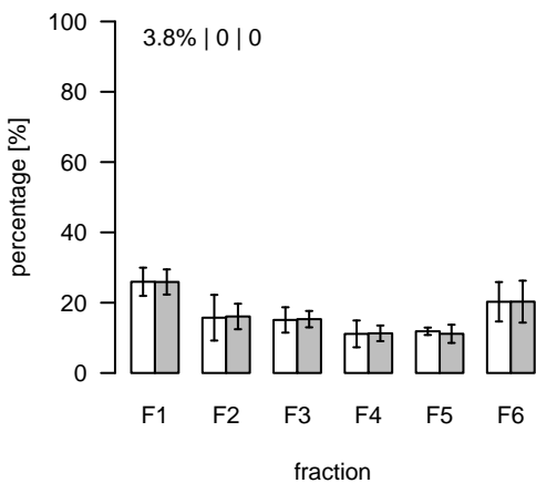
S346 (m/z=736.407149; rt=11.17579) T/S Cluster: S-11.2-1
