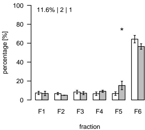
S817 (m/z=478.313321; rt=16.56961) T/S Cluster: S-16.6-3
