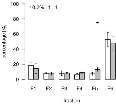
S829 (m/z=254.848185; rt=16.57421) T/S Cluster: S-16.6-1
