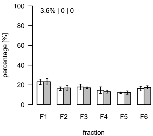
L2141 (m/z=681.625376; rt=10.6102) T/S Cluster: L-10.6-4
