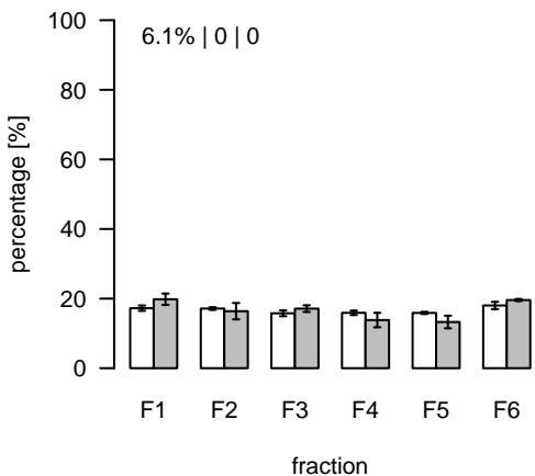
S505 (m/z=334.275069; rt=12.999) T/S Cluster: S-13-4
