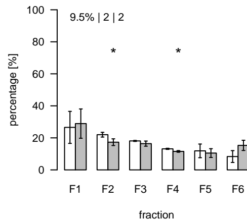
L1307 (m/z=818.517794; rt=7.32492) T/S Cluster: L-7.3-7
