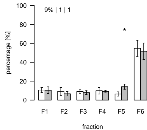
L1567 (m/z=926.511963; rt=8.11459) T/S Cluster: L-8.1-5
