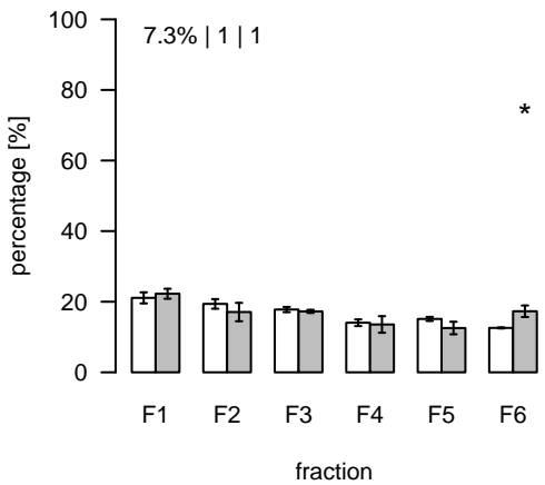
L2591 (m/z=423.149549; rt=15.46449) T/S Cluster: L-15.5-1
