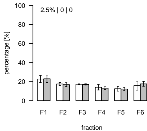
L1484 (m/z=760.571578; rt=7.93895) T/S Cluster: L-7.9-14
