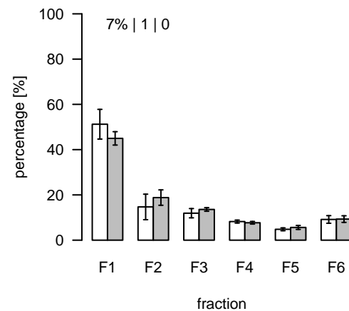
S105 (m/z=277.161517; rt=4.75558) T/S Cluster: S-4.8-1
