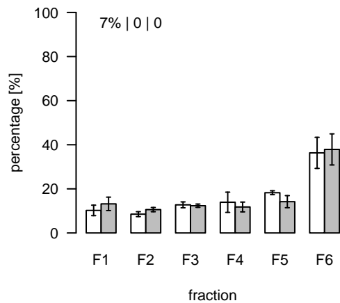
L1147 (m/z=957.632448; rt=6.65385) T/S Cluster: L-6.7-3
