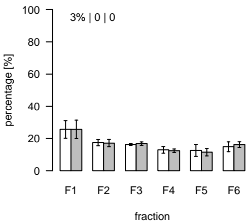
L1828 (m/z=759.576187; rt=9.09158) T/S Cluster: L-9.1-1
