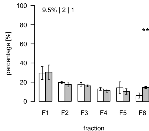
L1744 (m/z=786.574017; rt=8.87884) T/S Cluster: L-8.9-1
