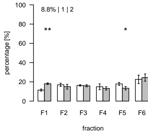
L2626 (m/z=491.142426; rt=15.8093) T/S Cluster: L-15.8-1
