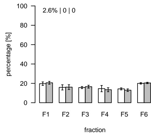
S510 (m/z=325.237852; rt=13.05783) T/S Cluster: S-13.1-2
