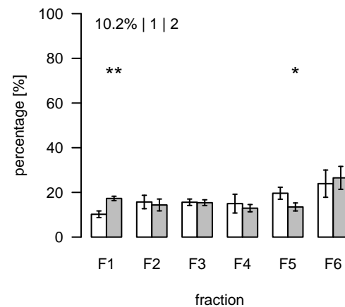
L2524 (m/z=379.113243; rt=14.004) T/S Cluster: L-14-1
