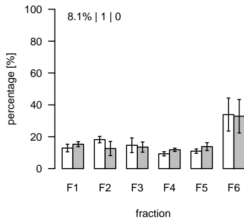
L170 (m/z=846.529389; rt=3.68132) T/S Cluster: L-3.7-18
