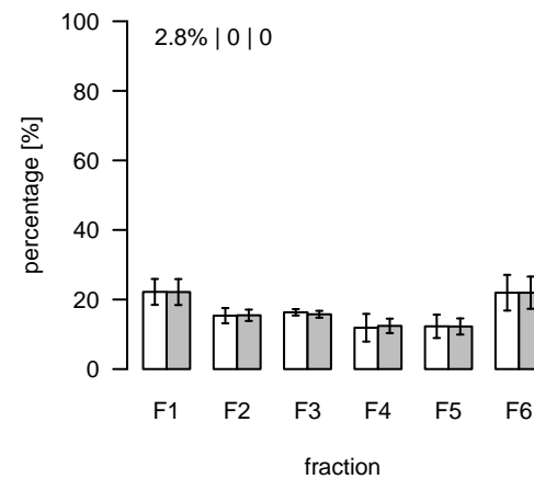
L874 (m/z=770.538266; rt=5.72204) T/S Cluster: L-5.7-7
