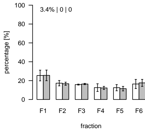
L1965 (m/z=393.301447; rt=9.82739) T/S Cluster: L-9.8-1
