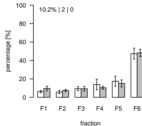
L1736 (m/z=896.489246; rt=8.744) T/S Cluster: L-8.7-8
