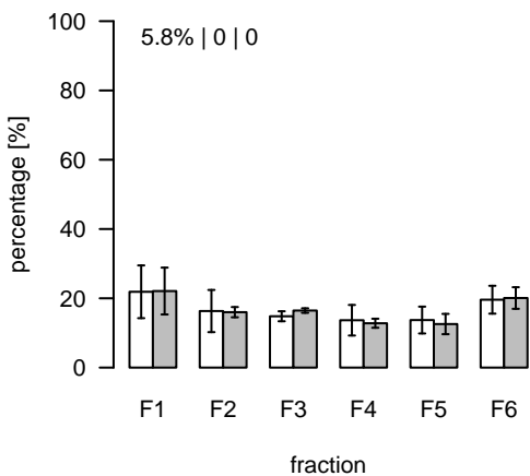
L278 (m/z=662.427147; rt=4.07558) T/S Cluster: L-4.1-2
