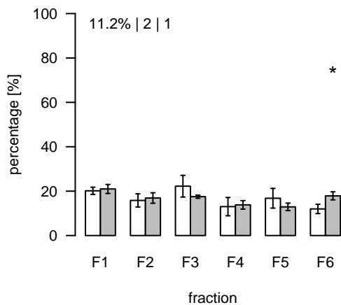
L2562 (m/z=769.713692; rt=15.24951) T/S Cluster: L-15.2-2
