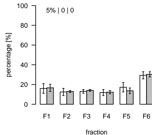
L134 (m/z=843.516913; rt=3.65148) T/S Cluster: L-3.7-3
