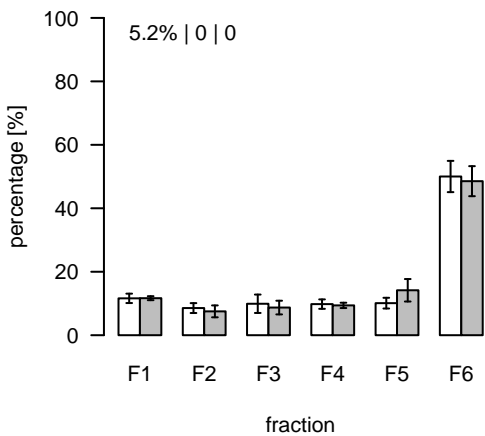
L1627 (m/z=904.542929; rt=8.5506) T/S Cluster: L-8.6-1
