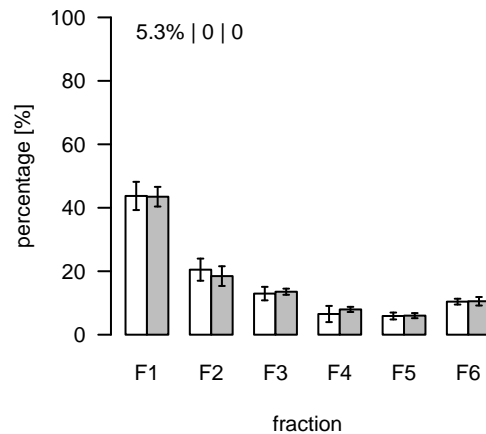
S639 (m/z=678.46747; rt=14.86874) T/S Cluster: S-14.9-2
