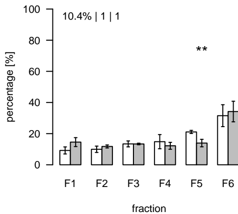
L643 (m/z=785.475774; rt=4.95277) T/S Cluster: L-5-2
