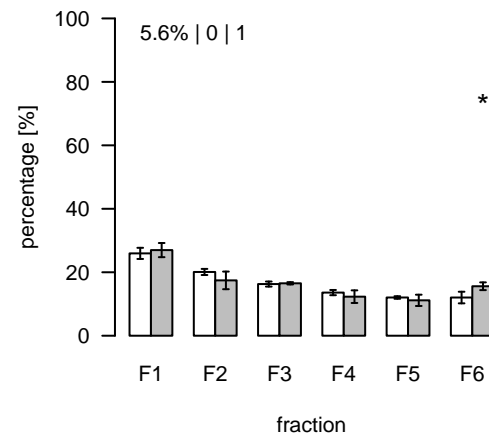
L2244 (m/z=355.261902; rt=11.32663) T/S Cluster: L-11.3-11
