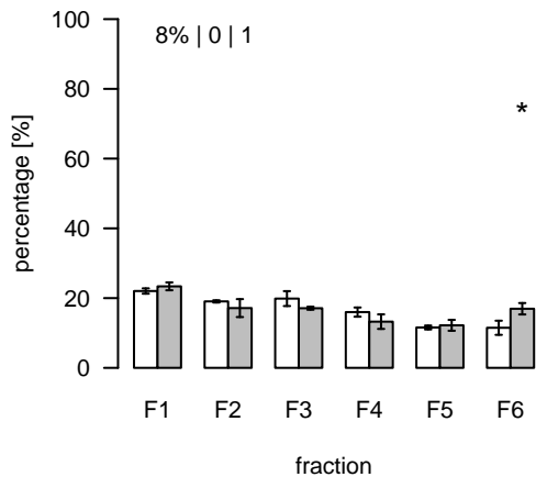
L2536 (m/z=698.257822; rt=14.29215) T/S Cluster: L-14.3-1
