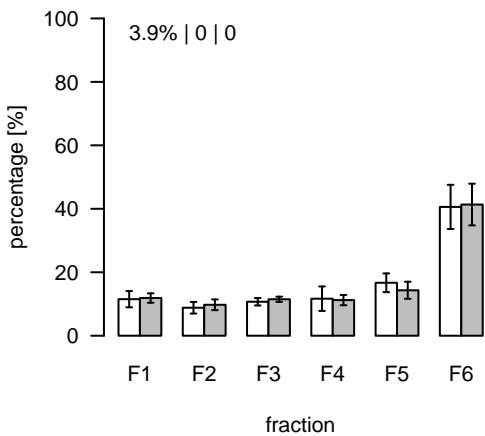
L691 (m/z=1008.590818; rt=5.09888) T/S Cluster: L-5.1-1
