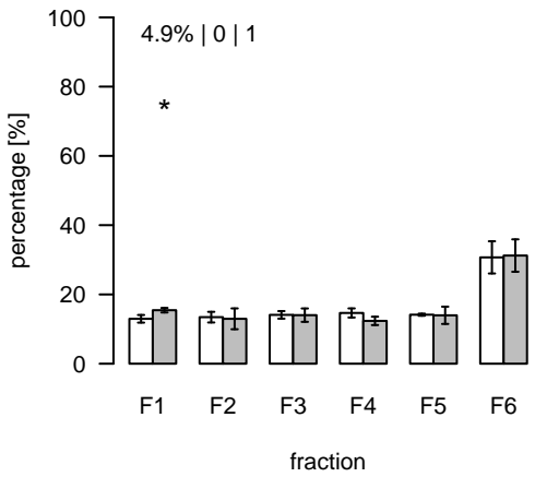
L2121 (m/z=297.845926; rt=10.50542) T/S Cluster: L-10.5-13
