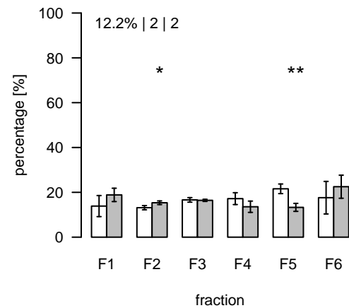
L1101 (m/z=806.526737; rt=6.54913) T/S Cluster: L-6.5-10
