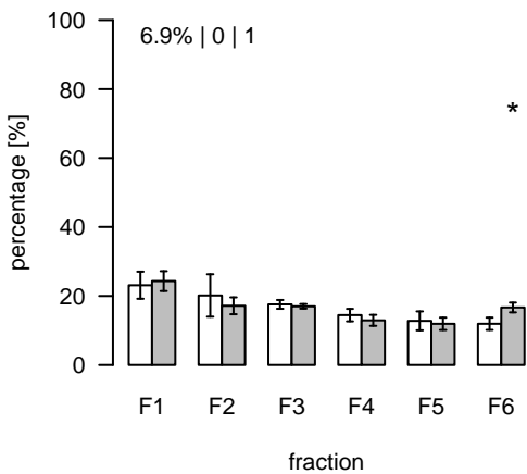
L508 (m/z=804.546739; rt=4.77266) T/S Cluster: L-4.8-5
