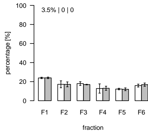
L2430 (m/z=845.696883; rt=11.74123) T/S Cluster: L-11.7-3
