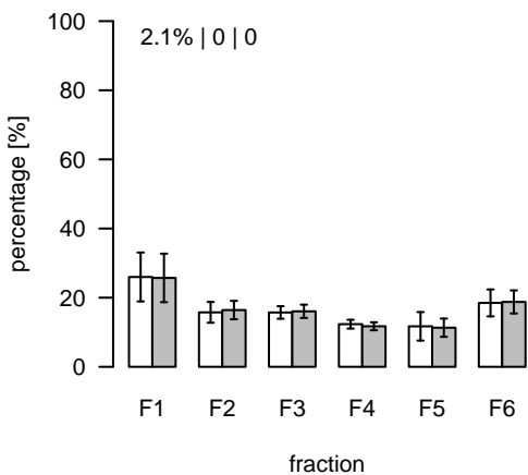
L1824 (m/z=392.298975; rt=9.06084) T/S Cluster: L-9.1-1
