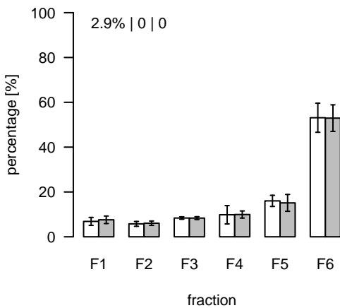
L1299 (m/z=958.643937; rt=7.30007) T/S Cluster: L-7.3-3
