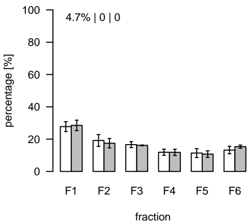
L1371 (m/z=776.544716; rt=7.47644) T/S Cluster: L-7.5-2
