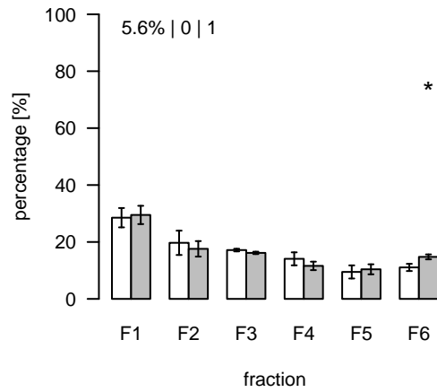
L1915 (m/z=380.797058; rt=9.59703) T/S Cluster: L-9.6-3
