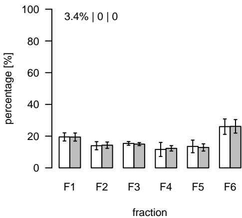
L969 (m/z=776.574217; rt=6.19002) T/S Cluster: L-6.2-5
