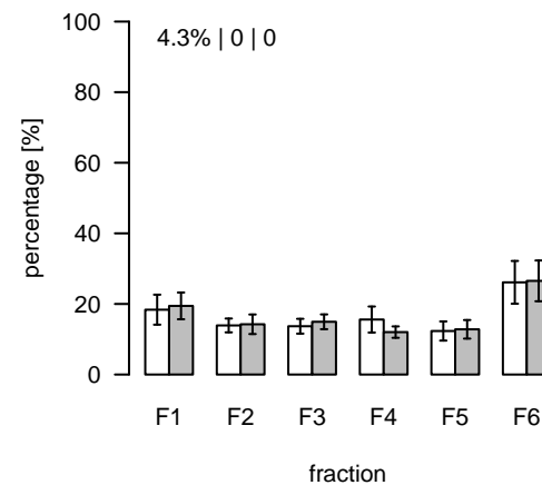
L473 (m/z=814.598303; rt=4.64612) T/S Cluster: L-4.6-9
