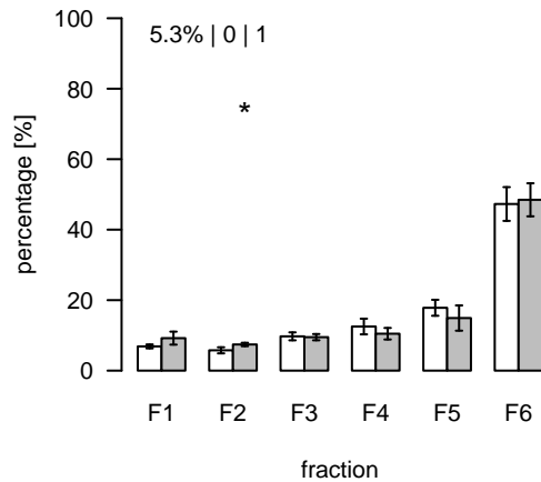
L423 (m/z=757.433746; rt=4.44758) T/S Cluster: L-4.4-2
