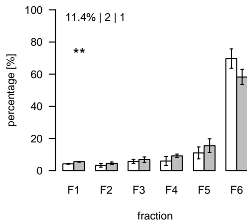
L12 (m/z=675.401071; rt=2.50425) T/S Cluster: L-2.5-1
