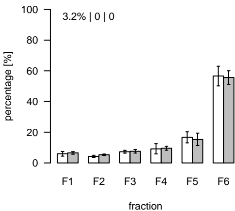
L900 (m/z=463.800668; rt=5.93348) T/S Cluster: L-5.9-4
