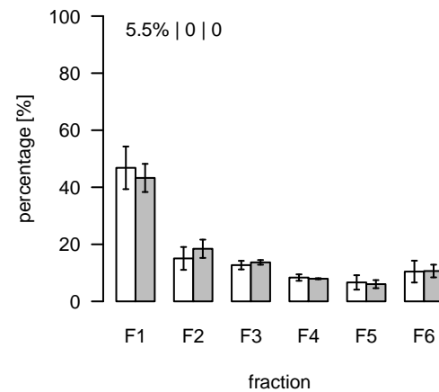
S126 (m/z=496.107072; rt=5.18076) T/S Cluster: S-5.2-1
