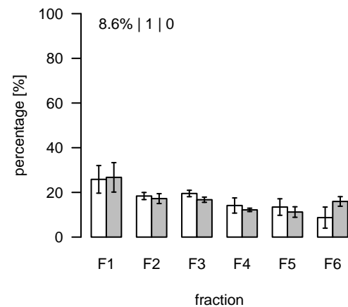
L1540 (m/z=804.561193; rt=8.05621) T/S Cluster: L-8.1-3
