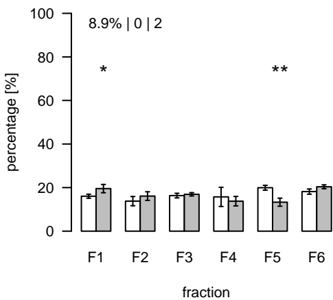
L1873 (m/z=941.575212; rt=9.51523) T/S Cluster: L-9.5-4
