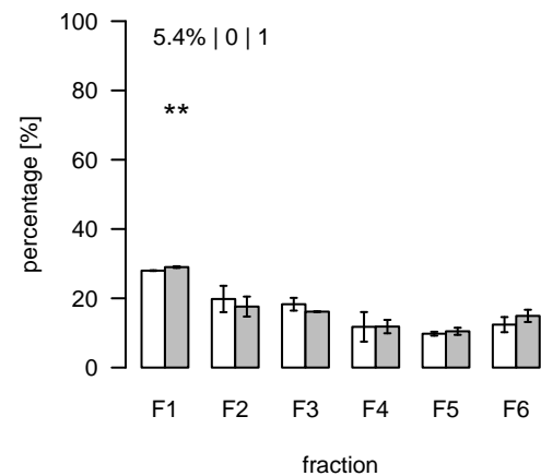
L1479 (m/z=718.580796; rt=7.93884) T/S Cluster: L-7.9-13
