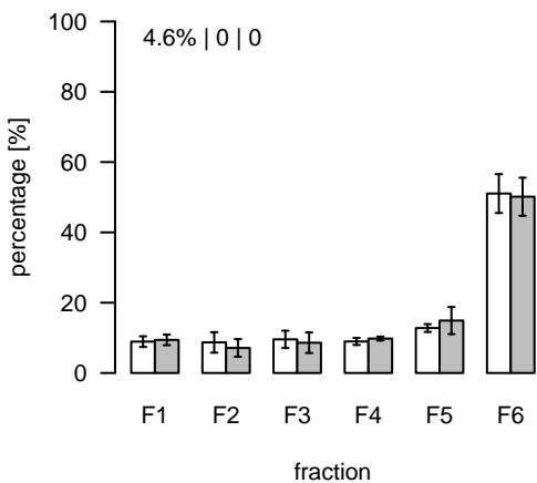
L24 (m/z=1002.610193; rt=2.84661) T/S Cluster: L-2.8-1
