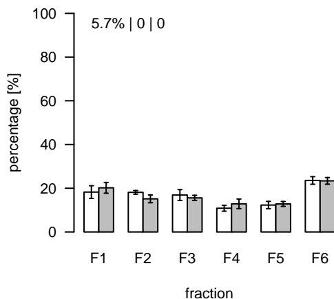
S572 (m/z=323.223915; rt=14.239) T/S Cluster: S-14.2-3
