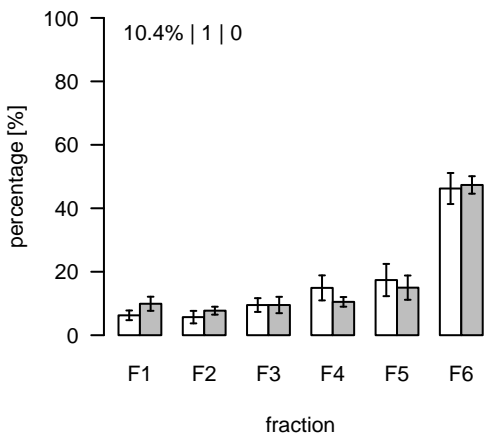
L1734 (m/z=895.495819; rt=8.7439) T/S Cluster: L-8.7-8
