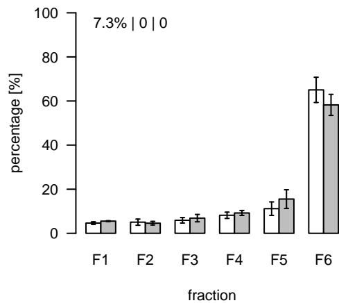
L114 (m/z=795.5146; rt=3.58173) T/S Cluster: L-3.6-3
