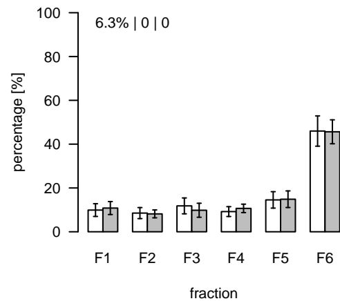
L2479 (m/z=435.795442; rt=12.38312) T/S Cluster: L-12.4-1
