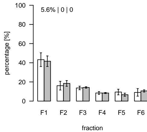
S166 (m/z=757.195874; rt=6.3684) T/S Cluster: S-6.4-1
