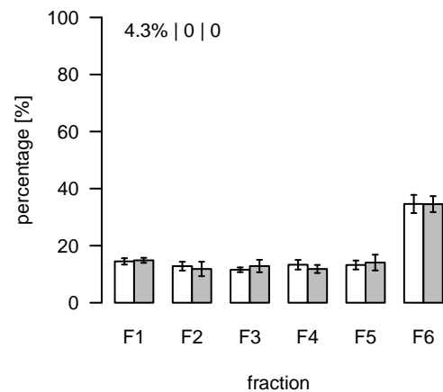
L2458 (m/z=436.797365; rt=11.84777) T/S Cluster: L-11.8-5
