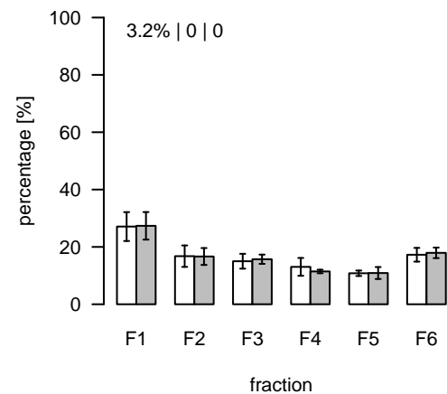
S375 (m/z=710.426472; rt=12.17141) T/S Cluster: S-12.2-5
