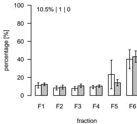
L1401 (m/z=764.54776; rt=7.6285) T/S Cluster: L-7.6-3
