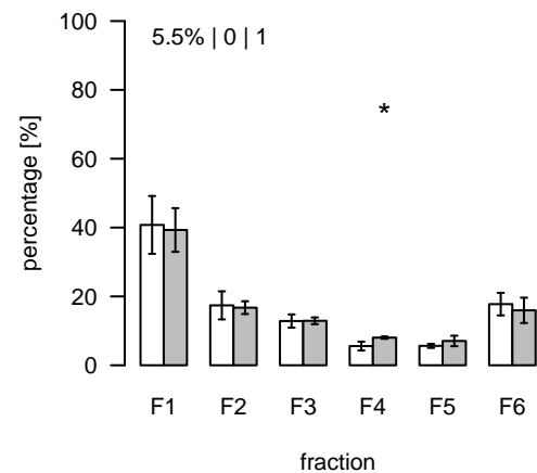
S596 (m/z=690.437074; rt=14.51024) T/S Cluster: S-14.5-4
