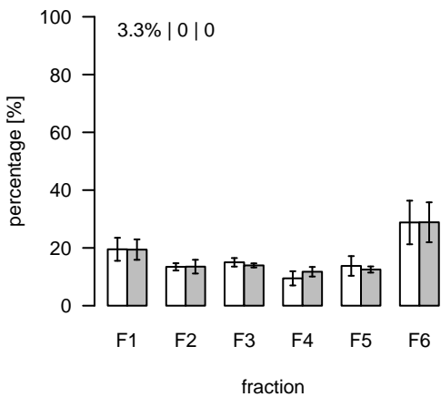
S379 (m/z=752.446382; rt=12.22445) T/S Cluster: S-12.2-9
