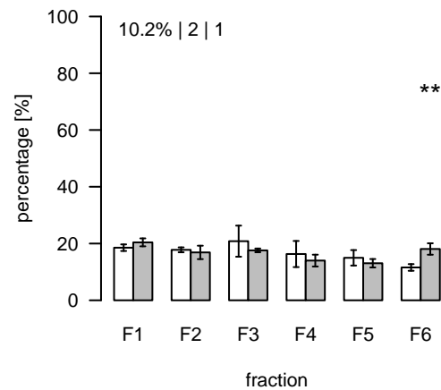
L2690 (m/z=878.820353; rt=16.06301) T/S Cluster: L-16.1-1
