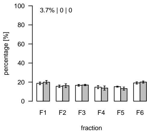
S520 (m/z=299.050765; rt=13.23219) T/S Cluster: S-13.2-4
