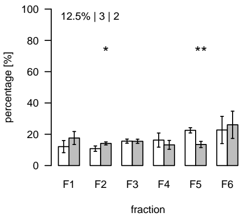
L1063 (m/z=806.561732; rt=6.54756) T/S Cluster: L-6.5-9
