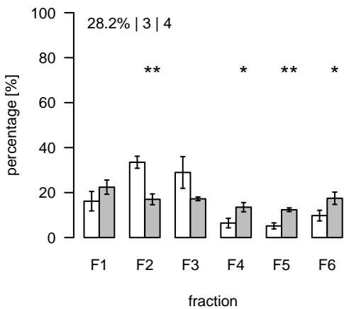
S106 (m/z=823.790996; rt=4.77803) T/S Cluster: S-4.8-2
