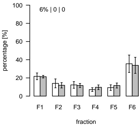
S251 (m/z=608.356404; rt=7.49364) T/S Cluster: S-7.5-1
