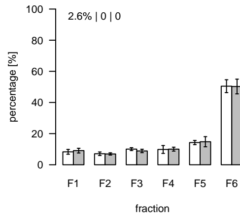
L538 (m/z=783.537361; rt=4.81341) T/S Cluster: L-4.8-10
