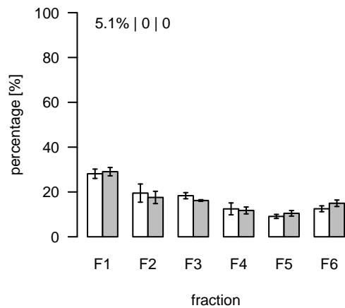
L1485 (m/z=358.792133; rt=7.93903) T/S Cluster: L-7.9-13
