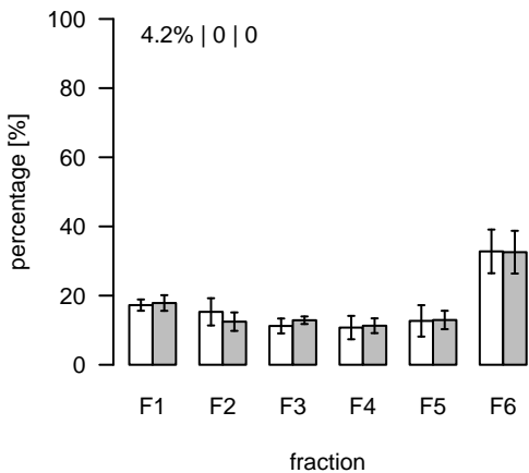
L721 (m/z=790.565777; rt=5.23257) T/S Cluster: L-5.2-5
