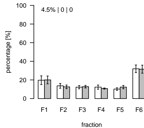
S416 (m/z=702.37831; rt=12.5375) T/S Cluster: S-12.5-8
