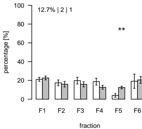
S908 (m/z=823.711869; rt=18.53472) T/S Cluster: S-18.5-3
