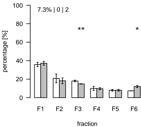
S133 (m/z=214.089921; rt=5.70086) T/S Cluster: S-5.7-1
