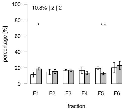
L2572 (m/z=949.288889; rt=15.36437) T/S Cluster: L-15.4-3
