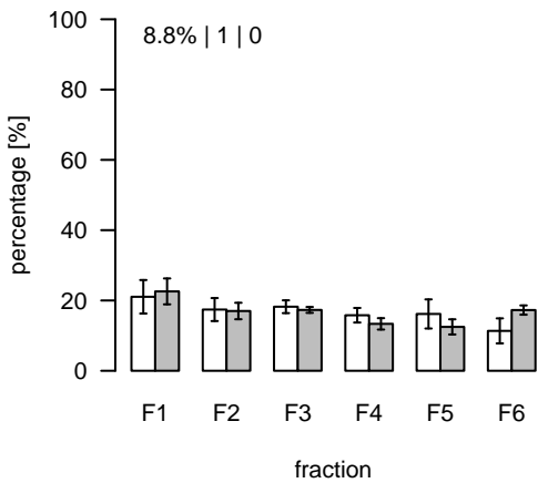
L974 (m/z=796.529682; rt=6.19047) T/S Cluster: L-6.2-7
