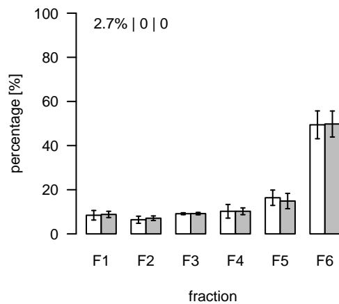
L1656 (m/z=937.66167; rt=8.64251) T/S Cluster: L-8.6-6
