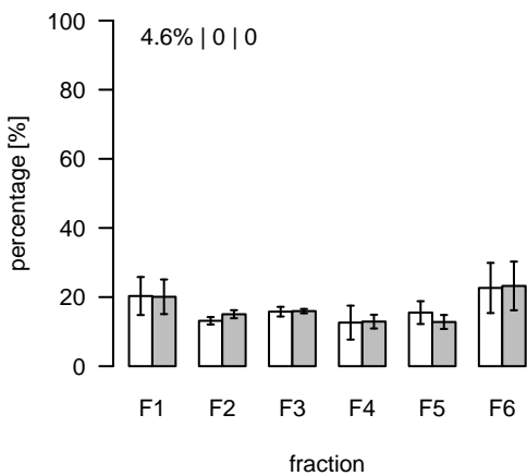
L1196 (m/z=389.272583; rt=6.66701) T/S Cluster: L-6.7-8
