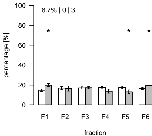
L2257 (m/z=751.528498; rt=11.32756) T/S Cluster: L-11.3-13
