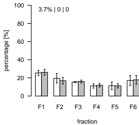
L790 (m/z=789.551303; rt=5.43732) T/S Cluster: L-5.4-5
