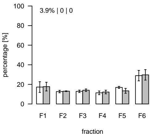
L131 (m/z=844.51624; rt=3.65103) T/S Cluster: L-3.7-1
