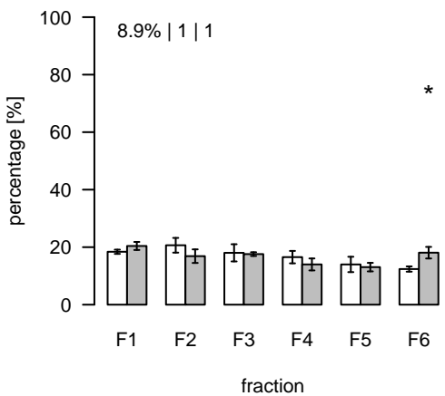
L2708 (m/z=892.836476; rt=16.17521) T/S Cluster: L-16.2-4
