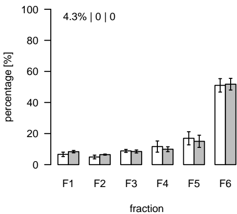
L712 (m/z=786.48602; rt=5.22187) T/S Cluster: L-5.2-4
