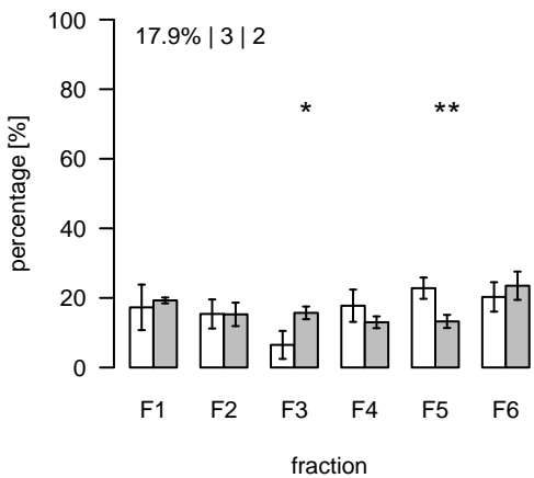
S286 (m/z=437.727472; rt=8.56096) T/S Cluster: S-8.6-1
