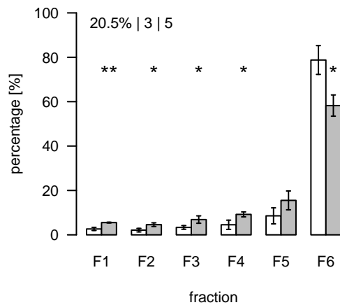
L1214 (m/z=765.536437; rt=6.77162) T/S Cluster: L-6.8-1
