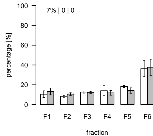
L1156 (m/z=614.492777; rt=6.65418) T/S Cluster: L-6.7-3
