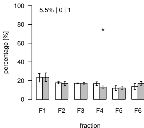
L1480 (m/z=379.28644; rt=7.93884) T/S Cluster: L-7.9-14
