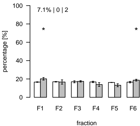
S13 (m/z=437.74301; rt=1.28657) T/S Cluster: S-1.3-2
