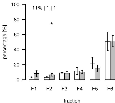
L2201 (m/z=894.48373; rt=10.91697) T/S Cluster: L-10.9-2
