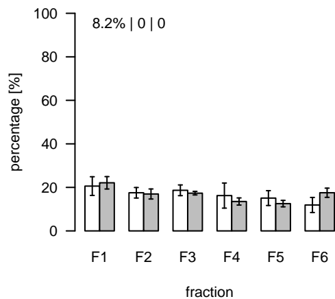
L1023 (m/z=798.534167; rt=6.52481) T/S Cluster: L-6.5-3
