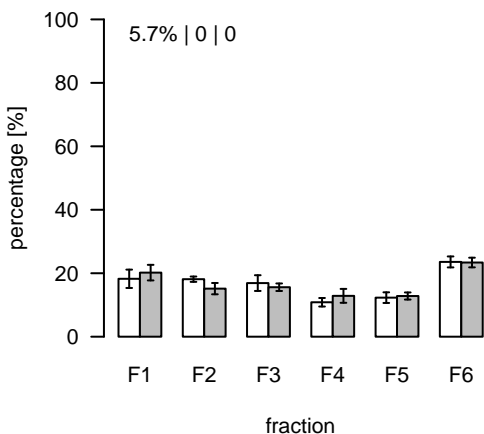
S571 (m/z=323.220665; rt=14.23897) T/S Cluster: S-14.2-3
