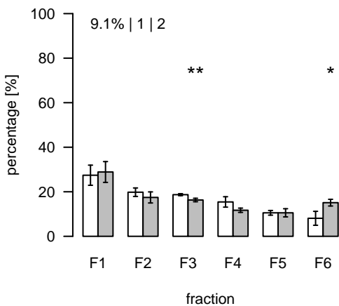
L1679 (m/z=380.791609; rt=8.70676) T/S Cluster: L-8.7-5
