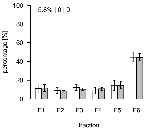
L2216 (m/z=886.533728; rt=11.02704) T/S Cluster: L-11-2
