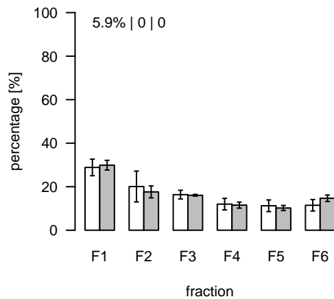
L452 (m/z=790.543574; rt=4.57147) T/S Cluster: L-4.6-1
