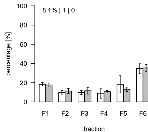
L252 (m/z=326.373085; rt=3.94277) T/S Cluster: L-3.9-9
