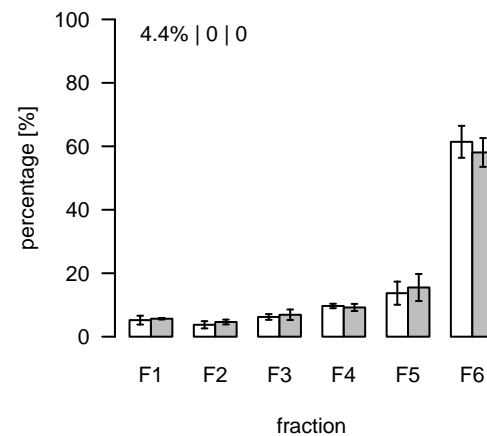
L548 (m/z=778.566698; rt=4.83544) T/S Cluster: L-4.8-10
