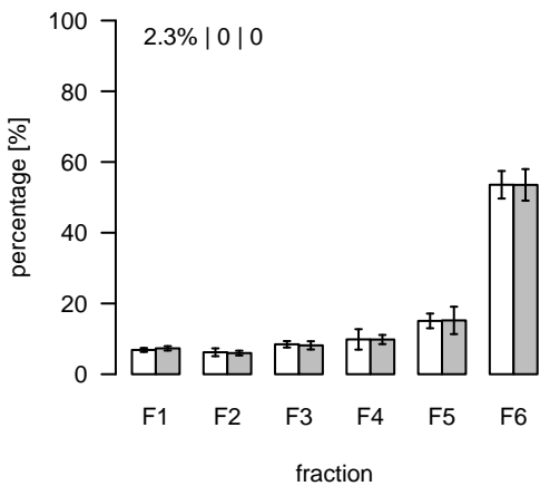
L838 (m/z=474.316668; rt=5.70357) T/S Cluster: L-5.7-1
