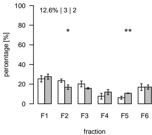
S674 (m/z=823.770988; rt=15.11552) T/S Cluster: S-15.1-1
