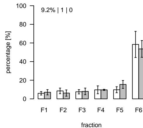
L16 (m/z=813.522831; rt=2.60859) T/S Cluster: L-2.6-1
