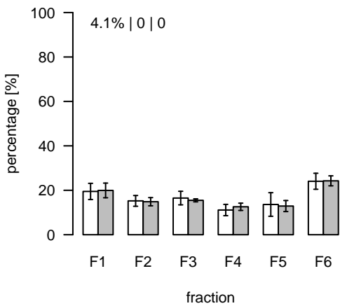
L311 (m/z=810.535032; rt=4.18448) T/S Cluster: L-4.2-7
