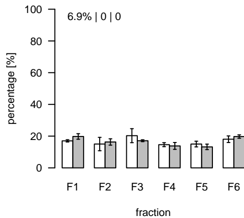
L1433 (m/z=391.283354; rt=7.89661) T/S Cluster: L-7.9-8
