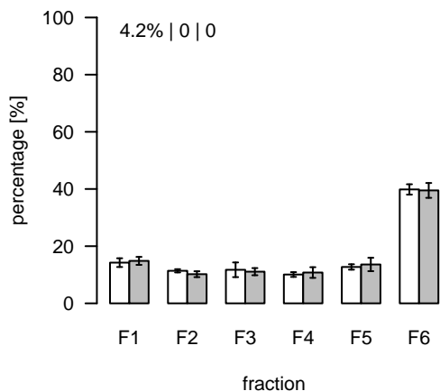
S383 (m/z=635.349453; rt=12.24472) T/S Cluster: S-12.2-12
