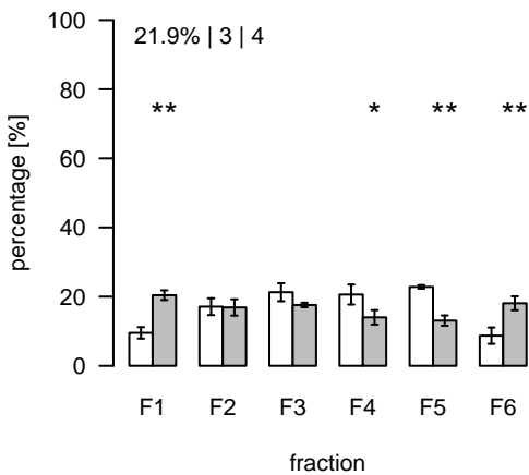
L2350 (m/z=1349.909259; rt=11.32854) T/S Cluster: L-11.3-2
