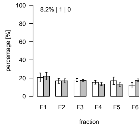
L967 (m/z=796.549956; rt=6.1899) T/S Cluster: L-6.2-7
