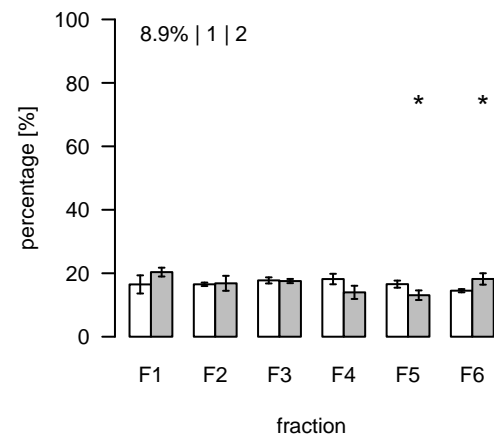
L2803 (m/z=1192.1306; rt=18.4148) T/S Cluster: L-18.4-1
