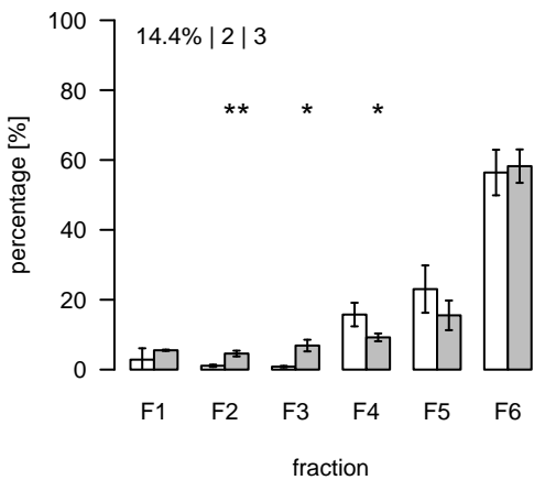
L169 (m/z=847.517056; rt=3.67854) T/S Cluster: L-3.7-17
