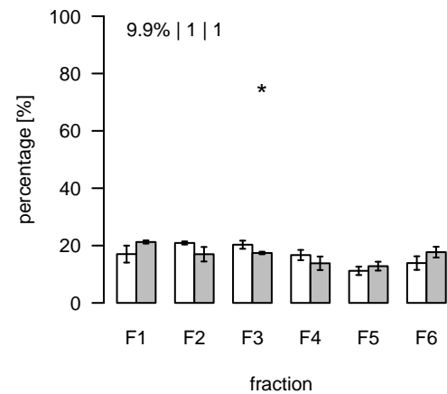
S189 (m/z=1212.317595; rt=6.58682) T/S Cluster: S-6.6-3
