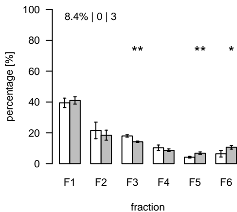
S229 (m/z=290.5894; rt=7.19631) T/S Cluster: S-7.2-2
