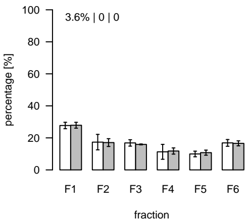
L1265 (m/z=732.565721; rt=7.16426) T/S Cluster: L-7.2-1
