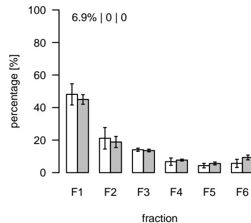
S107 (m/z=699.199053; rt=4.90916) T/S Cluster: S-4.9-1
