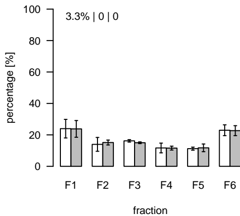
L2496 (m/z=828.695897; rt=12.50723) T/S Cluster: L-12.5-1
