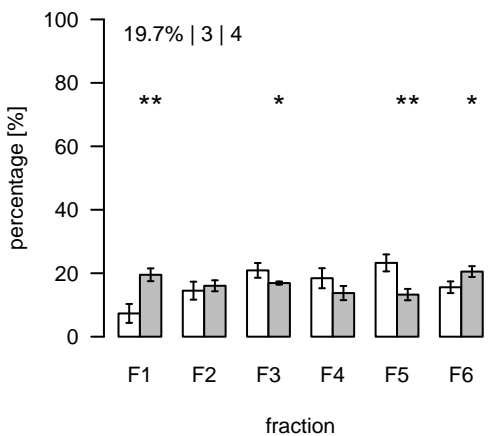
L2351 (m/z=1342.943031; rt=11.32855) T/S Cluster: L-11.3-4
