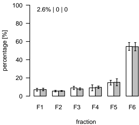
L630 (m/z=485.306997; rt=4.94296) T/S Cluster: L-4.9-9
