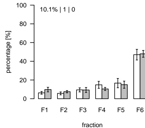
L1729 (m/z=896.531541; rt=8.7428) T/S Cluster: L-8.7-8
