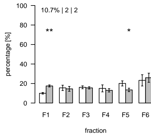
L2529 (m/z=760.227771; rt=14.00421) T/S Cluster: L-14-1
