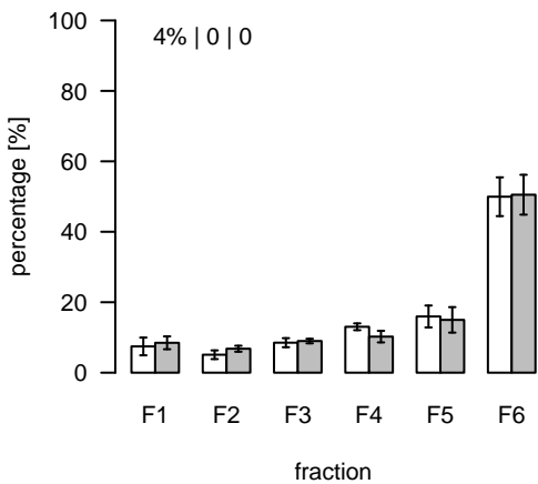
L1343 (m/z=794.538988; rt=7.34733) T/S Cluster: L-7.3-3
