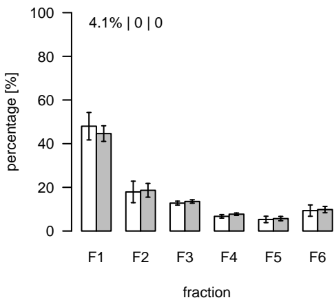
S41 (m/z=483.122906; rt=4.05862) T/S Cluster: S-4.1-2
