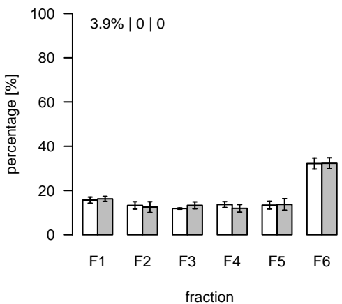
L2450 (m/z=291.196179; rt=11.84605) T/S Cluster: L-11.8-5
