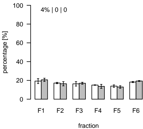
S519 (m/z=300.042948; rt=13.23151) T/S Cluster: S-13.2-5
