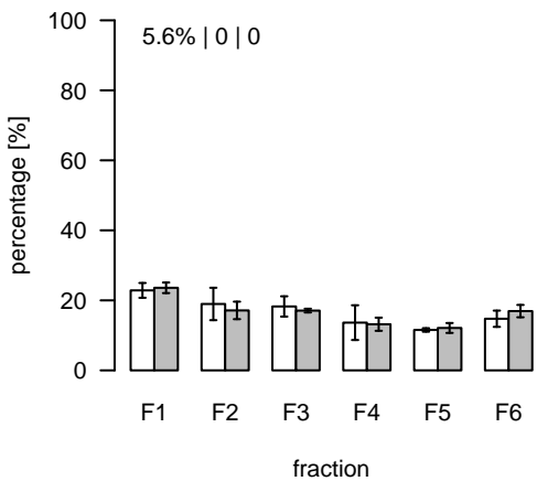
L2439 (m/z=682.637905; rt=11.74877) T/S Cluster: L-11.7-3
