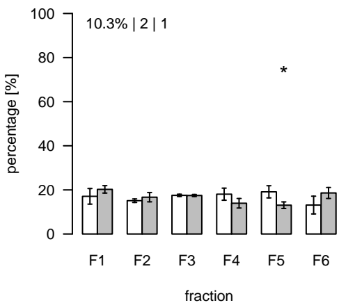
L1427 (m/z=938.562162; rt=7.88639) T/S Cluster: L-7.9-4
