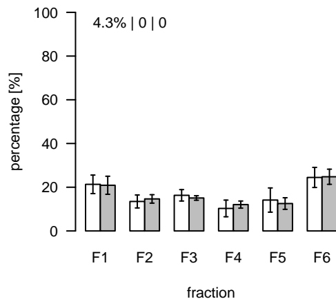
L891 (m/z=770.512297; rt=5.83664) T/S Cluster: L-5.8-5
