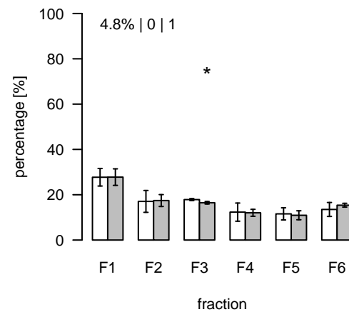
L377 (m/z=838.494291; rt=4.37985) T/S Cluster: L-4.4-7
