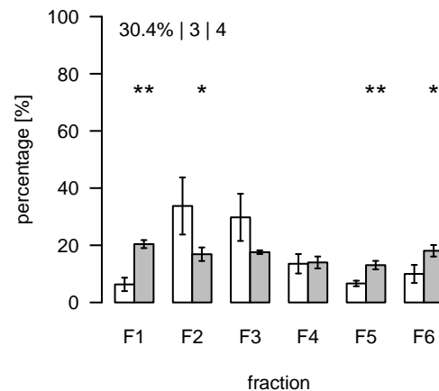
S876 (m/z=575.505854; rt=16.99119) T/S Cluster: S-17-12
