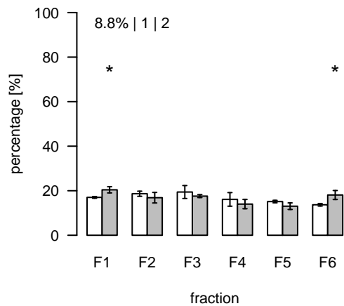
L2622 (m/z=836.773468; rt=15.70573) T/S Cluster: L-15.7-1
