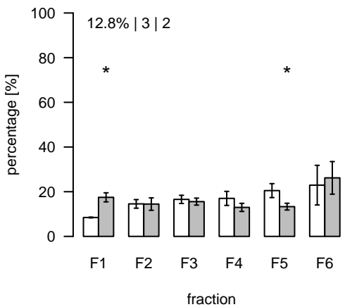
L2765 (m/z=1243.369687; rt=16.96444) T/S Cluster: L-17-1
