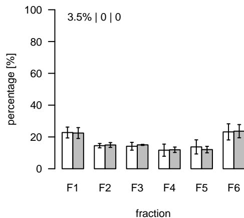
L1600 (m/z=756.556074; rt=8.28772) T/S Cluster: L-8.3-1
