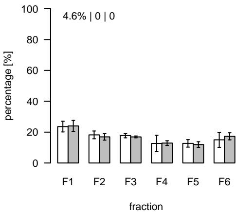
L1475 (m/z=758.567863; rt=7.93877) T/S Cluster: L-7.9-14
