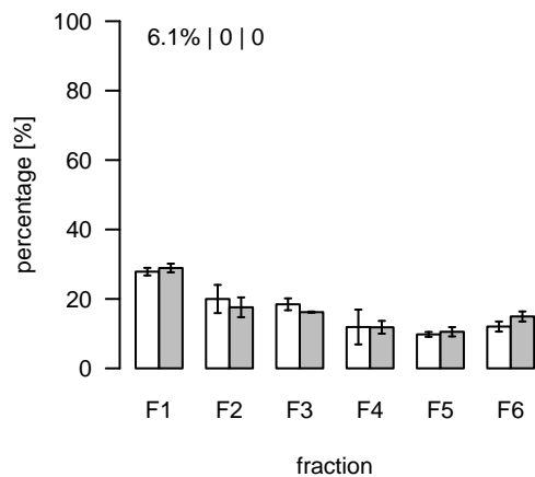
L1500 (m/z=358.284075; rt=7.93941) T/S Cluster: L-7.9-13
