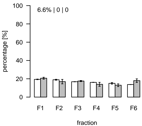
L2703 (m/z=996.339399; rt=16.1563) T/S Cluster: L-16.2-1
