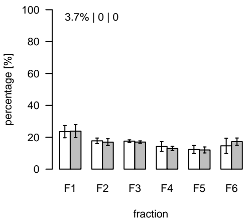
L1472 (m/z=252.858794; rt=7.93866) T/S Cluster: L-7.9-14
