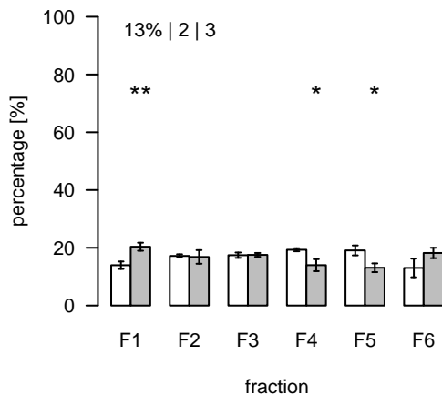
L2371 (m/z=342.719049; rt=11.32878) T/S Cluster: L-11.3-15
