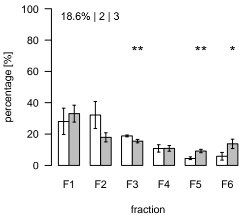
S880 (m/z=714.509132; rt=16.99751) T/S Cluster: S-17-14
