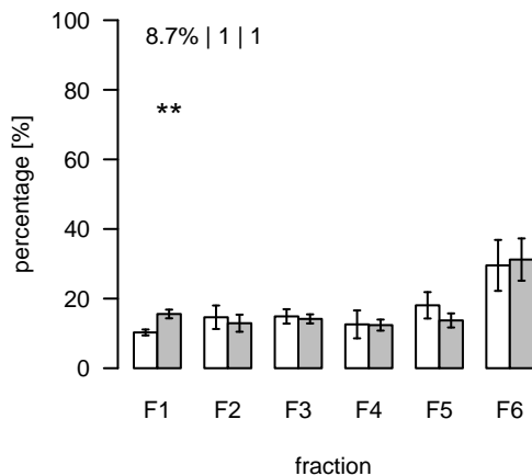
L2498 (m/z=342.103516; rt=12.7659) T/S Cluster: L-12.8-1
