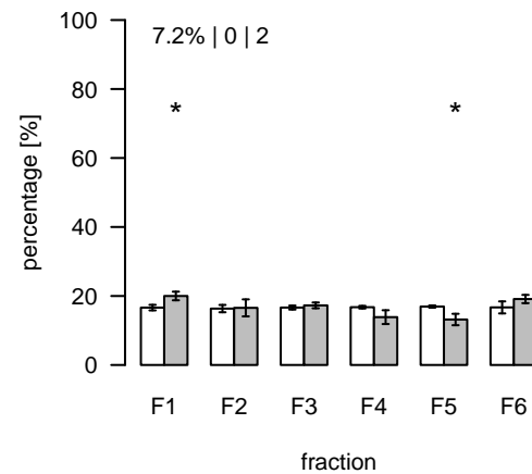
S12 (m/z=437.771517; rt=1.26495) T/S Cluster: S-1.3-1
