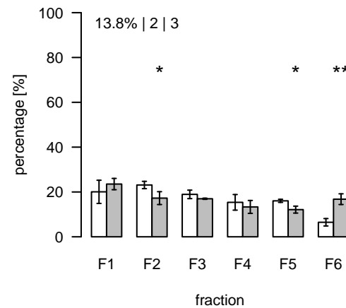
L1665 (m/z=391.286526; rt=8.6978) T/S Cluster: L-8.7-3
