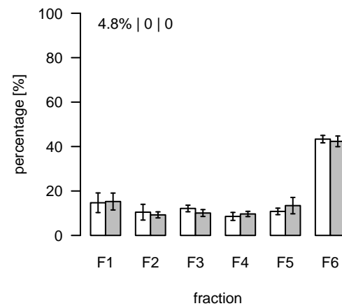
S314 (m/z=775.381896; rt=9.99427) T/S Cluster: S-10-2
