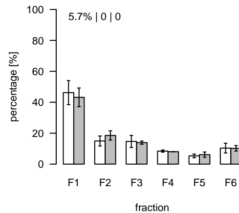
S241 (m/z=506.167432; rt=7.24815) T/S Cluster: S-7.2-2
