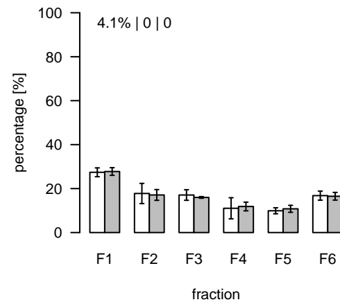
L1259 (m/z=734.558029; rt=7.16398) T/S Cluster: L-7.2-1
