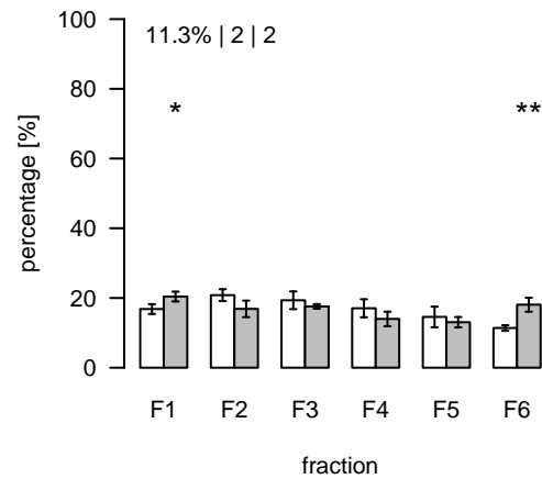
L2599 (m/z=835.76125; rt=15.47115) T/S Cluster: L-15.5-2
