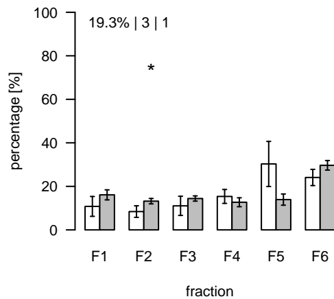
L1125 (m/z=417.278674; rt=6.63271) T/S Cluster: L-6.6-12
