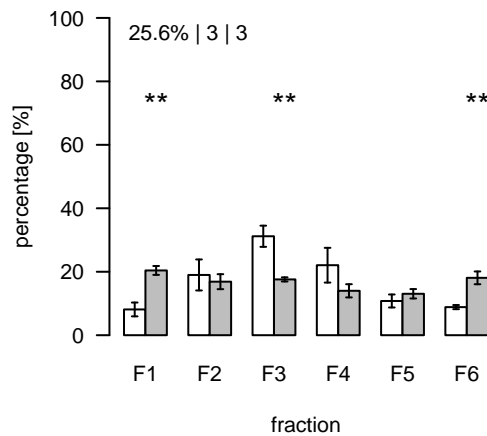
S899 (m/z=222.295543; rt=17.44805) T/S Cluster: S-17.4-2
