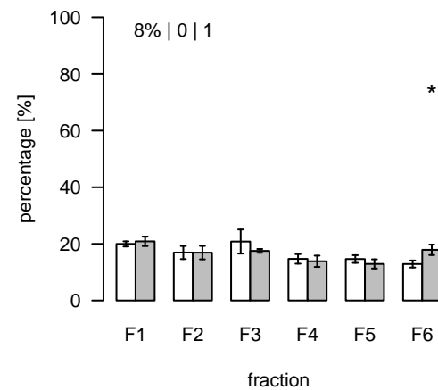
L2730 (m/z=880.83559; rt=16.28646) T/S Cluster: L-16.3-3
