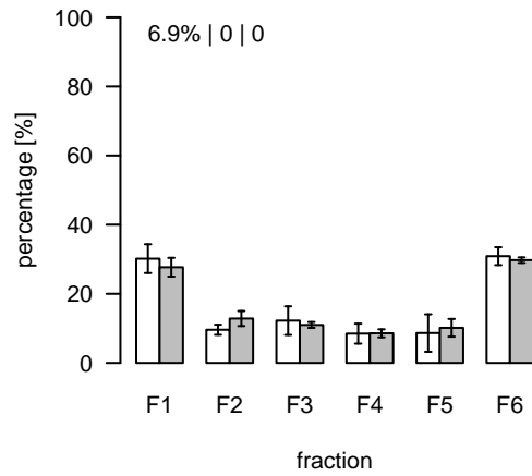
S235 (m/z=547.319702; rt=7.20005) T/S Cluster: S-7.2-1
