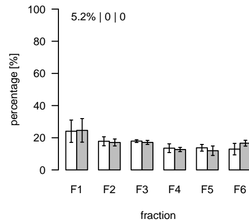
L1966 (m/z=808.587079; rt=9.82783) T/S Cluster: L-9.8-1
