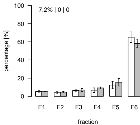
L46 (m/z=702.445824; rt=3.2722) T/S Cluster: L-3.3-1
