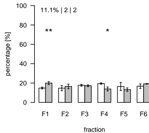
L2497 (m/z=437.746443; rt=12.52308) T/S Cluster: L-12.5-2
