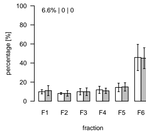
L1585 (m/z=924.524549; rt=8.19978) T/S Cluster: L-8.2-3
