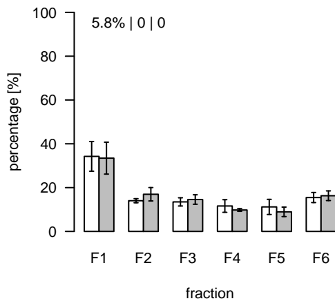
S35 (m/z=214.089763; rt=4.05278) T/S Cluster: S-4.1-1
