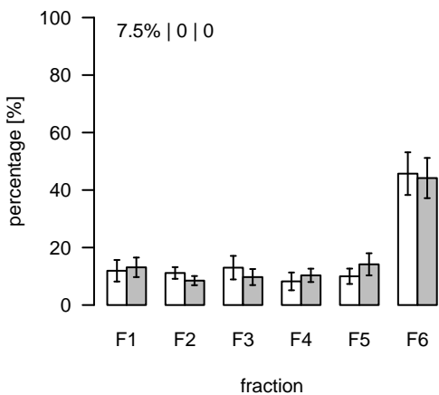
L4 (m/z=415.209739; rt=1.36442) T/S Cluster: L-1.4-1
