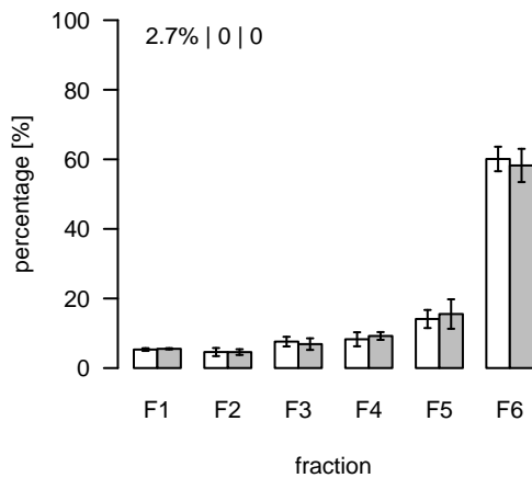
L743 (m/z=971.619662; rt=5.30886) T/S Cluster: L-5.3-5
