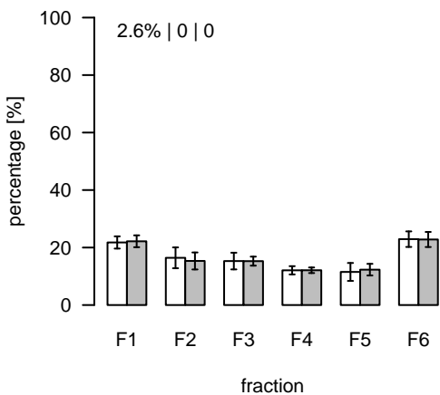
L489 (m/z=789.550473; rt=4.72916) T/S Cluster: L-4.7-1
