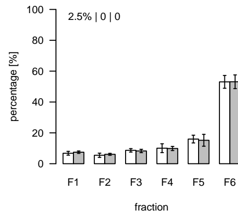
L615 (m/z=968.557067; rt=4.91145) T/S Cluster: L-4.9-9
