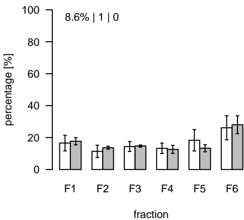
L1606 (m/z=934.569132; rt=8.3706) T/S Cluster: L-8.4-1
