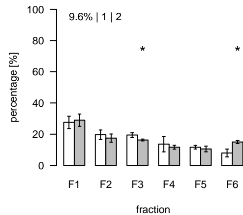
L1687 (m/z=761.556019; rt=8.70695) T/S Cluster: L-8.7-5
