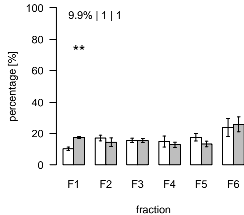
L2573 (m/z=454.132165; rt=15.36452) T/S Cluster: L-15.4-3
