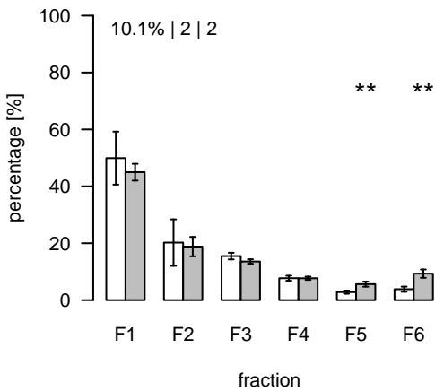
S171 (m/z=1207.36308; rt=6.57759) T/S Cluster: S-6.6-2
