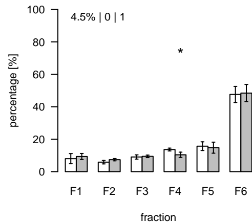
L1346 (m/z=614.48004; rt=7.34755) T/S Cluster: L-7.3-3
