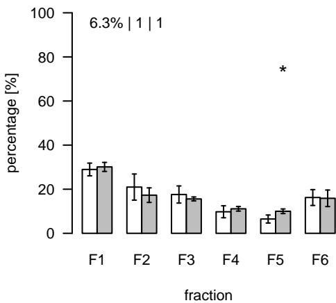
S328 (m/z=655.330428; rt=10.14866) T/S Cluster: S-10.1-1
