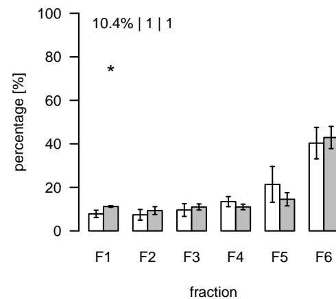
L1662 (m/z=926.509583; rt=8.65451) T/S Cluster: L-8.7-1
