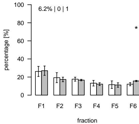
L211 (m/z=704.425208; rt=3.81637) T/S Cluster: L-3.8-7
