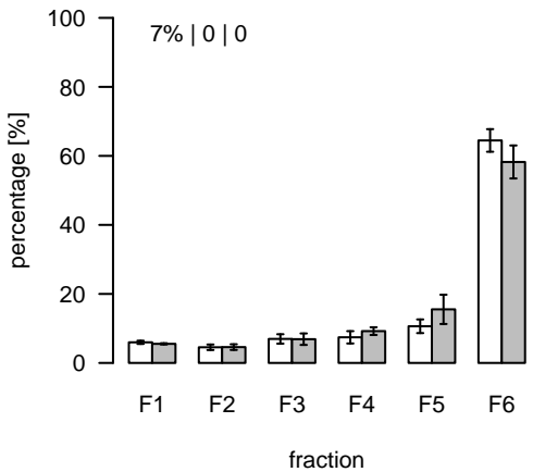
L2181 (m/z=953.594068; rt=10.68831) T/S Cluster: L-10.7-2
