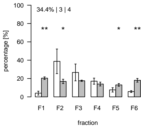
S881 (m/z=716.525504; rt=16.99825) T/S Cluster: S-17-15
