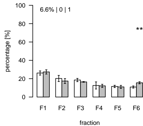
L2138 (m/z=817.642509; rt=10.58553) T/S Cluster: L-10.6-2
