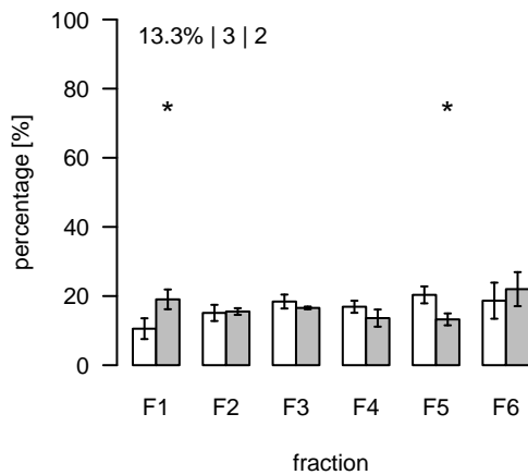
L2277 (m/z=681.486801; rt=11.32778) T/S Cluster: L-11.3-4
