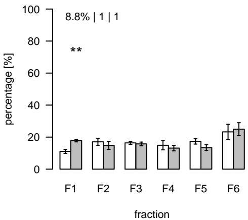
L2758 (m/z=1128.326137; rt=16.54791) T/S Cluster: L-16.5-6
