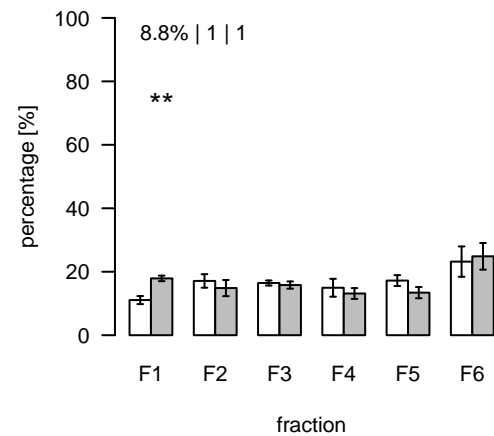
L2759 (m/z=1128.276334; rt=16.54795) T/S Cluster: L-16.5-6
