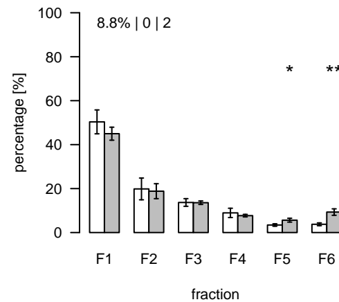
S108 (m/z=698.195742; rt=4.90929) T/S Cluster: S-4.9-1
