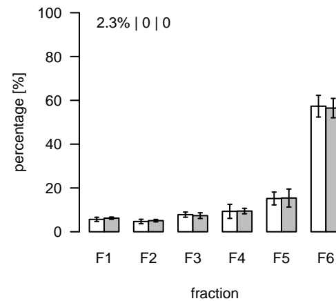
L585 (m/z=970.561489; rt=4.8976) T/S Cluster: L-4.9-9
