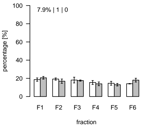
L2624 (m/z=862.788662; rt=15.72817) T/S Cluster: L-15.7-2
