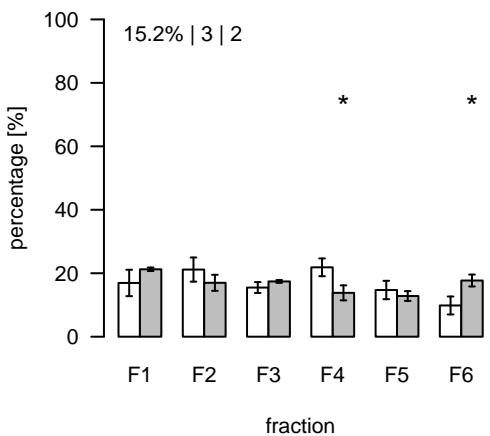
L2443 (m/z=895.568809; rt=11.82929) T/S Cluster: L-11.8-3
