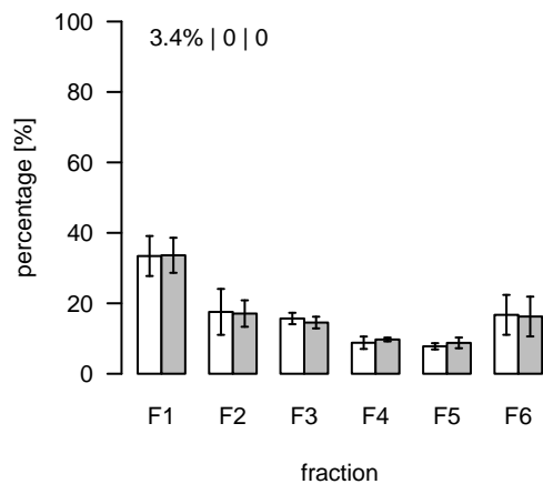
S327 (m/z=654.327051; rt=10.14652) T/S Cluster: S-10.1-1
