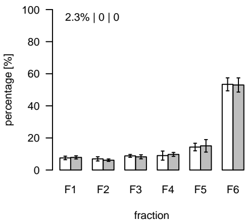
L924 (m/z=951.627282; rt=6.10912) T/S Cluster: L-6.1-1
