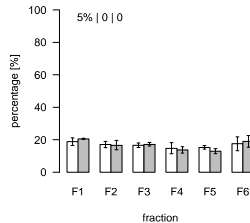
L992 (m/z=399.285022; rt=6.28332) T/S Cluster: L-6.3-3
