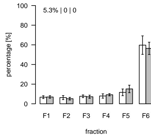
L937 (m/z=786.576653; rt=6.12744) T/S Cluster: L-6.1-1
