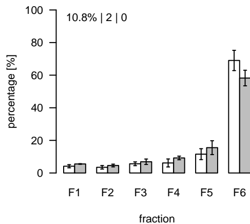
L420 (m/z=752.498548; rt=4.44469) T/S Cluster: L-4.4-2
