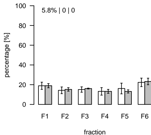
L895 (m/z=796.554231; rt=5.8725) T/S Cluster: L-5.9-2
