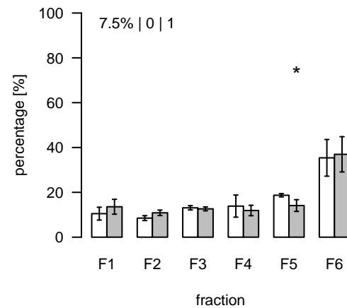
L1162 (m/z=613.47575; rt=6.65426) T/S Cluster: L-6.7-3
