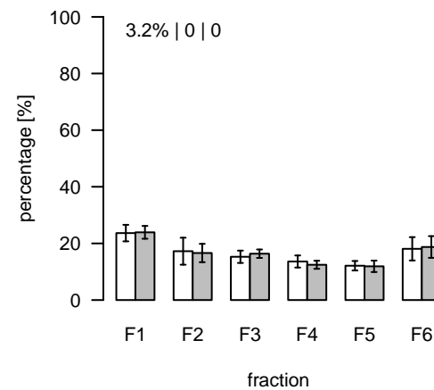
L657 (m/z=827.52213; rt=5.01227) T/S Cluster: L-5-4
