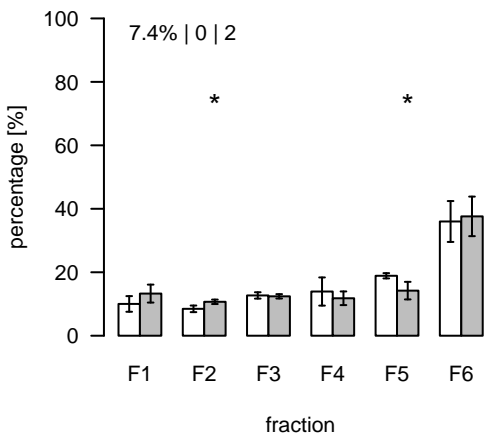
L1157 (m/z=318.54716; rt=6.65419) T/S Cluster: L-6.7-3
