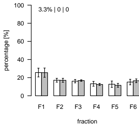
L1956 (m/z=788.588492; rt=9.82699) T/S Cluster: L-9.8-1
