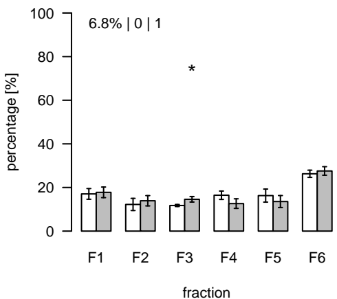
L2489 (m/z=893.537005; rt=12.38802) T/S Cluster: L-12.4-4
