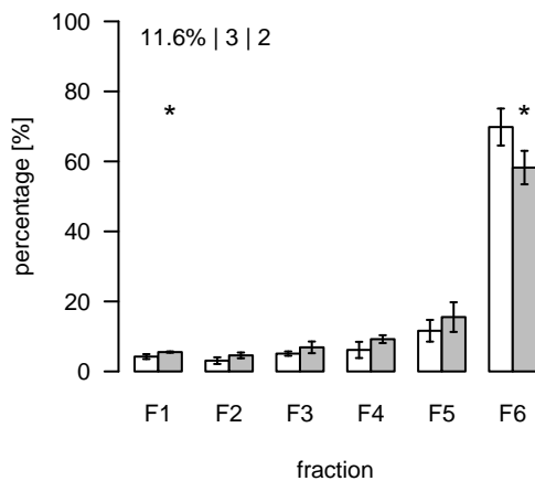
L1274 (m/z=766.549827; rt=7.18897) T/S Cluster: L-7.2-3
