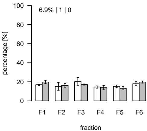
L1434 (m/z=391.286679; rt=7.8975) T/S Cluster: L-7.9-8
