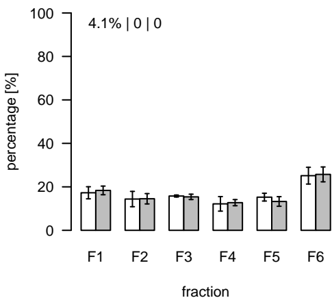
L474 (m/z=815.567381; rt=4.64622) T/S Cluster: L-4.6-10
