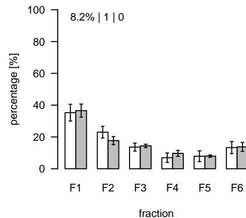
S704 (m/z=809.576754; rt=15.51047) T/S Cluster: S-15.5-1
