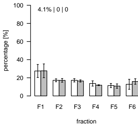
L1623 (m/z=770.55412; rt=8.48315) T/S Cluster: L-8.5-3
