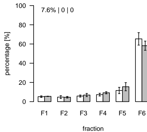
L650 (m/z=781.477537; rt=4.95317) T/S Cluster: L-5-1
