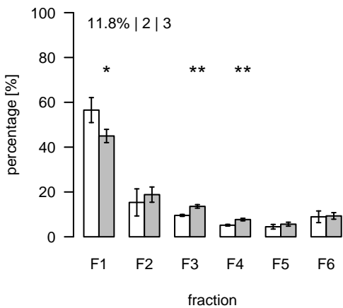
S16 (m/z=469.099402; rt=1.60204) T/S Cluster: S-1.6-1
