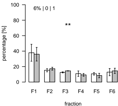
S154 (m/z=742.230501; rt=5.97411) T/S Cluster: S-6-2
