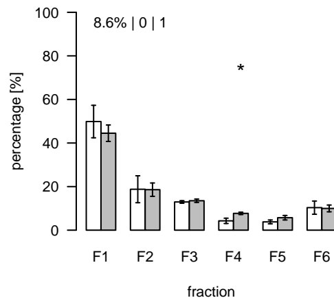
S638 (m/z=680.451106; rt=14.86026) T/S Cluster: S-14.9-2
