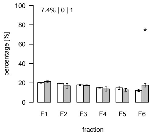
L2553 (m/z=775.275836; rt=14.97086) T/S Cluster: L-15-1
