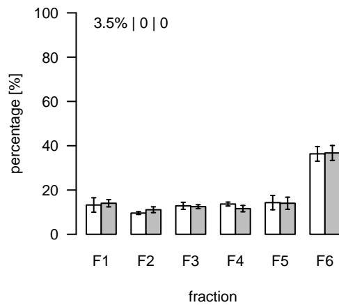
L261 (m/z=738.4612; rt=3.98668) T/S Cluster: L-4-5
