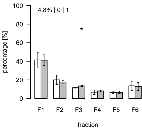
S540 (m/z=708.446992; rt=13.57372) T/S Cluster: S-13.6-1
