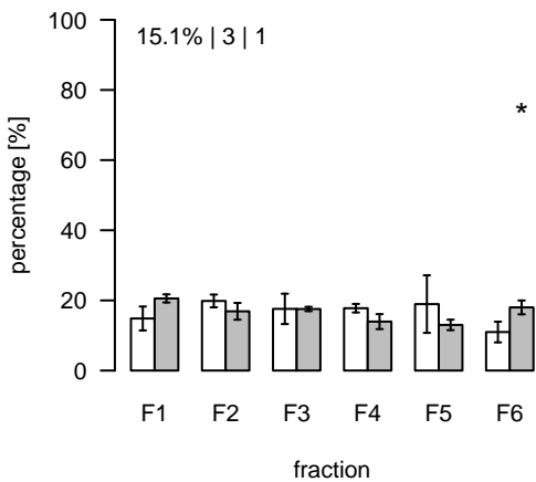
L1107 (m/z=388.345121; rt=6.56953) T/S Cluster: L-6.6-3
