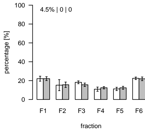
S400 (m/z=734.393512; rt=12.39435) T/S Cluster: S-12.4-6
