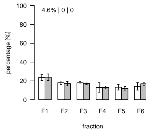
L1503 (m/z=252.519585; rt=7.93977) T/S Cluster: L-7.9-14
