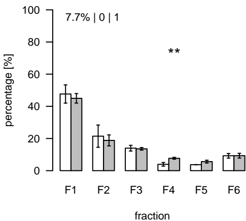
S626 (m/z=653.424876; rt=14.77945) T/S Cluster: S-14.8-2
