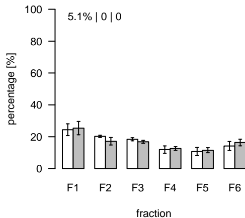
L1308 (m/z=802.539717; rt=7.32574) T/S Cluster: L-7.3-7
