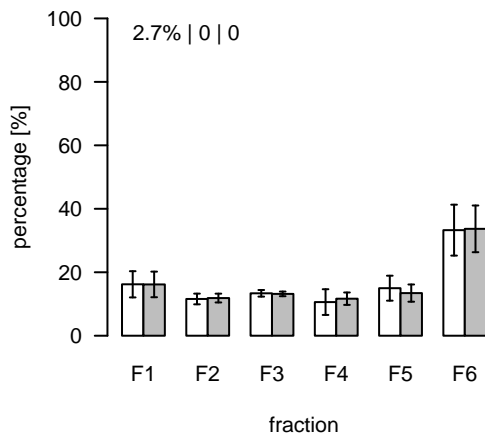
L733 (m/z=796.553455; rt=5.28739) T/S Cluster: L-5.3-1
