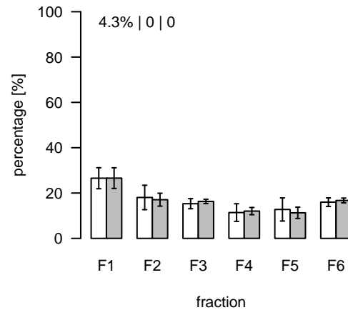
L2183 (m/z=788.62321; rt=10.74725) T/S Cluster: L-10.7-3
