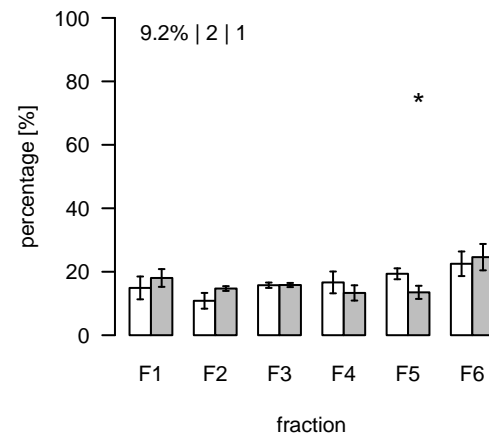
L1432 (m/z=953.614044; rt=7.89403) T/S Cluster: L-7.9-7
