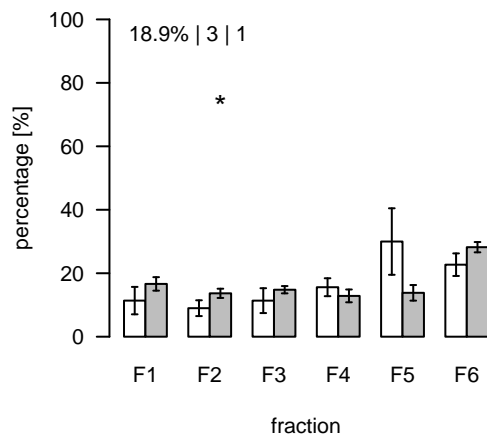
L1124 (m/z=834.519532; rt=6.6325) T/S Cluster: L-6.6-12
