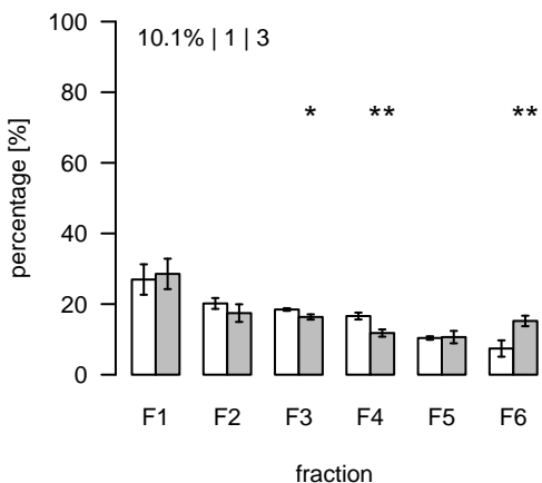
L1689 (m/z=379.774712; rt=8.70702) T/S Cluster: L-8.7-5
