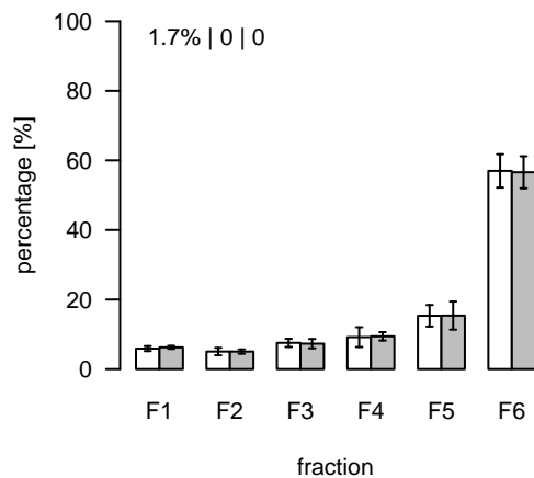
L576 (m/z=972.623201; rt=4.89637) T/S Cluster: L-4.9-9
