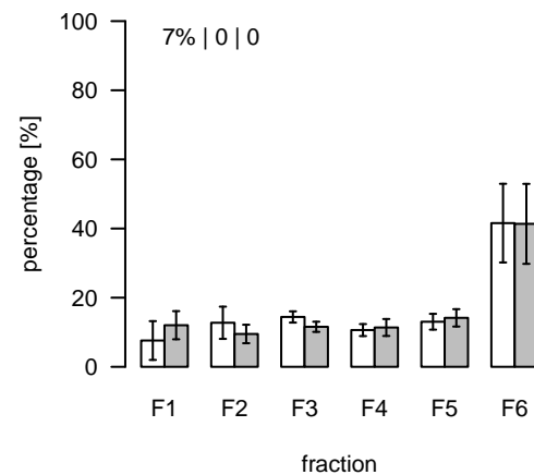
L1987 (m/z=923.554724; rt=10.03938) T/S Cluster: L-10-4
