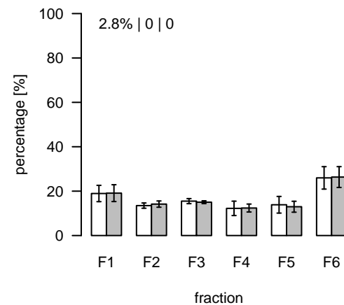
L861 (m/z=774.558863; rt=5.71565) T/S Cluster: L-5.7-4
