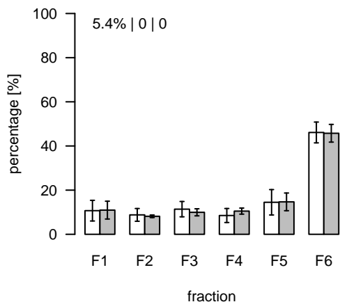
L2217 (m/z=886.56205; rt=11.02721) T/S Cluster: L-11-2
