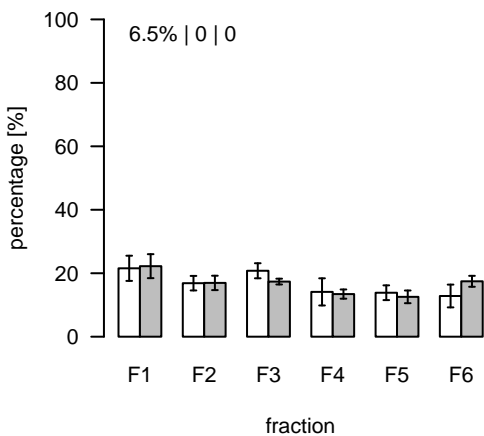
L1025 (m/z=799.554736; rt=6.52714) T/S Cluster: L-6.5-3
