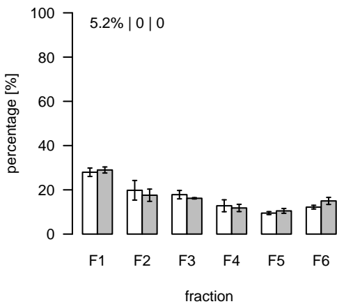
L1497 (m/z=238.861499; rt=7.93927) T/S Cluster: L-7.9-13
