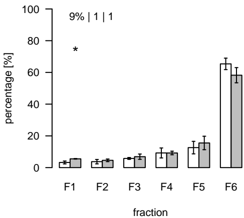
L2125 (m/z=446.272203; rt=10.50817) T/S Cluster: L-10.5-11
