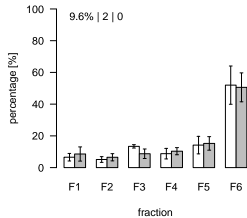
L1865 (m/z=453.770089; rt=9.43512) T/S Cluster: L-9.4-1
