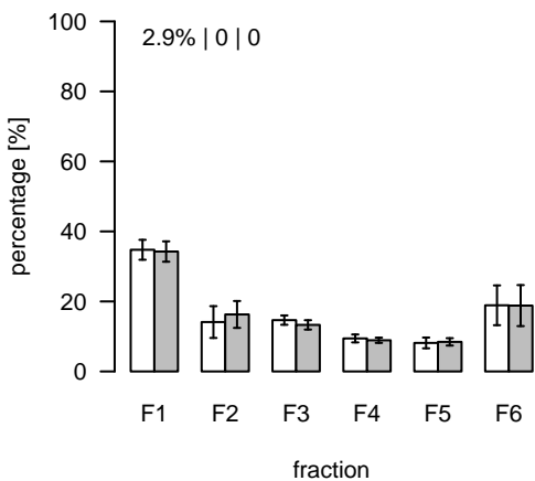
S309 (m/z=612.317534; rt=9.78218) T/S Cluster: S-9.8-1
