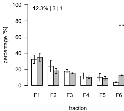
L161 (m/z=668.423692; rt=3.67491) T/S Cluster: L-3.7-14
