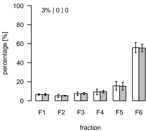
L529 (m/z=583.423061; rt=4.80981) T/S Cluster: L-4.8-10
