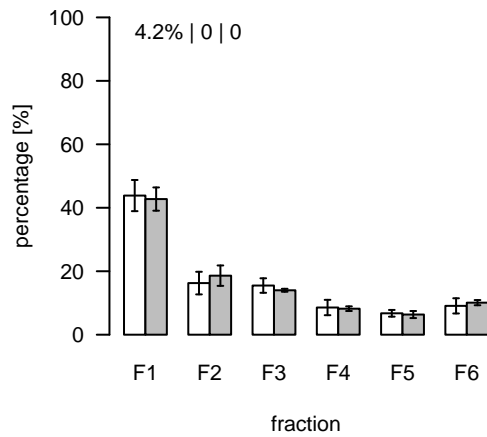
S158 (m/z=700.284163; rt=6.07869) T/S Cluster: S-6.1-1
