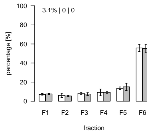
L933 (m/z=685.465203; rt=6.12643) T/S Cluster: L-6.1-1
