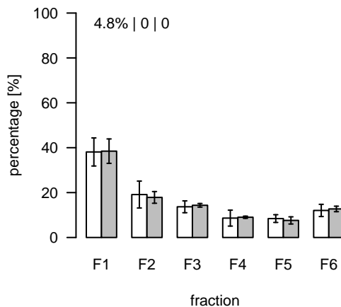
S607 (m/z=822.553074; rt=14.63054) T/S Cluster: S-14.6-1
