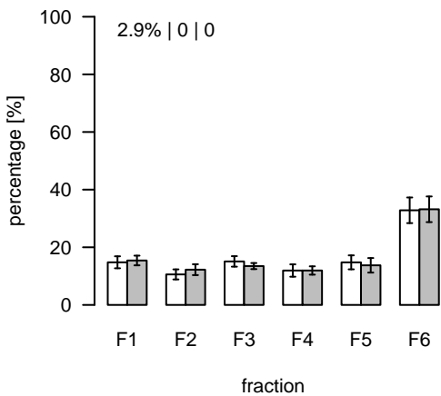
L722 (m/z=398.271569; rt=5.24916) T/S Cluster: L-5.2-8
