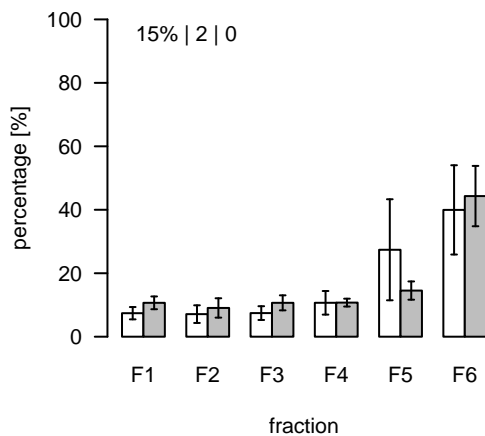
L1663 (m/z=925.53108; rt=8.68542) T/S Cluster: L-8.7-1
