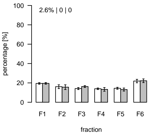
S466 (m/z=666.496271; rt=12.90916) T/S Cluster: S-12.9-4
