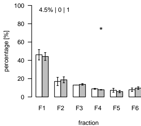
S36 (m/z=485.116158; rt=4.05656) T/S Cluster: S-4.1-2
