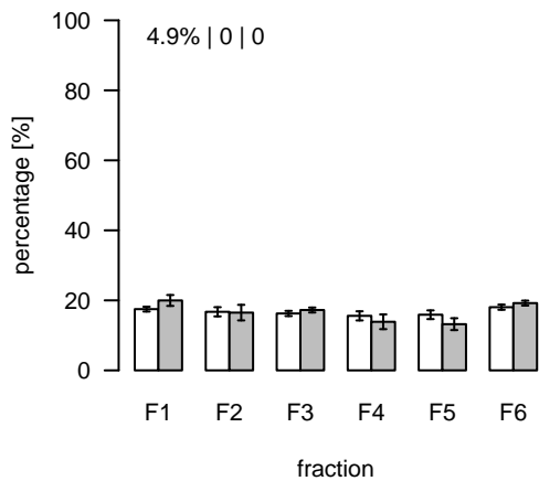
S490 (m/z=308.230632; rt=12.91259) T/S Cluster: S-12.9-19
