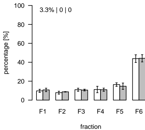
L2059 (m/z=780.571324; rt=10.38554) T/S Cluster: L-10.4-1
