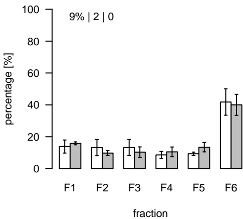
S862 (m/z=743.488757; rt=16.97627) T/S Cluster: S-17-3
