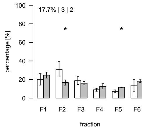
S873 (m/z=774.565713; rt=16.98635) T/S Cluster: S-17-9
