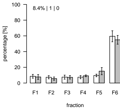
L1630 (m/z=903.569045; rt=8.55883) T/S Cluster: L-8.6-2
