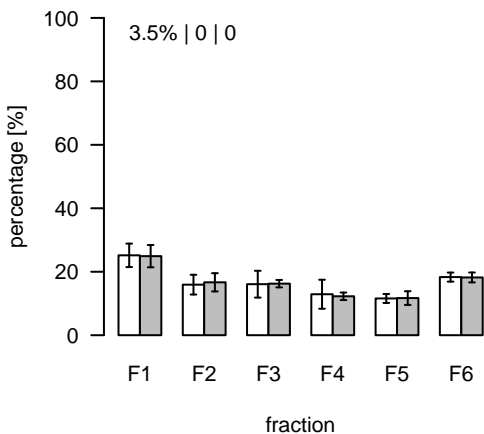
S394 (m/z=718.395347; rt=12.35006) T/S Cluster: S-12.4-1
