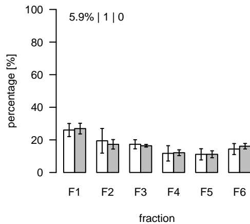
L440 (m/z=806.558876; rt=4.52927) T/S Cluster: L-4.5-3
