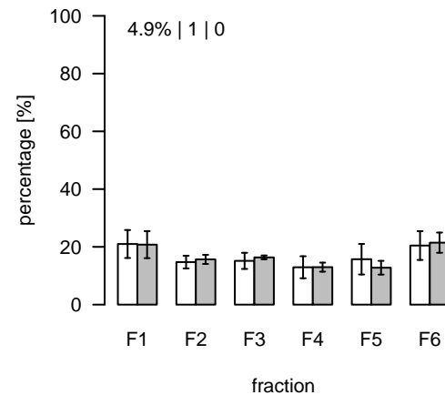
L1294 (m/z=800.550555; rt=7.28624) T/S Cluster: L-7.3-4
