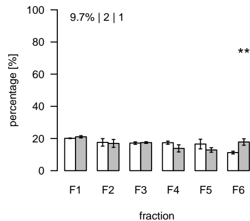
L2241 (m/z=391.28595; rt=11.32357) T/S Cluster: L-11.3-10
