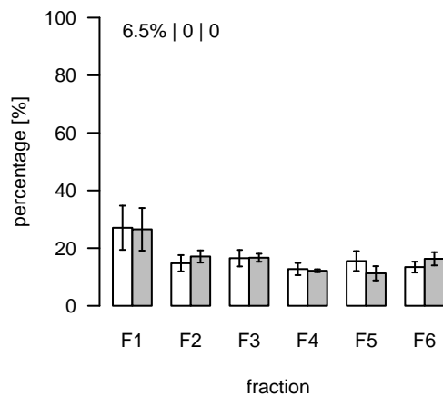
L915 (m/z=834.545491; rt=5.9447) T/S Cluster: L-5.9-6
