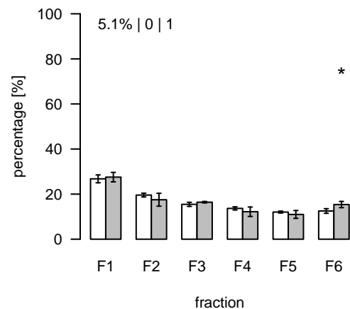
L2251 (m/z=710.508794; rt=11.32746) T/S Cluster: L-11.3-11
