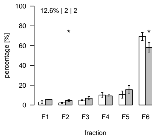
L1942 (m/z=891.531148; rt=9.64419) T/S Cluster: L-9.6-1
