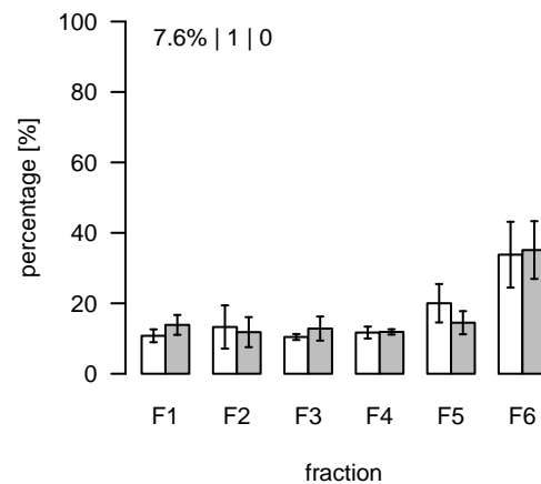
L619 (m/z=987.614556; rt=4.9171) T/S Cluster: L-4.9-2
