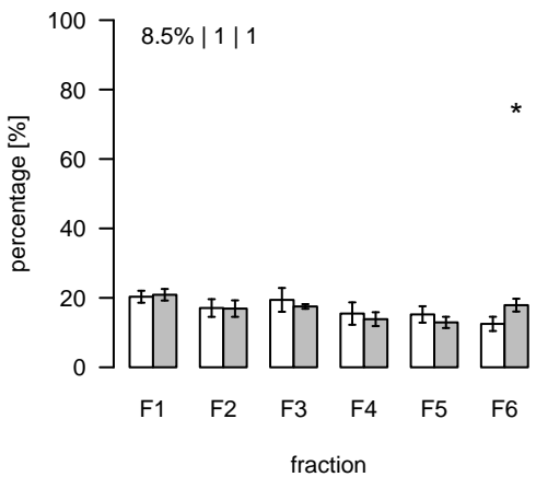
L2612 (m/z=876.800256; rt=15.589) T/S Cluster: L-15.6-1
