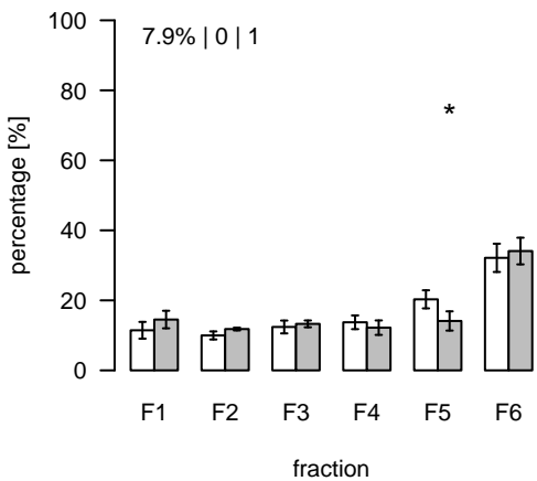
L1856 (m/z=915.606045; rt=9.34536) T/S Cluster: L-9.3-6
