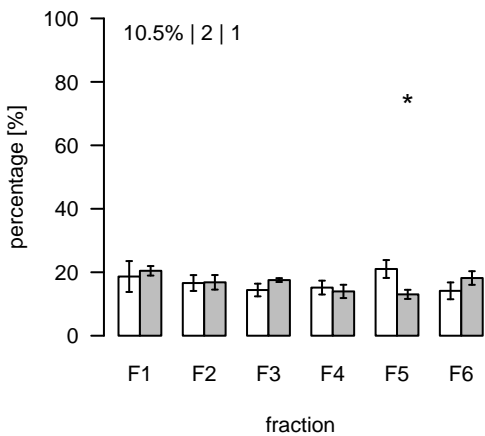
L803 (m/z=763.605779; rt=5.55204) T/S Cluster: L-5.6-1
