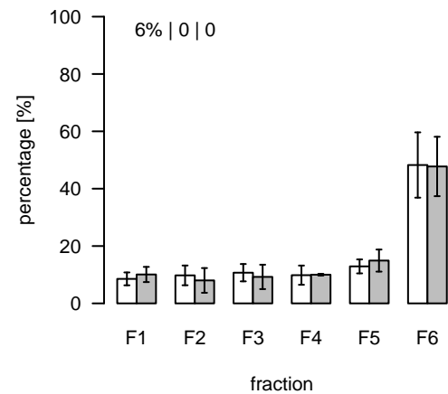
S381 (m/z=912.484429; rt=12.24036) T/S Cluster: S-12.2-11
