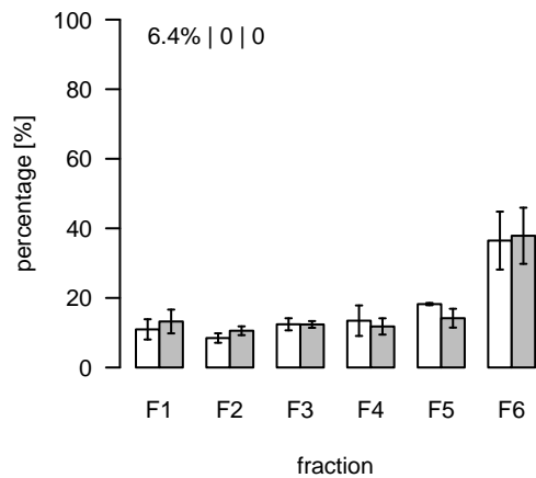
L1091 (m/z=335.259751; rt=6.54785) T/S Cluster: L-6.5-1
