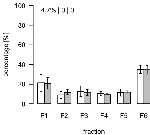
S6 (m/z=665.122478; rt=1.1478) T/S Cluster: S-1.1-1
