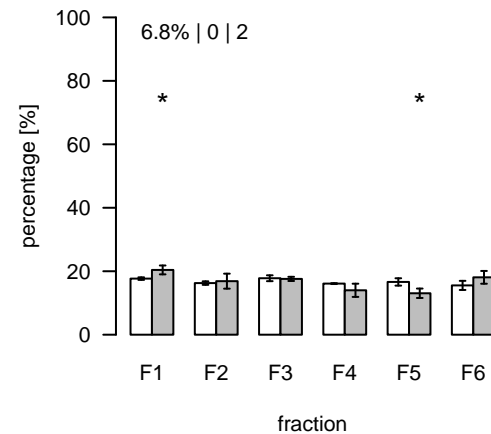
S897 (m/z=437.760659; rt=17.1805) T/S Cluster: S-17.2-1
