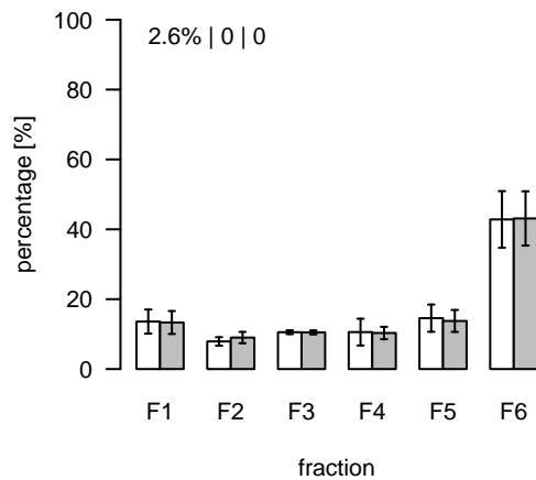
L913 (m/z=750.512718; rt=5.93759) T/S Cluster: L-5.9-4
