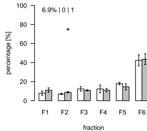
L1117 (m/z=477.813741; rt=6.61326) T/S Cluster: L-6.6-10
