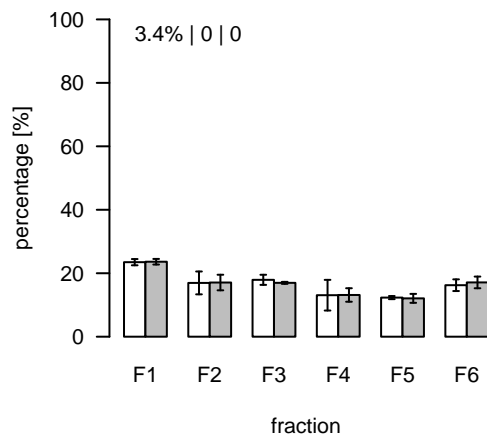
L2432 (m/z=422.344261; rt=11.7414) T/S Cluster: L-11.7-3
