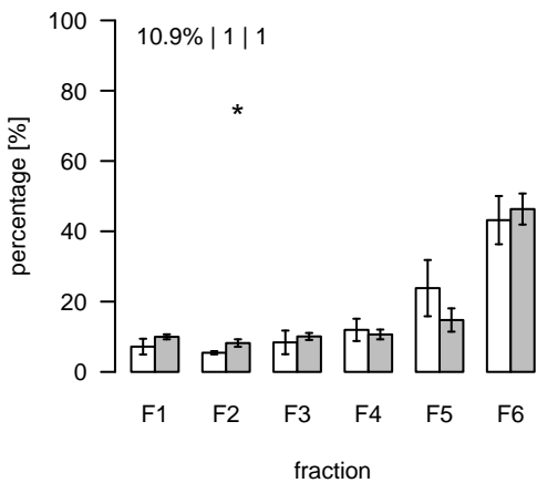
L818 (m/z=856.528616; rt=5.66113) T/S Cluster: L-5.7-1
