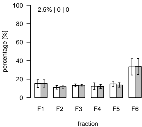
L591 (m/z=397.268576; rt=4.89983) T/S Cluster: L-4.9-10
