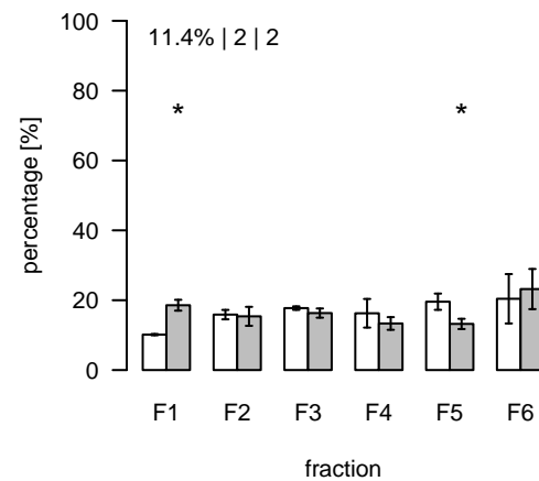
L2750 (m/z=1173.346117; rt=16.54767) T/S Cluster: L-16.5-6
