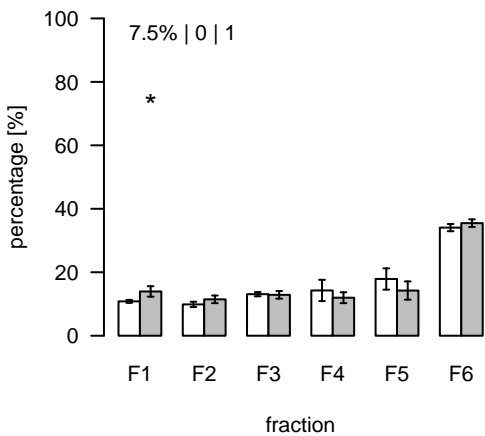
L1893 (m/z=778.55665; rt=9.56058) T/S Cluster: L-9.6-1
