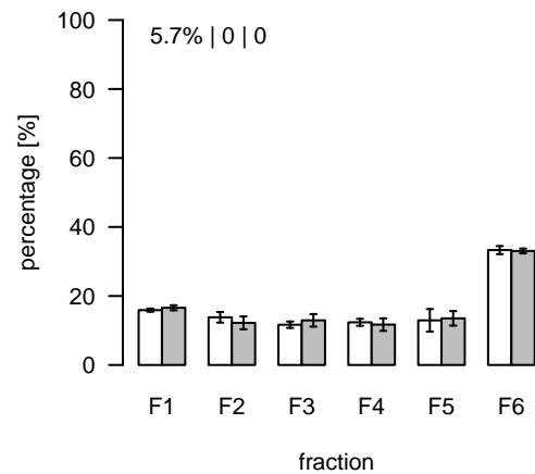
L2454 (m/z=875.592652; rt=11.84757) T/S Cluster: L-11.8-5
