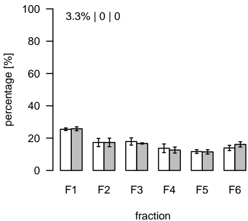
L2517 (m/z=901.756297; rt=13.70076) T/S Cluster: L-13.7-2
