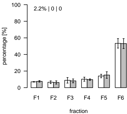
L535 (m/z=746.485037; rt=4.8115) T/S Cluster: L-4.8-10
