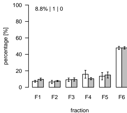
L1381 (m/z=911.515006; rt=7.53212) T/S Cluster: L-7.5-3
