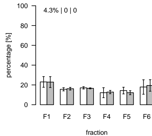
L1310 (m/z=260.520444; rt=7.32736) T/S Cluster: L-7.3-5
