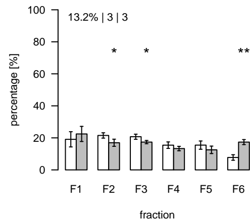
L2352 (m/z=685.998371; rt=11.32855) T/S Cluster: L-11.3-17
