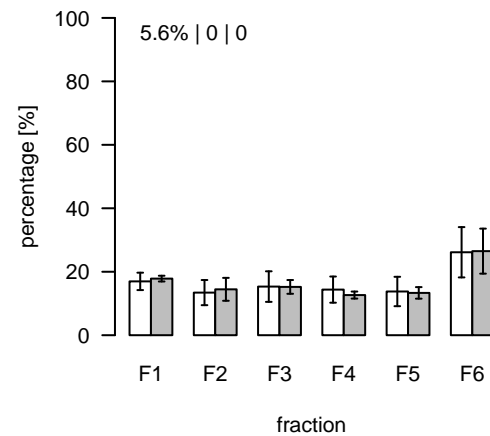
L1396 (m/z=781.56125; rt=7.61712) T/S Cluster: L-7.6-2
