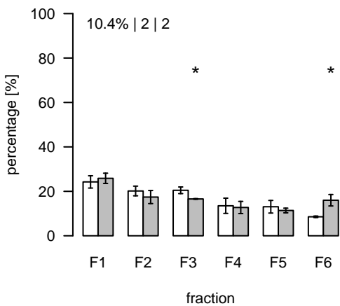
L829 (m/z=416.376182; rt=5.69754) T/S Cluster: L-5.7-5
