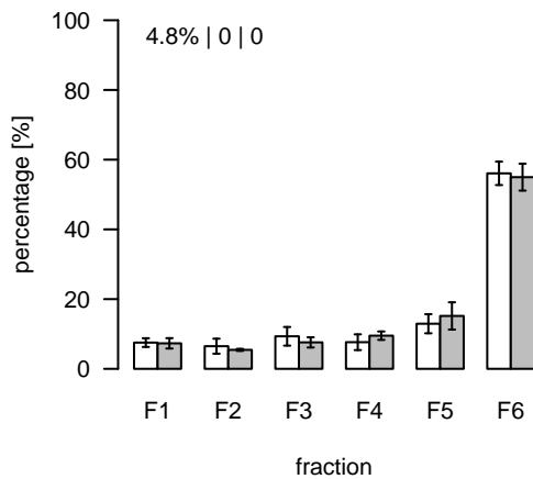
L2210 (m/z=870.565836; rt=11.00451) T/S Cluster: L-11-2
