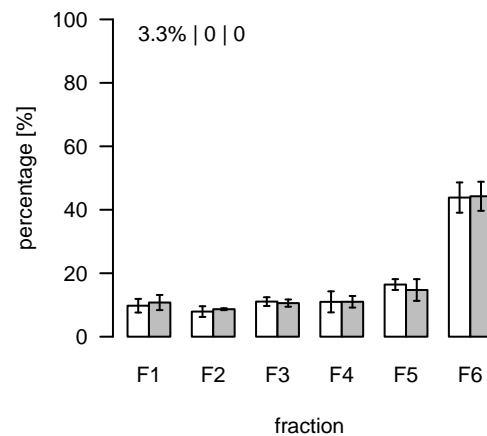
L2058 (m/z=779.570103; rt=10.38536) T/S Cluster: L-10.4-1
