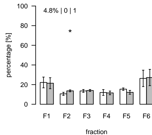
L1357 (m/z=821.604608; rt=7.35127) T/S Cluster: L-7.4-2
