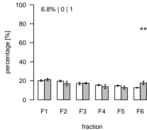
L2669 (m/z=460.657971; rt=15.84407) T/S Cluster: L-15.8-4
