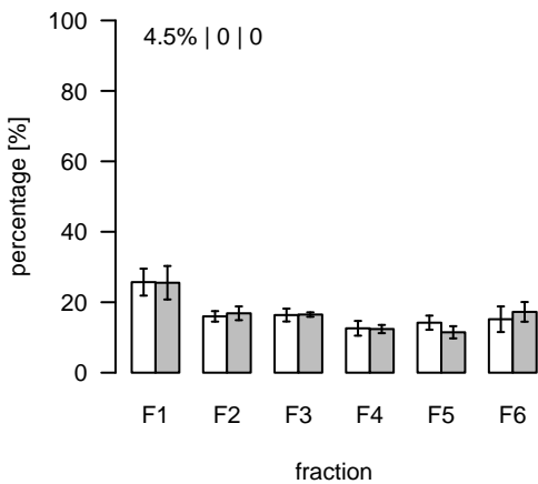
L1046 (m/z=793.572475; rt=6.54672) T/S Cluster: L-6.5-5
