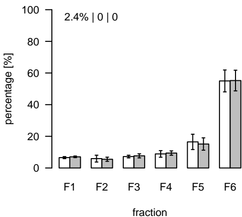
L20 (m/z=864.49964; rt=2.74845) T/S Cluster: L-2.7-2
