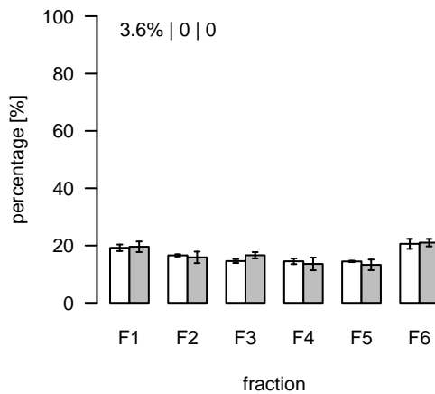
S478 (m/z=672.414907; rt=12.91116) T/S Cluster: S-12.9-10
