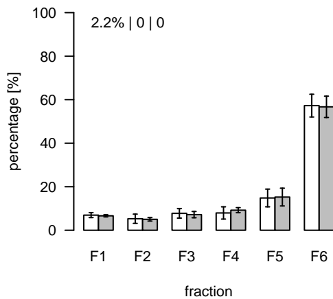
L220 (m/z=900.541573; rt=3.84179) T/S Cluster: L-3.8-5
