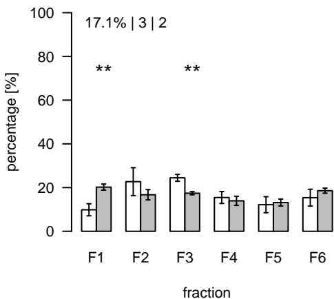
S874 (m/z=577.521396; rt=16.98764) T/S Cluster: S-17-10
