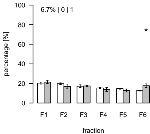
L2667 (m/z=460.666603; rt=15.84373) T/S Cluster: L-15.8-4
