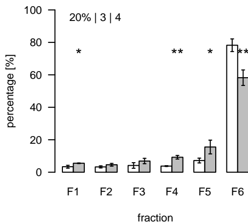
L1975 (m/z=908.528529; rt=9.87999) T/S Cluster: L-9.9-2
