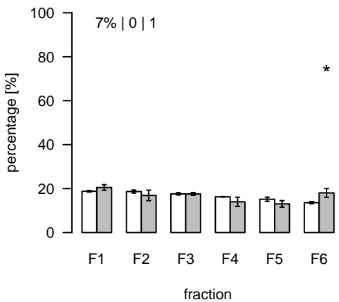
L2696 (m/z=497.169149; rt=16.15517) T/S Cluster: L-16.2-1
