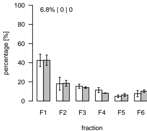
S130 (m/z=404.14443; rt=5.47232) T/S Cluster: S-5.5-1
