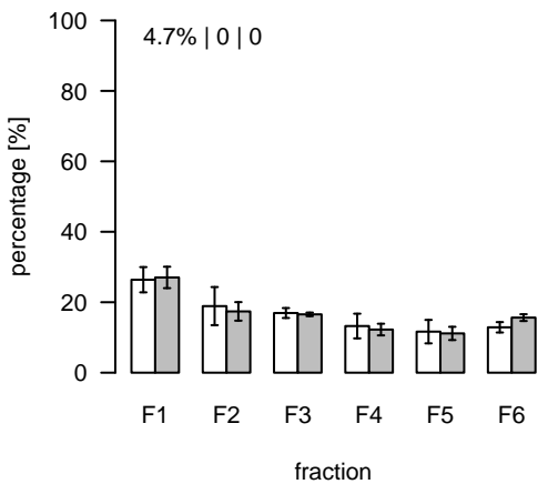
L453 (m/z=790.517958; rt=4.57223) T/S Cluster: L-4.6-1
