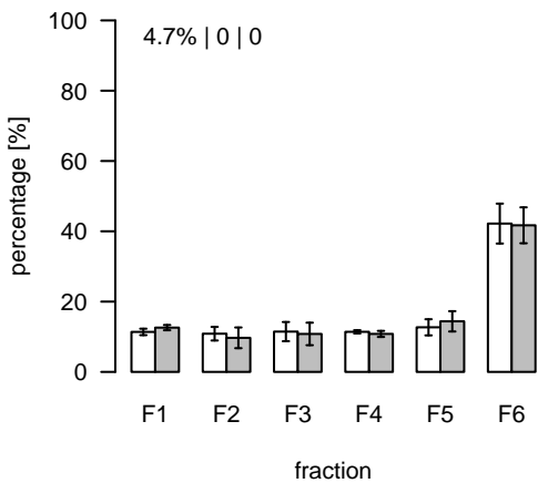
S433 (m/z=858.48741; rt=12.55491) T/S Cluster: S-12.6-10
