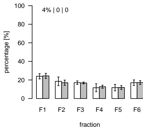
L1004 (m/z=773.529574; rt=6.33934) T/S Cluster: L-6.3-6
