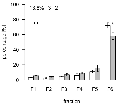
L1221 (m/z=792.50856; rt=6.7775) T/S Cluster: L-6.8-1
