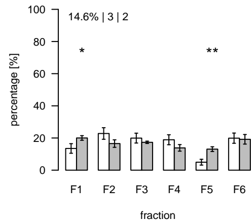
S630 (m/z=437.795513; rt=14.78491) T/S Cluster: S-14.8-6
