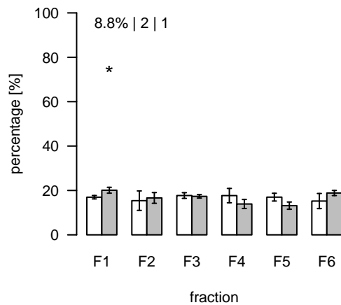
S2 (m/z=437.739853; rt=0.46198) T/S Cluster: S-0.5-1
