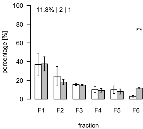
L256 (m/z=692.439643; rt=3.9774) T/S Cluster: L-4-4
