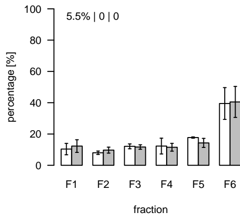
L1064 (m/z=587.461397; rt=6.54758) T/S Cluster: L-6.5-1
