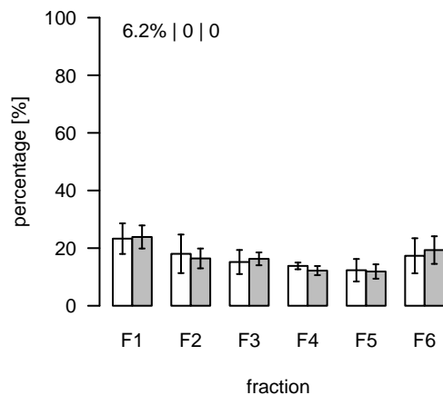
L471 (m/z=832.565407; rt=4.62405) T/S Cluster: L-4.6-8
