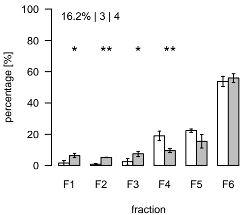
L710 (m/z=785.531198; rt=5.21845) T/S Cluster: L-5.2-4
