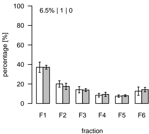
S706 (m/z=790.5612; rt=15.54154) T/S Cluster: S-15.5-2
