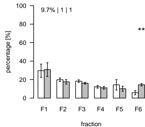
L1751 (m/z=392.800056; rt=8.87991) T/S Cluster: L-8.9-1
