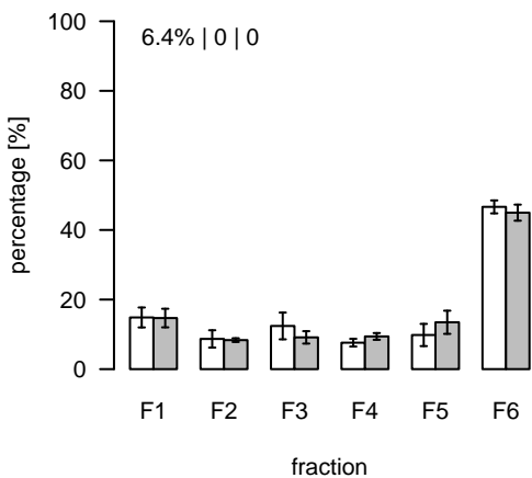
S776 (m/z=858.532452; rt=16.2402) T/S Cluster: S-16.2-6
