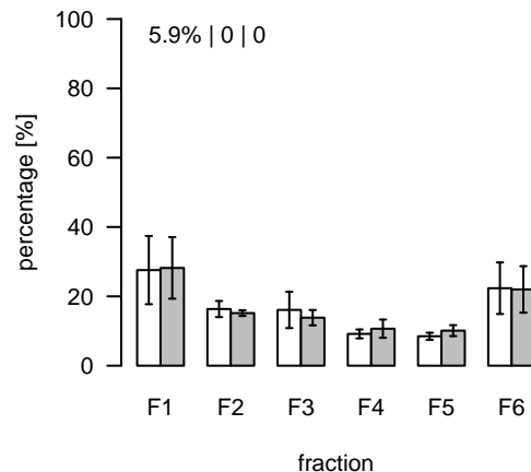
S773 (m/z=303.650248; rt=16.2161) T/S Cluster: S-16.2-5
