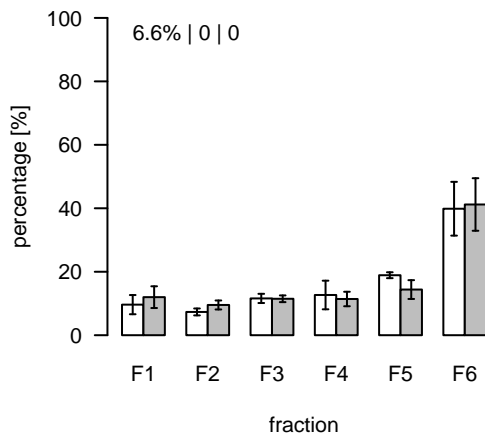
L1088 (m/z=764.533918; rt=6.54777) T/S Cluster: L-6.5-1
