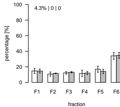
L100 (m/z=842.514619; rt=3.54818) T/S Cluster: L-3.5-8
