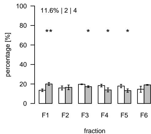
L2131 (m/z=1089.722261; rt=10.52438) T/S Cluster: L-10.5-17
