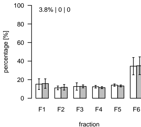
S335 (m/z=722.396797; rt=10.77744) T/S Cluster: S-10.8-2
