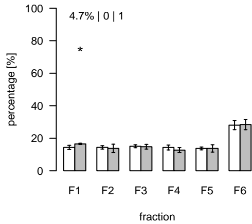
L2094 (m/z=448.281258; rt=10.50425) T/S Cluster: L-10.5-13
