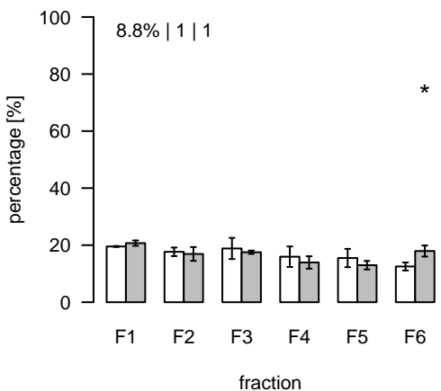
L2686 (m/z=905.838883; rt=16.06124) T/S Cluster: L-16.1-1
