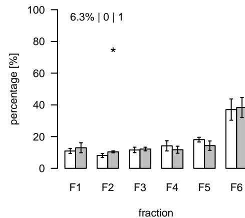
L1102 (m/z=568.439154; rt=6.54958) T/S Cluster: L-6.5-1
