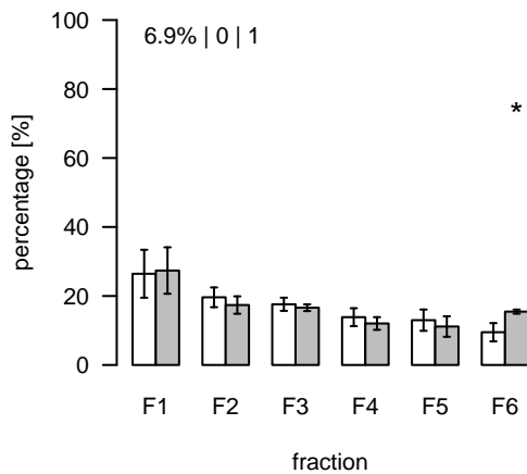
L2028 (m/z=774.588261; rt=10.15939) T/S Cluster: L-10.2-1
