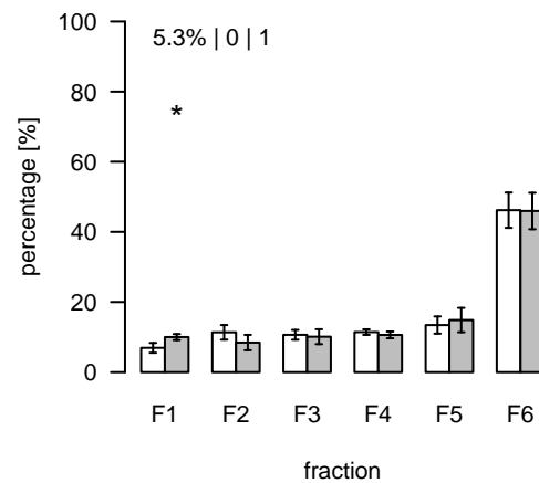
L797 (m/z=568.430111; rt=5.51248) T/S Cluster: L-5.5-2
