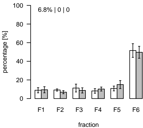
L6 (m/z=432.232293; rt=1.36462) T/S Cluster: L-1.4-1
