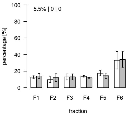
L561 (m/z=796.486616; rt=4.864) T/S Cluster: L-4.9-2
