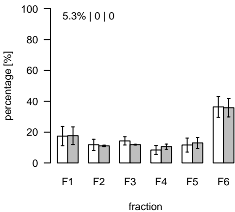
L1422 (m/z=885.558396; rt=7.87876) T/S Cluster: L-7.9-2
