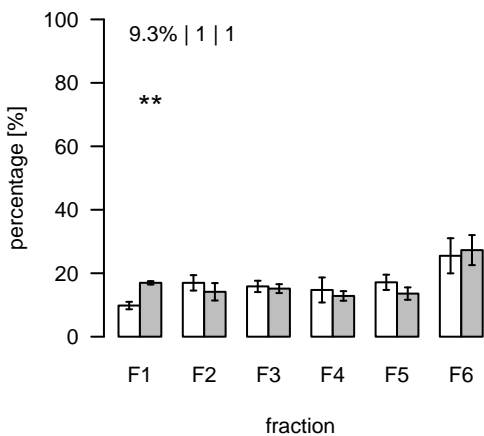
L2779 (m/z=1203.298756; rt=16.966) T/S Cluster: L-17-2
