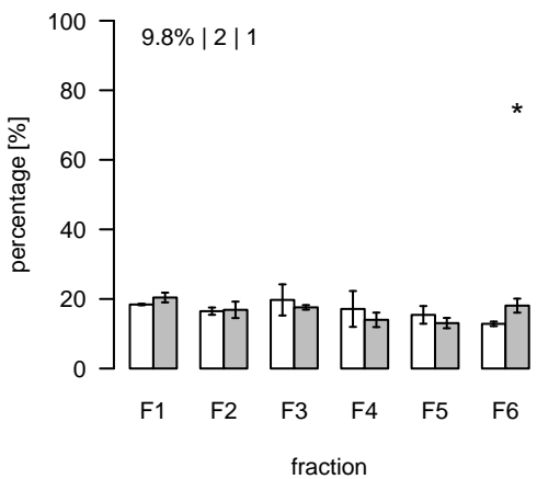
L2661 (m/z=876.808984; rt=15.83195) T/S Cluster: L-15.8-3
