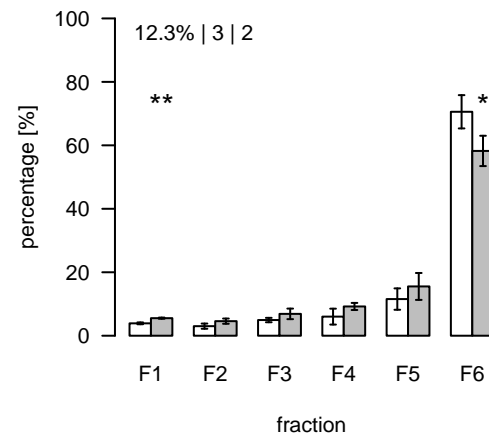
L214 (m/z=724.43977; rt=3.83764) T/S Cluster: L-3.8-5
