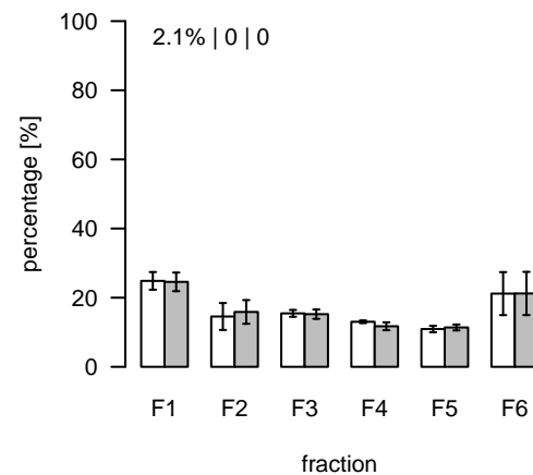
S24 (m/z=268.104359; rt=3.13672) T/S Cluster: S-3.1-1
