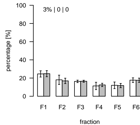
L1006 (m/z=772.5302; rt=6.33945) T/S Cluster: L-6.3-6
