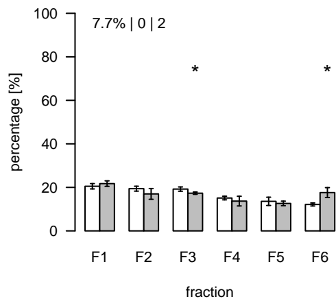
L2555 (m/z=772.265641; rt=14.97184) T/S Cluster: L-15-1
