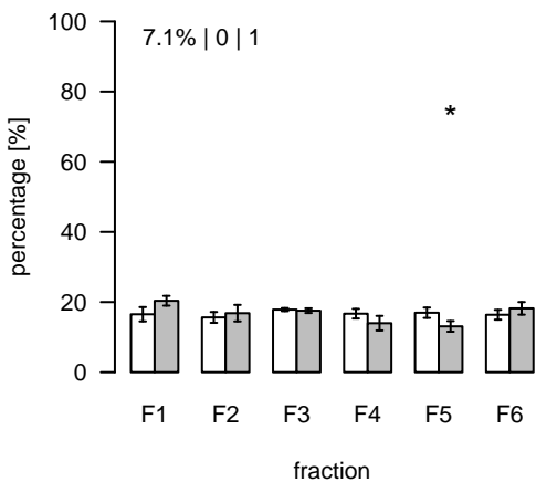
L1804 (m/z=911.530407; rt=8.92028) T/S Cluster: L-8.9-17
