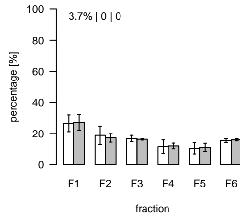
L1373 (m/z=777.587013; rt=7.47703) T/S Cluster: L-7.5-1
