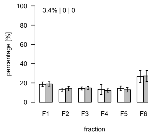
L472 (m/z=814.566896; rt=4.64567) T/S Cluster: L-4.6-9
