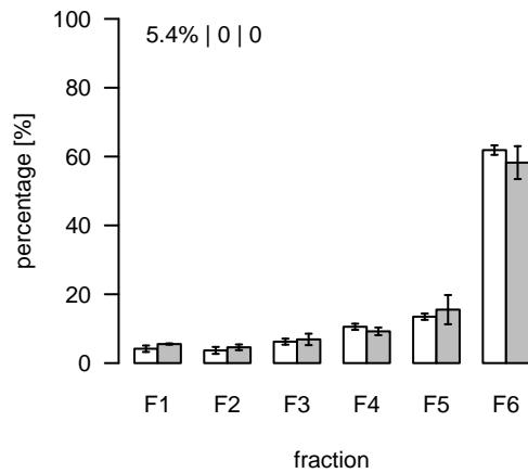
L795 (m/z=551.427179; rt=5.51048) T/S Cluster: L-5.5-2
