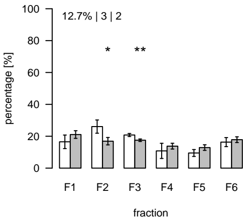
S754 (m/z=483.369505; rt=16.04463) T/S Cluster: S-16-4
