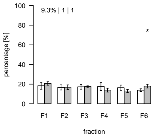
L2565 (m/z=872.774212; rt=15.32187) T/S Cluster: L-15.3-2
