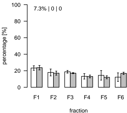
L447 (m/z=840.533472; rt=4.5346) T/S Cluster: L-4.5-10
