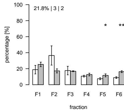
S892 (m/z=788.546257; rt=17.04346) T/S Cluster: S-17-17
