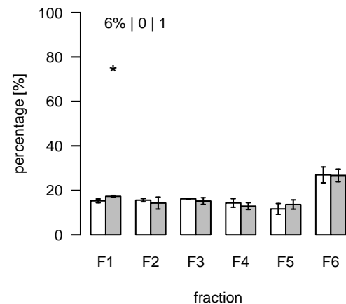
L2079 (m/z=953.612228; rt=10.49444) T/S Cluster: L-10.5-4
