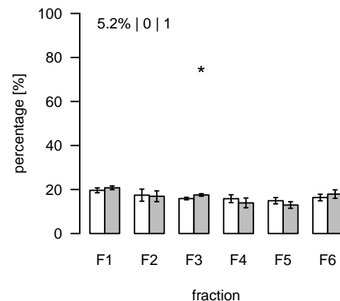
L132 (m/z=402.272308; rt=3.65112) T/S Cluster: L-3.7-2
