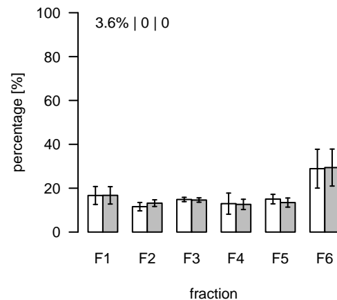
L588 (m/z=794.492845; rt=4.89898) T/S Cluster: L-4.9-10
