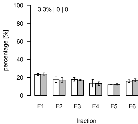
L2429 (m/z=846.700909; rt=11.74101) T/S Cluster: L-11.7-3
