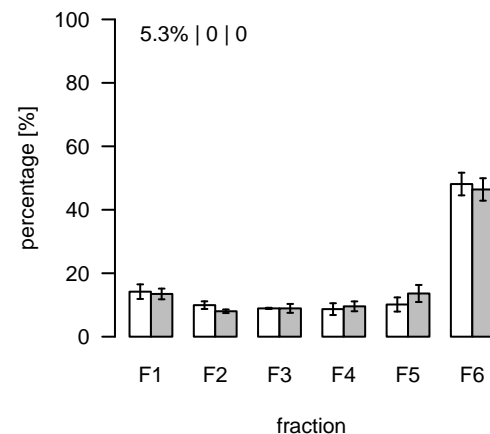
S600 (m/z=848.543625; rt=14.51931) T/S Cluster: S-14.5-8
