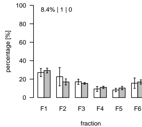
L729 (m/z=825.524196; rt=5.28591) T/S Cluster: L-5.3-3
