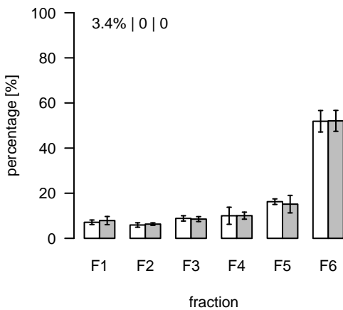
L1706 (m/z=771.586395; rt=8.70873) T/S Cluster: L-8.7-7
