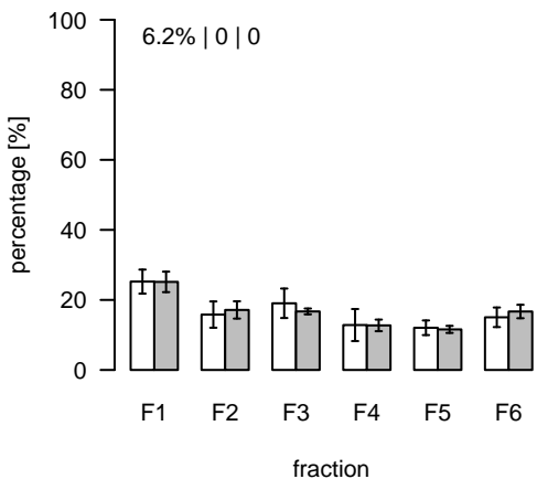
L2172 (m/z=844.681612; rt=10.66243) T/S Cluster: L-10.7-1
