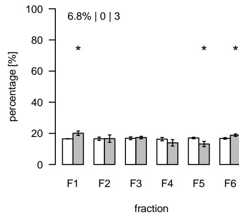
S493 (m/z=348.216957; rt=12.91269) T/S Cluster: S-12.9-23
