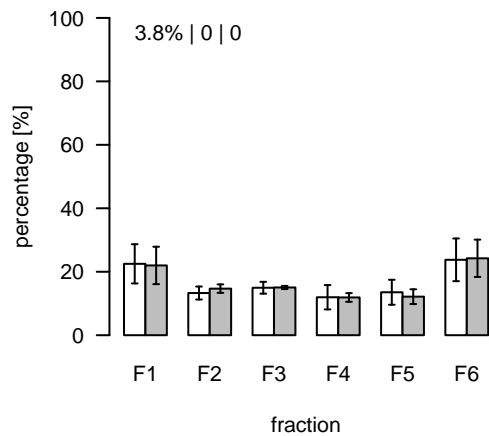
L1543 (m/z=391.792694; rt=8.05649) T/S Cluster: L-8.1-2
