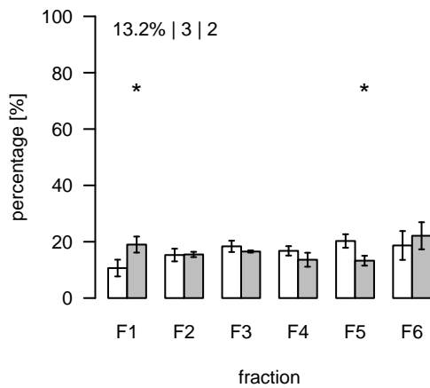
L2282 (m/z=340.744191; rt=11.32785) T/S Cluster: L-11.3-4
