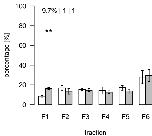
L2800 (m/z=1351.387937; rt=18.07367) T/S Cluster: L-18.1-1
