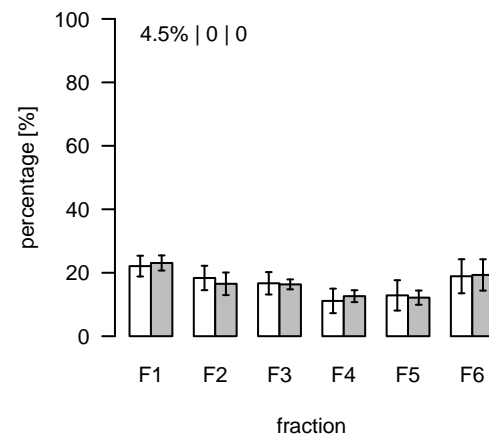
L677 (m/z=836.604221; rt=5.04905) T/S Cluster: L-5-9
