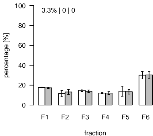
S387 (m/z=756.363331; rt=12.29686) T/S Cluster: S-12.3-2
