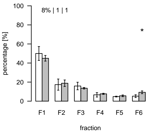
S174 (m/z=198.38746; rt=6.57798) T/S Cluster: S-6.6-2
