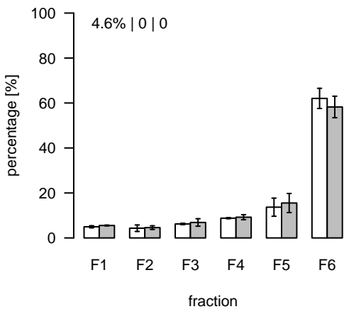
L127 (m/z=1002.57197; rt=3.61837) T/S Cluster: L-3.6-5
