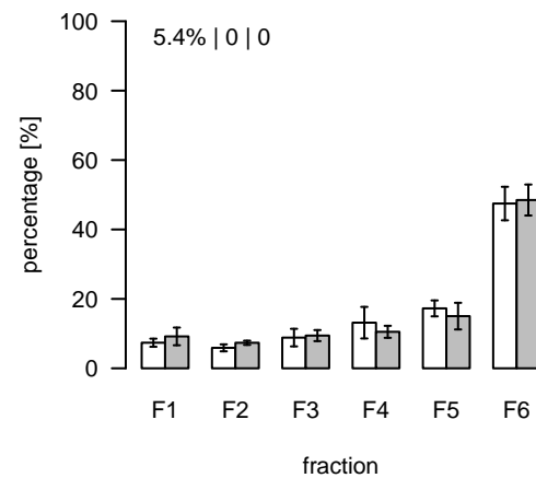
L340 (m/z=801.479976; rt=4.27825) T/S Cluster: L-4.3-1
