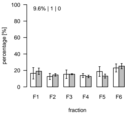
L1788 (m/z=888.54002; rt=8.91741) T/S Cluster: L-8.9-4
