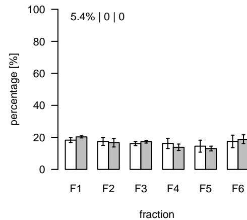
L1633 (m/z=366.279522; rt=8.60107) T/S Cluster: L-8.6-4
