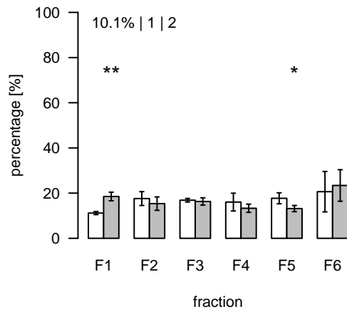
L2753 (m/z=1129.324232; rt=16.54773) T/S Cluster: L-16.5-6
