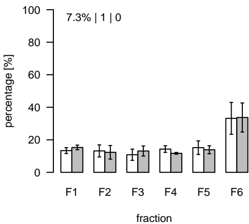
S456 (m/z=922.504506; rt=12.708) T/S Cluster: S-12.7-8
