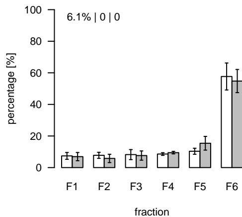
L52 (m/z=840.519244; rt=3.33556) T/S Cluster: L-3.3-1
