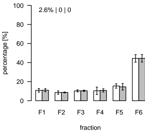
L1879 (m/z=938.673722; rt=9.5288) T/S Cluster: L-9.5-5
