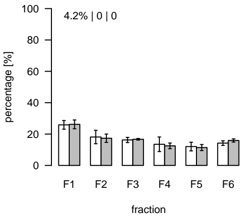
L144 (m/z=804.543424; rt=3.65345) T/S Cluster: L-3.7-4
