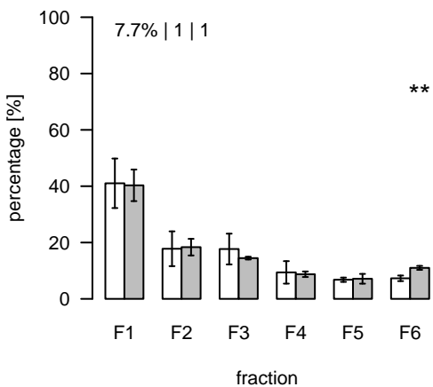
S281 (m/z=202.123209; rt=8.5313) T/S Cluster: S-8.5-1
