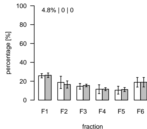
L1016 (m/z=776.583235; rt=6.44457) T/S Cluster: L-6.4-4
