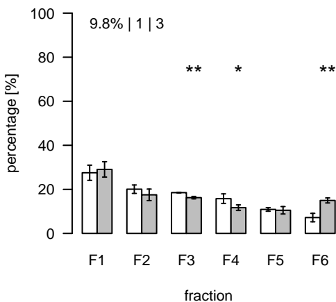
L1683 (m/z=189.894143; rt=8.70683) T/S Cluster: L-8.7-5
