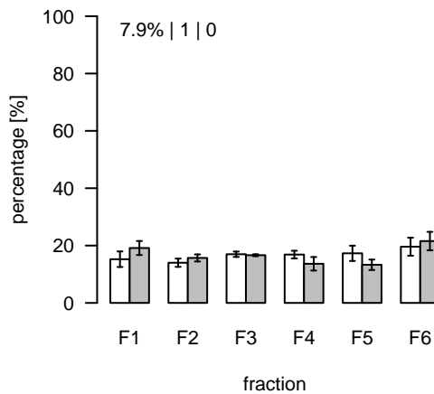
L1797 (m/z=968.587407; rt=8.91804) T/S Cluster: L-8.9-12
