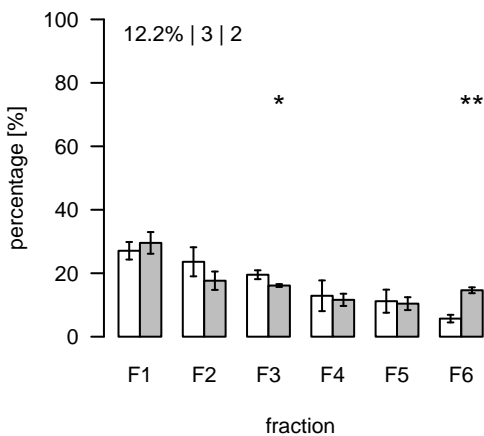
L1935 (m/z=783.557531; rt=9.59878) T/S Cluster: L-9.6-3
