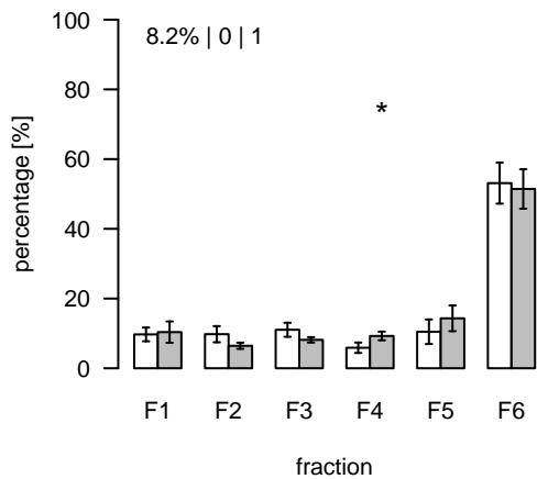
S854 (m/z=954.618844; rt=16.96745) T/S Cluster: S-17-2
