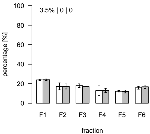
L2426 (m/z=845.667029; rt=11.74026) T/S Cluster: L-11.7-3
