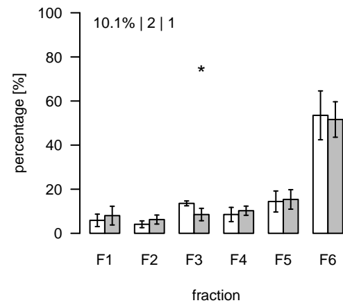
L1859 (m/z=908.528466; rt=9.43462) T/S Cluster: L-9.4-1
