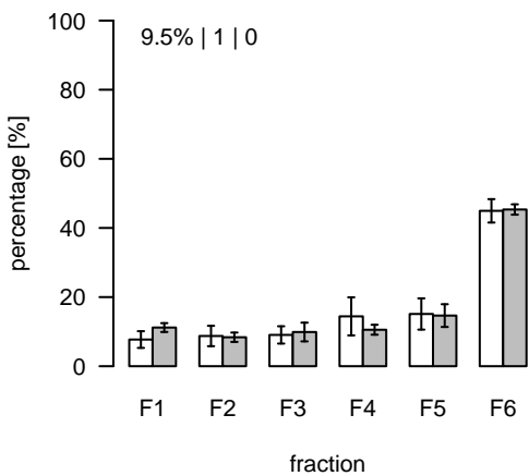
L1378 (m/z=912.49985; rt=7.50503) T/S Cluster: L-7.5-3
