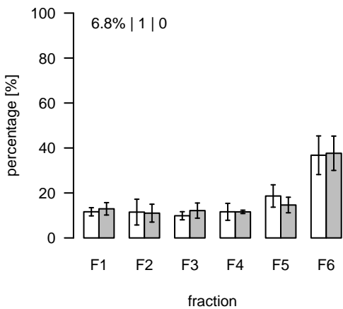
L620 (m/z=986.612313; rt=4.91768) T/S Cluster: L-4.9-2
