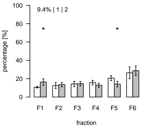
L2045 (m/z=948.522734; rt=10.21488) T/S Cluster: L-10.2-3
