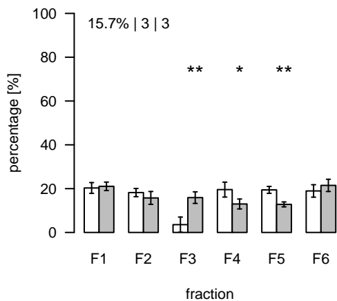
S554 (m/z=437.738666; rt=13.89993) T/S Cluster: S-13.9-1
