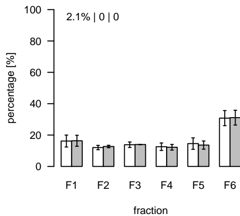
L727 (m/z=798.566932; rt=5.28473) T/S Cluster: L-5.3-1
