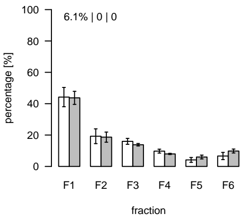
S100 (m/z=1378.365763; rt=4.70723) T/S Cluster: S-4.7-1
