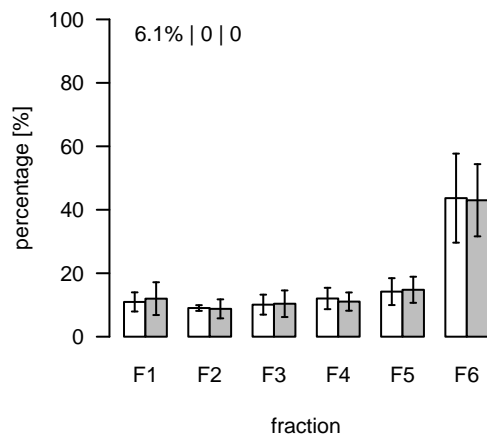
L1586 (m/z=924.498092; rt=8.19986) T/S Cluster: L-8.2-3
