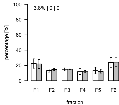
L1554 (m/z=391.786568; rt=8.05694) T/S Cluster: L-8.1-2
