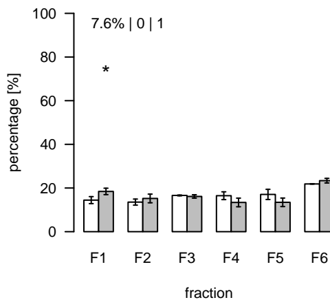
L1781 (m/z=302.50903; rt=8.91532) T/S Cluster: L-8.9-5
