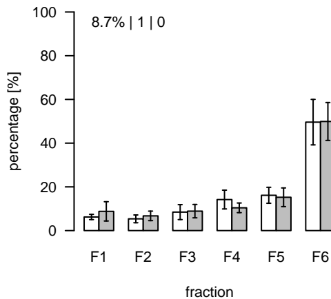
L1940 (m/z=911.54772; rt=9.62003) T/S Cluster: L-9.6-5
