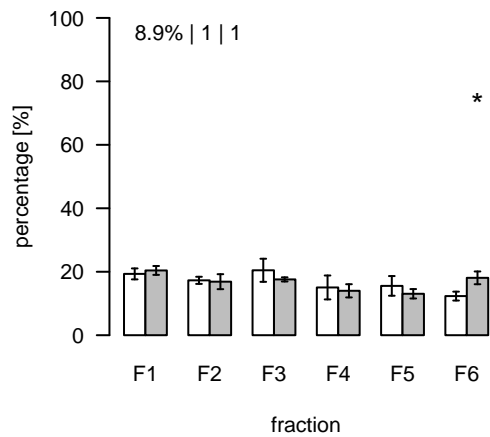
L2604 (m/z=822.758106; rt=15.57404) T/S Cluster: L-15.6-1
