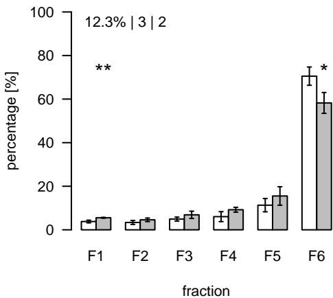
L215 (m/z=725.470861; rt=3.83766) T/S Cluster: L-3.8-5
