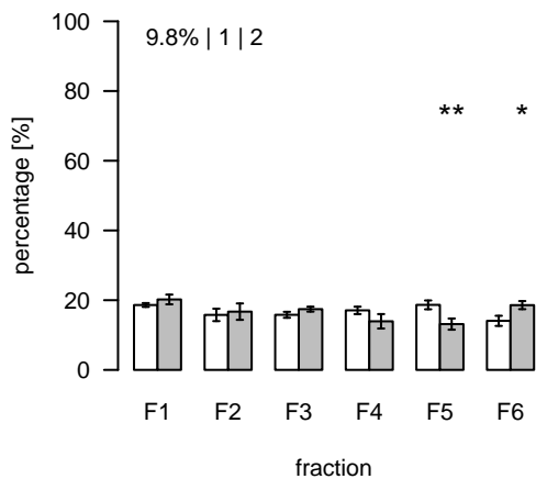
S428 (m/z=422.260419; rt=12.55149) T/S Cluster: S-12.6-5
