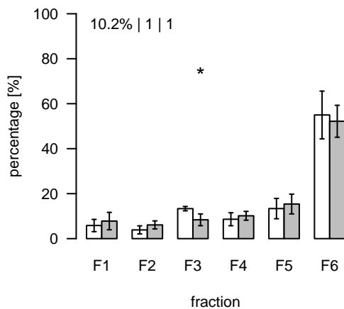
L1858 (m/z=907.466113; rt=9.43455) T/S Cluster: L-9.4-1
