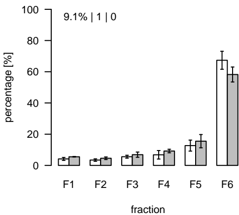
L644 (m/z=781.532906; rt=4.95285) T/S Cluster: L-5-1
