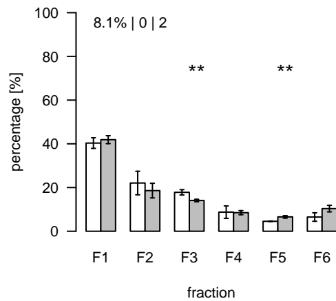
S219 (m/z=580.176219; rt=7.1957) T/S Cluster: S-7.2-2
