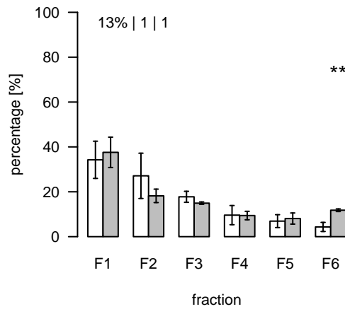
L165 (m/z=688.42026; rt=3.6753) T/S Cluster: L-3.7-14
