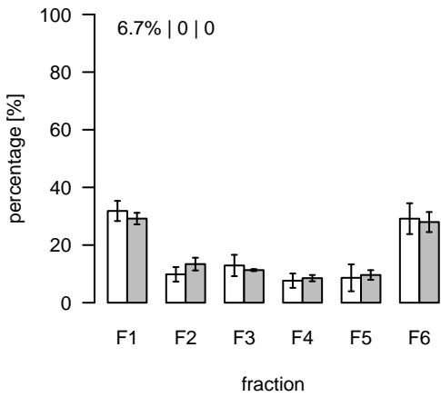
S237 (m/z=547.334301; rt=7.20078) T/S Cluster: S-7.2-1
