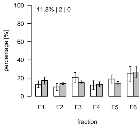
L1999 (m/z=885.507446; rt=10.09008) T/S Cluster: L-10.1-6
