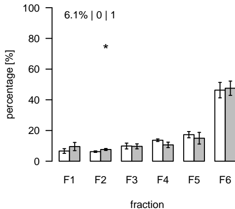
L1564 (m/z=799.522707; rt=8.05962) T/S Cluster: L-8.1-1
