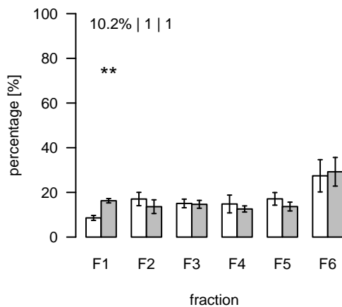
L2789 (m/z=1277.321876; rt=17.44891) T/S Cluster: L-17.4-1
