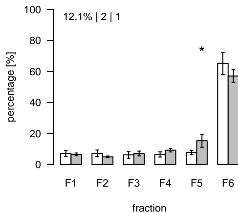
S808 (m/z=613.456524; rt=16.56719) T/S Cluster: S-16.6-2
