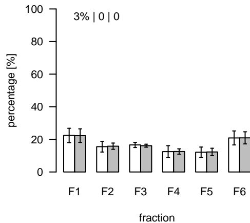
L877 (m/z=771.542687; rt=5.72224) T/S Cluster: L-5.7-7
