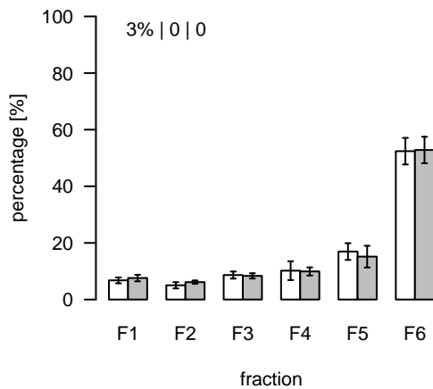
L610 (m/z=484.305093; rt=4.91022) T/S Cluster: L-4.9-9
