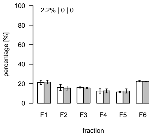
L2237 (m/z=681.625381; rt=11.31723) T/S Cluster: L-11.3-6
