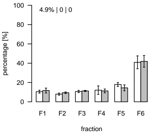
L1450 (m/z=467.327978; rt=7.90476) T/S Cluster: L-7.9-9
