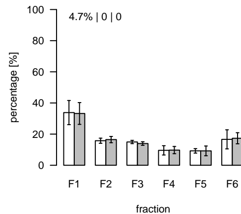
S708 (m/z=774.566459; rt=15.58079) T/S Cluster: S-15.6-1
