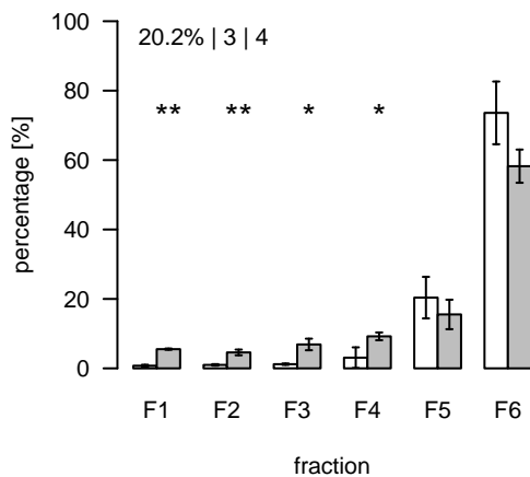
L639 (m/z=780.601868; rt=4.95212) T/S Cluster: L-5-1
