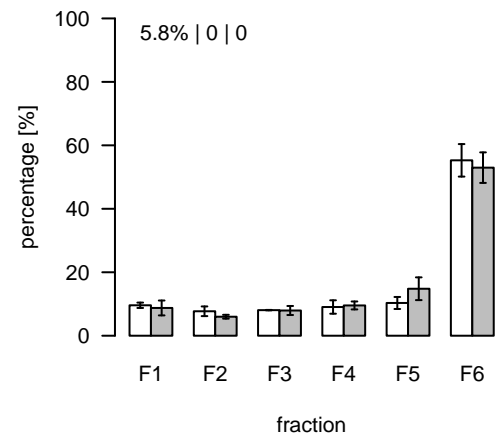
S595 (m/z=848.50231; rt=14.49453) T/S Cluster: S-14.5-6
