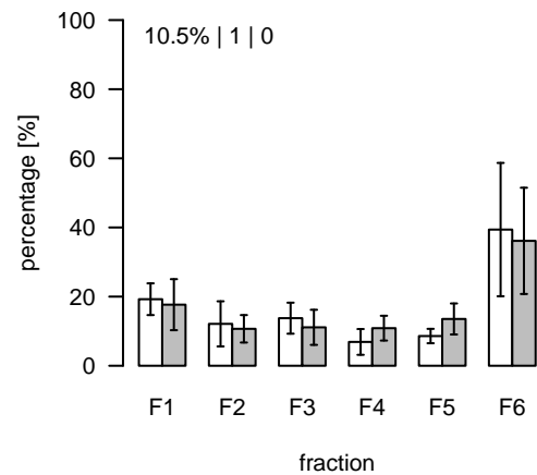
S861 (m/z=760.515728; rt=16.97621) T/S Cluster: S-17-3
