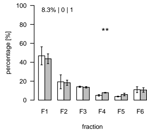
S696 (m/z=652.449083; rt=15.39129) T/S Cluster: S-15.4-1
