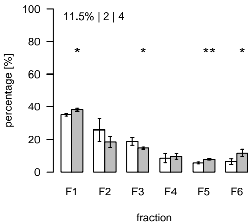
S226 (m/z=289.573397; rt=7.19596) T/S Cluster: S-7.2-2
