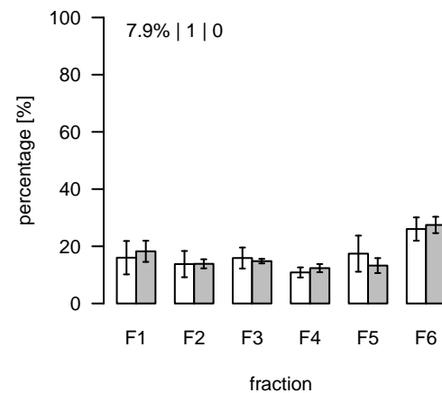
L1760 (m/z=888.577083; rt=8.91329) T/S Cluster: L-8.9-4
