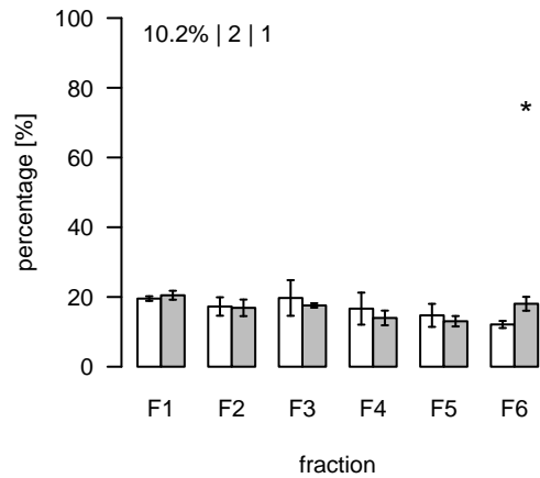
L2645 (m/z=852.798226; rt=15.82628) T/S Cluster: L-15.8-3
