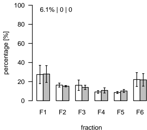
S774 (m/z=303.646433; rt=16.21619) T/S Cluster: S-16.2-5
