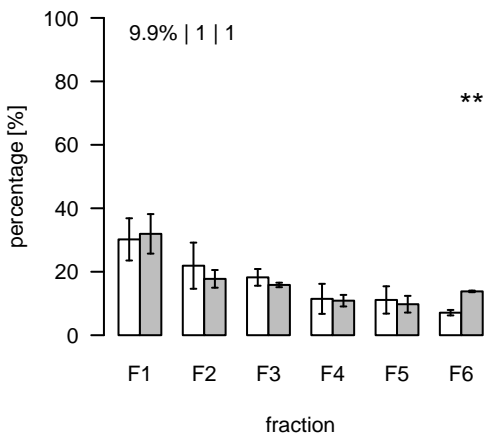
L235 (m/z=680.452785; rt=3.90662) T/S Cluster: L-3.9-6
