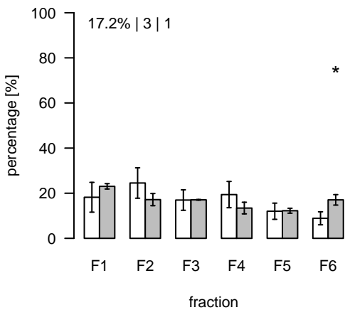
L2472 (m/z=894.570314; rt=11.85309) T/S Cluster: L-11.9-2
