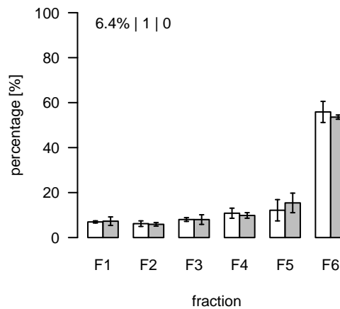
L1388 (m/z=926.535473; rt=7.58533) T/S Cluster: L-7.6-1
