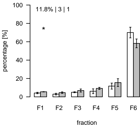
L1276 (m/z=383.276107; rt=7.18909) T/S Cluster: L-7.2-3
