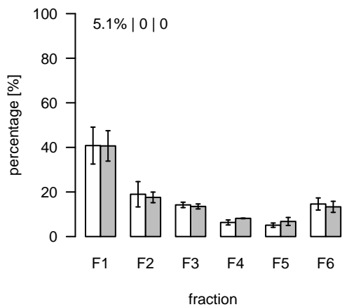
S669 (m/z=804.541272; rt=14.9733) T/S Cluster: S-15-1
