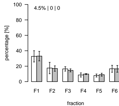
S311 (m/z=654.327737; rt=9.80671) T/S Cluster: S-9.8-1
