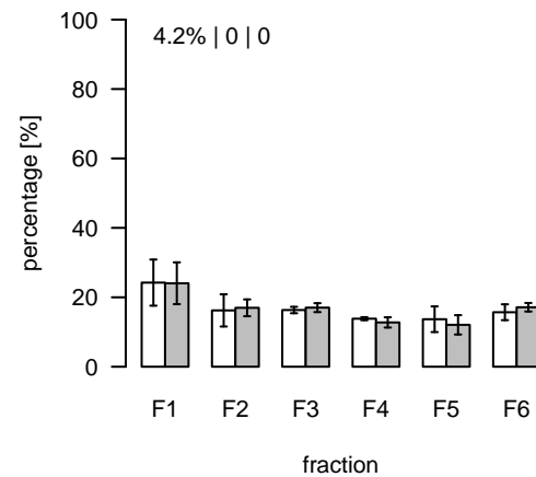
L1990 (m/z=760.588967; rt=10.05401) T/S Cluster: L-10.1-2
