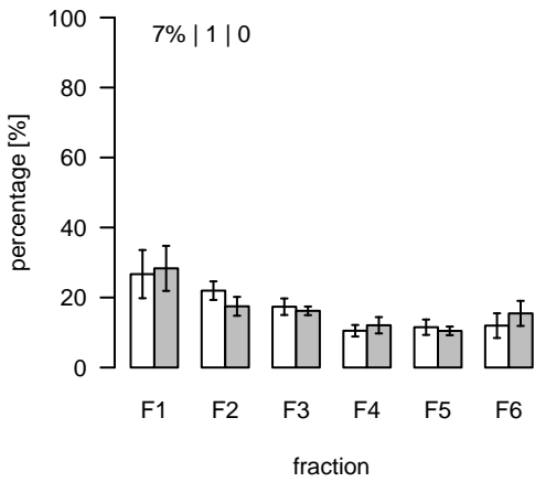
S169 (m/z=214.089913; rt=6.56579) T/S Cluster: S-6.6-1
