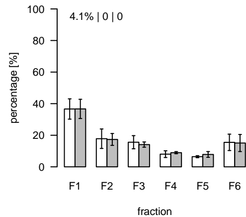
S323 (m/z=199.436003; rt=10.0615) T/S Cluster: S-10.1-1
