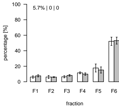
L273 (m/z=801.480595; rt=4.05539) T/S Cluster: L-4.1-1
