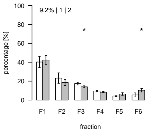
S203 (m/z=193.064387; rt=7.19262) T/S Cluster: S-7.2-2
