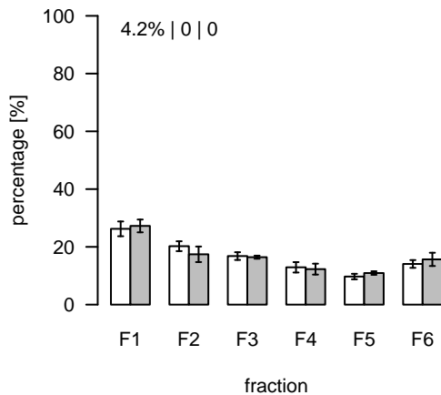
L2515 (m/z=832.705531; rt=13.69529) T/S Cluster: L-13.7-2
