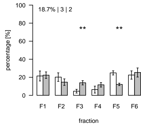
S378 (m/z=437.725748; rt=12.21421) T/S Cluster: S-12.2-8
