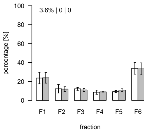
S339 (m/z=612.32494; rt=10.8184) T/S Cluster: S-10.8-4
