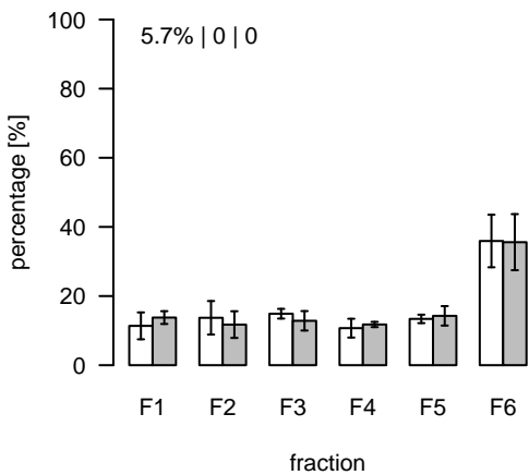
S376 (m/z=898.511282; rt=12.18795) T/S Cluster: S-12.2-6
