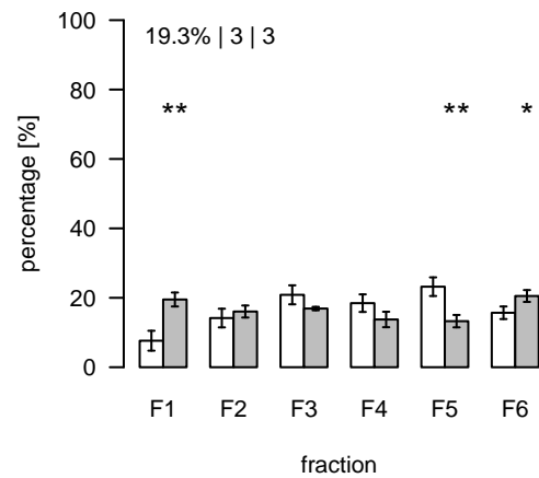
L2320 (m/z=1344.94999; rt=11.32827) T/S Cluster: L-11.3-4
