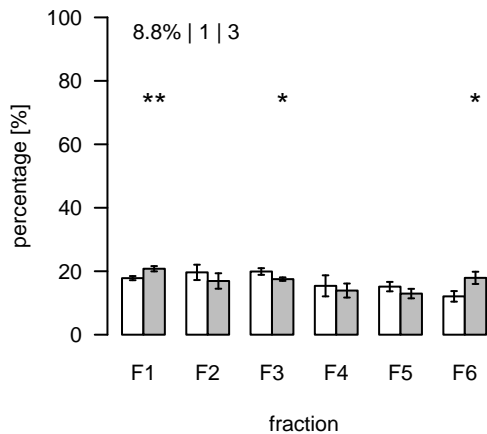
L2163 (m/z=865.660386; rt=10.62507) T/S Cluster: L-10.6-7
