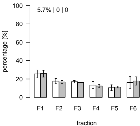
L1514 (m/z=379.790352; rt=7.965) T/S Cluster: L-8-1
