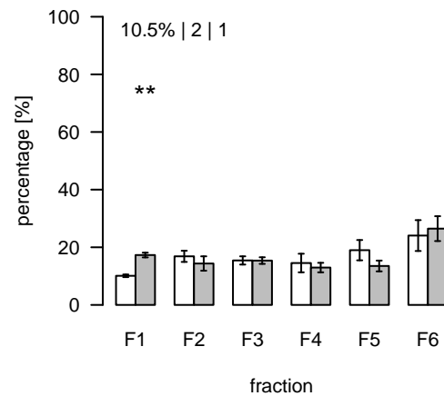
L2542 (m/z=834.245074; rt=14.79748) T/S Cluster: L-14.8-1
