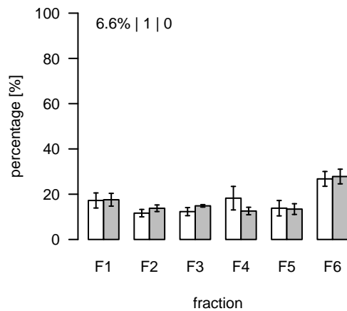
L408 (m/z=804.580244; rt=4.42687) T/S Cluster: L-4.4-1
