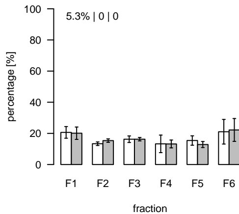
L1022 (m/z=752.527978; rt=6.52324) T/S Cluster: L-6.5-2
