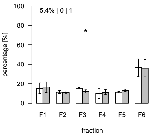
S599 (m/z=655.384721; rt=14.51391) T/S Cluster: S-14.5-7
