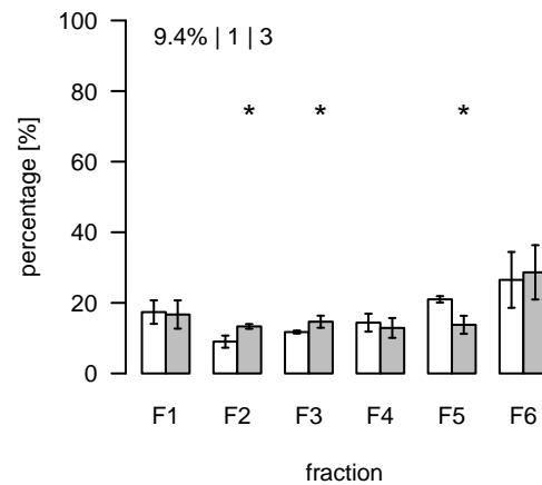
L539 (m/z=784.50747; rt=4.81367) T/S Cluster: L-4.8-11
