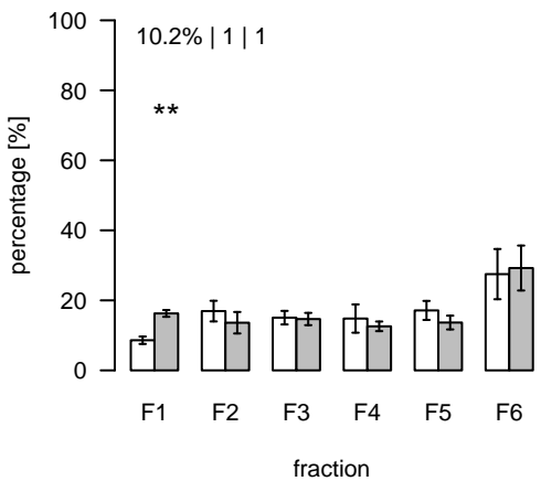
L2790 (m/z=1277.374997; rt=17.44917) T/S Cluster: L-17.4-1
