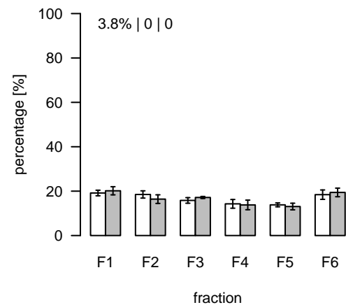
S549 (m/z=399.211433; rt=13.70865) T/S Cluster: S-13.7-1
