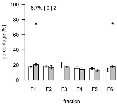
L2620 (m/z=811.761057; rt=15.68151) T/S Cluster: L-15.7-1
