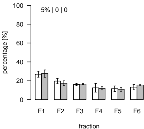
L1620 (m/z=732.538311; rt=8.47433) T/S Cluster: L-8.5-1
