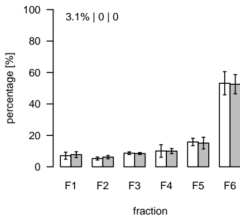
L1301 (m/z=957.640988; rt=7.30054) T/S Cluster: L-7.3-3
