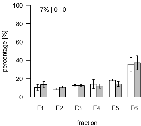
L1160 (m/z=614.480477; rt=6.65424) T/S Cluster: L-6.7-3
