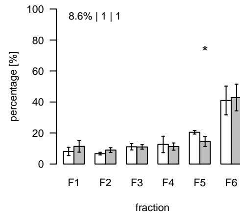
L1283 (m/z=772.508637; rt=7.19016) T/S Cluster: L-7.2-3
