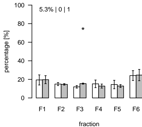
L568 (m/z=802.535644; rt=4.88137) T/S Cluster: L-4.9-5
