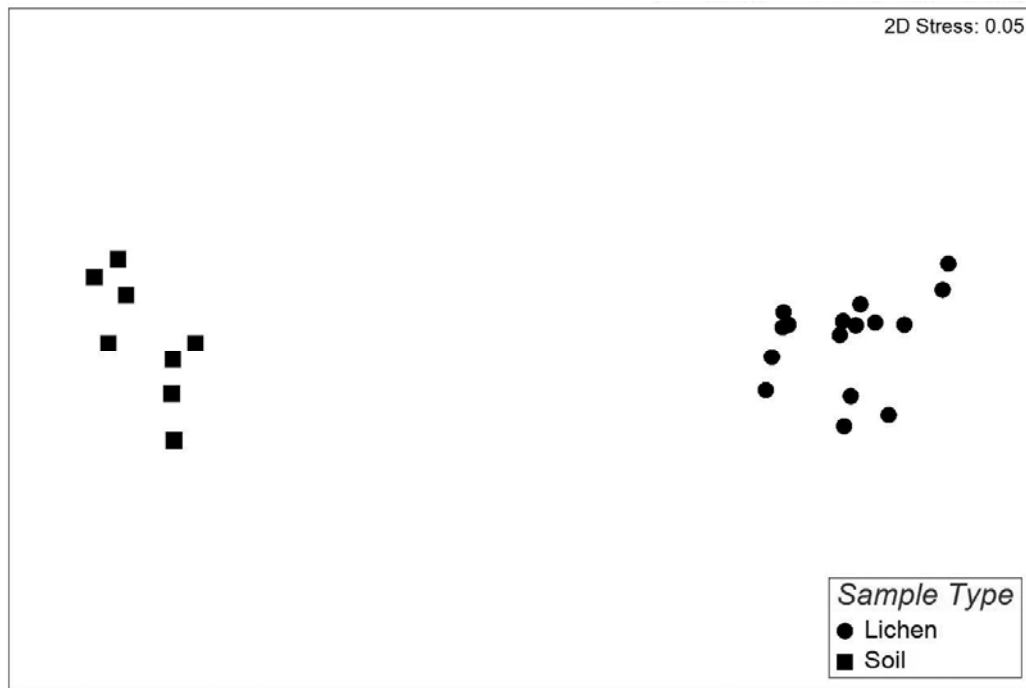
FIG. S2. Non-metric multidimensional scaling plot (on a Bray-Curtis distance matrix) depicting patterns of beta diversity for bacterial communities associated with lichen thalli and nearby soil samples collected at Gordon Gulch. Points that are closer together on the ordination have communities that are more similar. The difference between bacterial communities of lichen and soil samples was highly significant ( P < 0.001 ) under PERMANOVA analysis.
