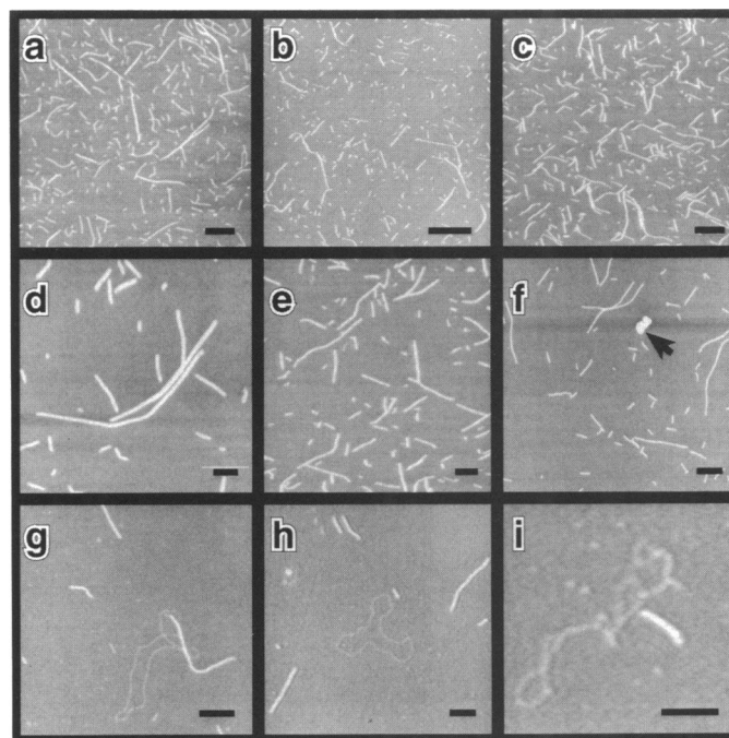
Figure 1. AFM gallery of G-wires grown in the presence of spermidine. The average height of the G-wires is 23.9 \pm 1.1 Å and the lengths range from 10 to >1000 nm. (a-i) are G-wires grown with Tet 1.5 at a concentration of 0.25 μg/μl in buffer containing 50 mM NaCl, 50 mM Tris-HCl, pH 7.5, 10 mM MgCl 2 and 1 μM spermidine at 37°C for 12–24 h. Panel f is an image of G-wires deposited with 15 nm colloidal gold (indicated by arrow) as an internal height standard. Panels g–i are G-wires deposited with pSKII (Stratagene) plasmid DNA. The apparent height of the plasmid DNA was ~7 Å. Images were collected with a Nanoscope III D-scanner (Digital Instruments, Inc.) using contact and tapping modes (32). Scale bars: a and b = 500 nm, c = 200 nm, d = 50 nm, e–i = 100 nm.
