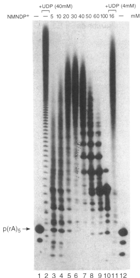
Figure 2. Autoradiogram of the gel electrophoretogram of the products from the polymerization of NMNDP + by polynucleotide phosphorylase primed by p(rA) 5 after 24 h: lane 1 and lane 12, 32 P-labelled primer. Substrates: lane 2, 40 mM UDP; lanes 3–10, 5, 10, 20, 30, 40, 50, 60 and 100 mM NMNDP + , respectively; lane 11, 4 mM UDP and 16 mM NMNDP + . The concentration of PNPase was 20 U/ml.
