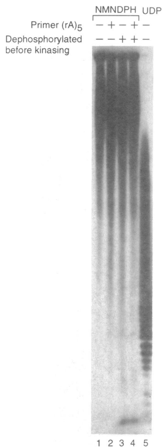
Figure 4. Autoradiogram of the products from the de novo polymerization of NMNDPH by polynucleotide phosphorylase. The polymeric products were kinased directly (lanes 1 and 2) or after dephosphorylation with alkaline phosphatase (lanes 3 and 4).
