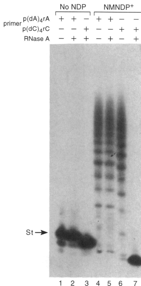
Figure 7. Ribonuclease A analysis of the polymeric products from the primed polymerization of NMNDP + by polynucleotide phosphorylase. The nature of the primer and the substrate for polymerization is indicated at the top of the Figure. St is the primer (dA) 4 rA.
