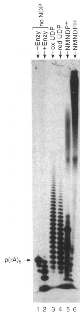
Figure 3. Autoradiogram of the gel electrophoretogram of the products from the polymerization of NMNDPH by polynucleotide phosphorylase using p(rA) 5 as primer after 4 h: lane 1, 32 P-labelled primer; lane 2, primer incubated with PNPase; lane 3, substrate, 1.5 mM UDP; lane 4, substrate, 1.5 mM UDP in reduction buffer; lane 5, substrate, 1.5 mM NMNDP + ; lane 6, substrate, 1.5 mM NMNDPH. The reduction buffer was 1.2% (w) sodium hydrosulfite in 0.20 M Tris, pH 9.0. The concentration of PNPase was 20 U/ml.
