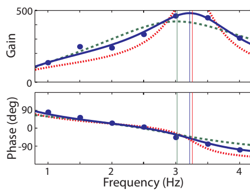
B) EMG to force transfer function
