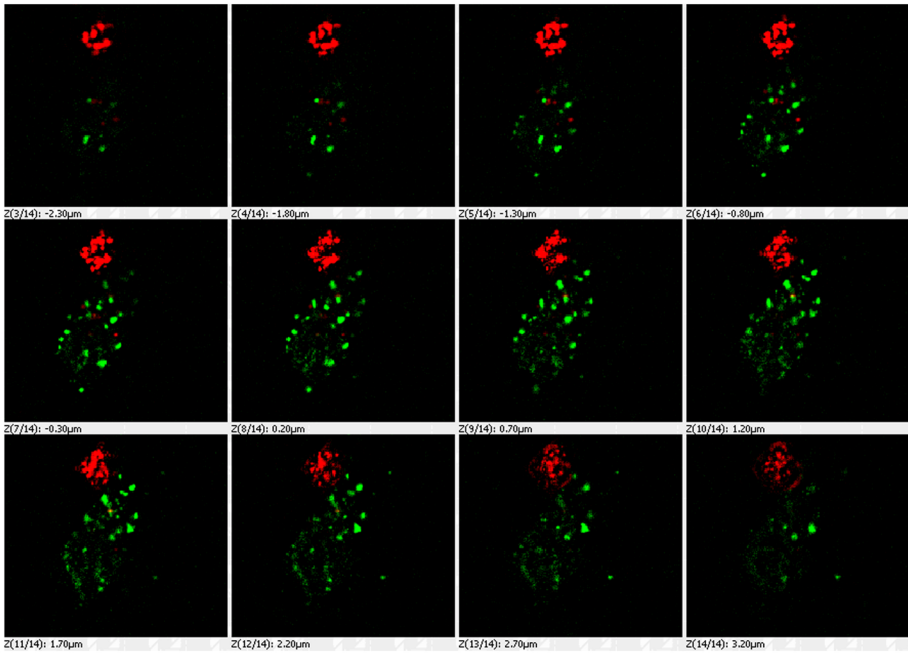
Supplemental Figure 2. Tile array of individual z-sections of 2DL4/EEA1 staining from two cells shown as a max-projection in Figure 8C. Overlaid fluorescence images of individual z-stack sections from two cells stained for EEA1 from each condition ( \pm Triad3A expression). 2DL4 is shown in red and EEA1 is green.
