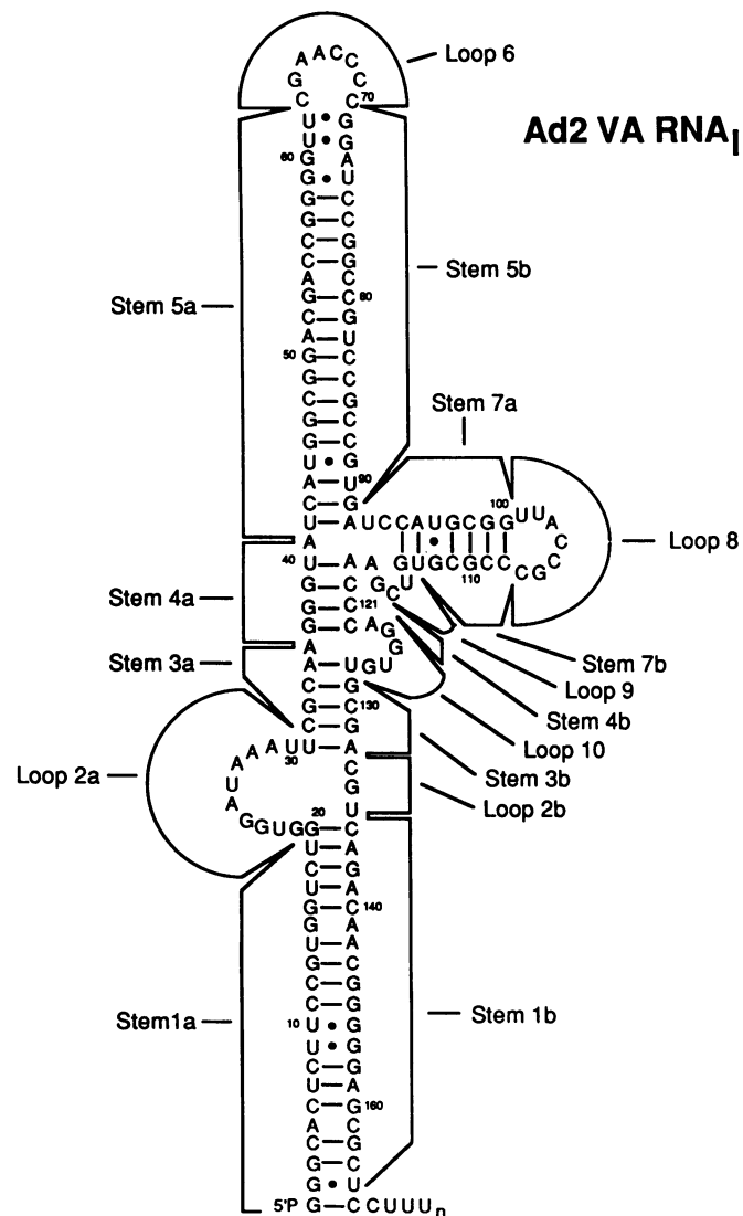
Figure 1. Secondary structure model of Ad2 VA RNA 1 . Stem 1 is the terminal stem, stem 5 and loop 6 comprise the apical stem-loop, and stems 3, 4 and 7 and loops 2, 8, 9 and 10 form the central domain. Stem 4 is phylogenetically conserved.
