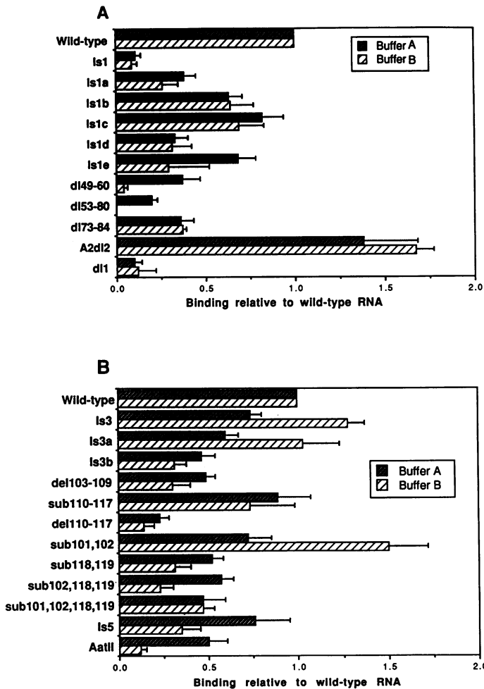
Figure 6. Binding of VA RNA 1 mutants to DAI. Mutant RNAs in the apical stem (A) and the central domain (B) were labeled and reacted with immobilized DAI. Binding was quantified by Cerenkov counting and is expressed relative to the binding of wild-type RNA included as a control in each experiment. Background binding obtained in the absence of DAI was subtracted. Error bars indicate standard errors.
