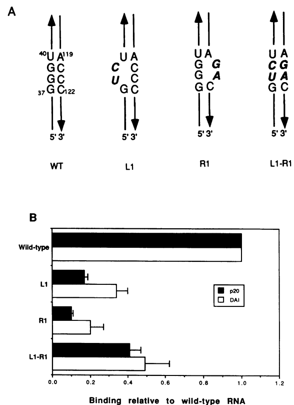
Figure 2. Effects of mutations in conserved stem 4 on binding to DAI and p20. (A) Diagram of mutant sequences, showing the alterations in bold italic type. (B) Binding of 3' end labeled wild-type and mutant RNAs to immobilized DAI or p20 in buffer B, expressed relative to that of wild-type RNA. Error bars show standard errors.
