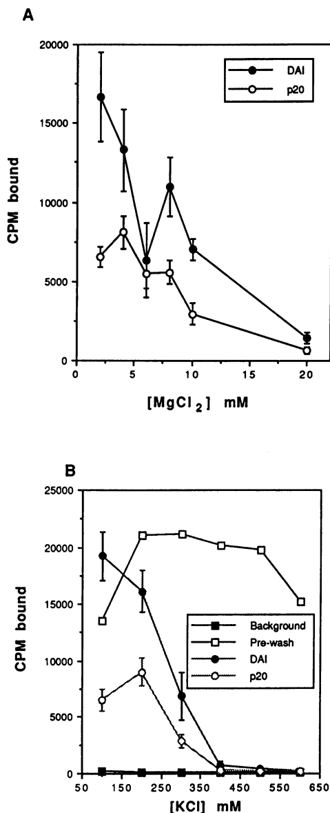
Figure 3. Influence of KCl and MgCl 2 concentrations on the binding of VA RNA 1 to DAI and p20. Wild-type VA RNA 1 was 3' end-labeled and reacted with immobilized DAI or p20 under buffer B conditions except that either (A) MgCl 2 or (B) KCl concentrations were varied. For the pre-wash control in (B), the DAI-containing immune complexes were washed at the KCl concentration indicated, then washed twice to bring the KCl concentration back to 100mM KCl prior to the RNA binding reaction and subsequent washing at 100mM KCl. The control background binding reaction was with protein G-Sepharose only. Error bars show standard deviations.
