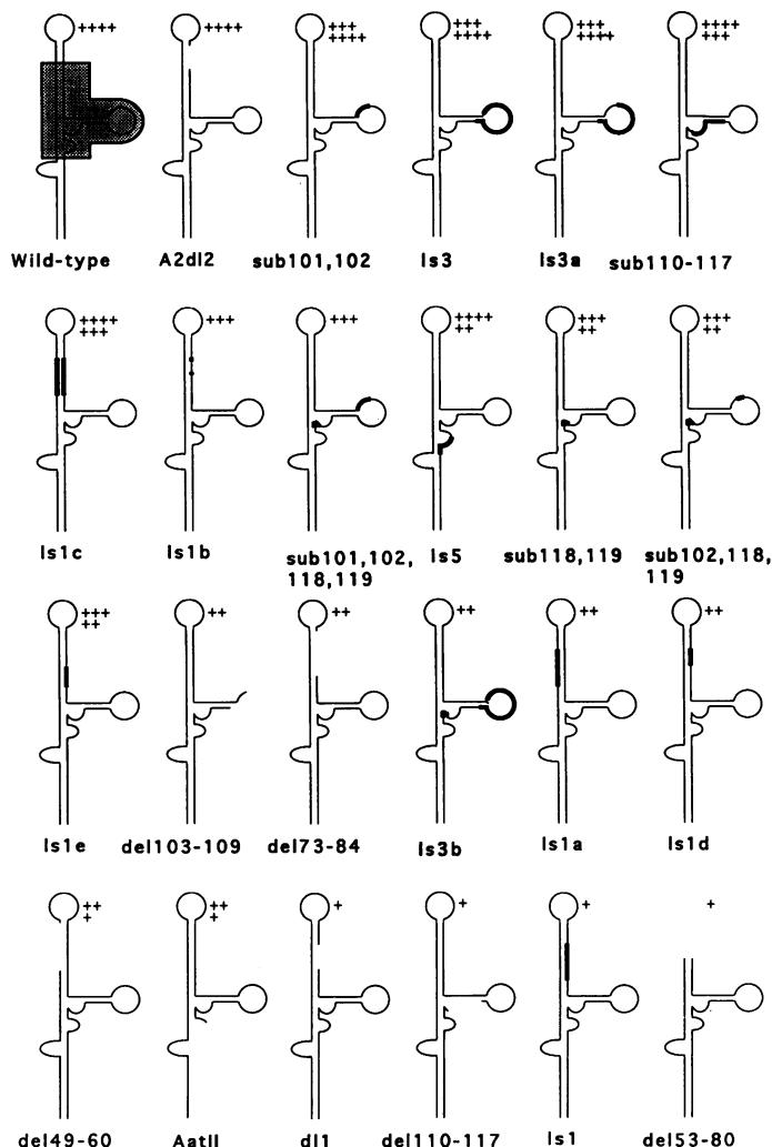
Figure 4. Schematic representation of the mutations. Superimposed on the wild-type VA RNA 1 structure, deletions are represented by gaps and substitutions by thick lines. The mutants are presented in order of decreasing binding efficiency, ranked as in Table 2. The stippled area outlines the region of wild-type VA RNA 1 that is protected from chemical and nuclease attack by DAI (29).
