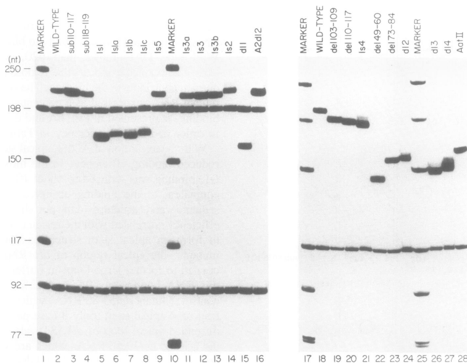
Figure 5. Mobility of wild-type and mutant RNAs. Each labeled VA RNA was mixed with marker RNAs and subjected to electrophoresis in 7M urea/polyacrylamide gels. Detection was by autoradiography.
