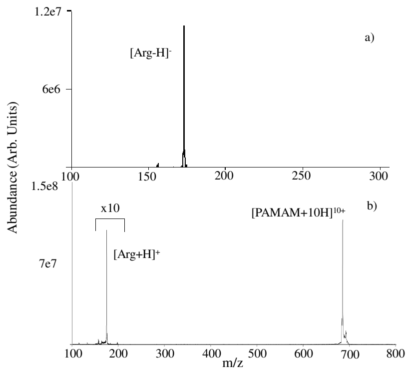
Figure S-1 – a) Isolated deprotonated arginine prior to ion/ion reaction. b) Post-ion/ion reaction positive ion mass spectrum after reaction of deprotonated arginine with the 10+ charge state of PAMAM generation 3.0.
