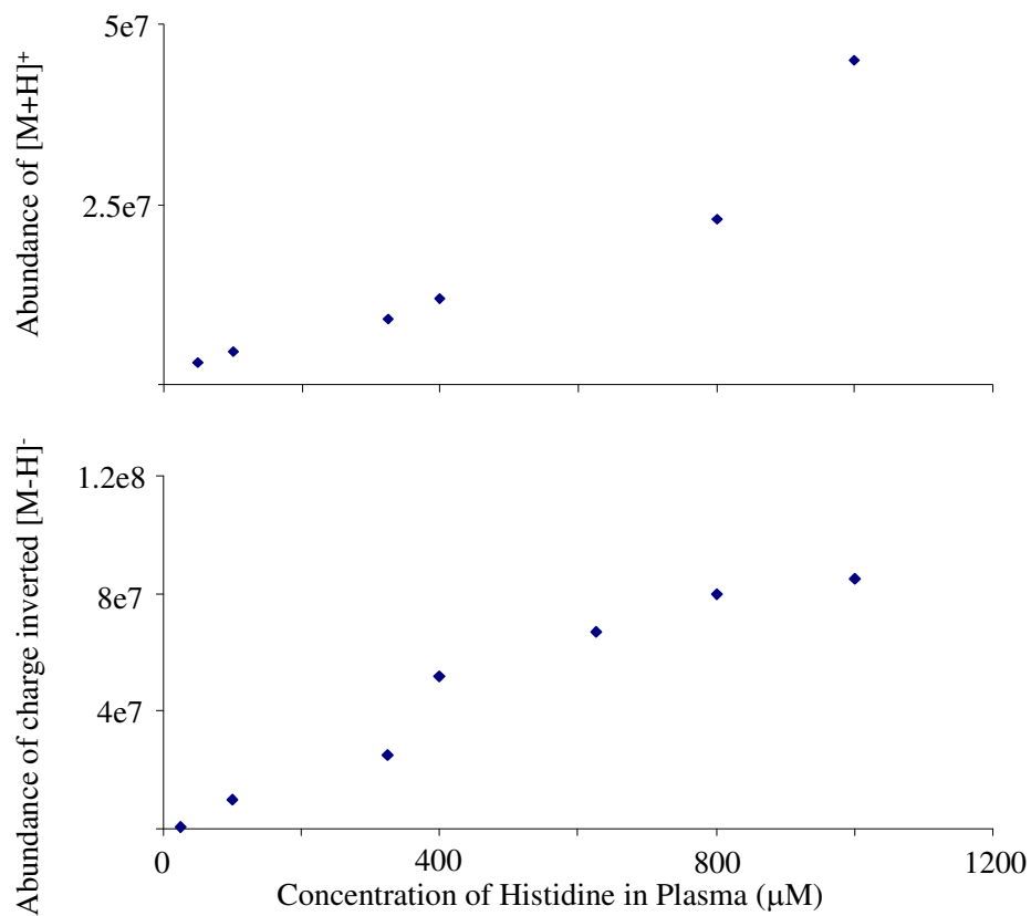
Figure S-4 – Response curves for histidine spiked in precipitated plasma. (a) Protonated histidine abundance versus concentration observed directly via positive nESI and (b) deprotonated histidine abundance versus concentration following charge inversion.
