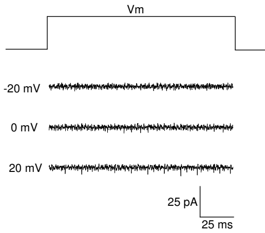
Supplemental Figure 3. Representative traces obtained after the application of depolarizing voltage steps from -20 to +20 mV in \text{Ca}_v\beta_3/\alpha_2\delta -1 transfected HEK-293 cells.
