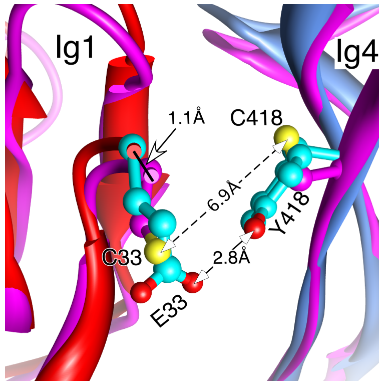
Fig. S1. Comparison of the homology models of WT-L1 and E33C/Y418C reduced. The wild type model is colored as in Fig. 6 A. and the E33C/Y418C reduced model as in Fig. 6B. The Ig4 domains of each model were superimposed.
