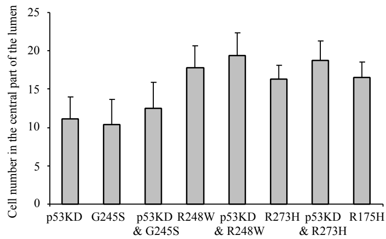
Figure S1. The number of cells in the center of the lumen from MCF10A cells in which a p53 mutant was ectopically expressed along with or without knockdown of endogenous wild-type p53. The number of cells in the central part of spherical structures from serial confocal cross-sections was counted.
