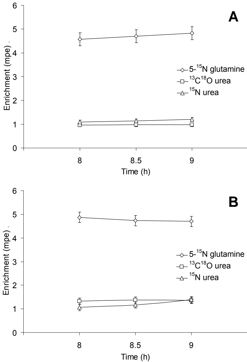
Supplemental Figure 1. Isotopic plateau enrichments of 5- 15 N glutamine, 13 C 18 O urea and 15 N urea in control (panel A) and partial OTCD (panel B) subjects. Each symbol represents the treatment and subject adjusted mean (control n=14; pOTCD n=21) and errors bars are SEM.
