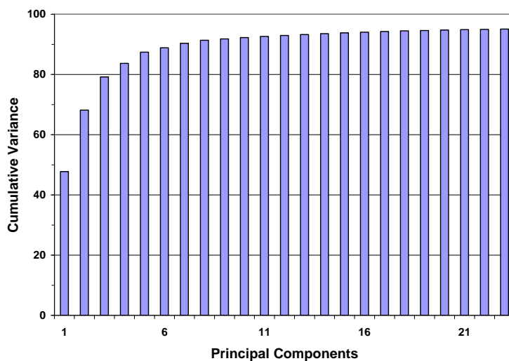
Figure S1. Scree plot showing the cumulative variance captured by each principal component in rank order. 7 and 23 principal components are required to capture 90% and 95% of the total variance, respectively.
