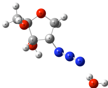
Figure S6. Geometry-optimized structure of 2-azido-1,2-dideoxyribose with one water molecule containing a \sigma -H-bond between the azide group and the water molecule.
