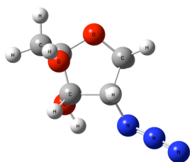
Figure S5. Geometry-optimized structure of 2-azido-1,2-dideoxyribose.
