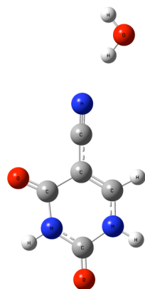
Figure S9. Geometry-optimized structure of 5-cyanouracil with one water molecule containing a \sigma -H-bond between the nitrile group and the water molecule.
