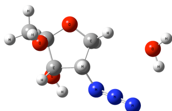
Figure S7. Geometry-optimized structure of 2-azido-1,2-dideoxyribose with one water molecule containing a \pi -H-bond between the azide group and the water molecule.
