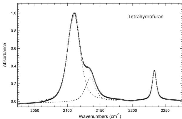
Figure S2. FTIR absorbance spectrum of \text{N}_3\text{CNdU} in tetrahydrofuran (open circles) recorded at 293 K where the maximum absorbance has been normalized to unity. The azide IR absorbance band was fit (solid curve) to two line shapes (dashed curves) described by Eqn. 1 and the nitrile IR absorbance band was fit (solid curve) to one line shape described by Eqn. 1. The fits represent the minimum number of line shapes required to fit the experimental spectrum.
