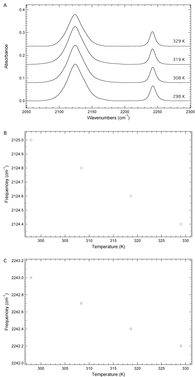
Figure S4. A. Temperature dependent FTIR absorbance spectra of \text{N}_3\text{CNDU} dissolved in water recorded from 293 to 329 K in \sim 10 K increments. B. Azide asymmetric stretching frequency dependence on temperature. C. Nitrile symmetric stretching frequency dependence on temperature.
