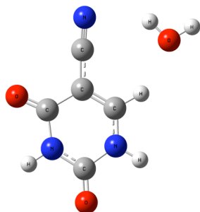
Figure S10. Geometry-optimized structure of 5-cyanouracil with one water molecule containing a \pi -H-bond between the nitrile group and the water molecule.
