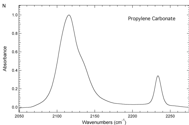
Figure S1. FTIR absorbance spectra of N 3 CNDU dissolved in water (A), methanol (B), propanol (C), 1-butanol (D), t -butanol (E), trifluoroethanol (F), tetrahydrofuran (G), dimethyl sulfoxide (H), acetone (I), nitromethane (J), formamide (K), N-methylformamide (L), dimethylformamide (M), propylene carbonate (N) recorded at 293 K with a concentration of 50 mM. The maximum absorbance of each spectrum has been normalized to unity.
