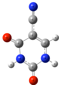
Figure S8. Geometry-optimized structure of 5-cyanouracil.
