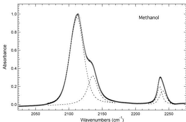
Figure S3. FTIR absorbance spectrum of \text{N}_3\text{CNdU} in methanol (open circles) recorded at 293 K where the maximum absorbance has been normalized to unity. The azide IR absorbance band was fit (solid curve) to two line shapes (dashed curves) described by Eqn. 1 and the nitrile IR absorbance band was also fit (solid curve) to two line shape described by Eqn. 1. The fits represent the minimum number of line shapes required to fit the experimental spectrum.
