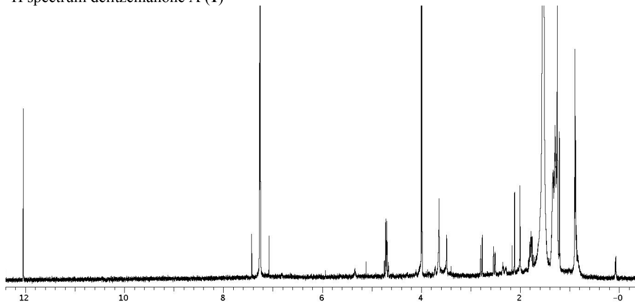
^{13}\text{C} spectrum delitzchianone A (1)
