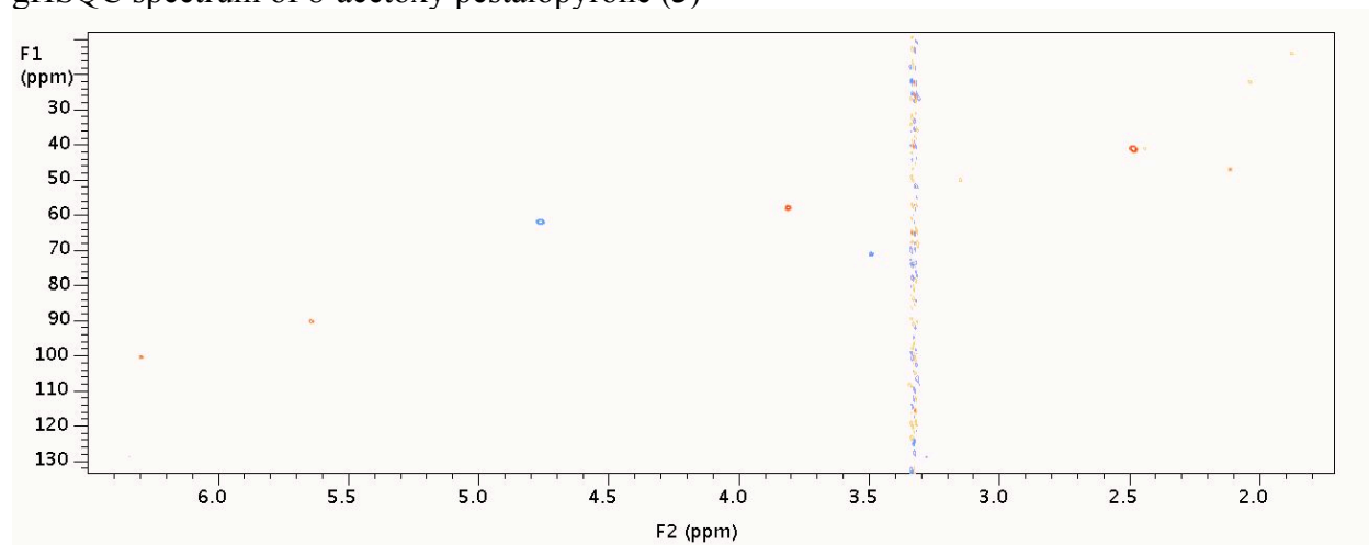
gHSQC spectrum of 8-acetoxy pestalopyrone ( 3 )
