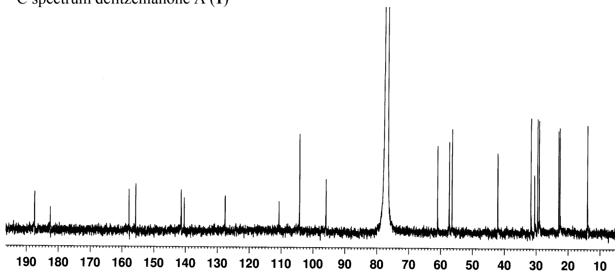
^{13}\text{C} spectrum delitzchianone A (1)
