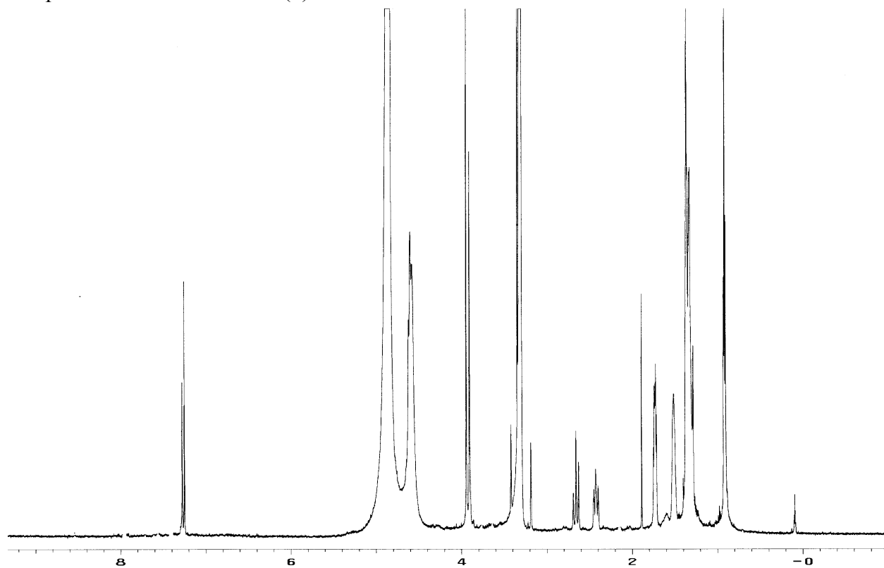
^1\text{H} spectrum delitzchianone B (2)
