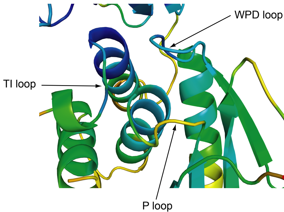
Supplemental Figure S1 The B-factor distribution of the cytoplasmic region of Ci-VSP. (A) The B-factor distribution in the overall Ci-VSP cytoplasmic region is represented in rainbow colors. The higher B-factor of the residue is shown in red color, and the lower B-factor in blue. The maximum B-factor of the residue is 63.19 Å 2 , and the minimum is 12.34 Å 2 . (B) Close-up view of Ci-VSP active site.
