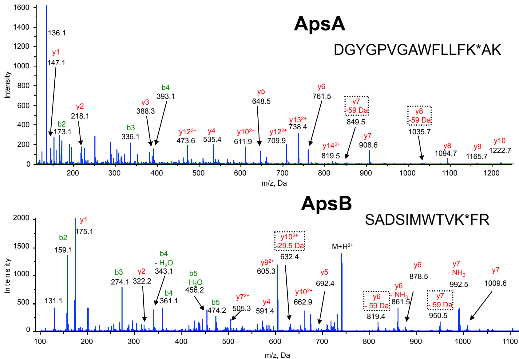
Figure S7: Q-Star MS/MS data for ApsA, ApsB, and DsrC post-translational modifications.
