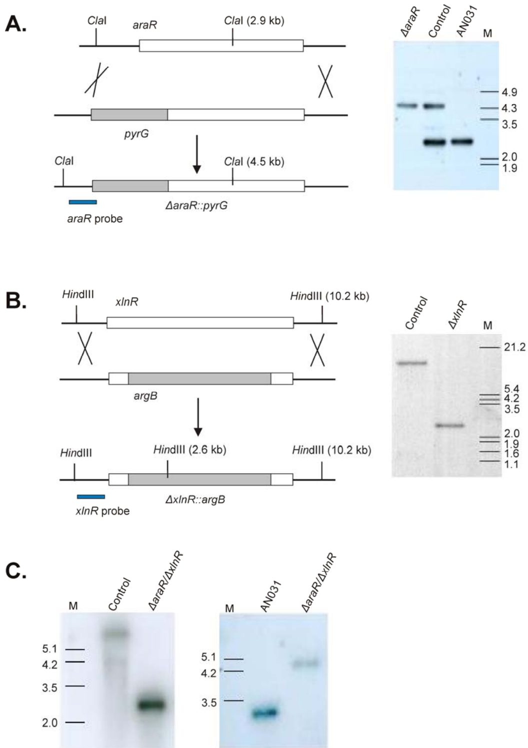
Supplemental Fig. 1. Schematic cloning strategies and Southern blot analysis of the A. nidulans \Delta araR , \Delta xlnR and \Delta araR/\Delta xlnR strains. A. Strategy and Southern analysis of the araR disruptant; B. Strategy and Southern analysis of the xlnR disruptant; C. Southern analysis of the \Delta araR/\Delta xlnR disruptant. Left: Hind III digest. Right: Cla I digest.
