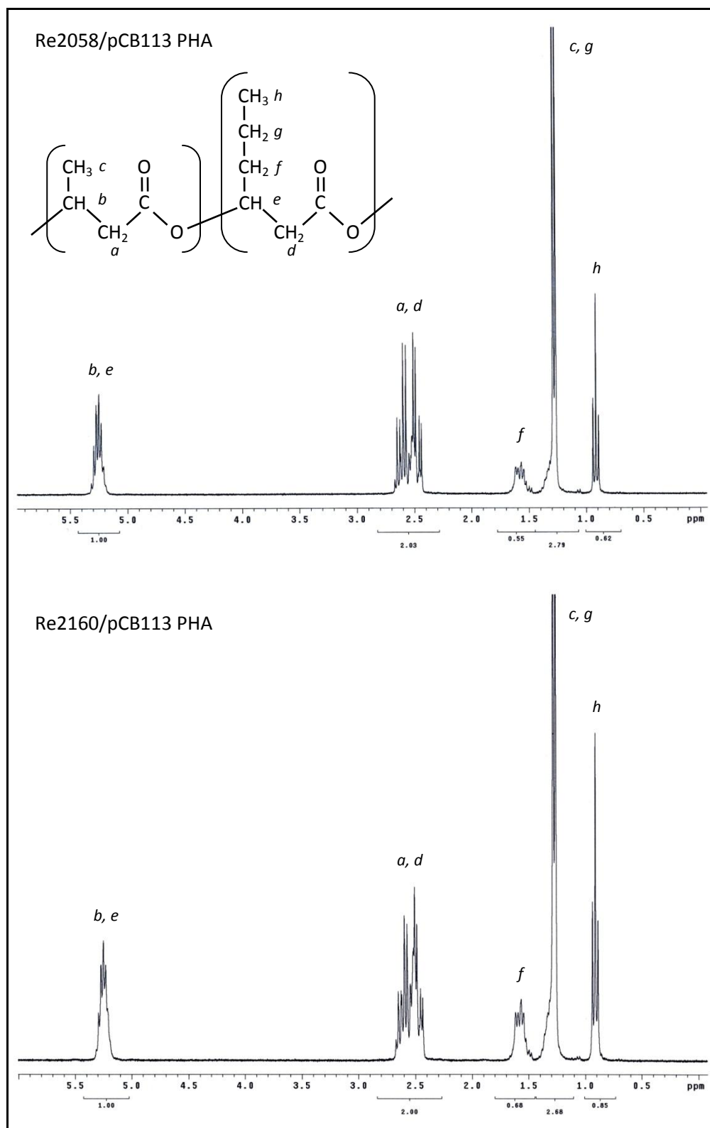
FIG. S2. ^1\text{H} NMR spectra in \text{CDCl}_3 of P(HB- co -HHx) isolated from Re2058/pCB113 and Re2160/pCB113. Based on the area of peak h , it was estimated that the Re2058/pCB113 contained 21mol% HHx, while the Re2160/pCB113 PHA contained 28mol% HHx.
