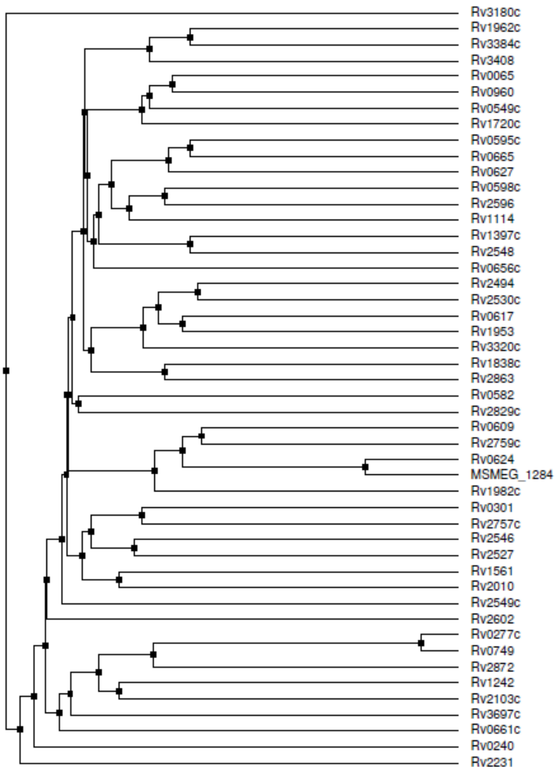
Fig. S2. Phylogenetic tree of VapC proteins from mycobacteria. VapC proteins were aligned using ClustalW2 multiple sequence and server alignment server ( http://www.ebi.ac.uk/Tools/clustalw2/index.html ). The tree was generated in Jalview 2.08.1 based on percentage identity between sequences.
