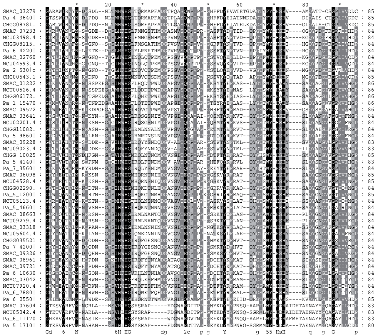
Fig. (S1). Clustal X Alignment of MCOs from Neurospora crassa , Sordaria macrospora , Chaetomium globosum and Podospora anserina . Alignment includes amino acid region of laccase L1 and L2 signature sequences.
